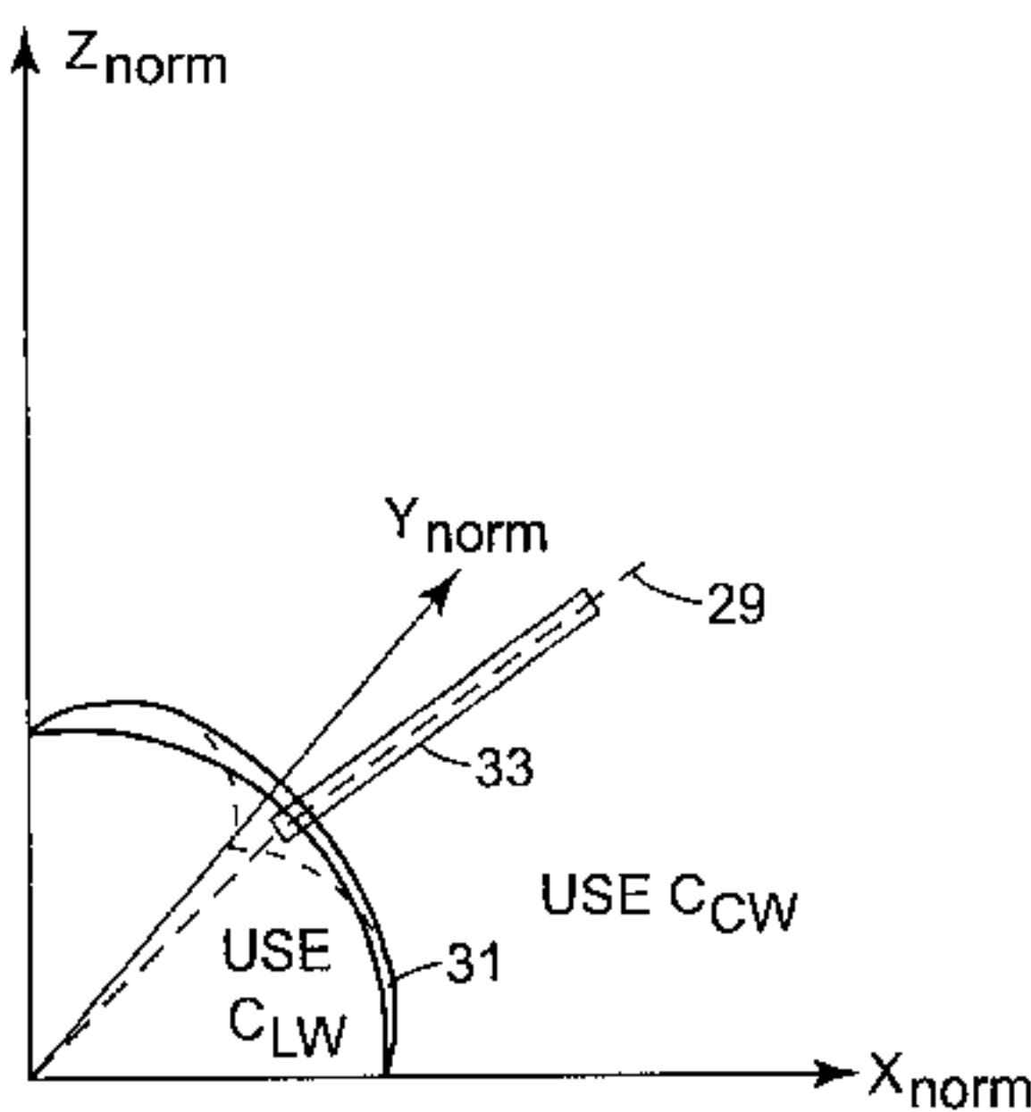
USE OF LOCAL WHITE POINT C LW AND COMMON WHITE POINT C CW , FOR DETERMINING Y-REFERENCE AND WHITE REFERENCE VECTOR, IN RELATION TO NORMALIZED ORIGINAL COLOR DATA TRISTIMULUS VALUES X norm , Y norm , AND Z norm .
