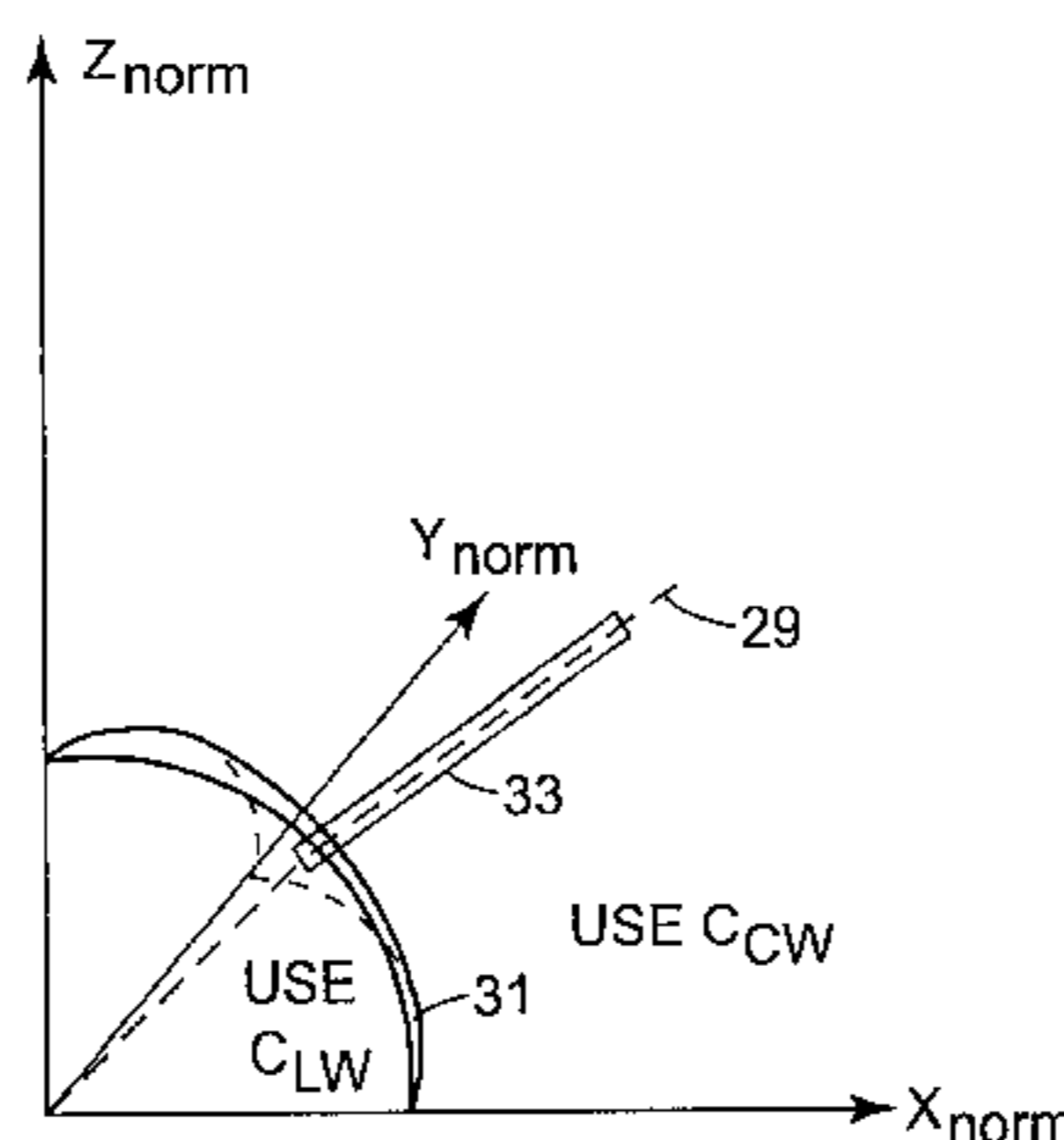
USE OF LOCAL WHITE POINT C LW AND COMMON WHITE POINT C CW , FOR DETERMINING Y-REFERENCE AND WHITE REFERENCE VECTOR, IN RELATION TO NORMALIZED ORIGINAL COLOR DATA TRISTIMULUS VALUES X norm , Y norm , AND Z norm .
