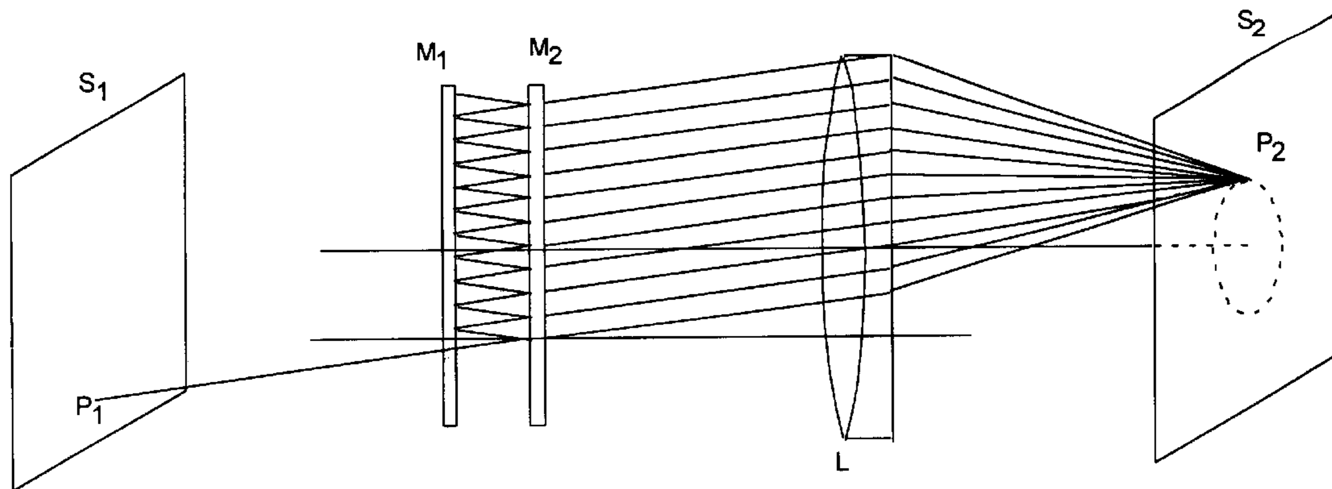
Figure 1. Prior art of a Fabry-Perot interferometer.
