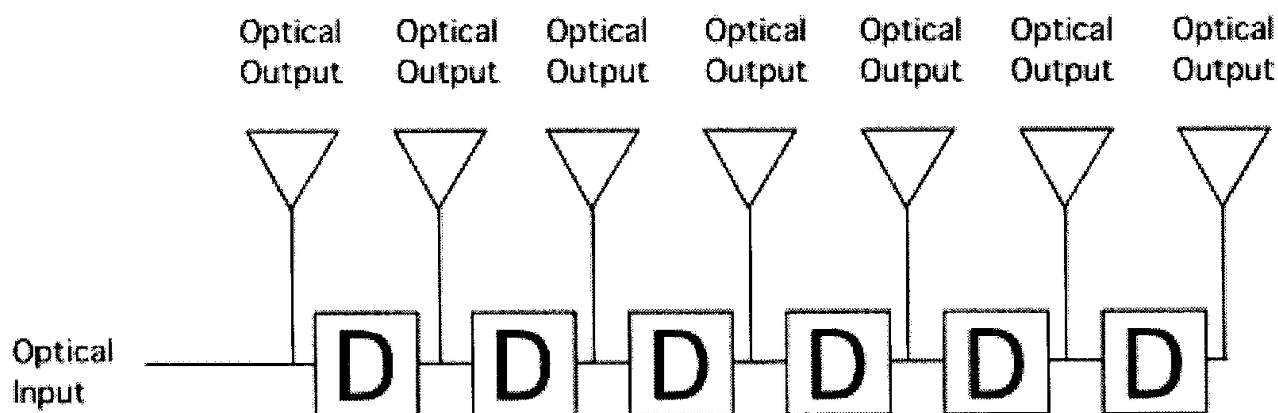
Figure 10. Functional block diagram of an OTDL device shown in a single input arrangement.
