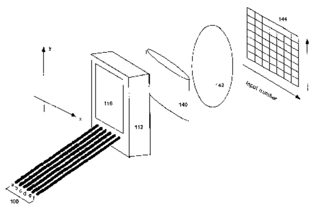
Example embodiment of an Optical Tapped Delay Line (OTDL) channelizer system.
