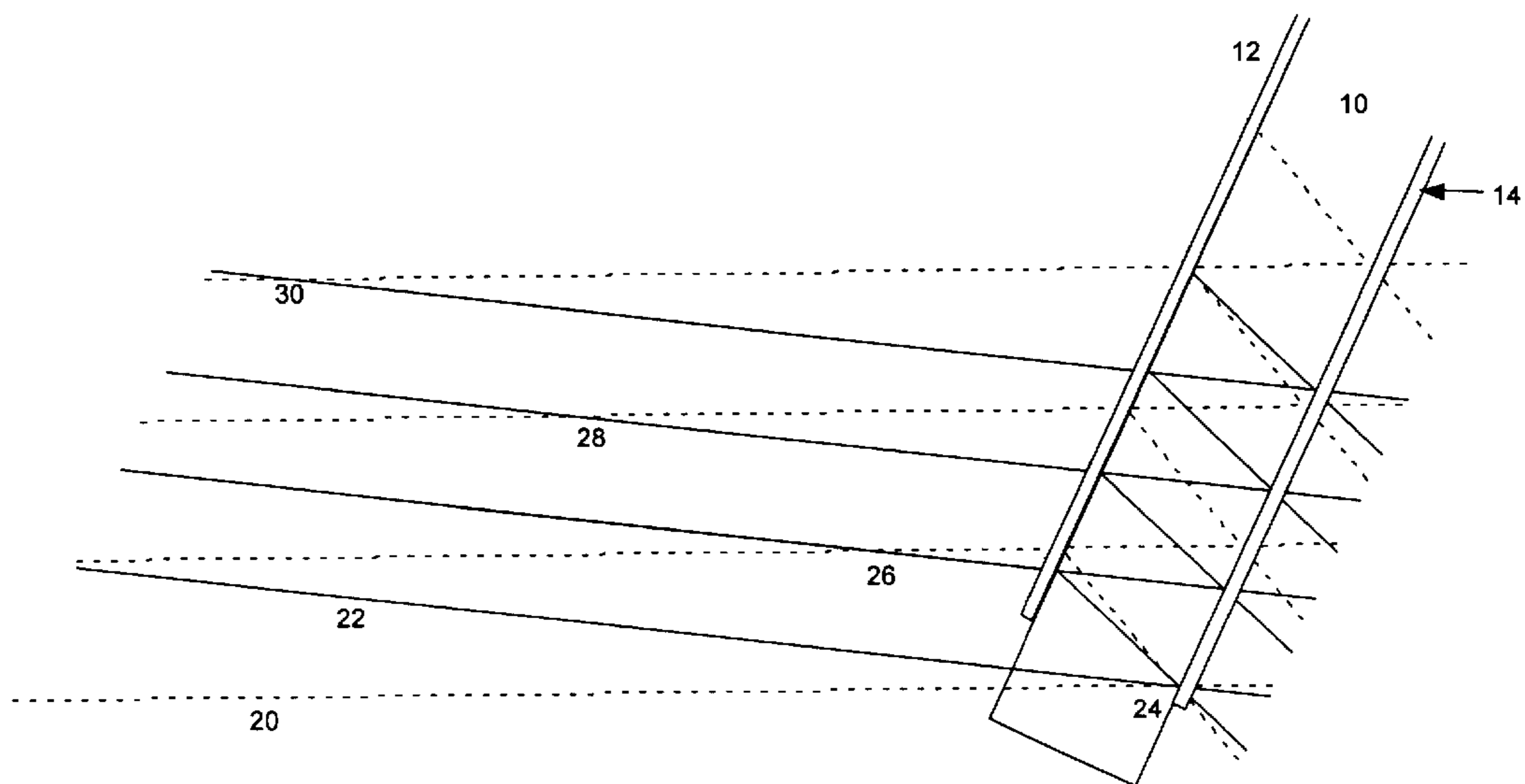
Figure 4. Operation of a prior art VIPA device.
