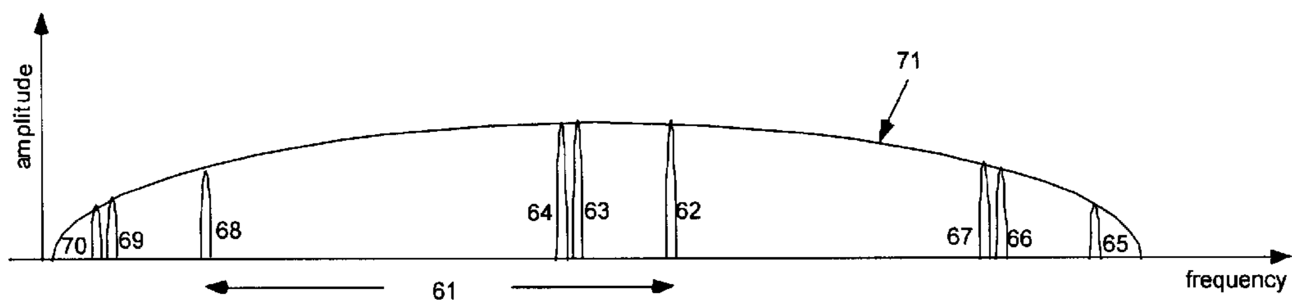
Figure 8. Example optical distribution along the frequency axis of an OTDL channelizer output.
