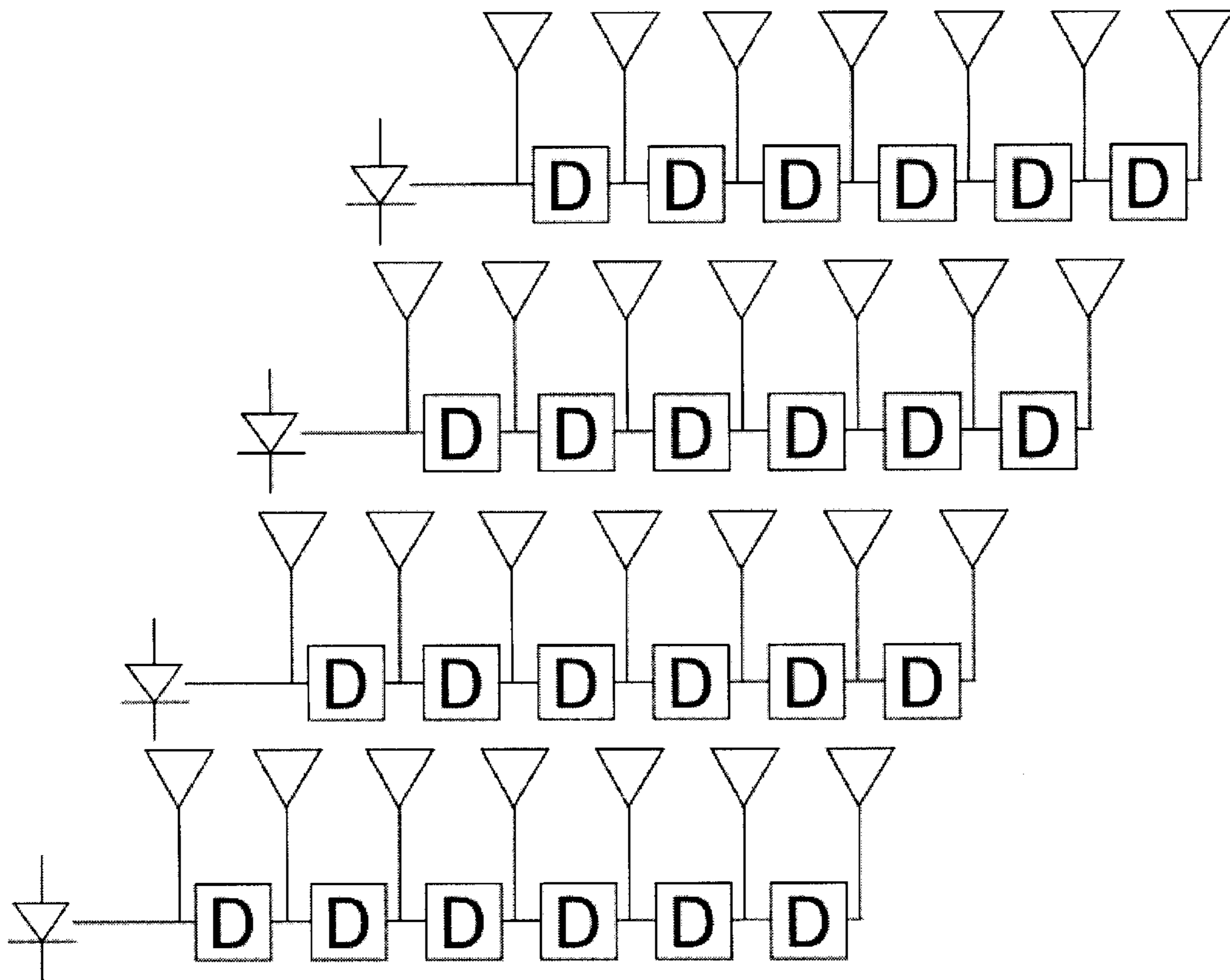
Figure 12. Functional block diagram of an OTDL device shown in a multiple input arrangement.
