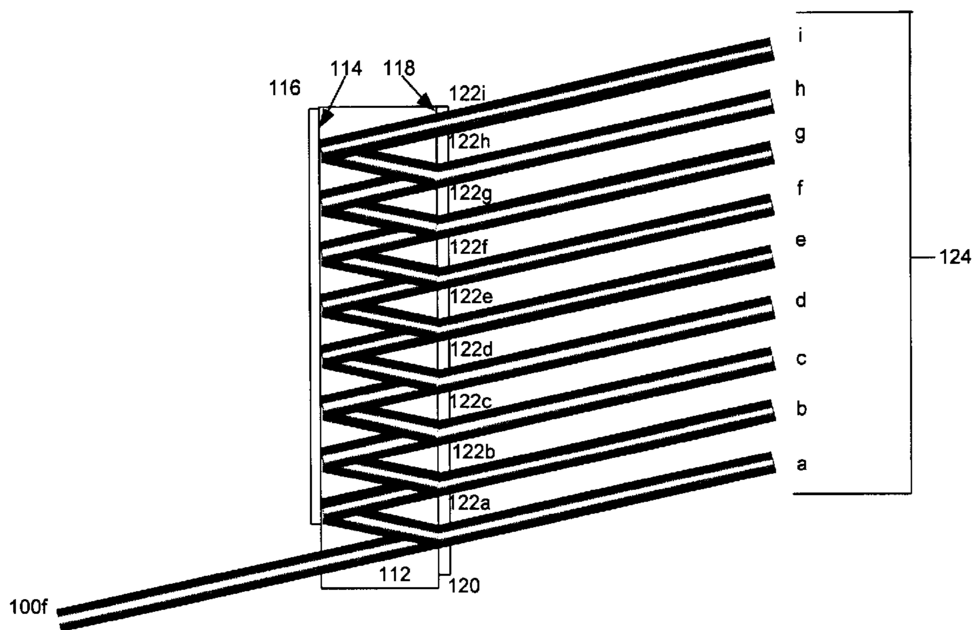
Figure 7. Operational side view of an OTDL device.
