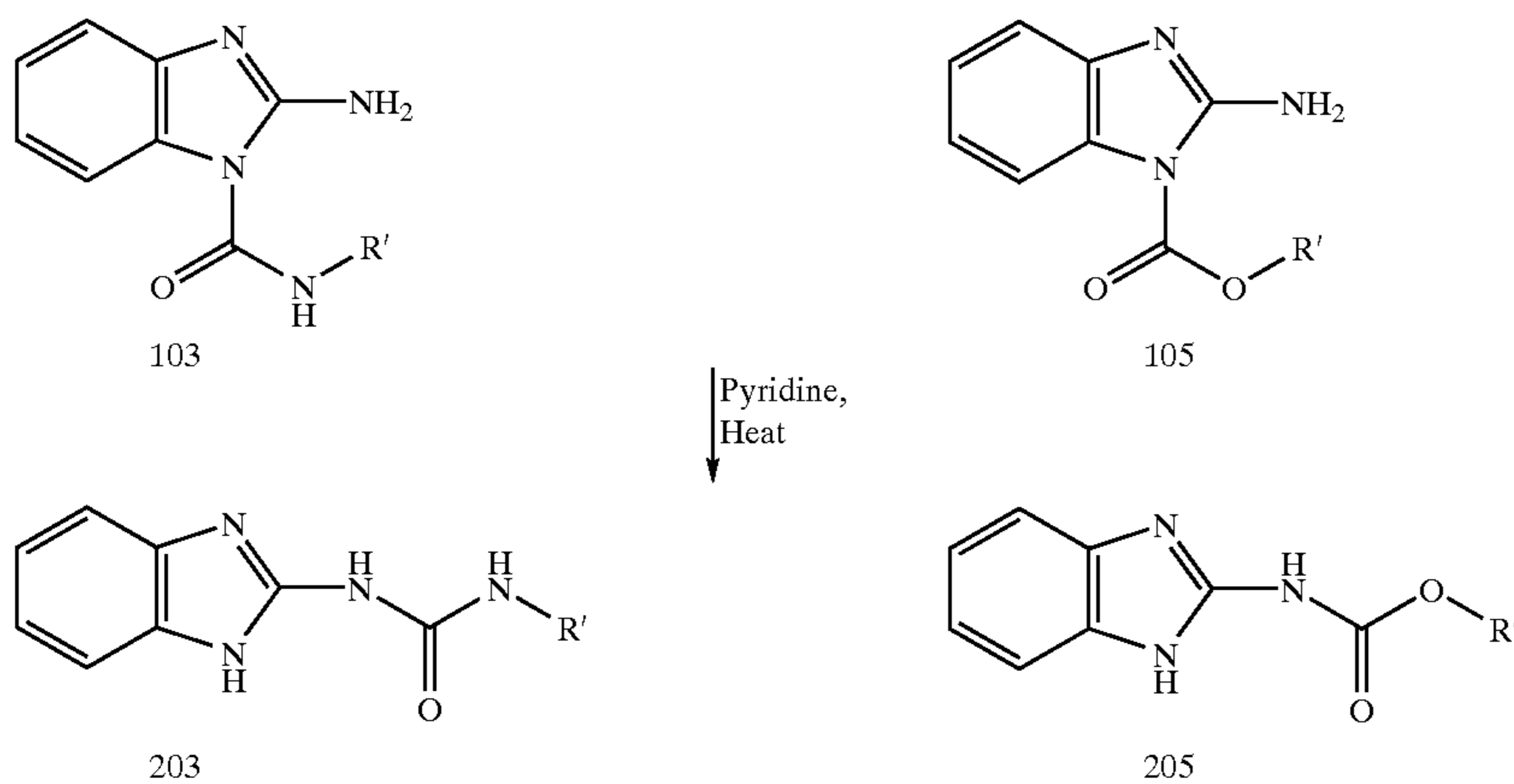
Reaction Scheme 2
