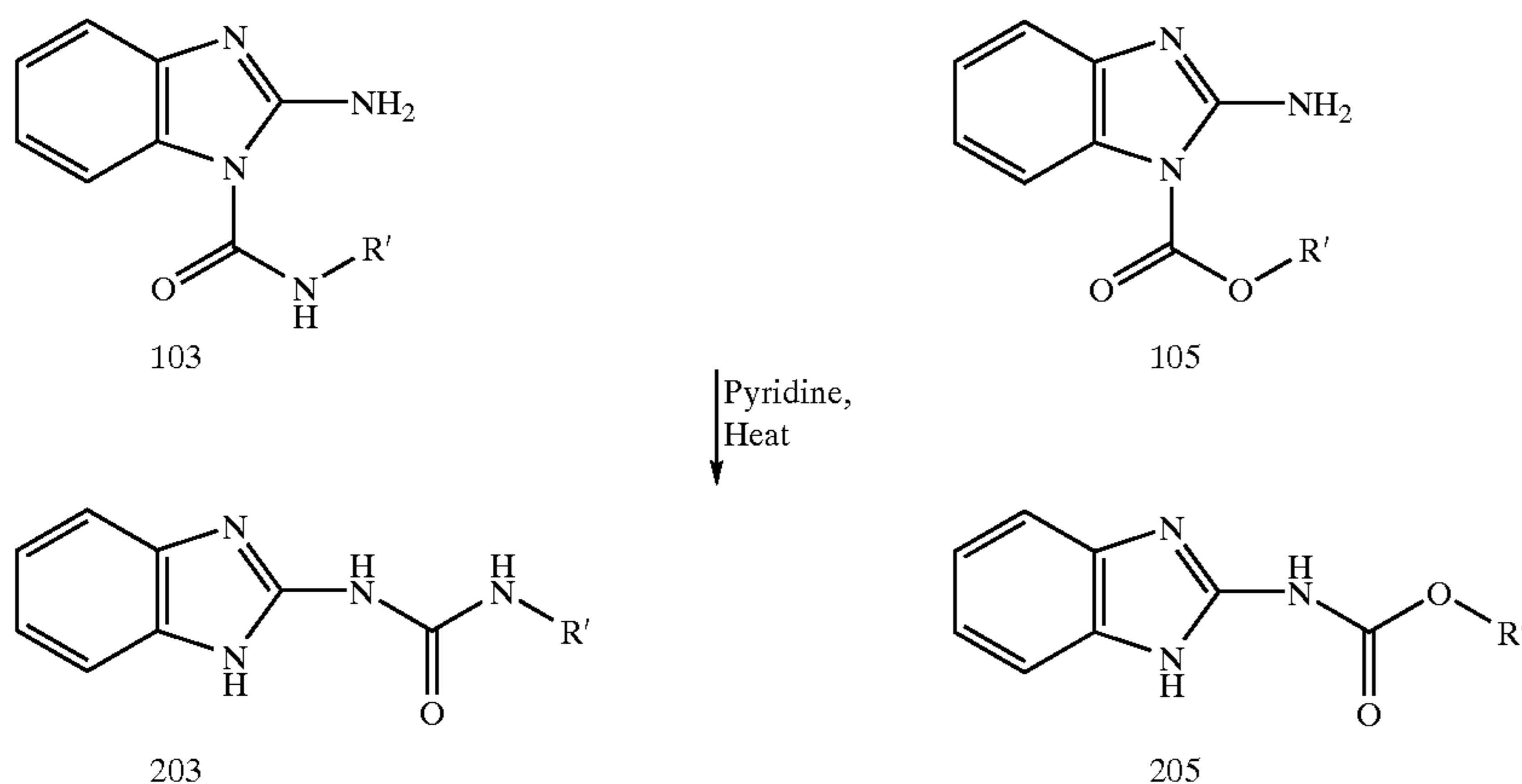
Reaction Scheme 2
