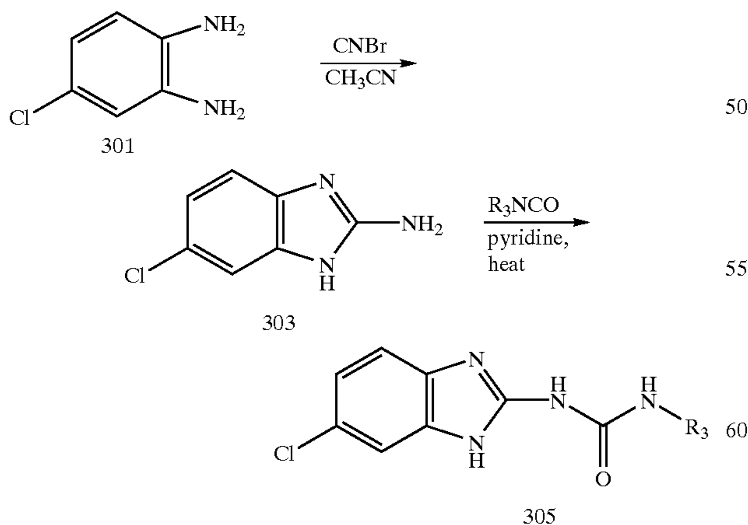
Reaction Scheme 3
