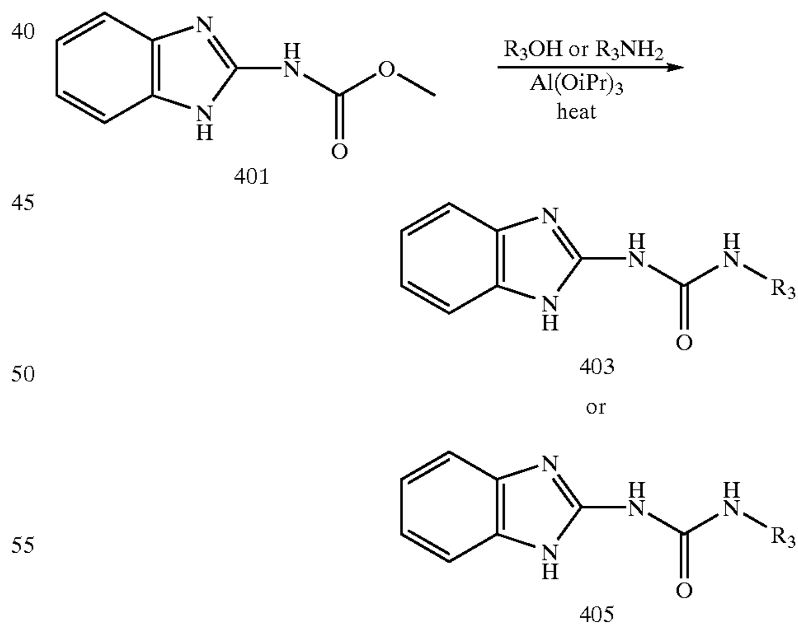
Reaction Scheme 4
