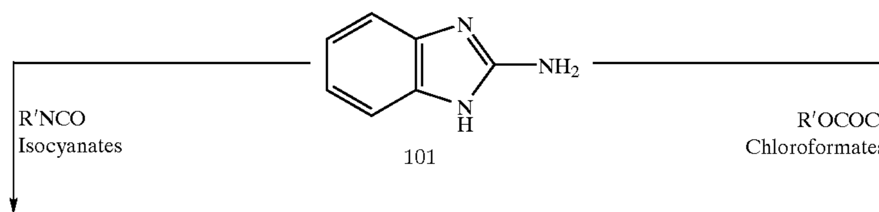
Reaction Scheme 1
