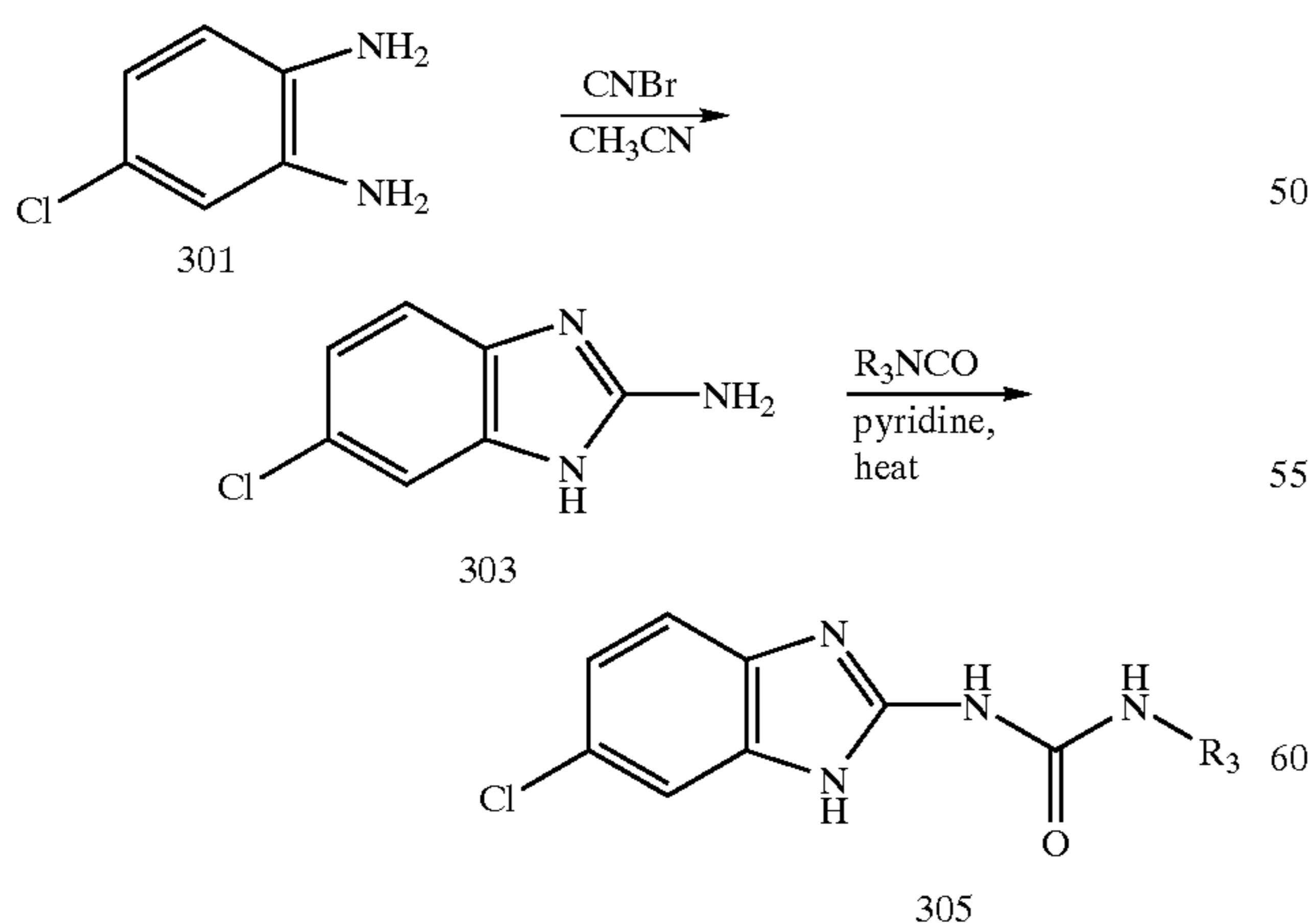
Reaction Scheme 3
