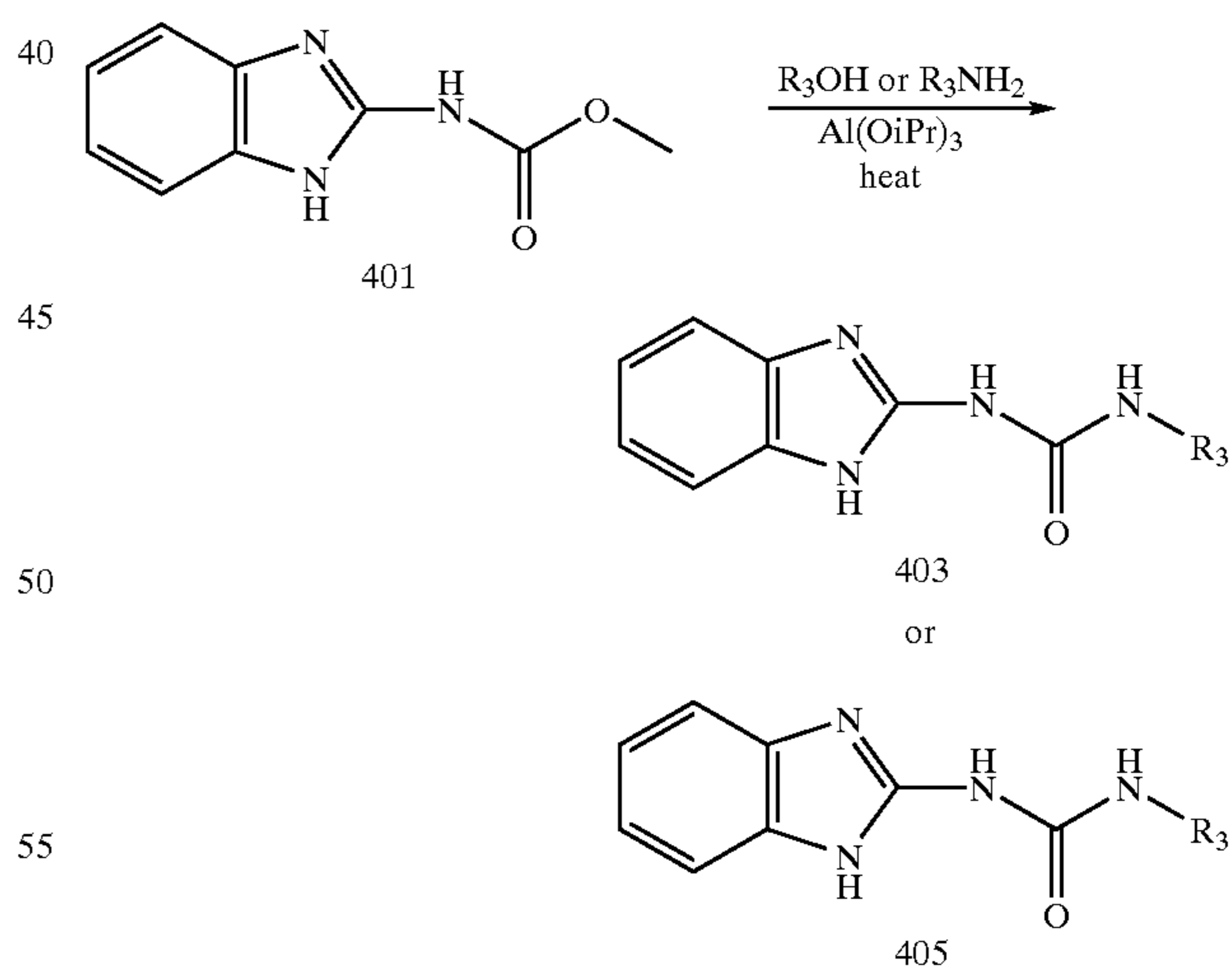
Reaction Scheme 4
