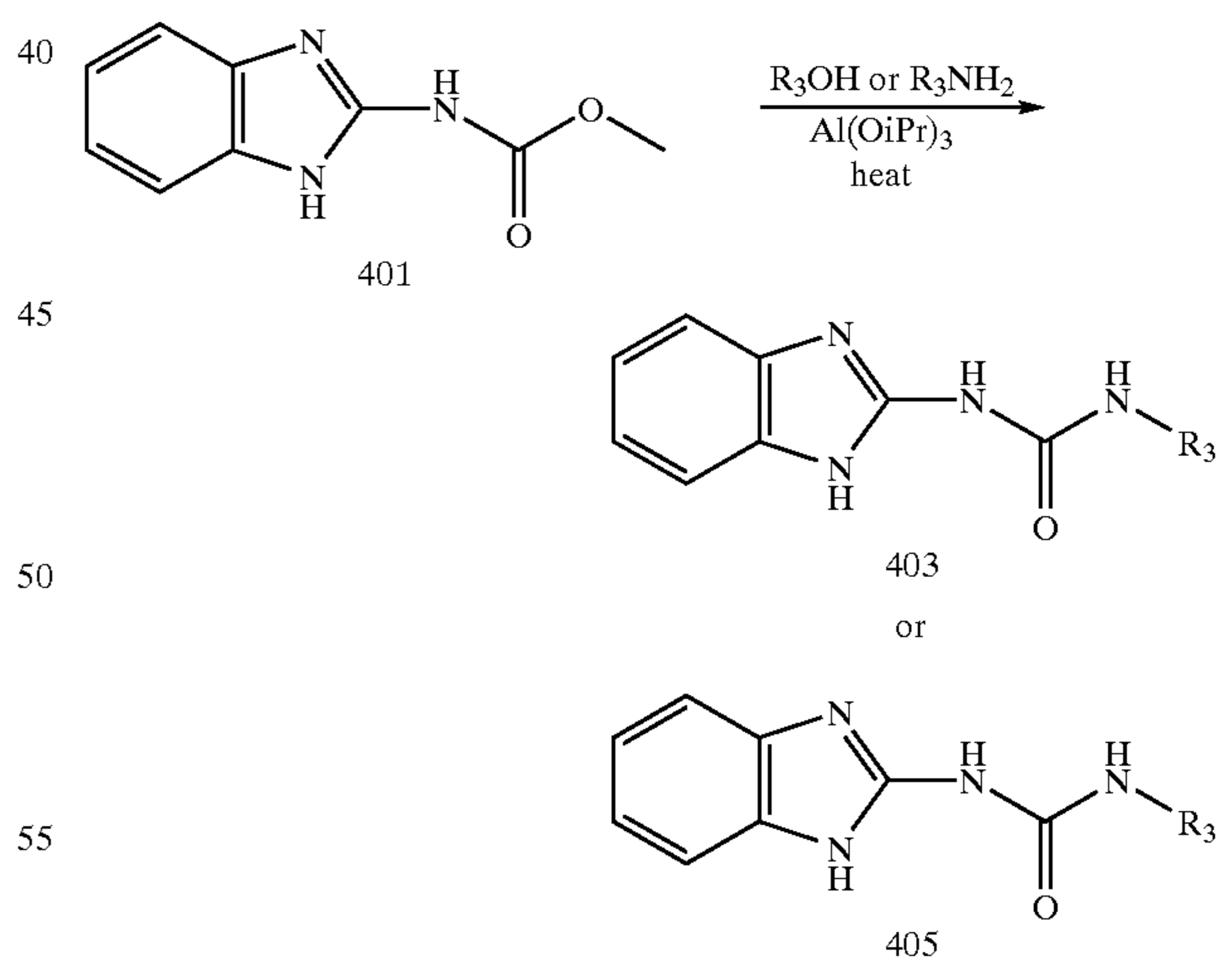
Reaction Scheme 4
