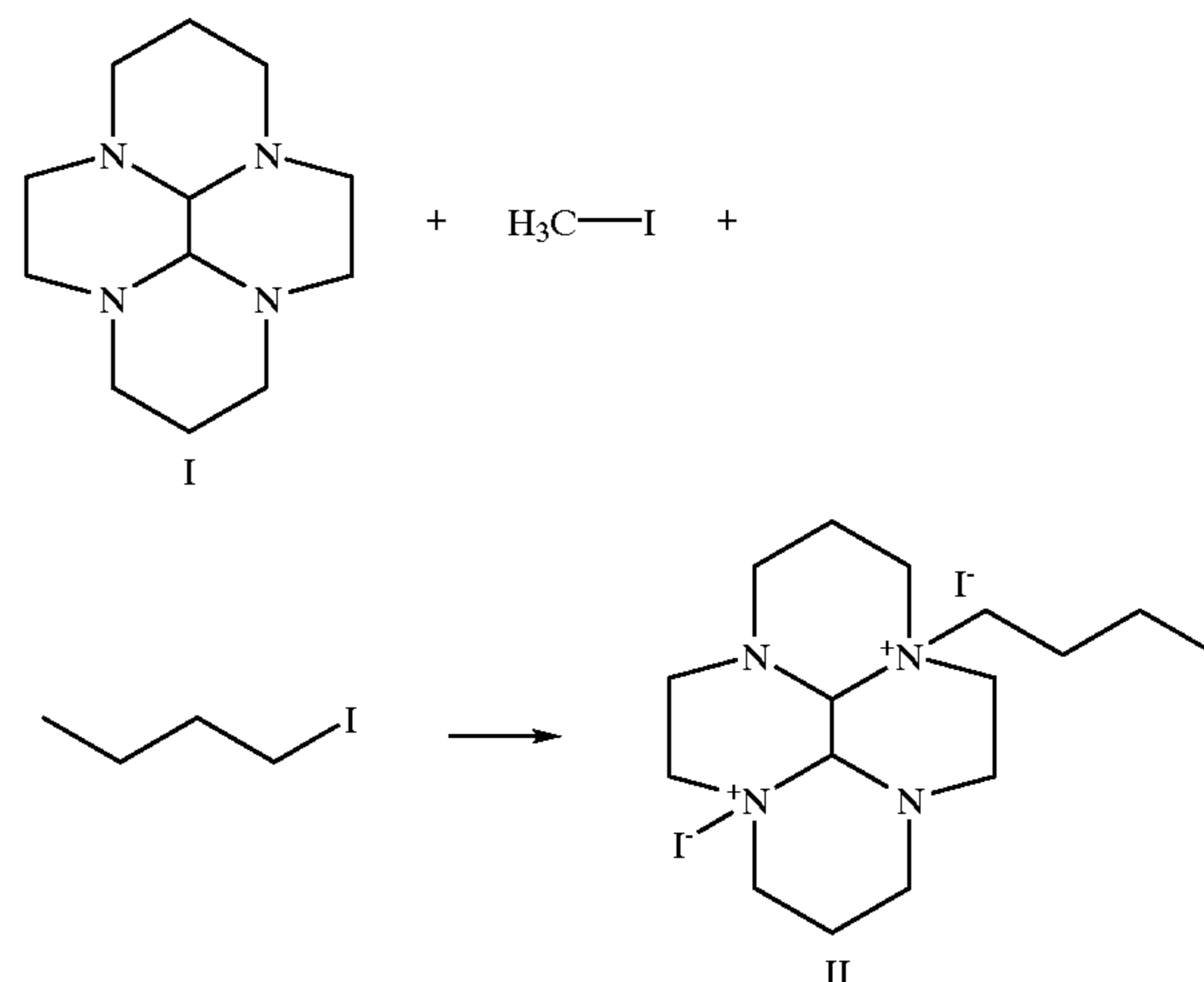
(a) \text{C}_4\text{-Bcyclam} Synthesis
