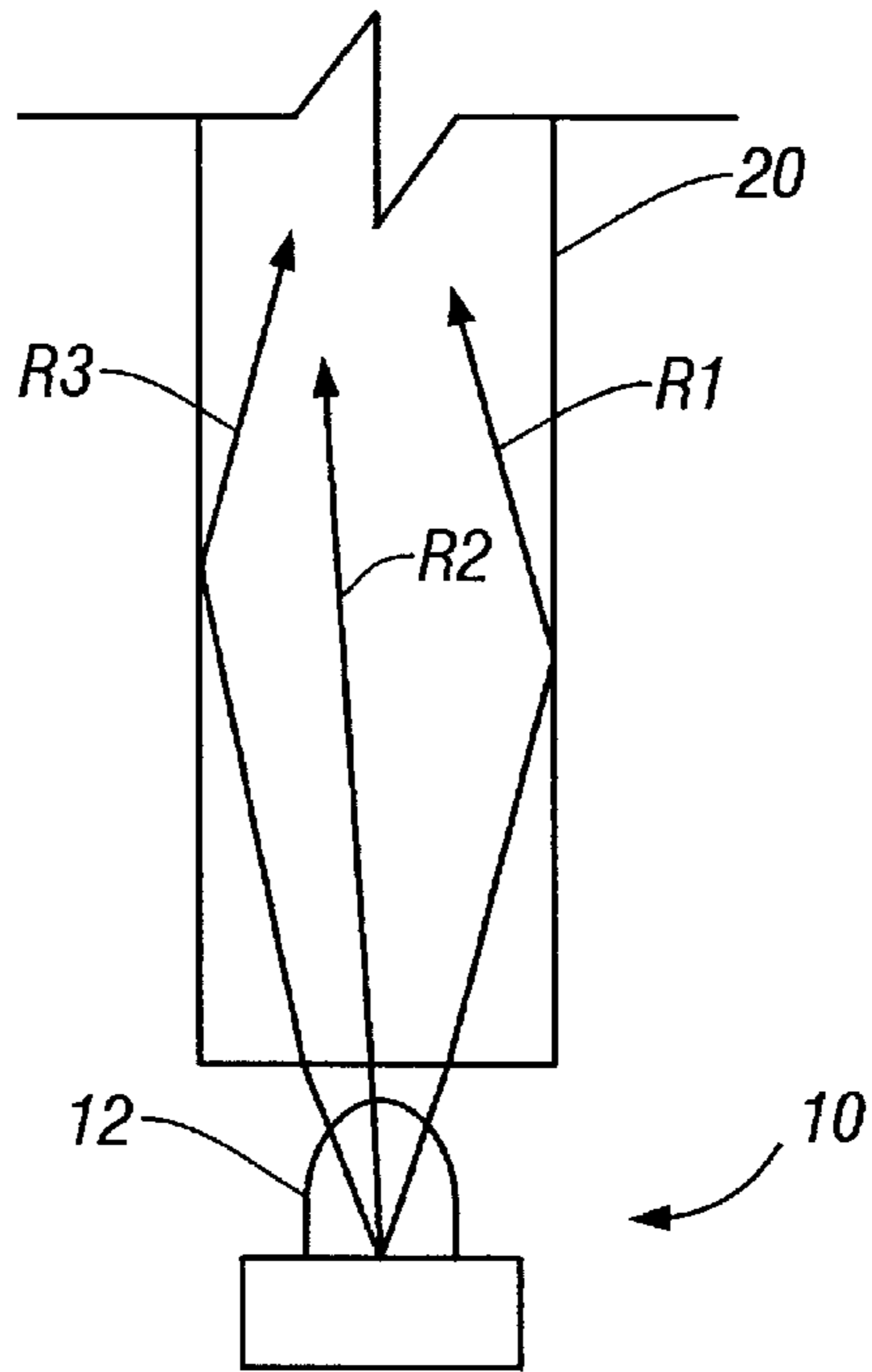
FIG. 2 (Prior Art)
