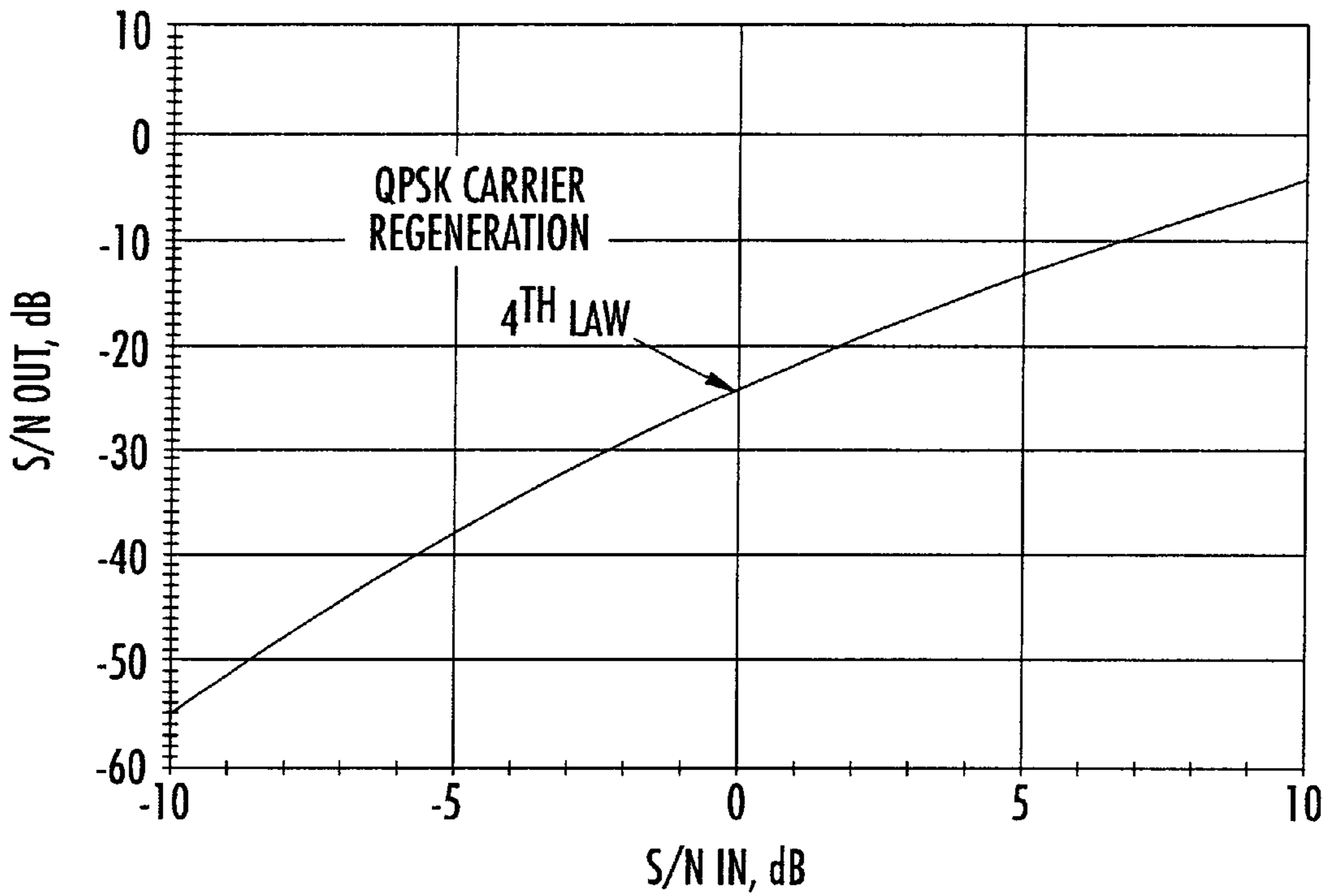
FIGURE 5 (Prior Art)
