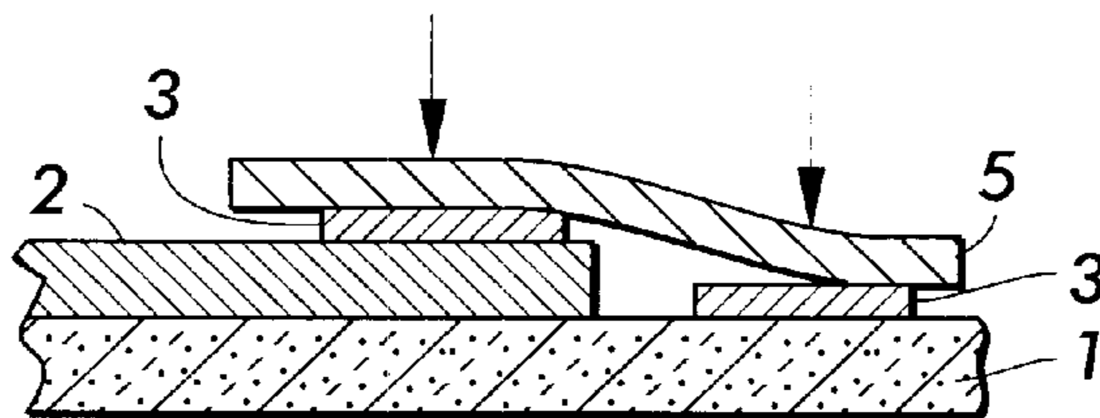
FIG. 2 PRIOR ART
