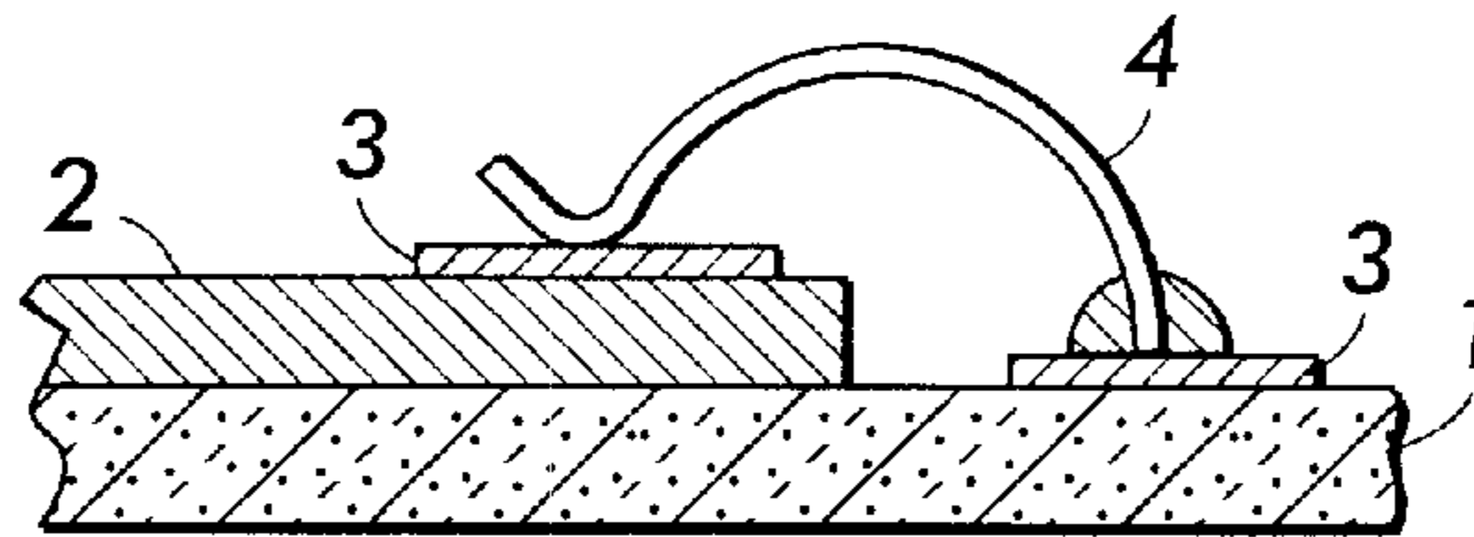
FIG. 1 PRIOR ART
