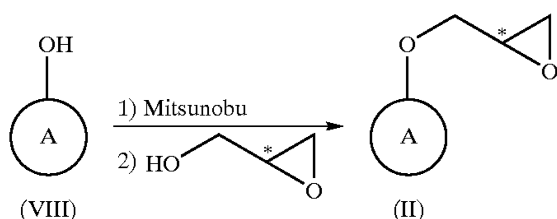
Scheme 2
