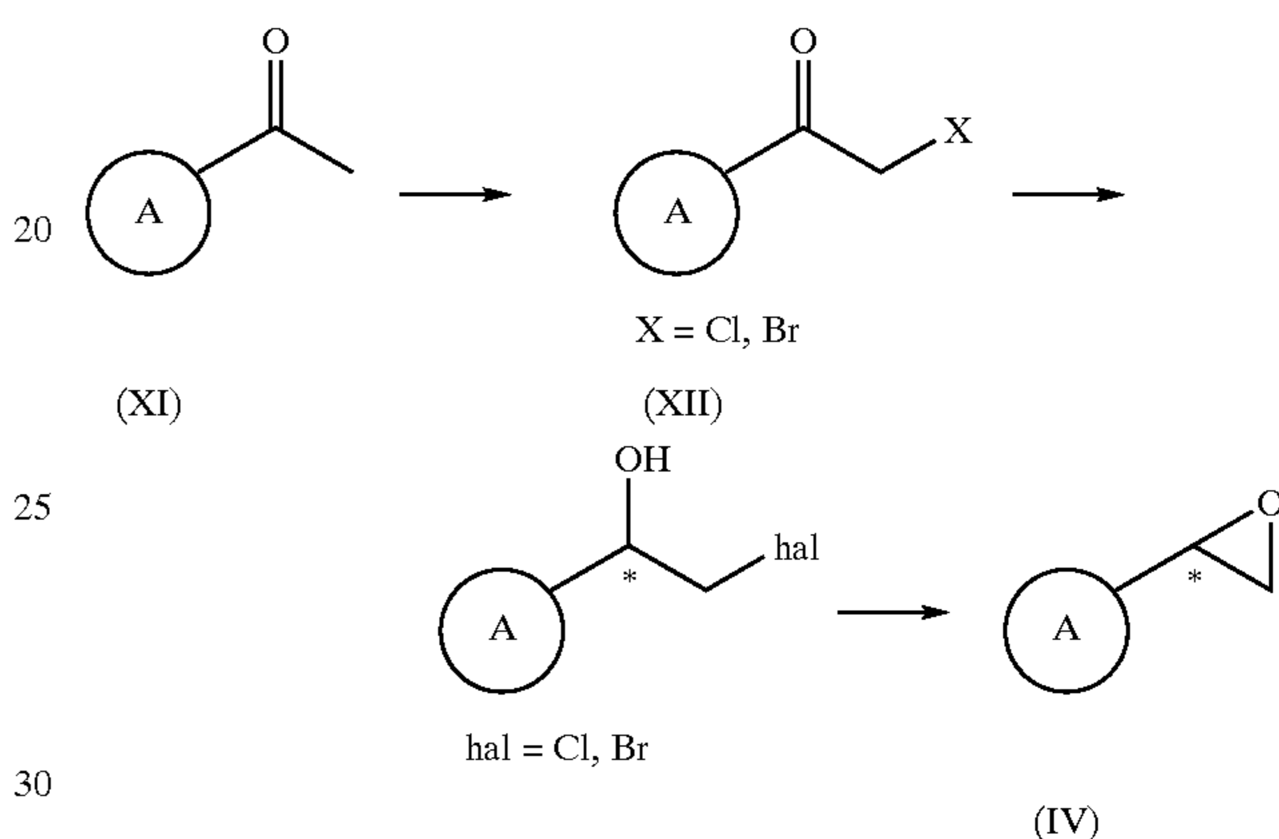
Scheme 4
