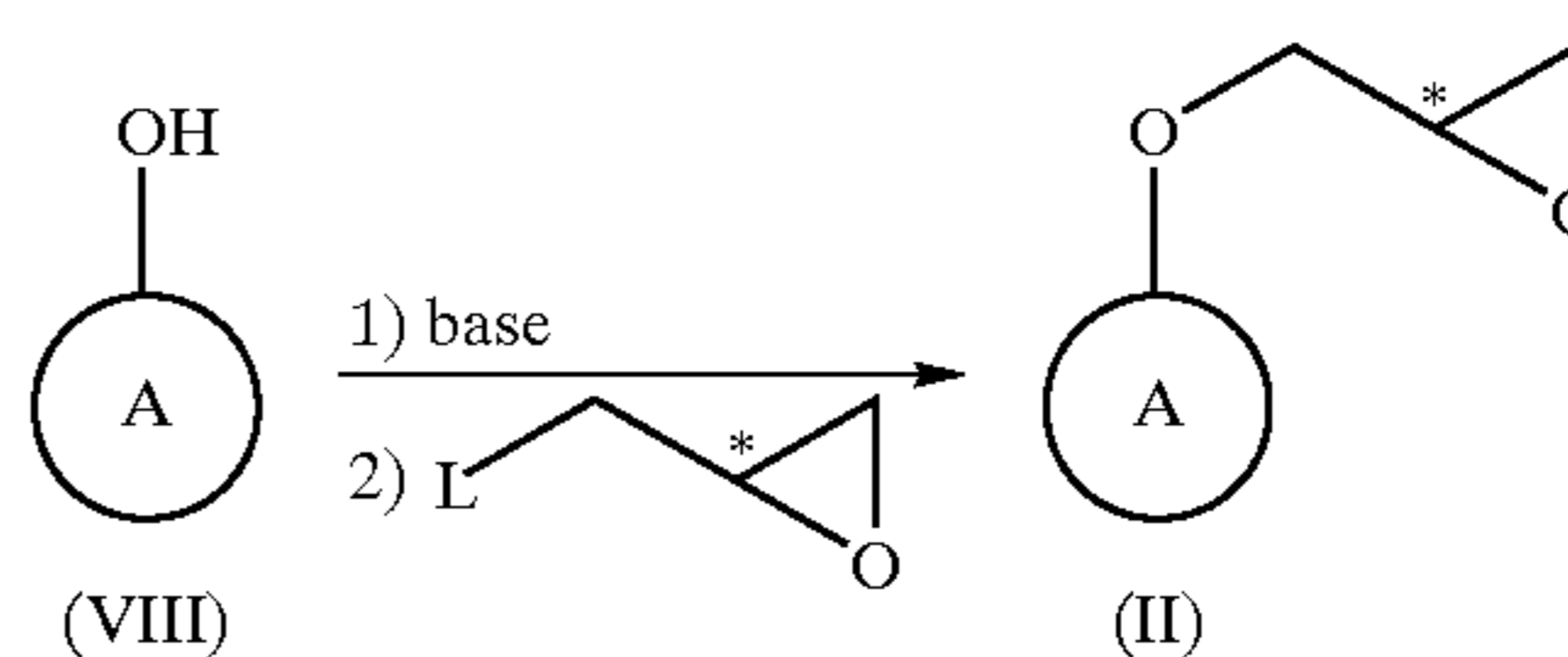
Scheme 1
