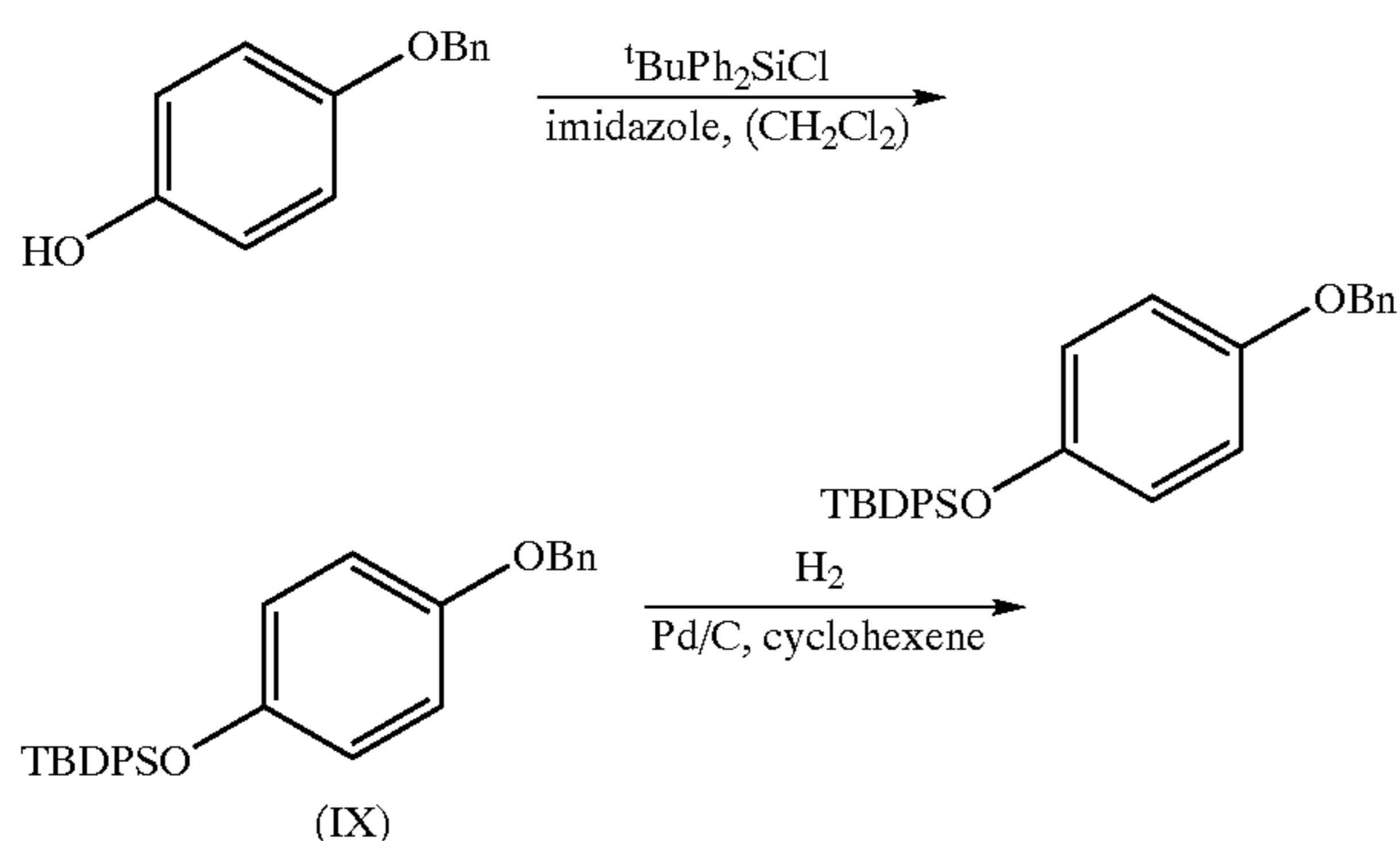
Scheme 3
