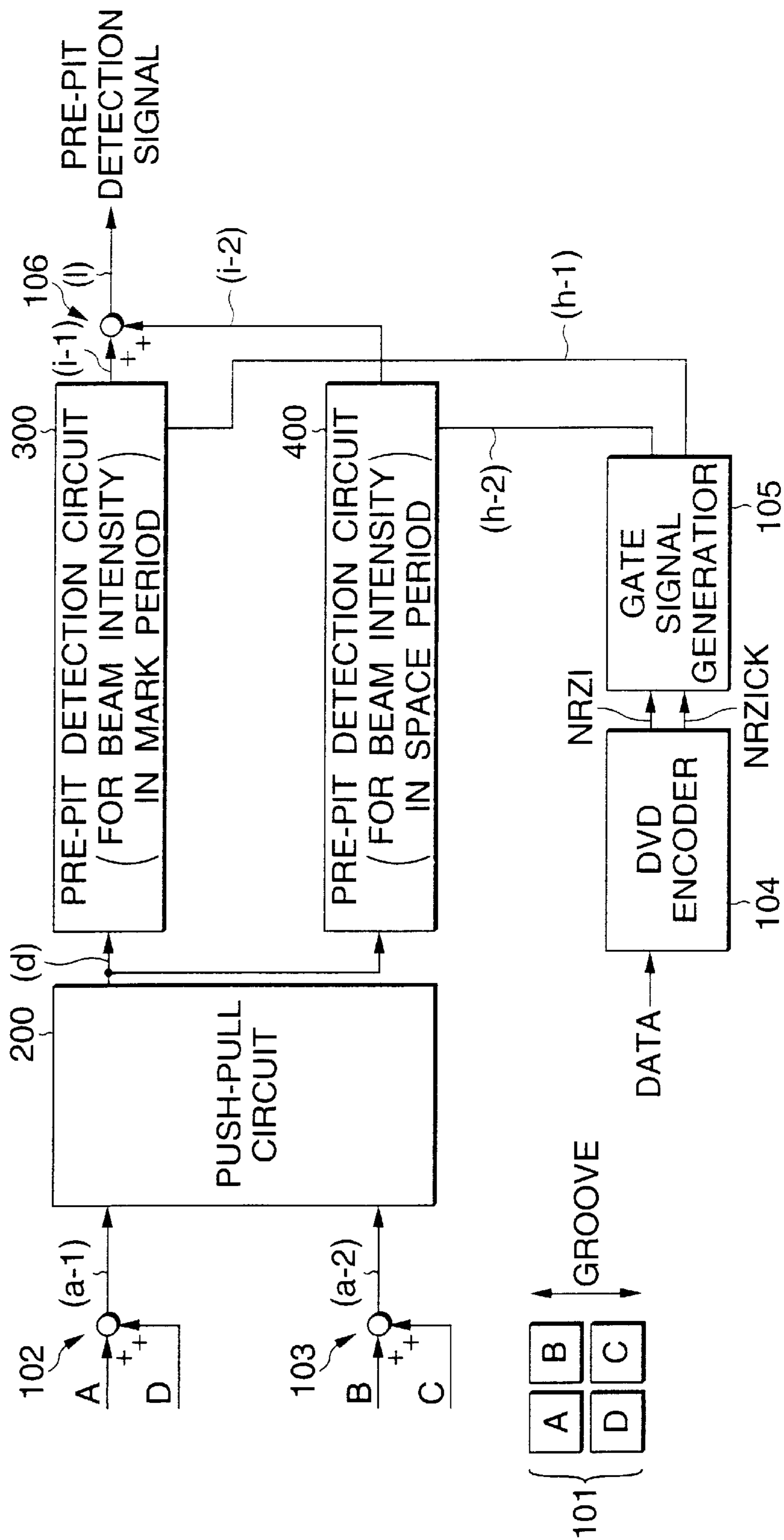
BLOCK DIAGRAM SHOWING OVERALL CONFIGURATION OF CONVENTIONAL PRE-PIT DETECTION UNIT
