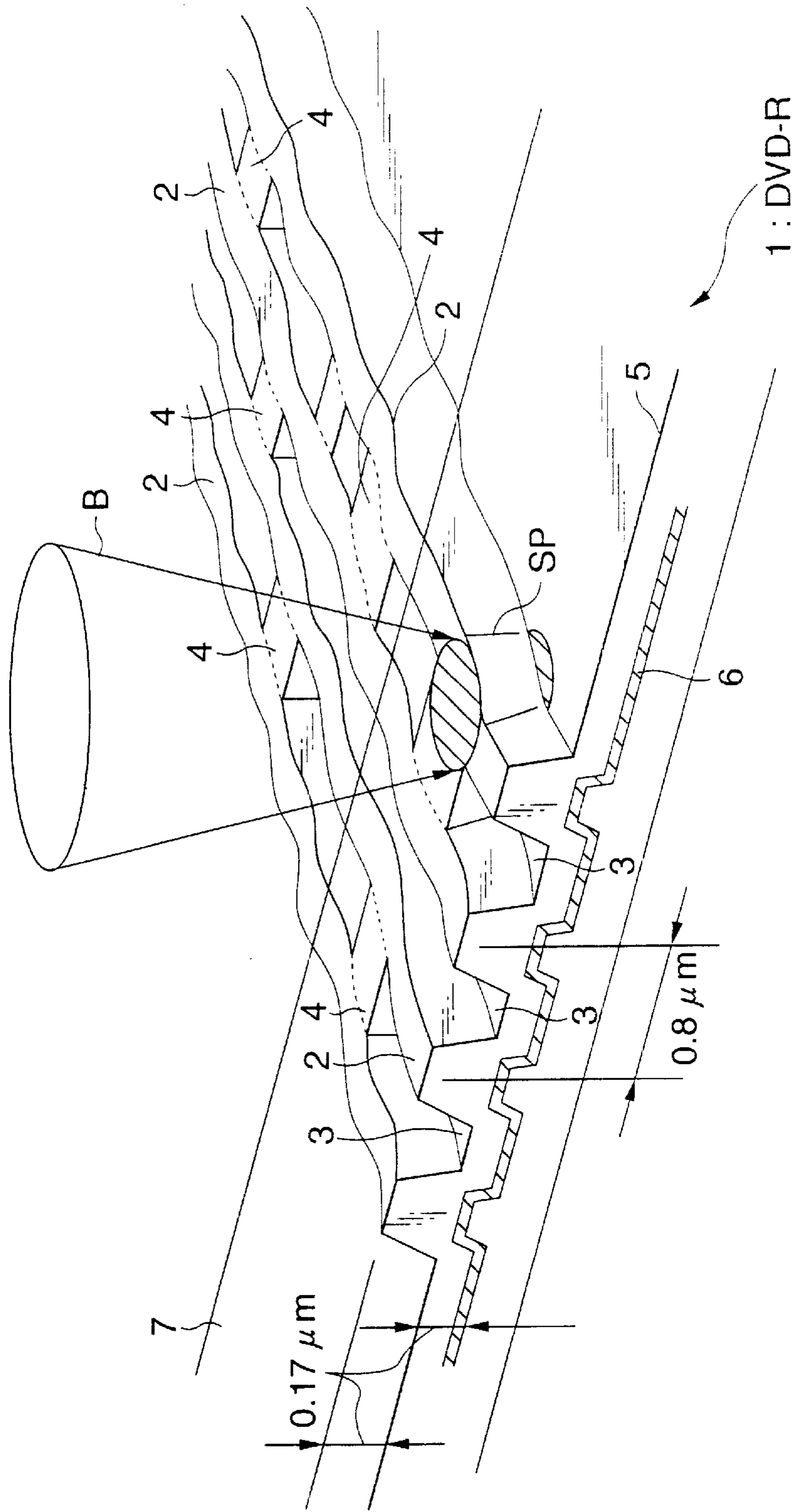
EXAMPLE OF DVD-R WITH PRE-PIT FORMED ON LAND TRACK
