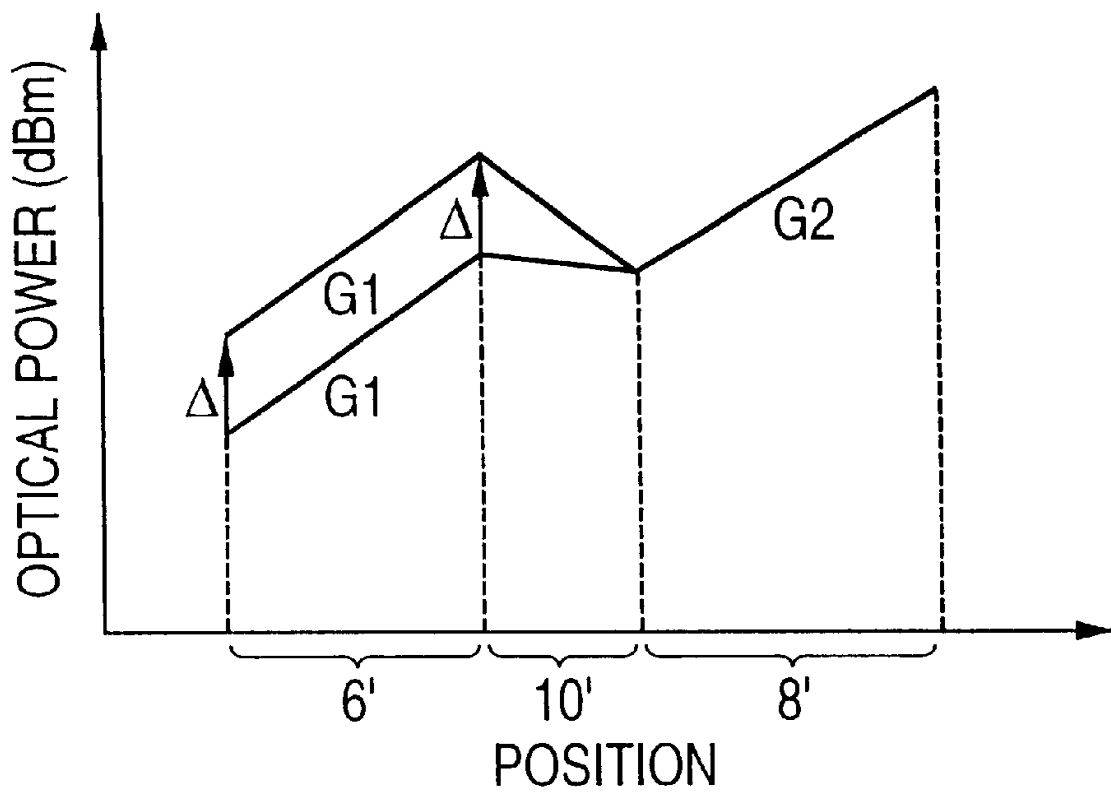
FIG. 4 (PRIOR ART)
