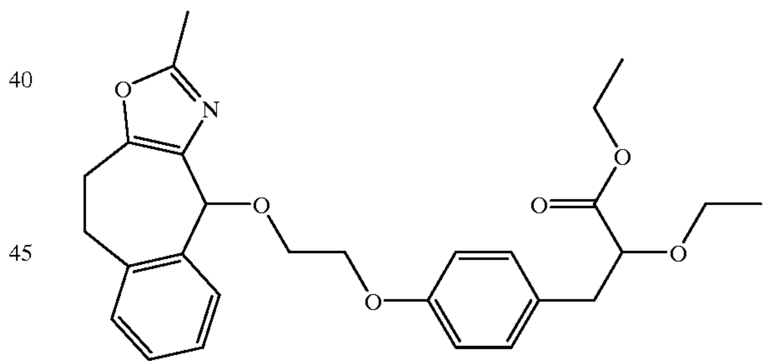
2-Ethoxy-3-(4-[2-(2-methyl-9,10-dihydro-4H-1-oxa-3-aza-benzo[f]azulen-4-yloxy)-ethoxy]-phenyl)-propionic acid ethyl ester
