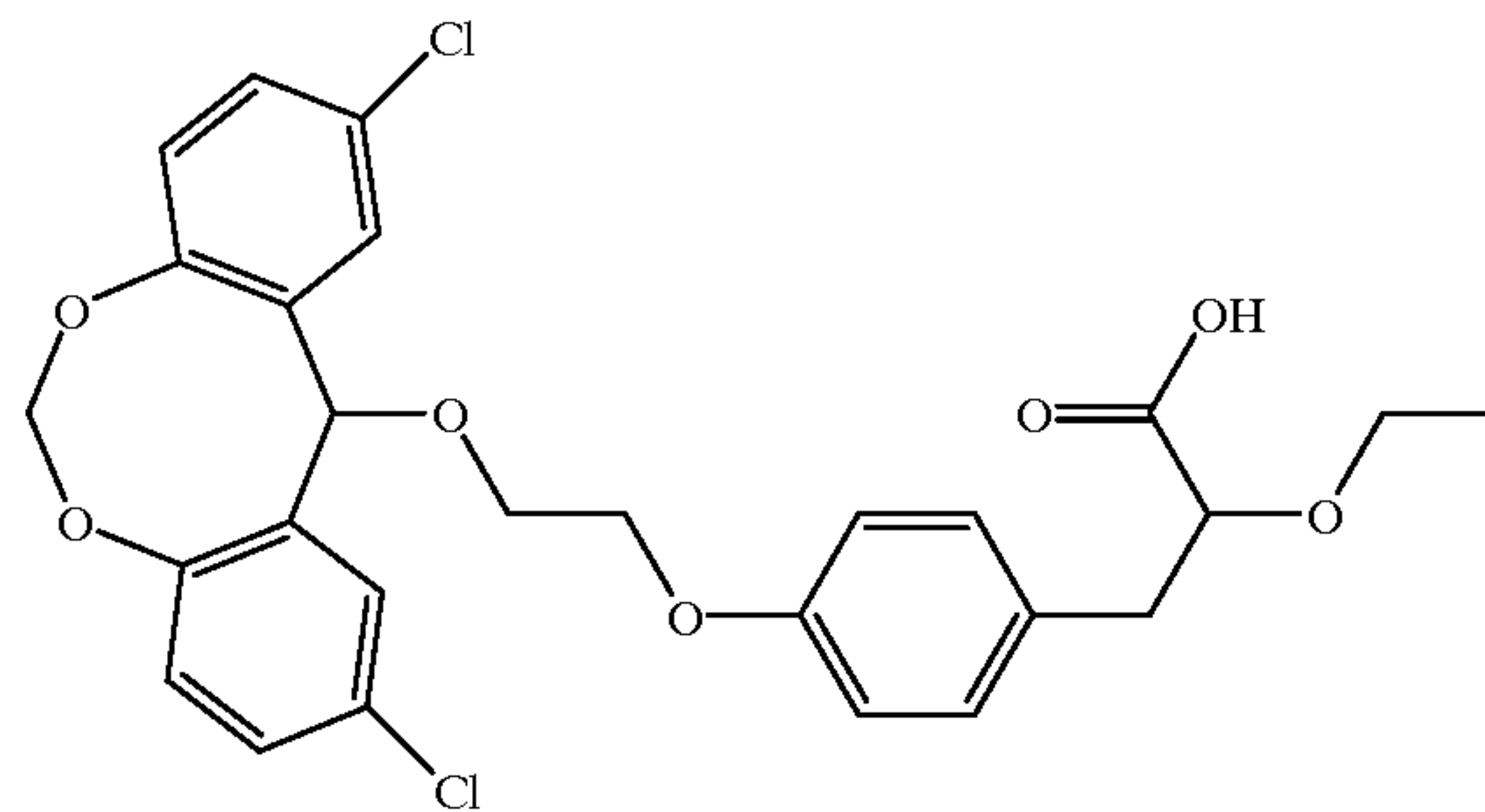
3-(4-[2-(2,10-Dichloro-12H-5,7-dioxo-dibenzo[a,d]cycloocten-12-yloxy)-ethoxy]-phenyl)-2-ethoxy-propionic acid
