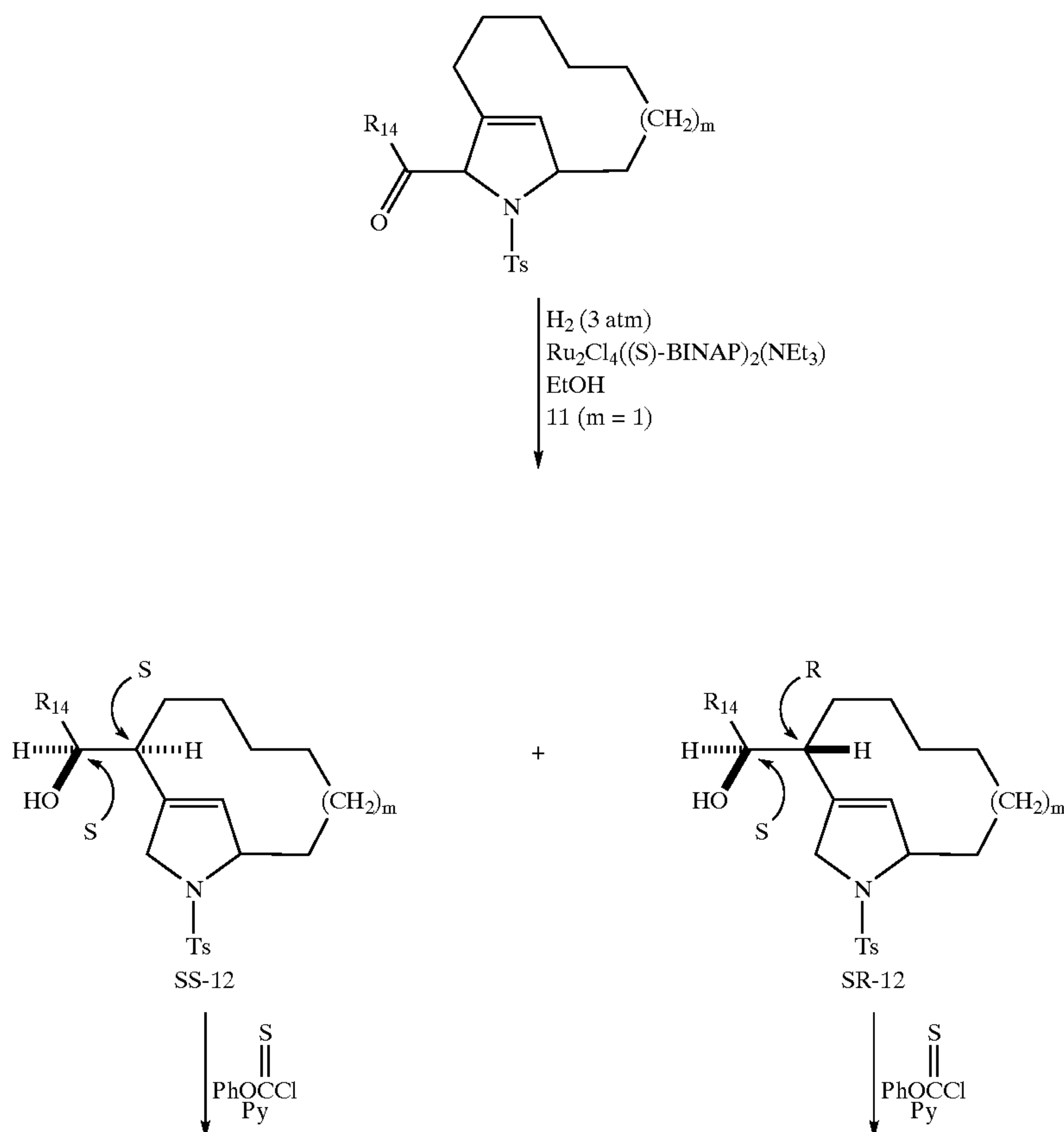
Scheme J
