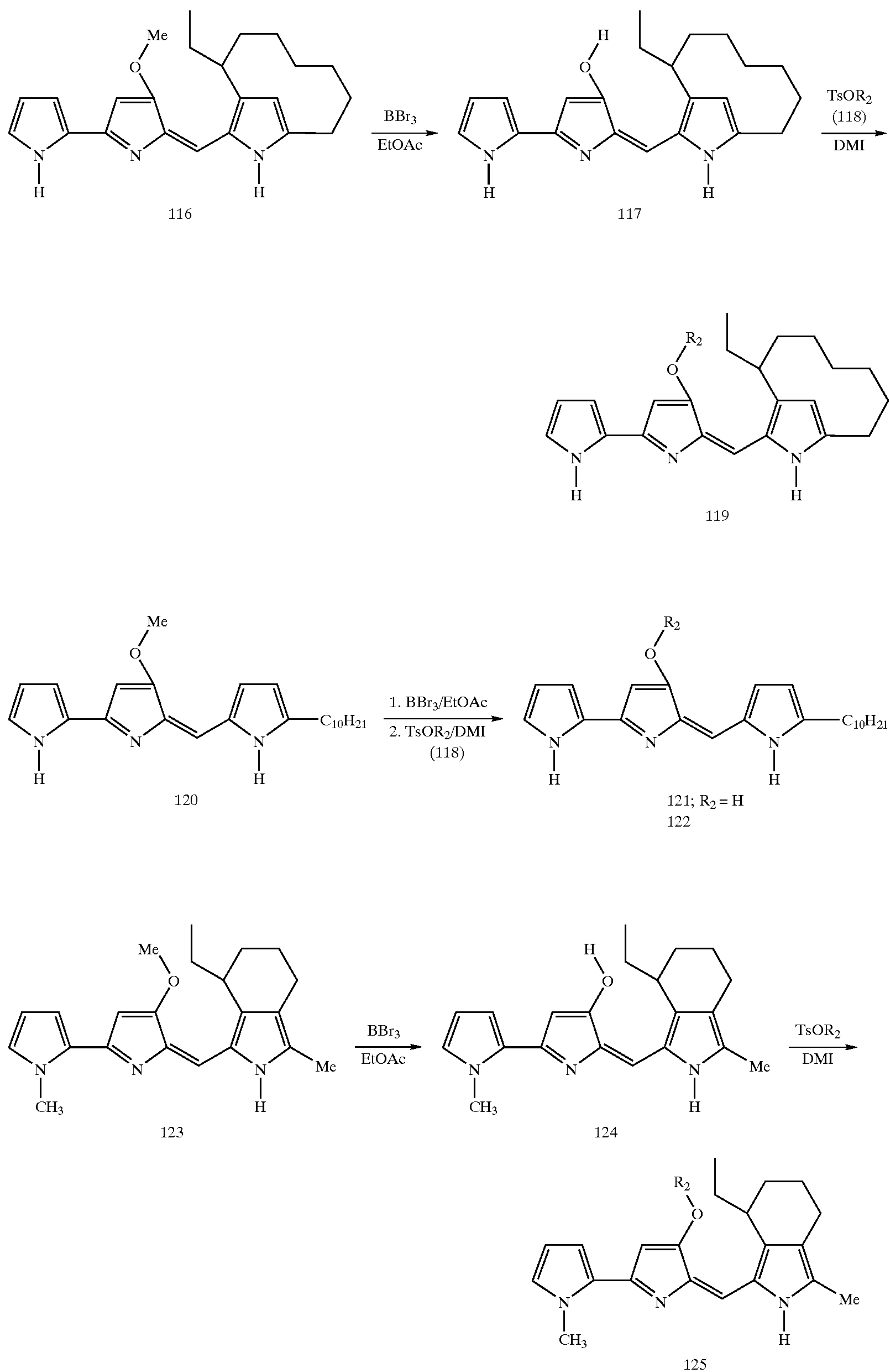
Scheme I
