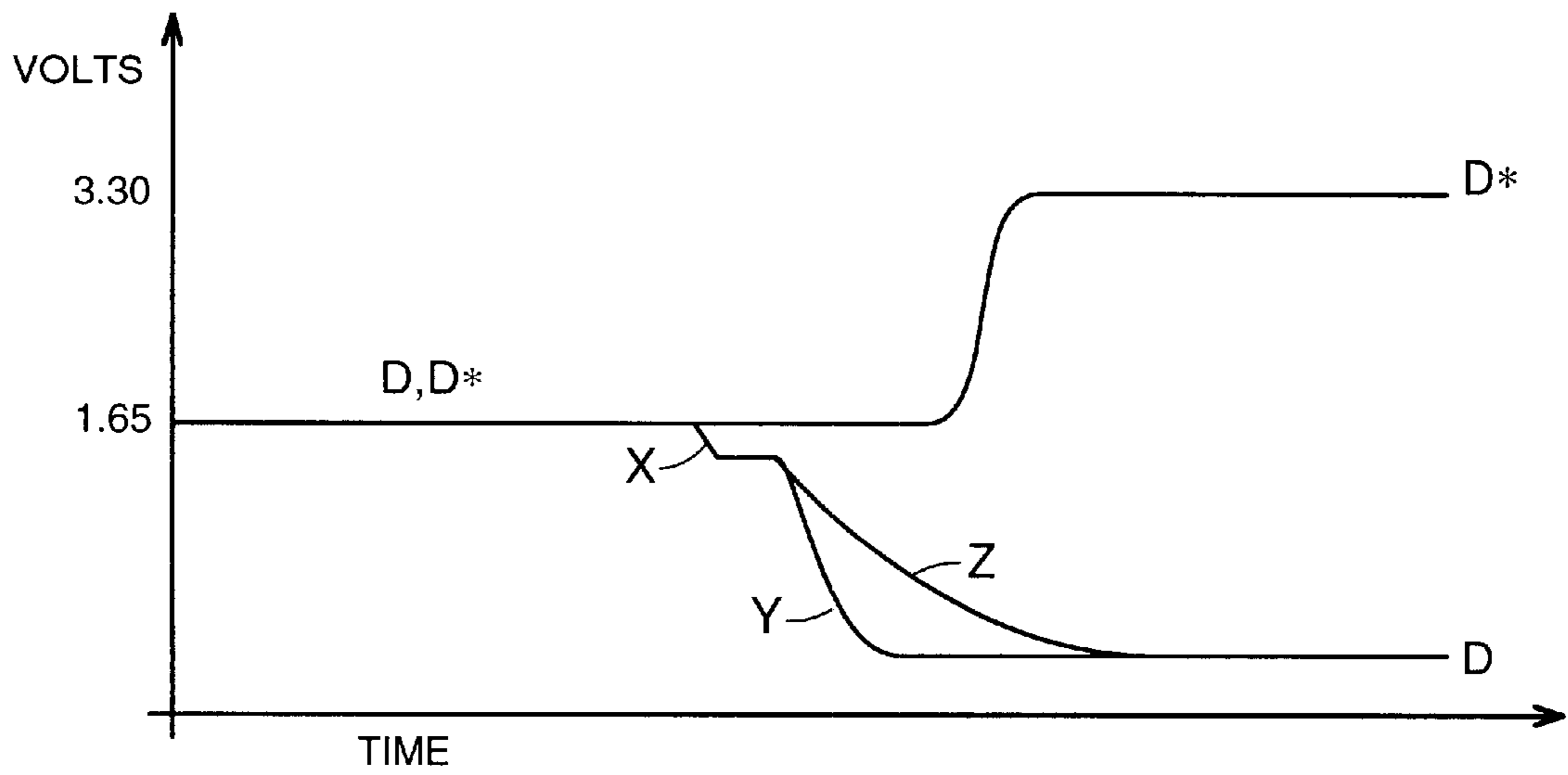
FIG. 2 (PRIOR ART)
