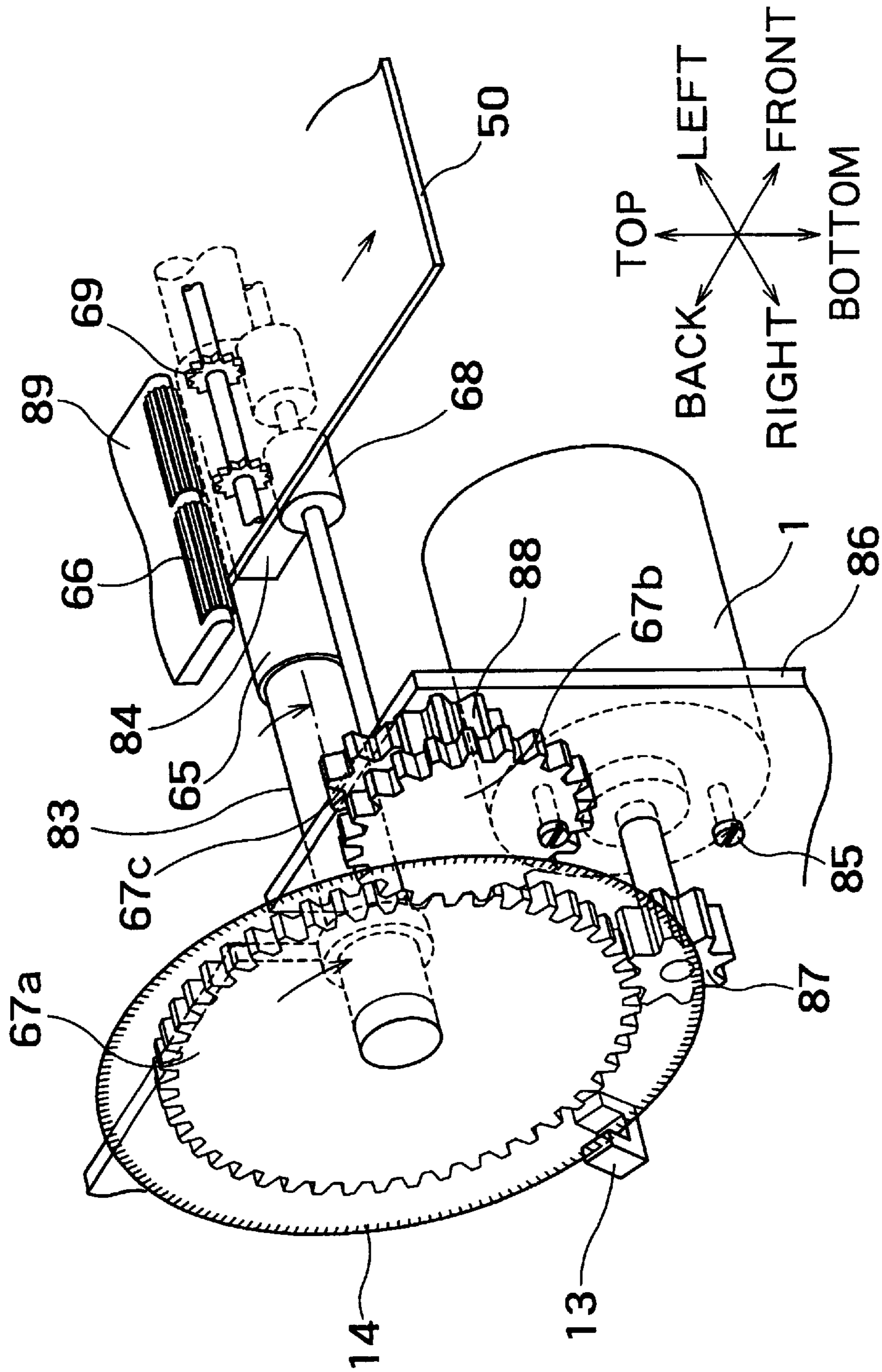
FIG. 6 PRIOR ART
