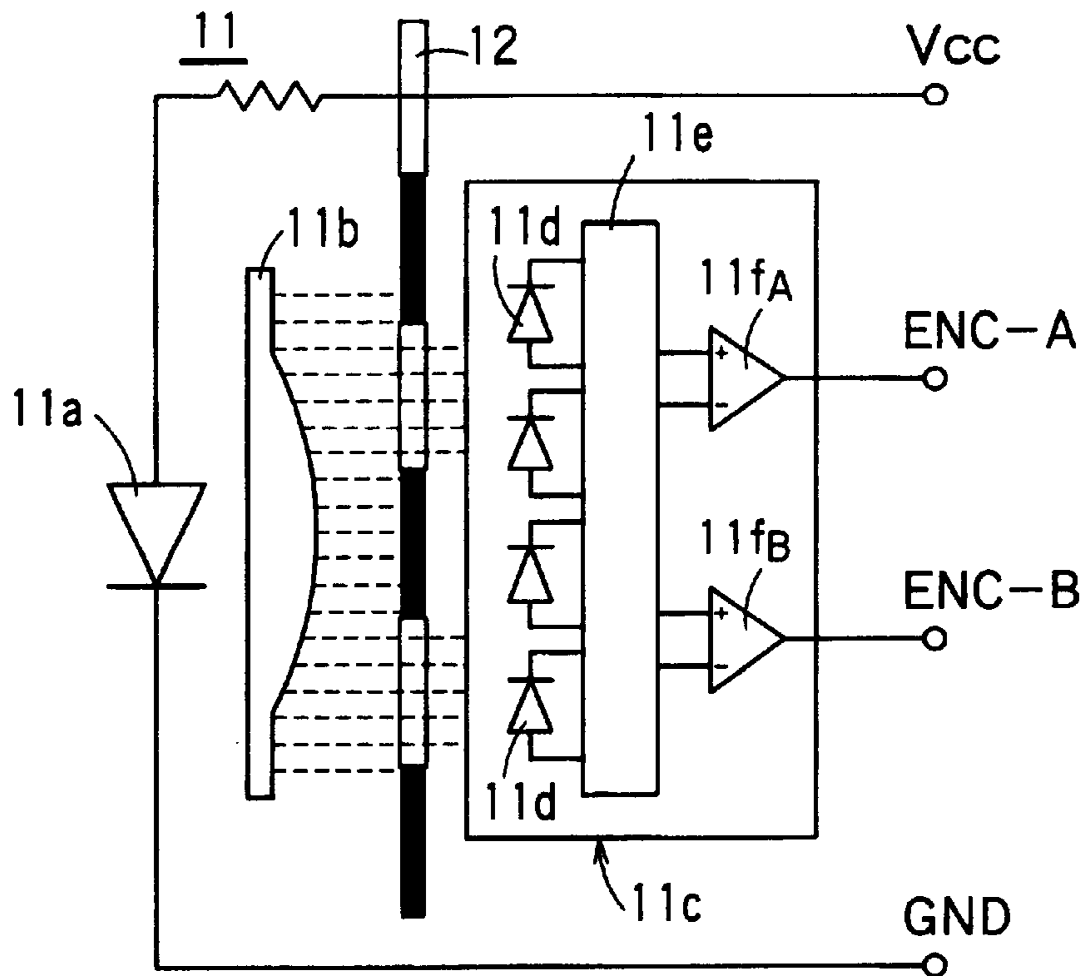
FIG. 3 PRIOR ART
