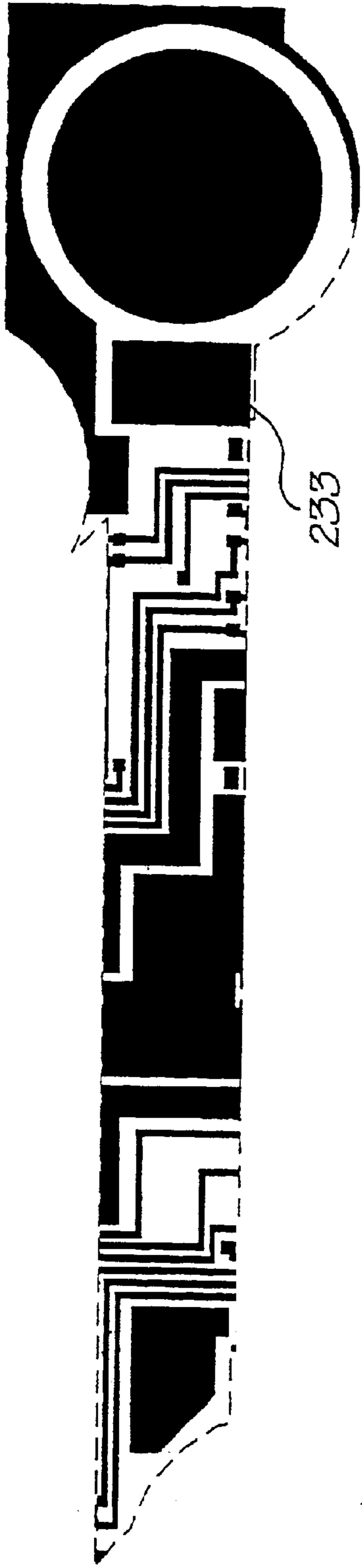
Metal 2 mask
