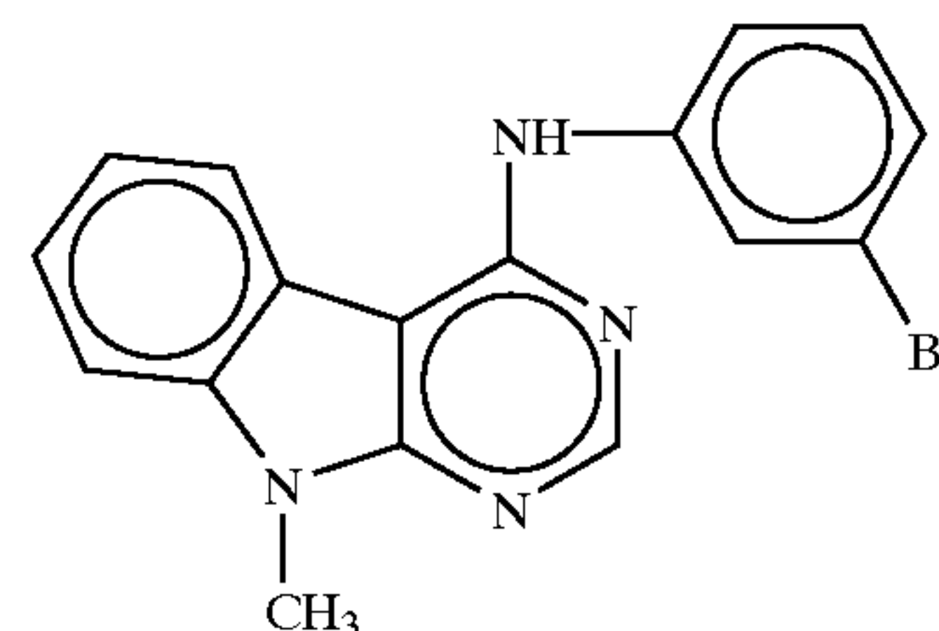
EXAMPLE 30
