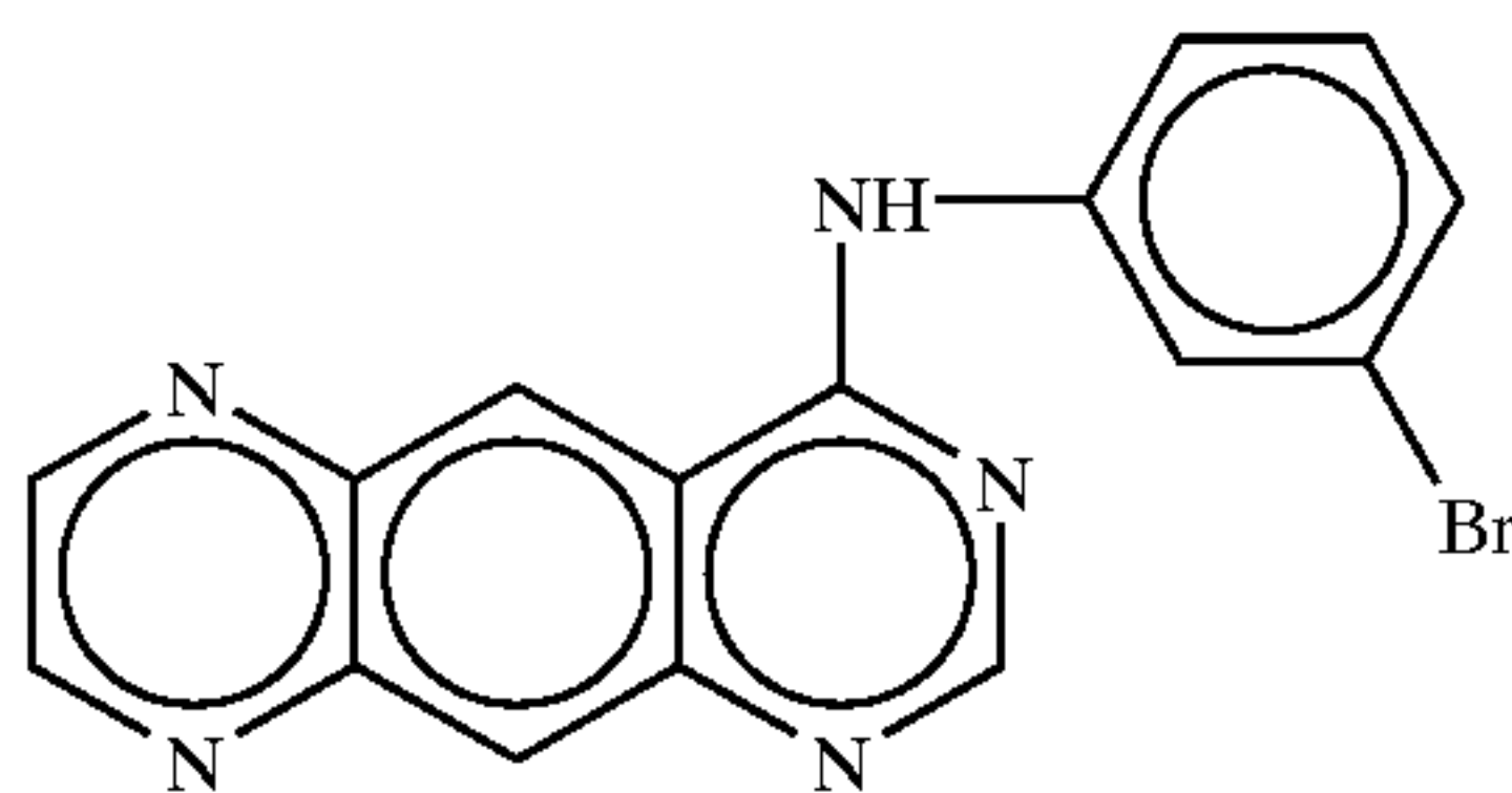
EXAMPLE 11
