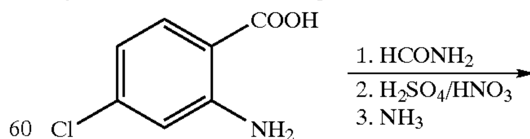
Scheme 10
