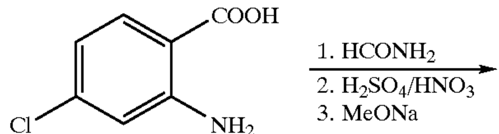
Scheme 3
