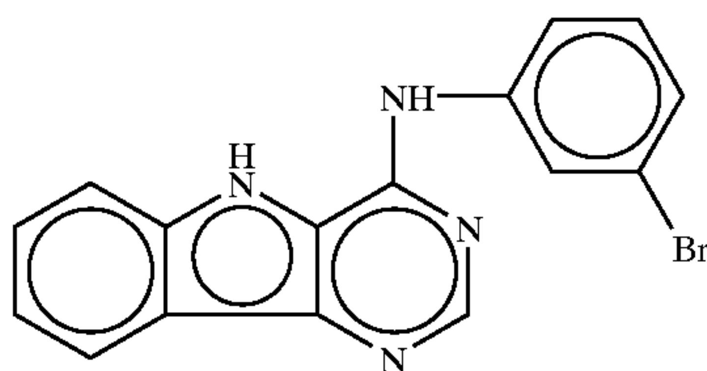
EXAMPLE 26
