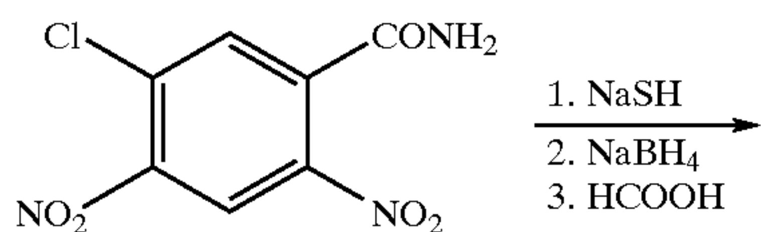
Scheme 6
