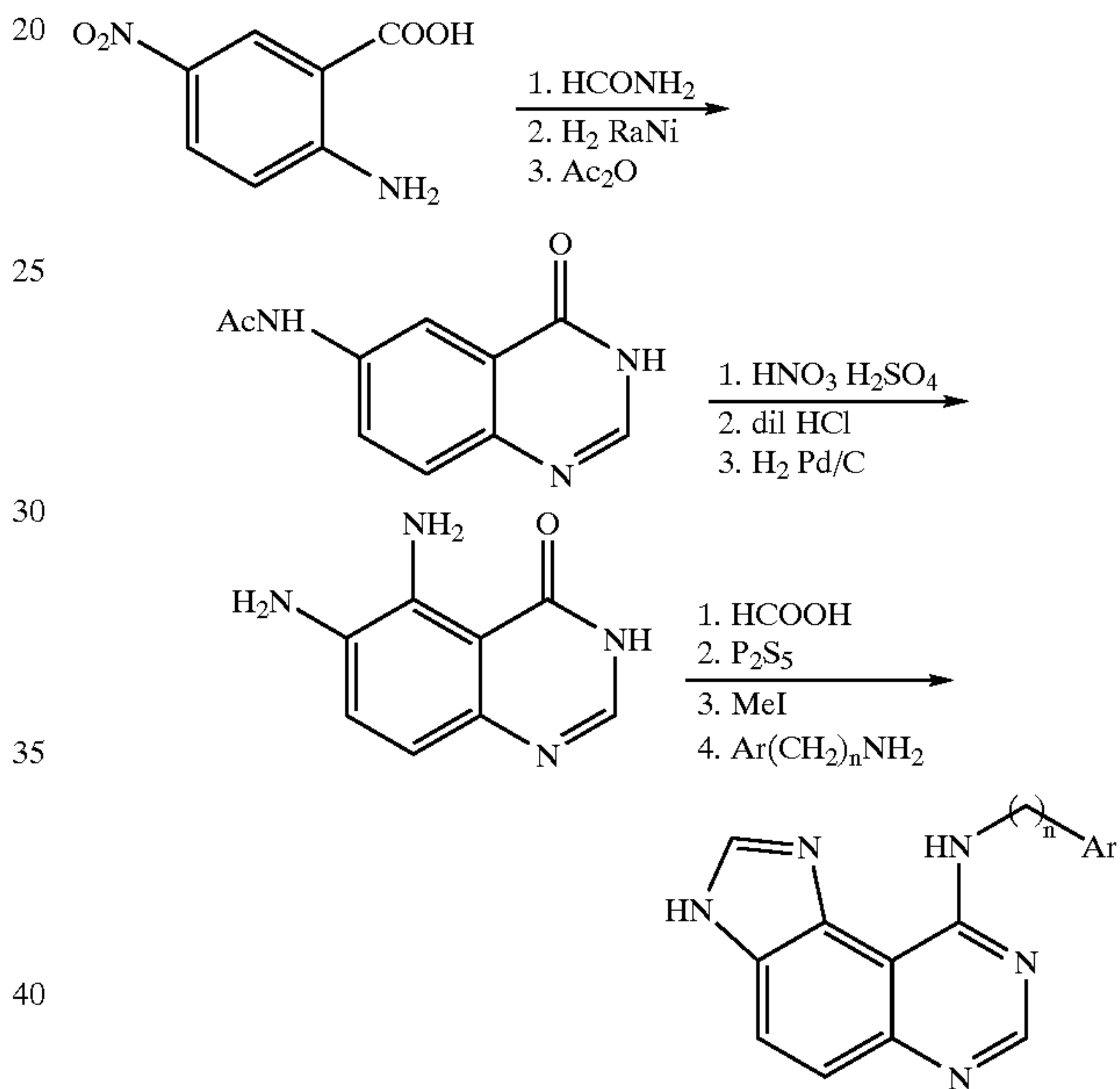
Scheme 13
