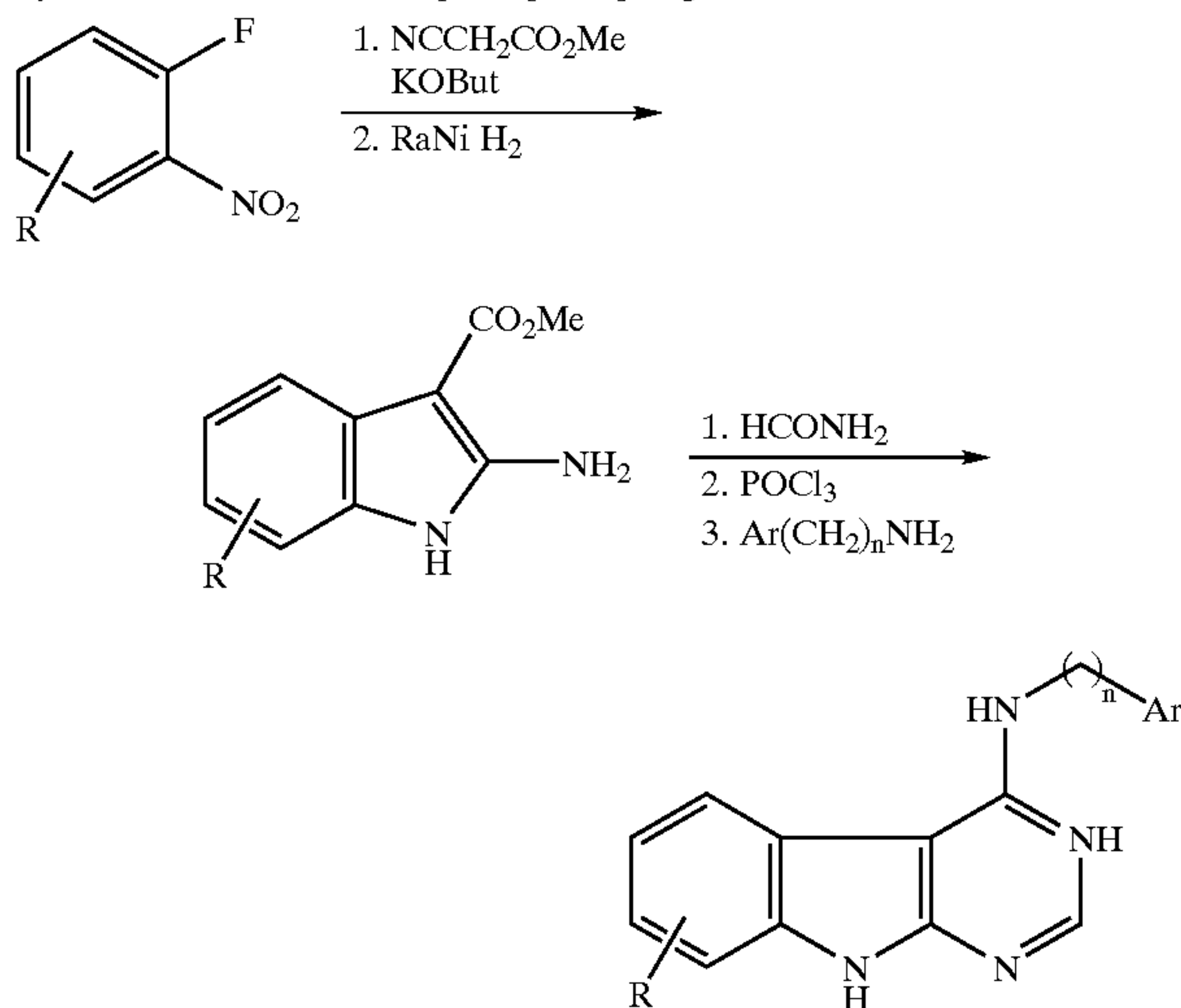
Scheme 24
