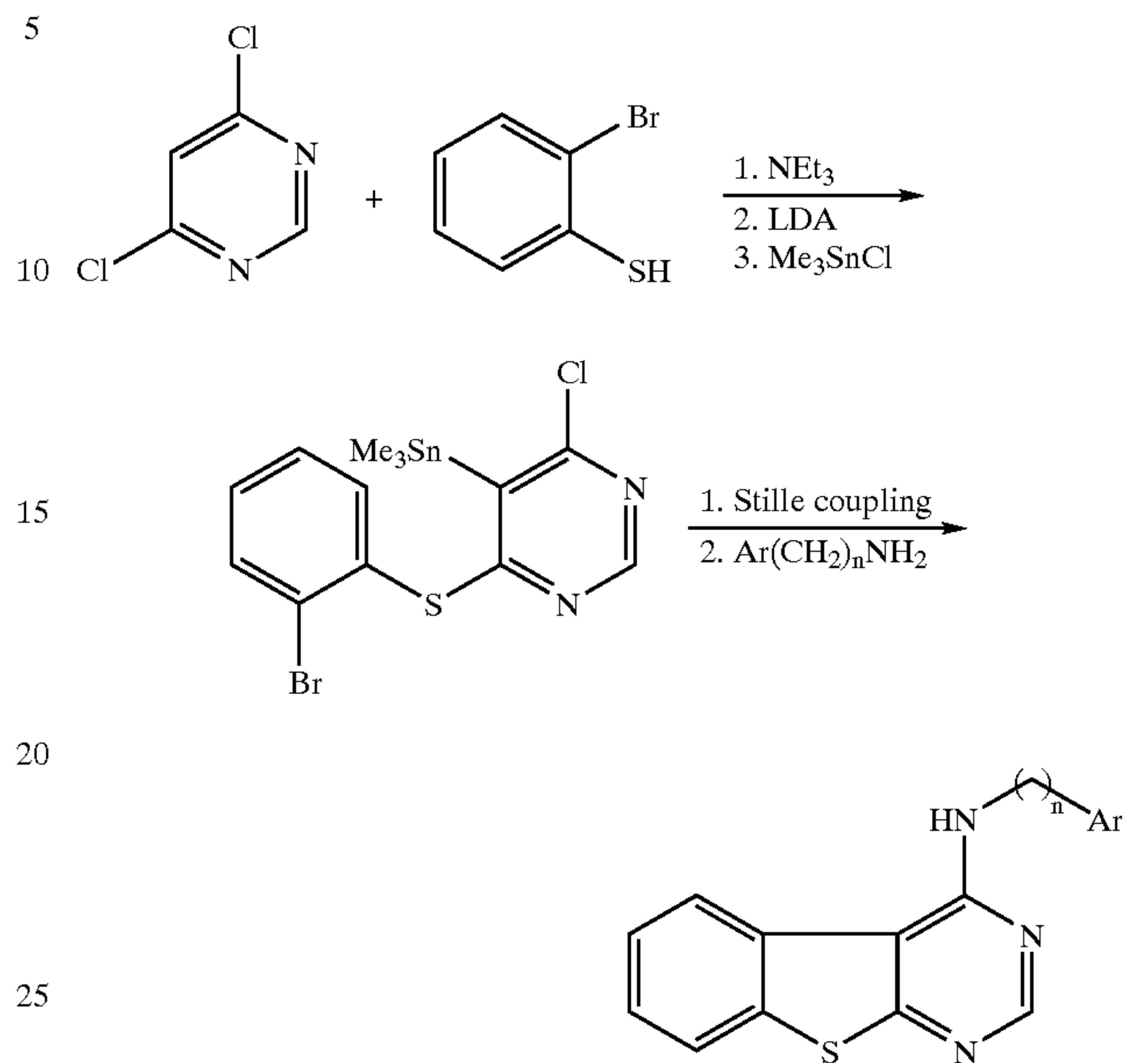
Scheme 17
