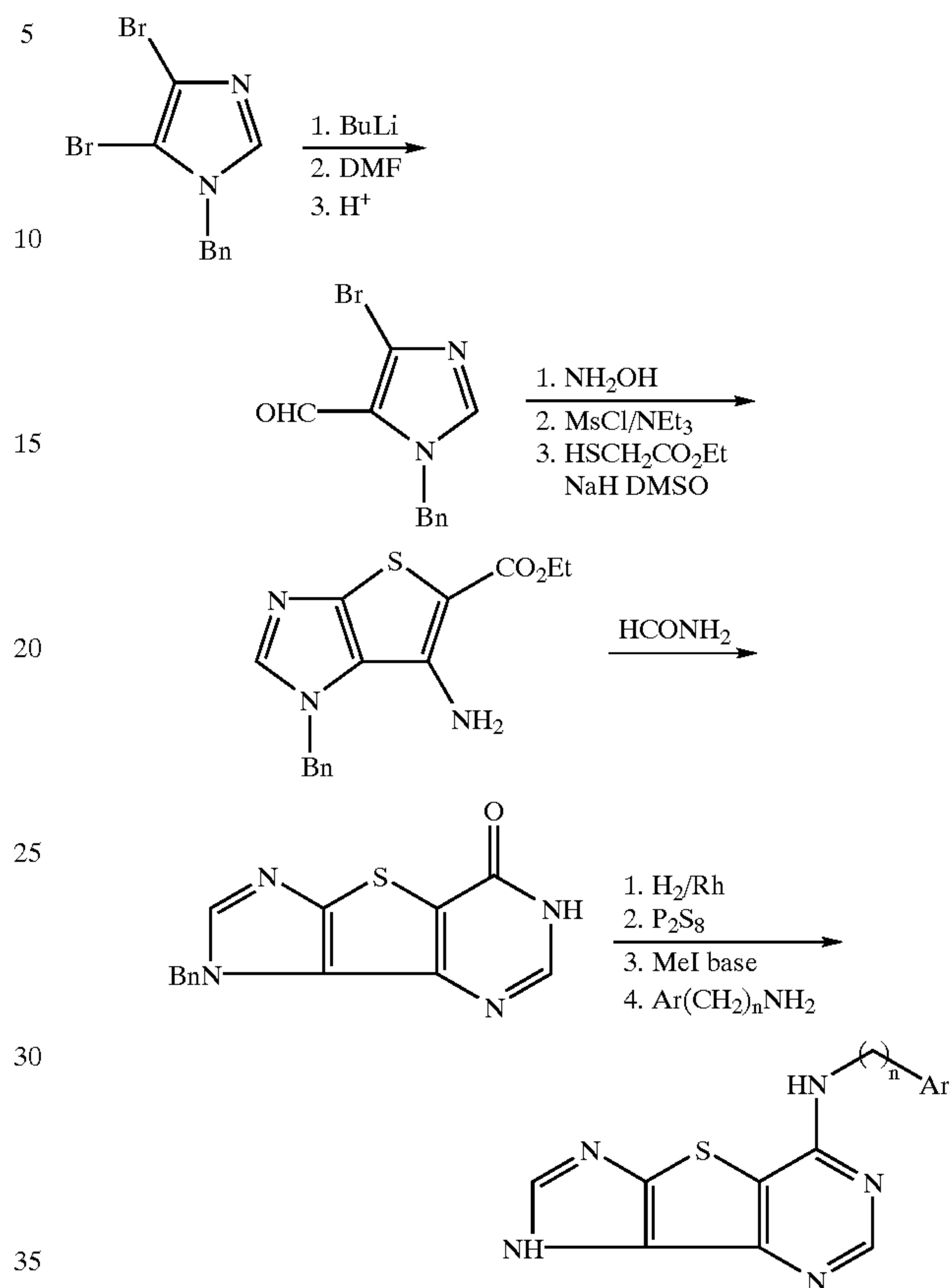
Scheme 21
