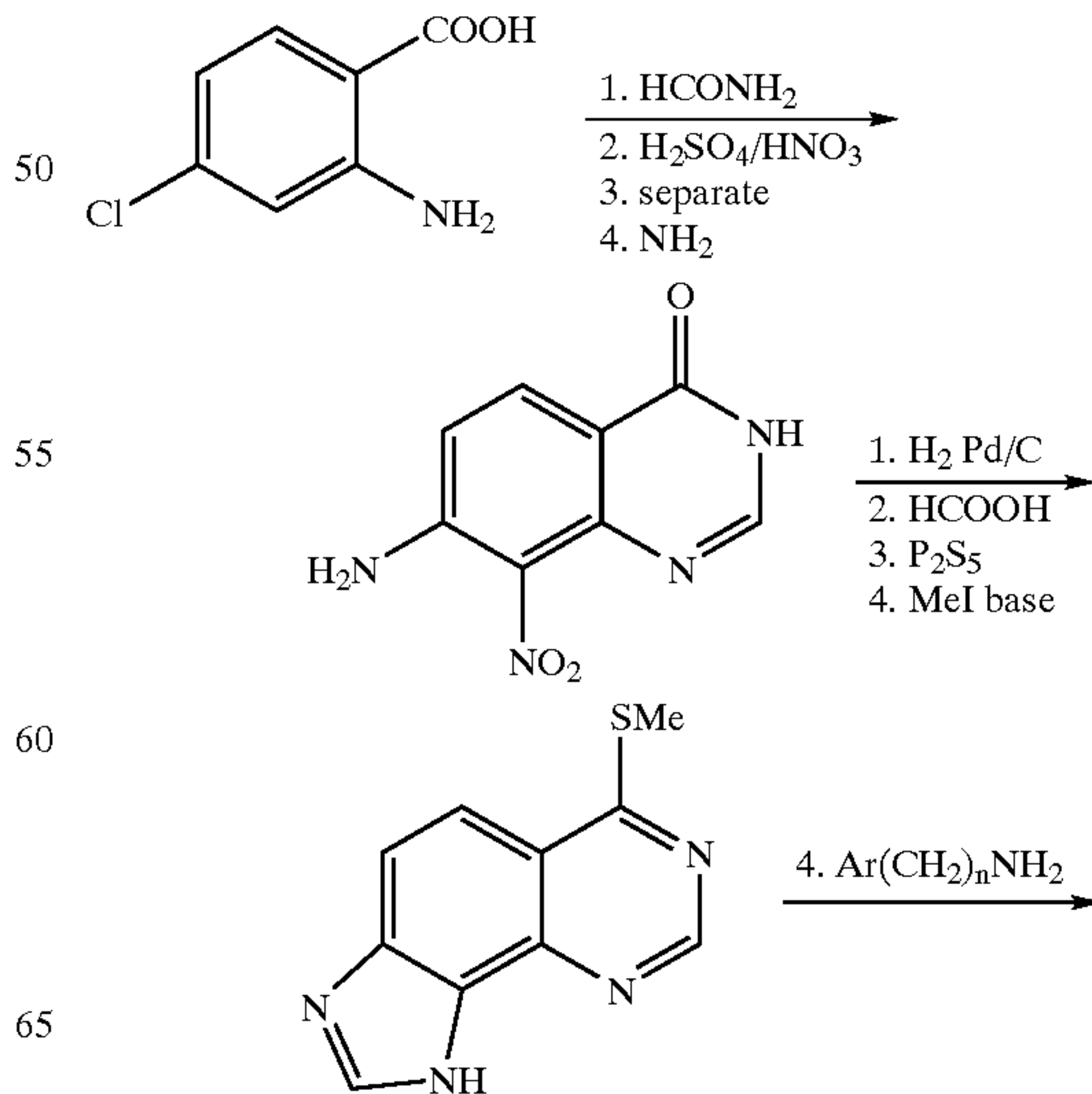
Scheme 14
