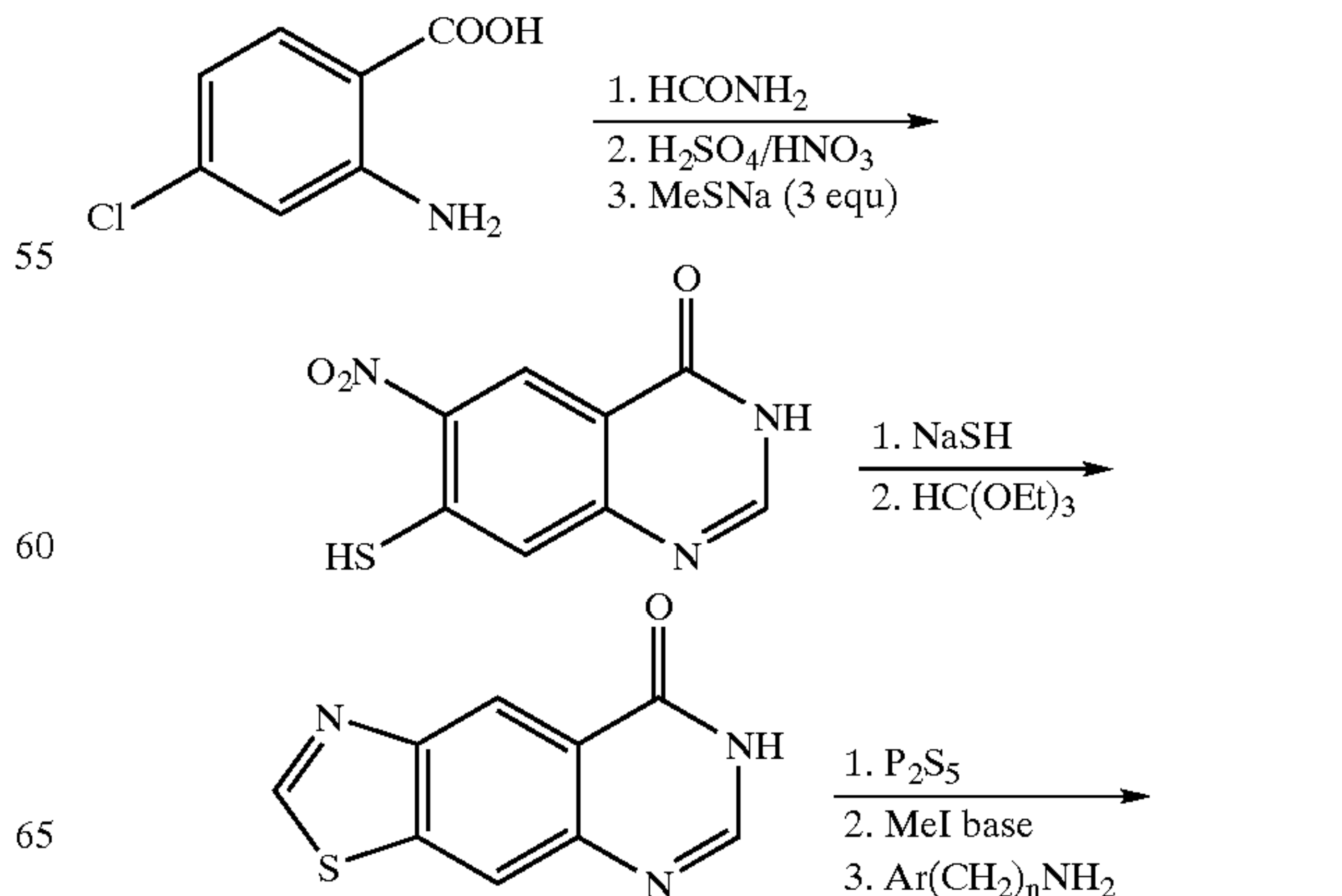
Scheme 5
