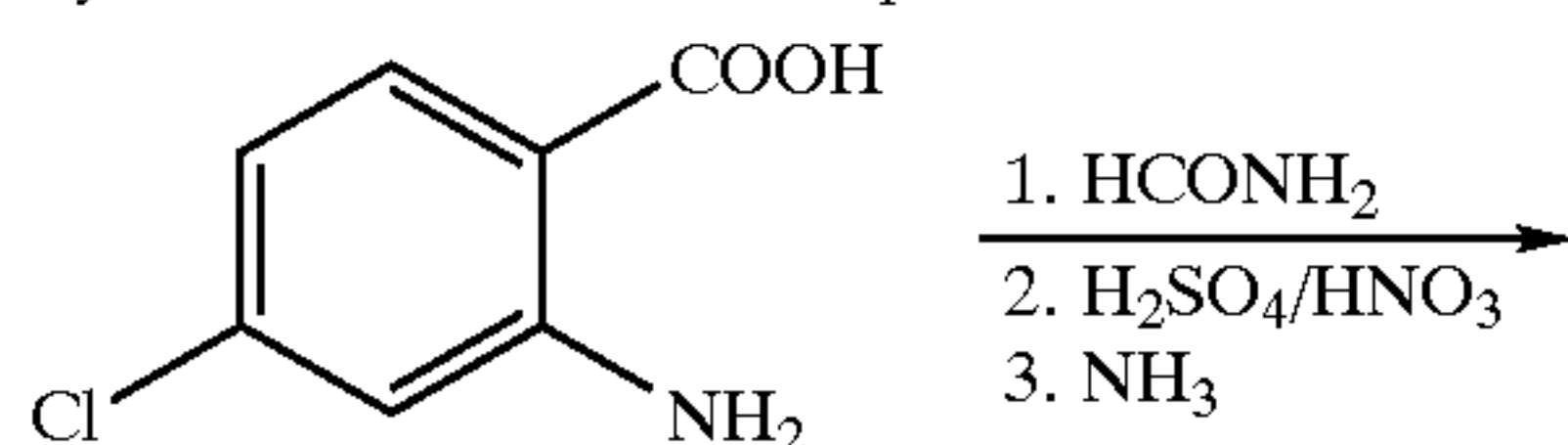
Scheme 7
