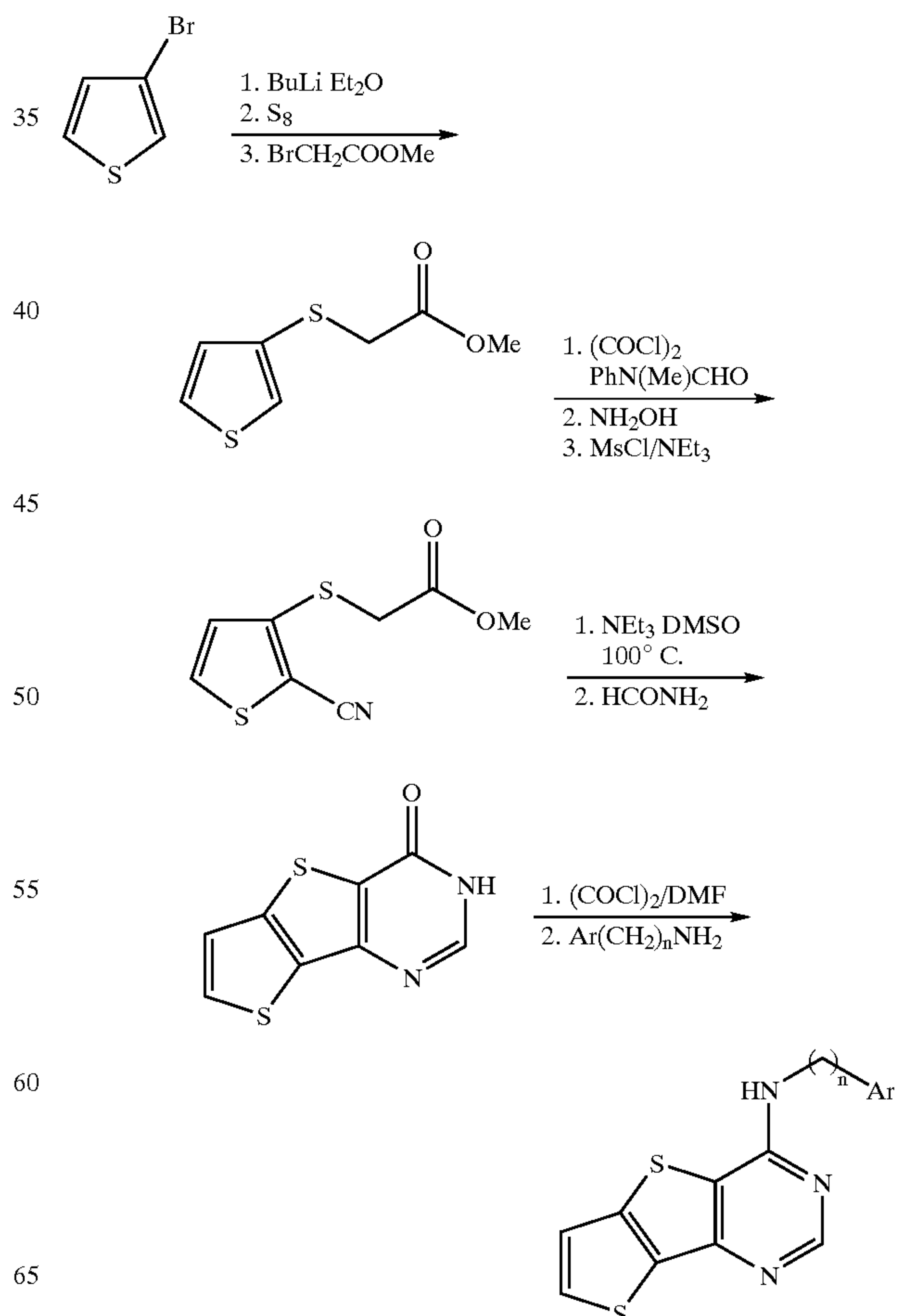
Scheme 18
