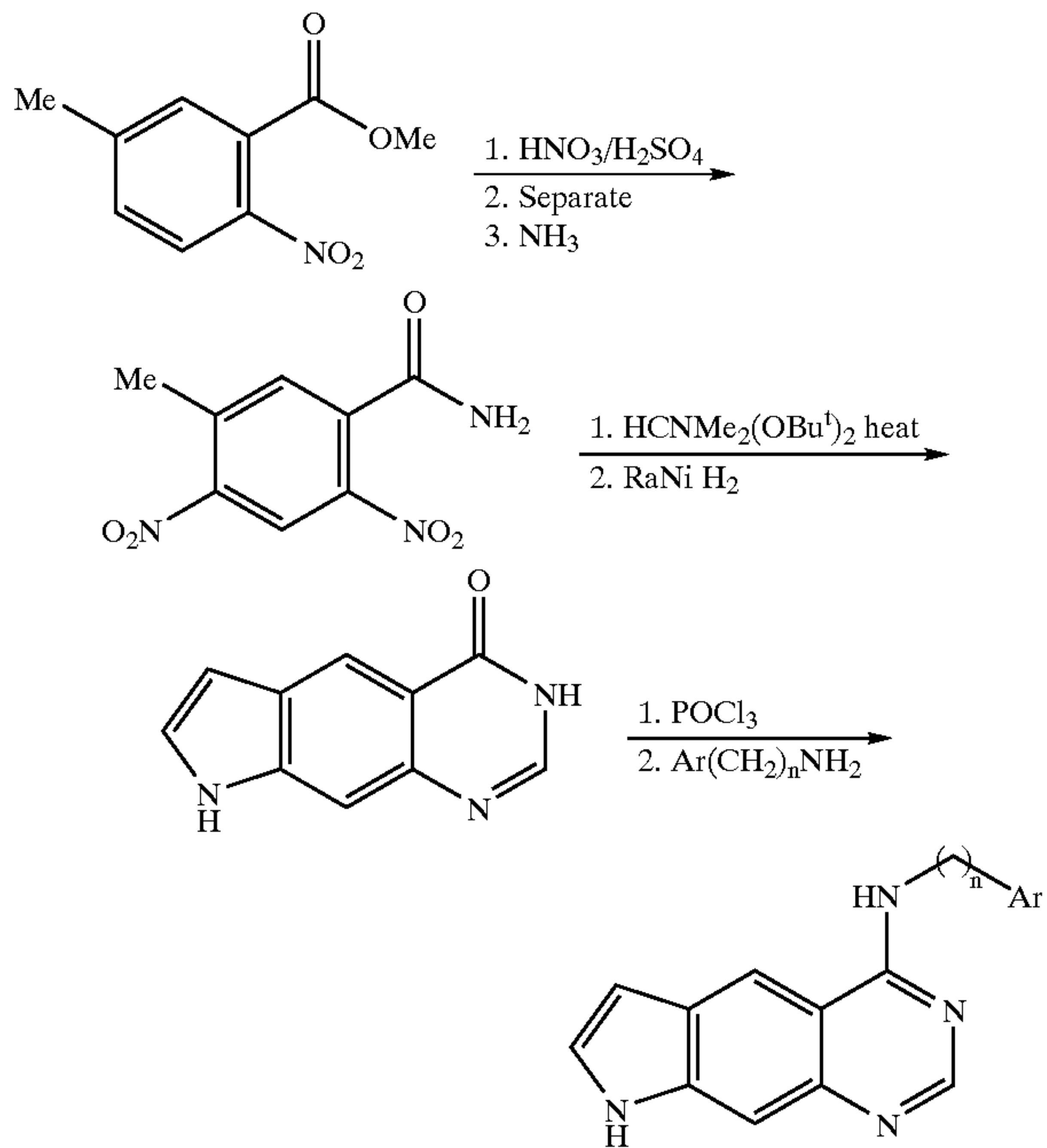
Scheme 3
