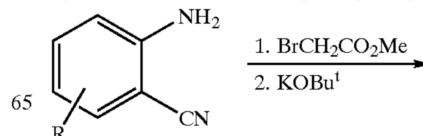
Scheme 23
