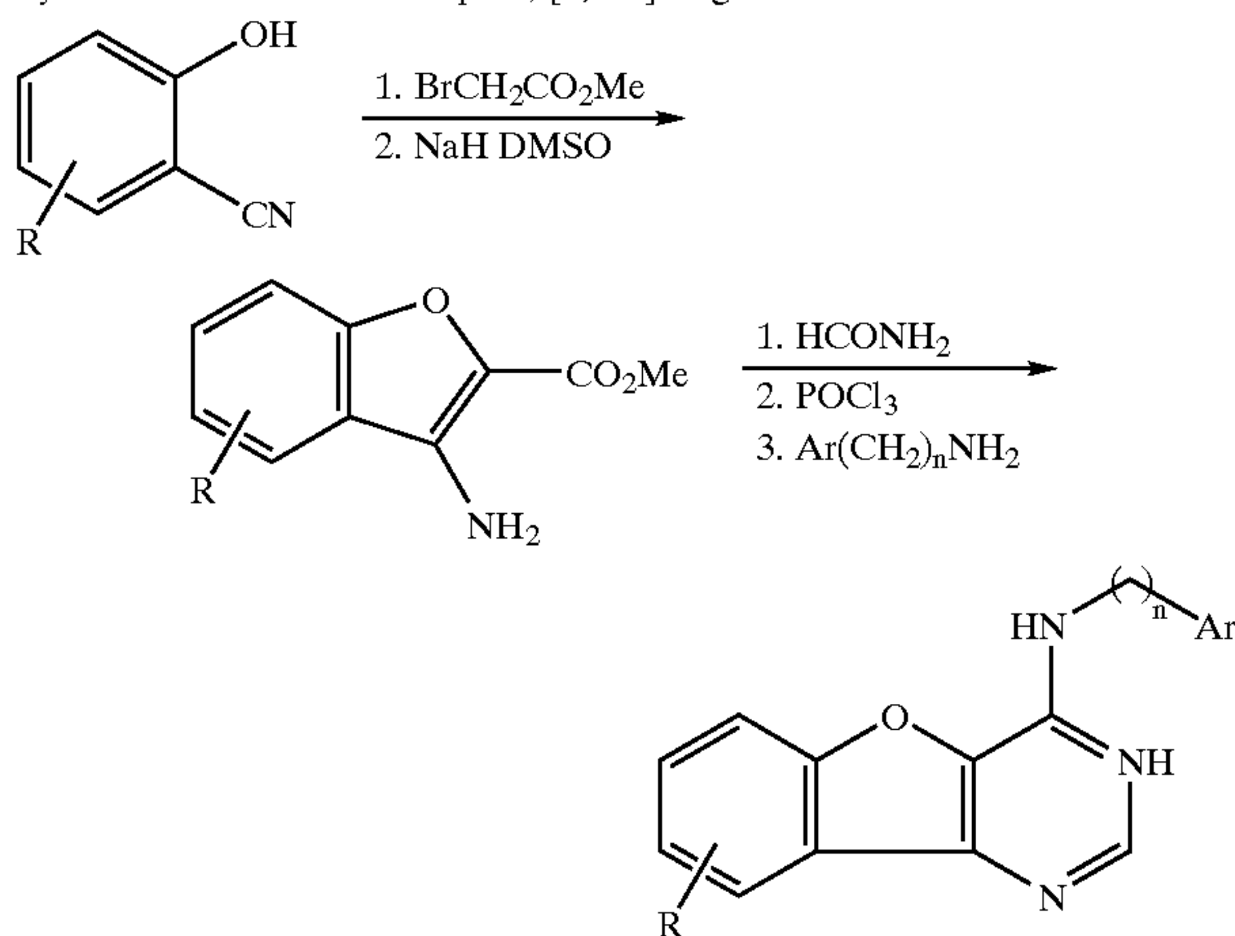
Scheme 25
