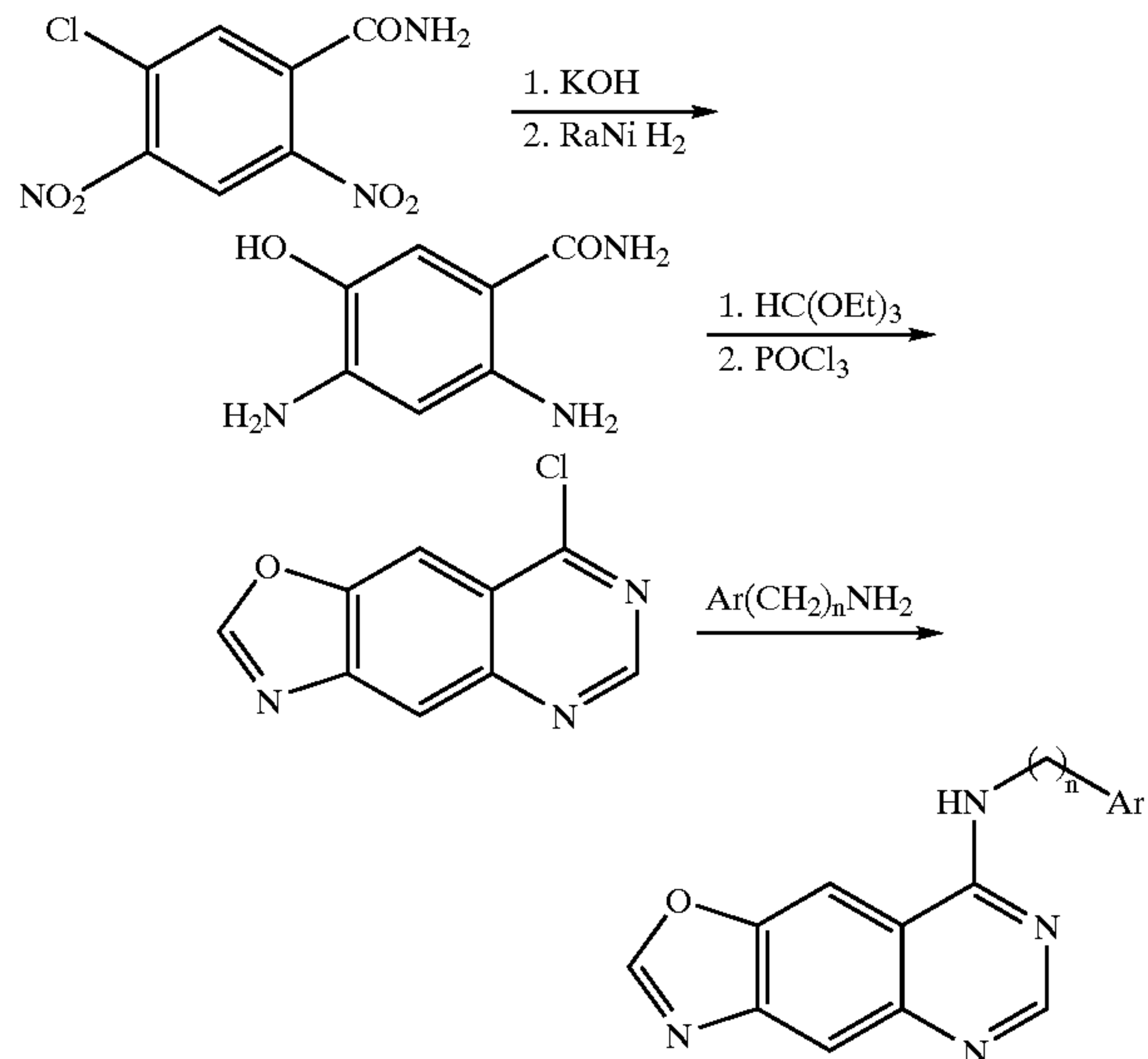
Scheme 4
