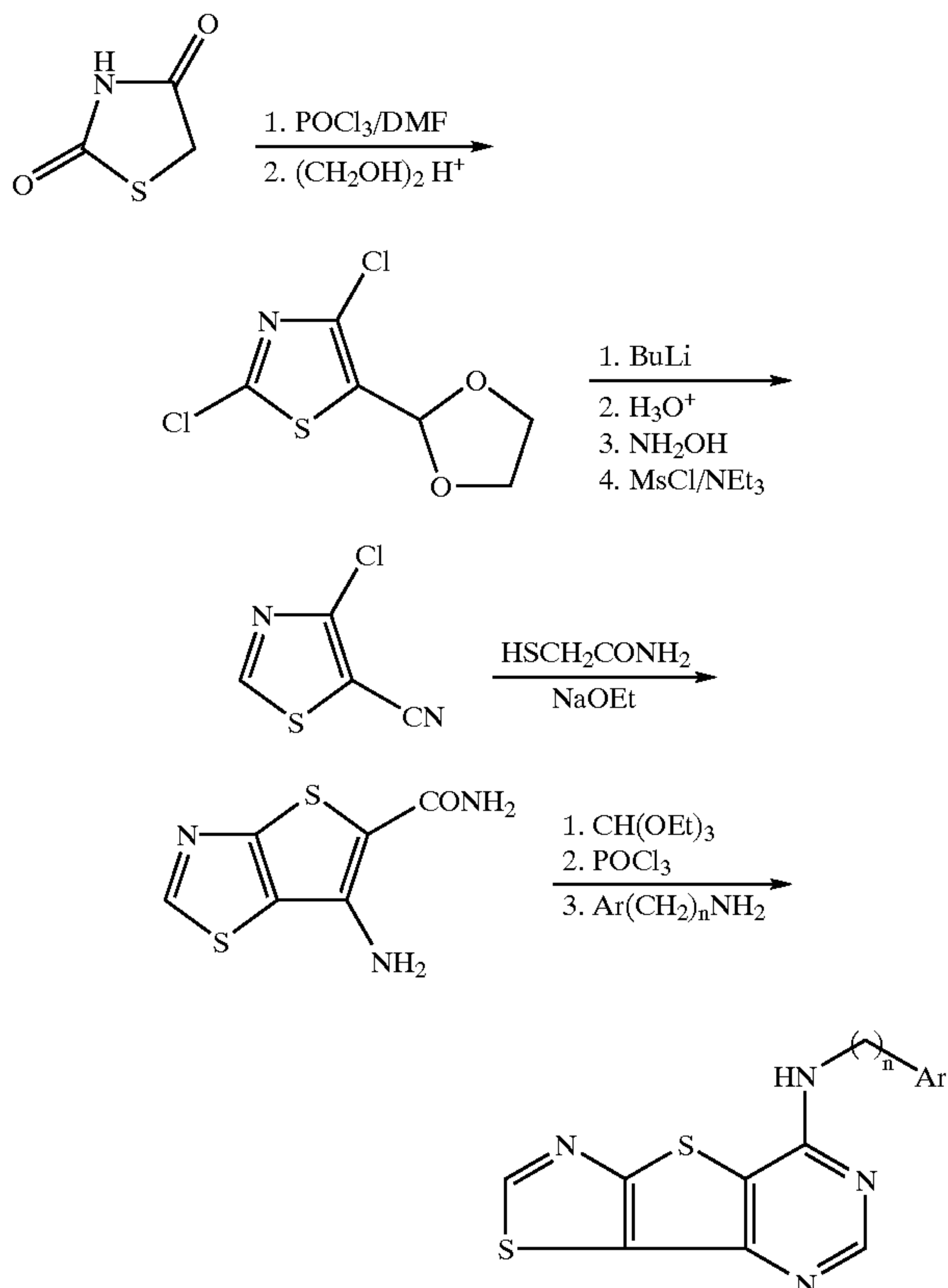
Scheme 20
