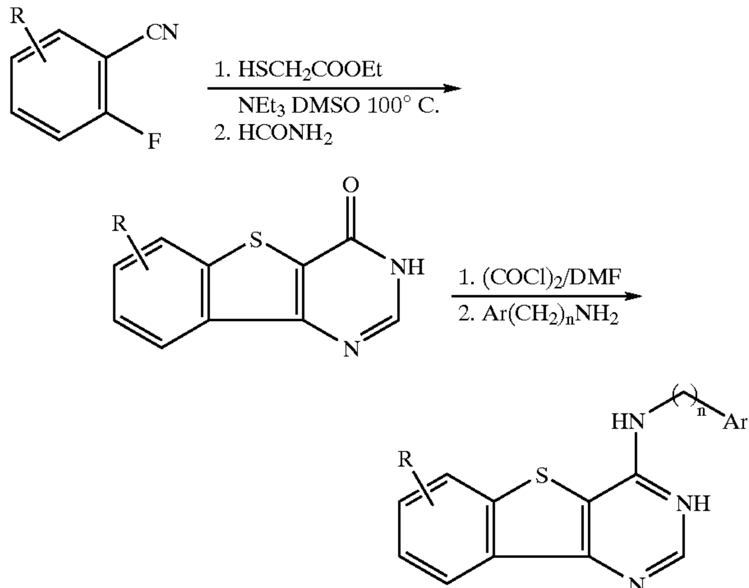
Scheme 15
