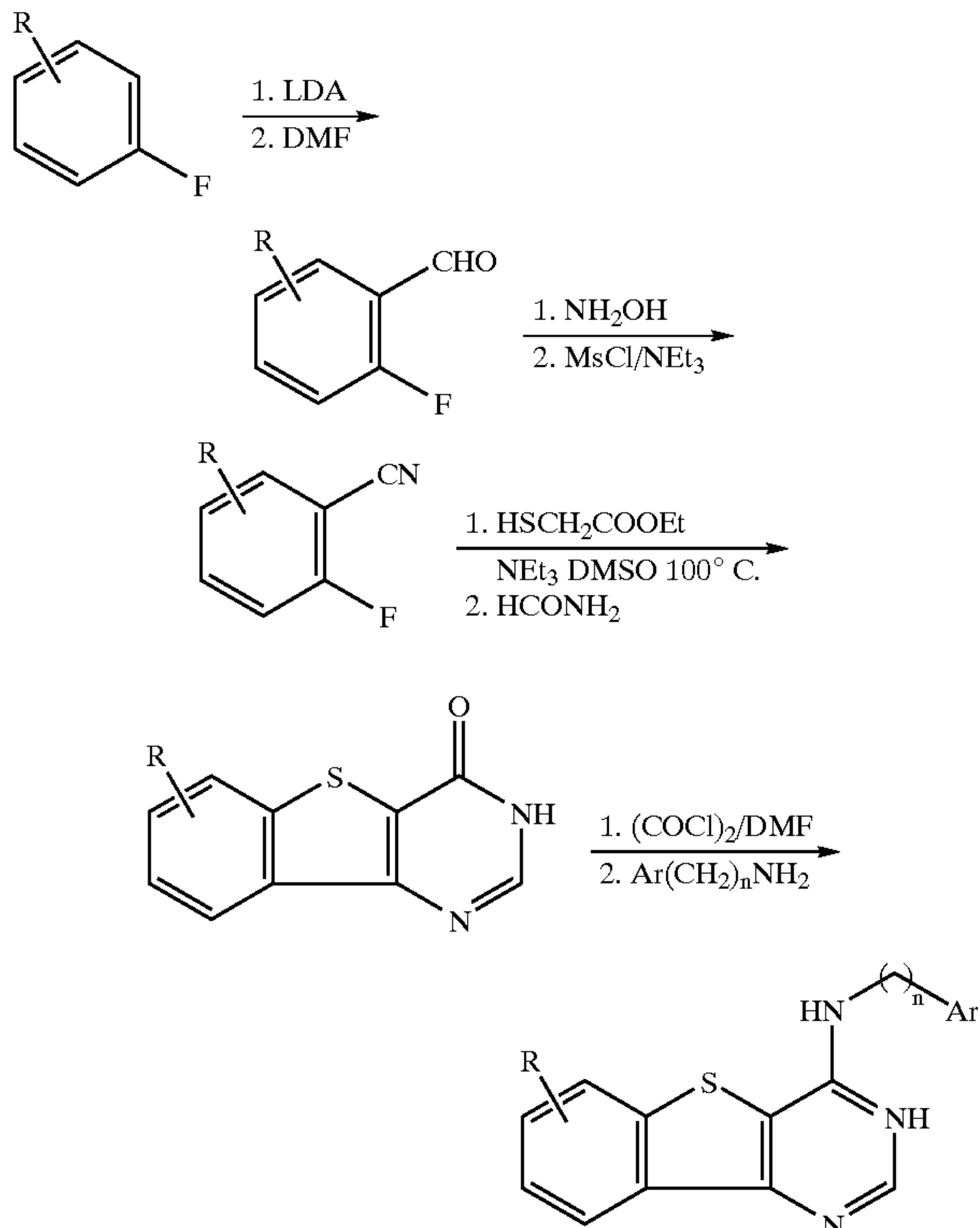
Scheme 16
