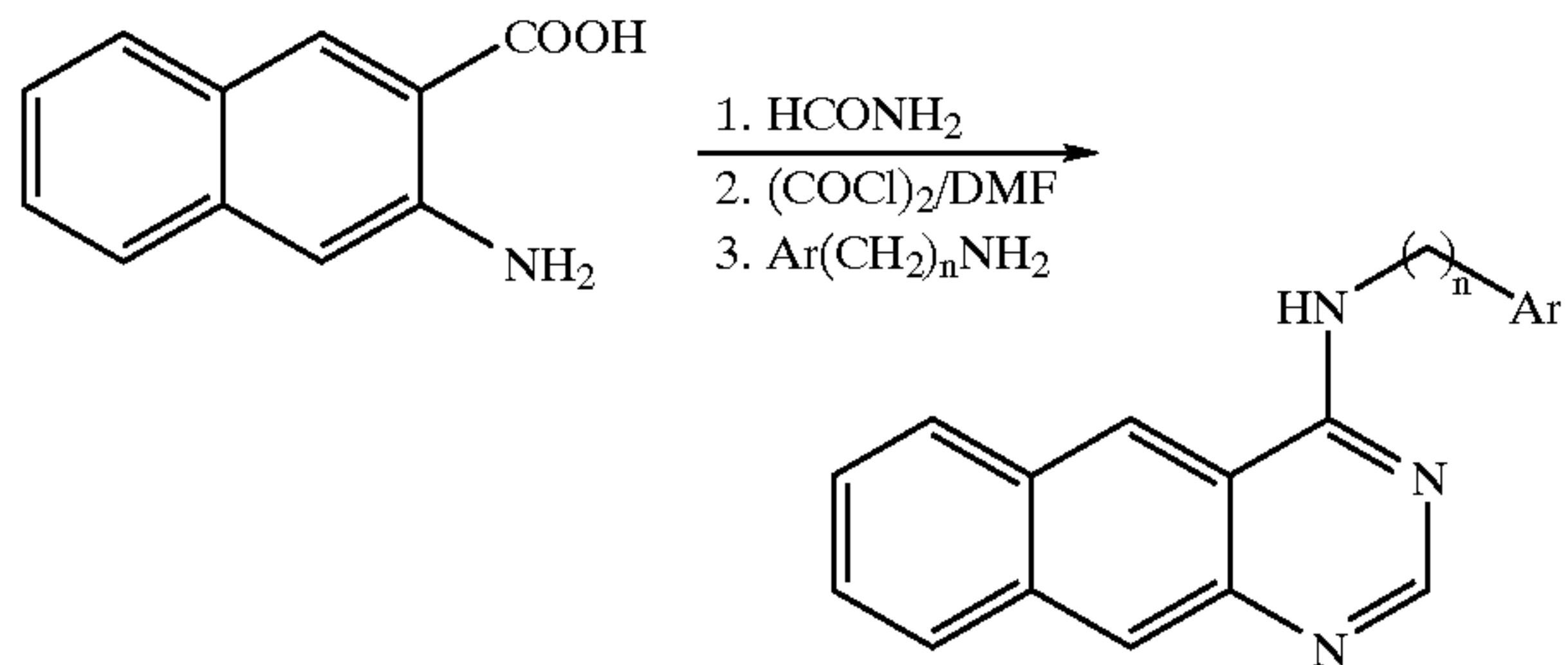
Scheme 2
