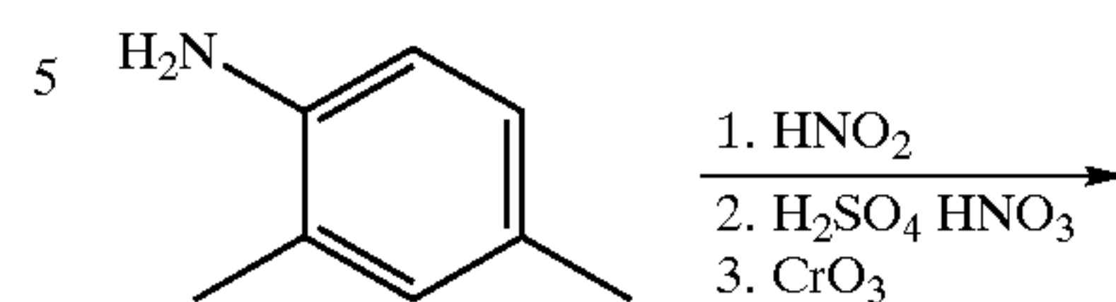
Scheme 8
