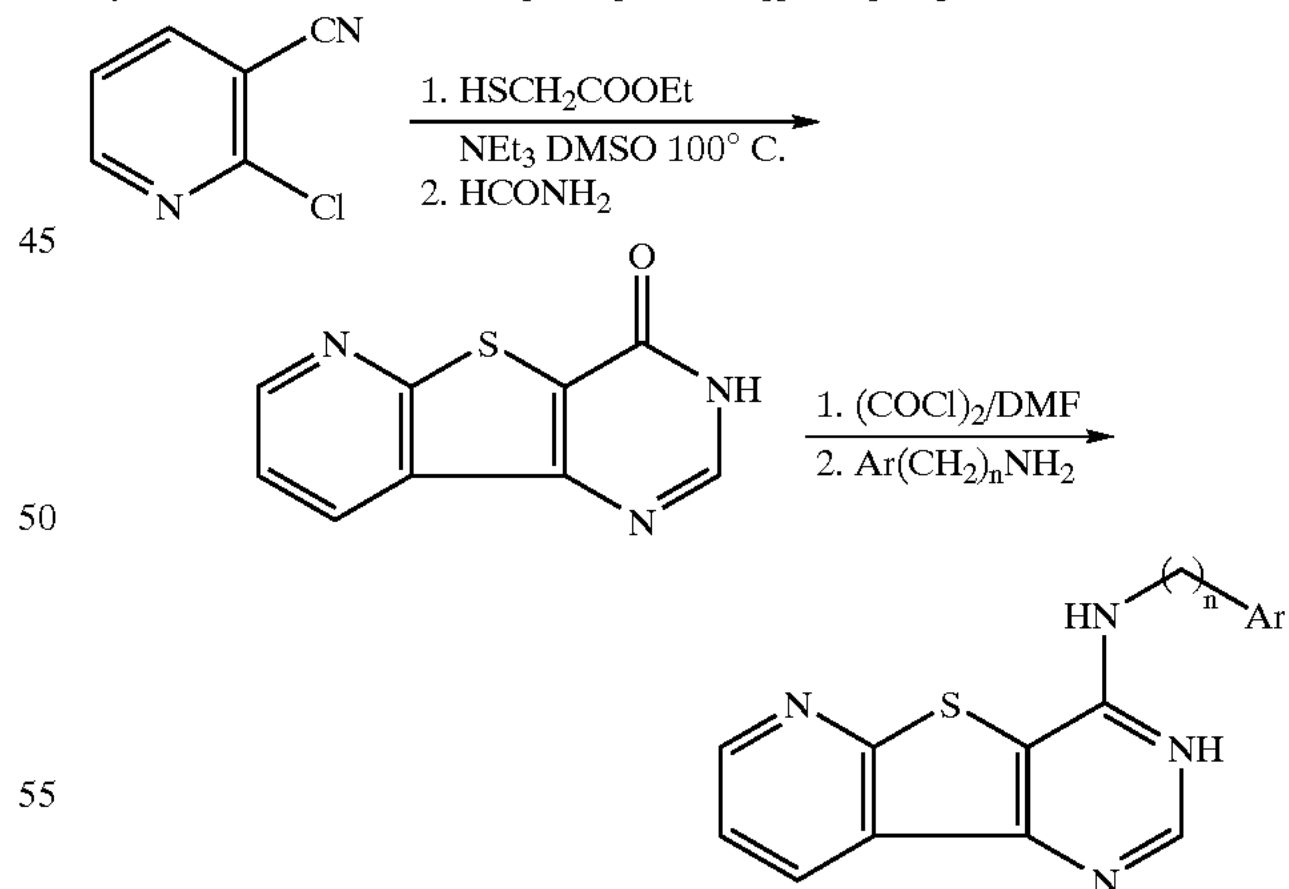
Scheme 22
