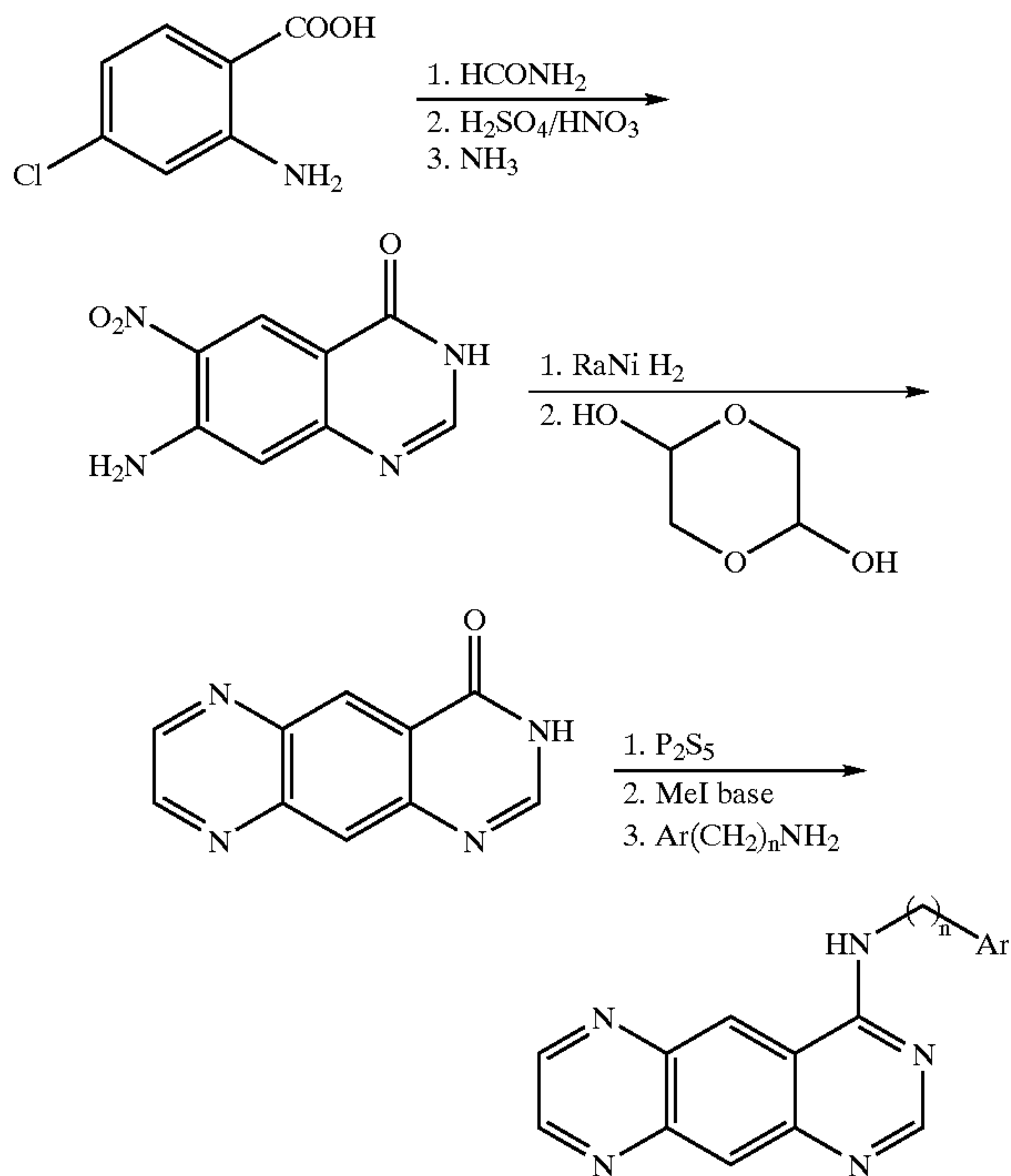
Scheme 11
