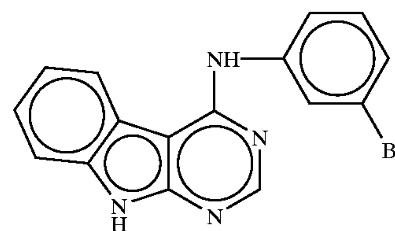
EXAMPLE 29
