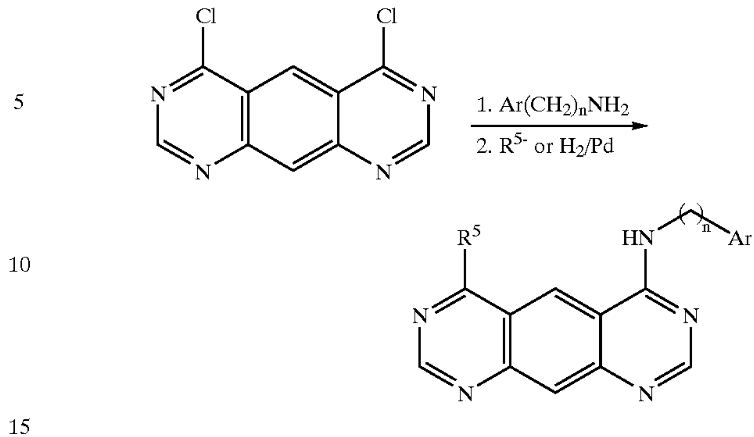
Scheme 13
