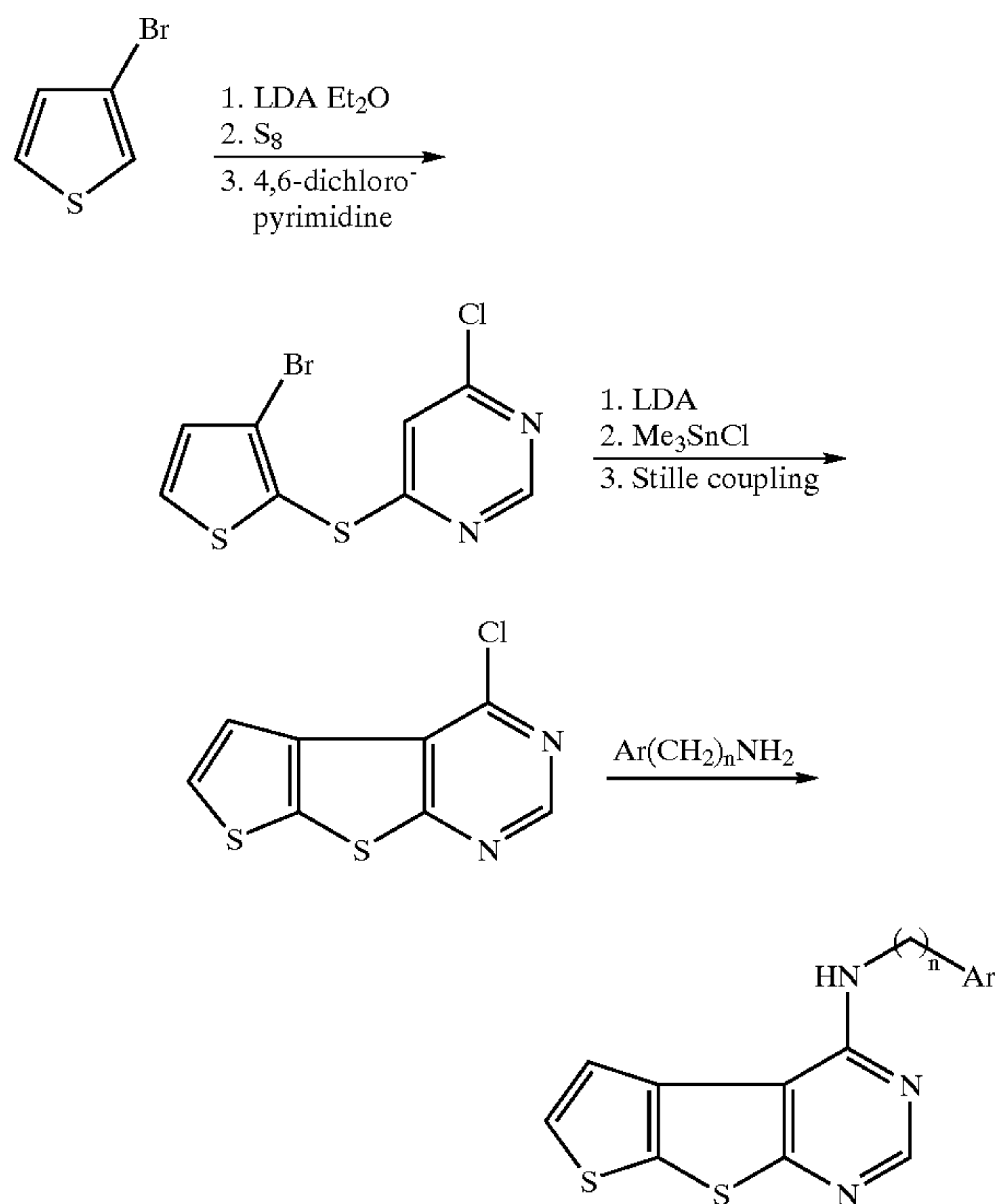
Scheme 19
