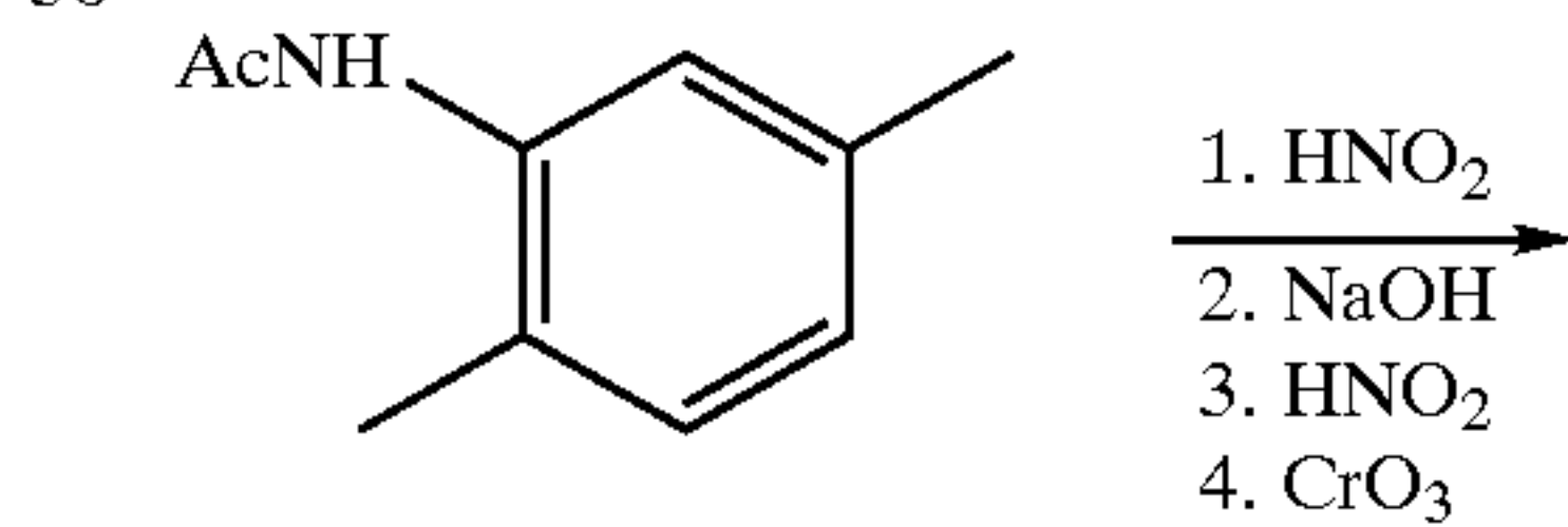
Scheme 9
