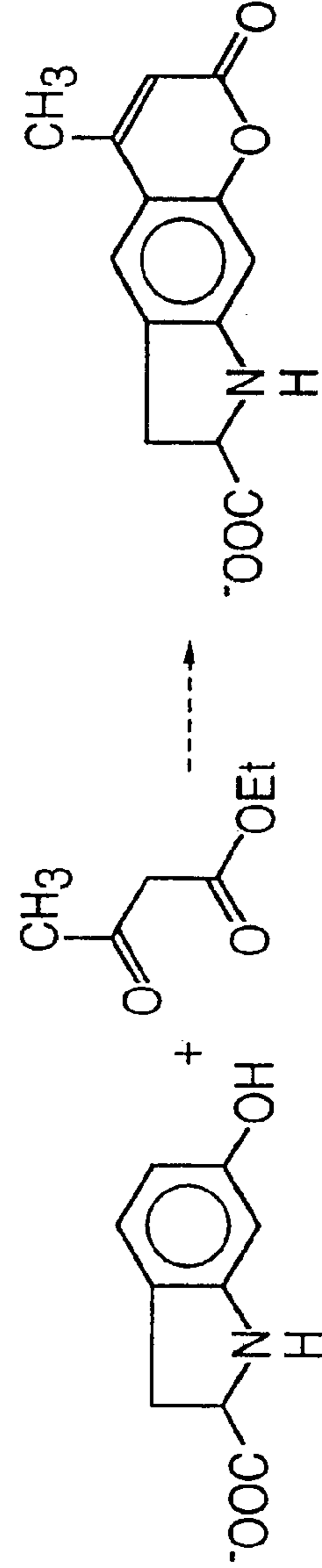
(R=H, METHYL, ETHYL ETC.) 6,7 - (4', 5' -PROLINO) COUMARIN BASED ANALOGS
