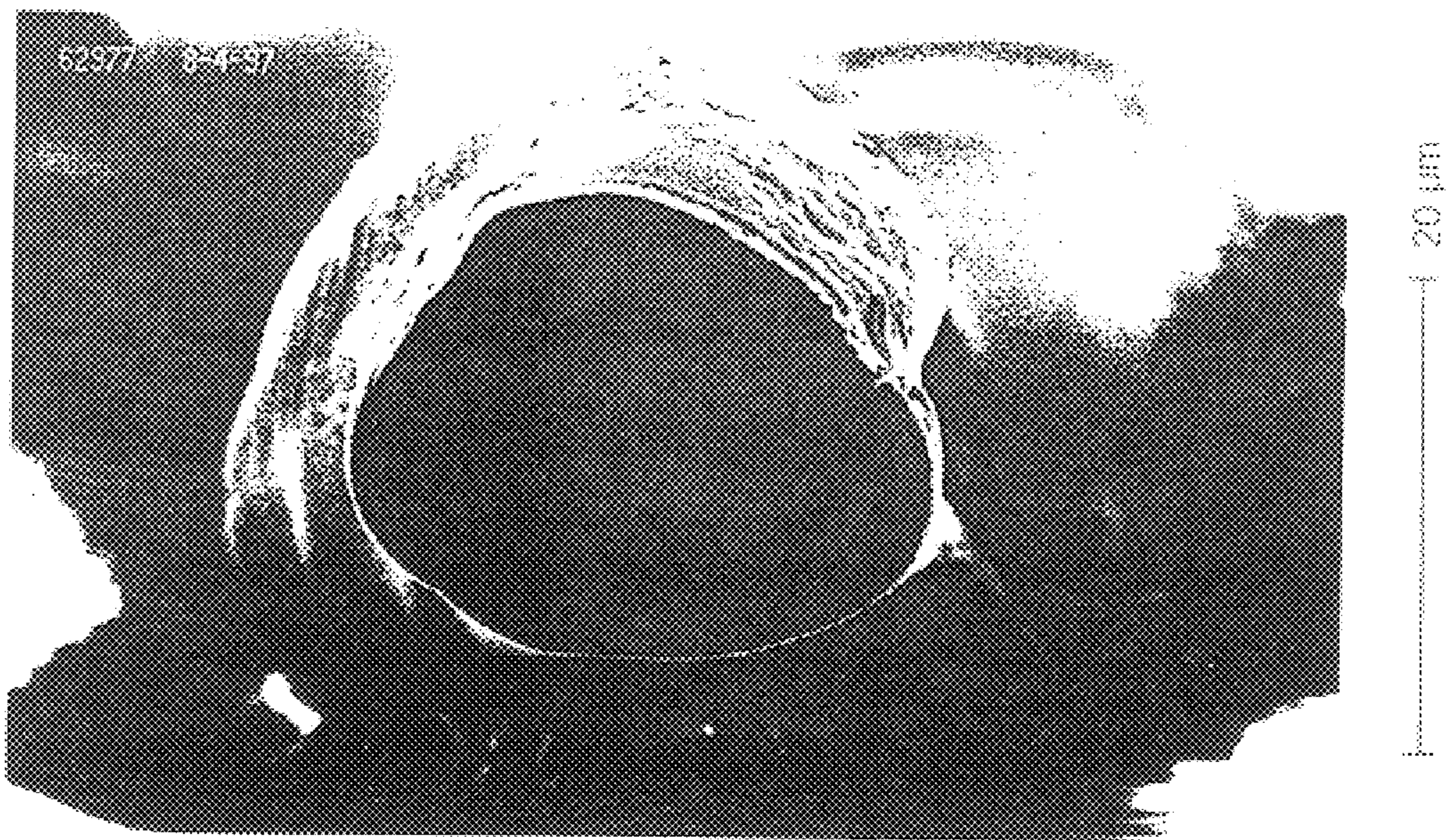
Centrifugally Spun Fiber End - 2,000X
