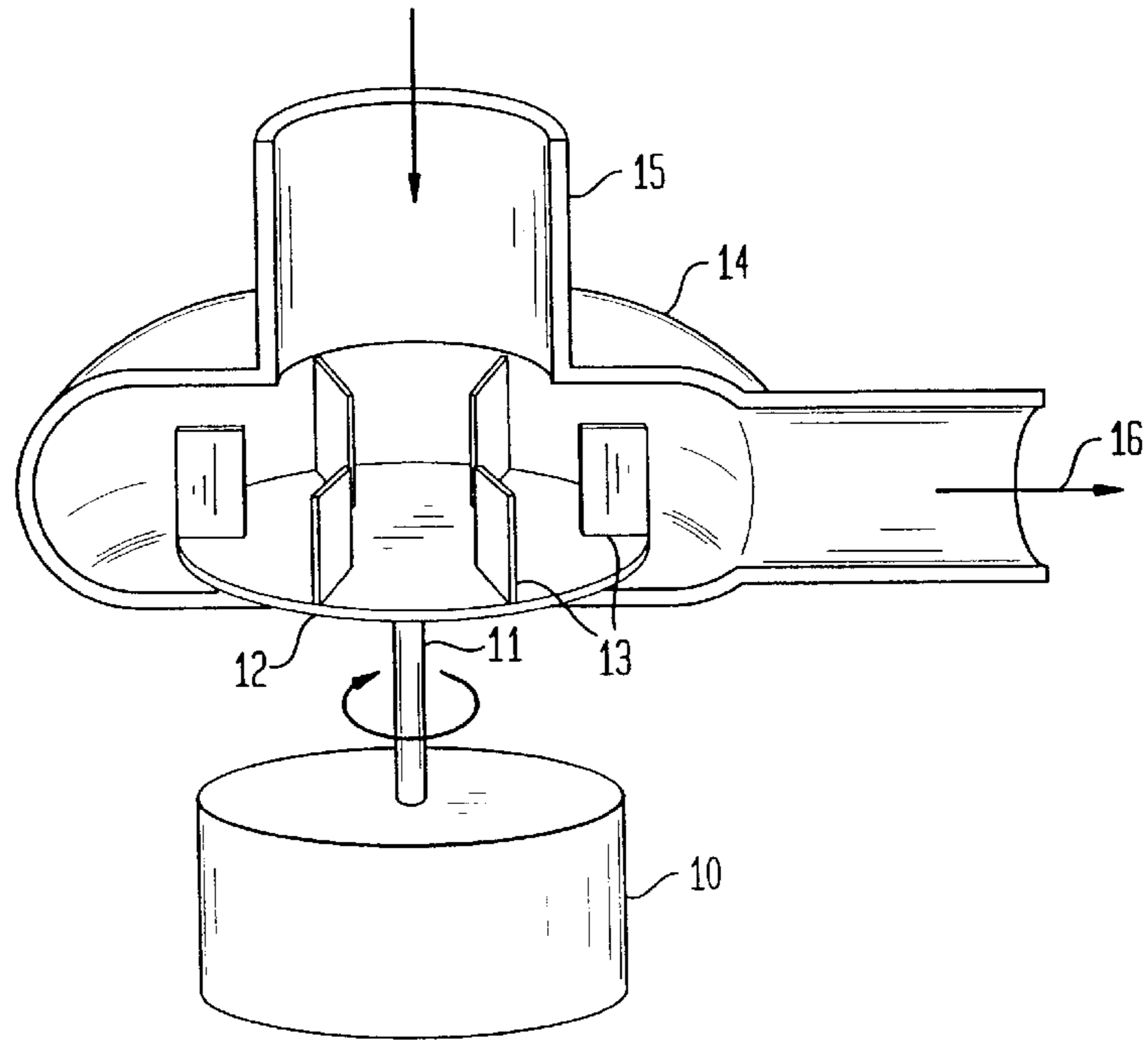
FIG. 13 (PRIOR ART)
