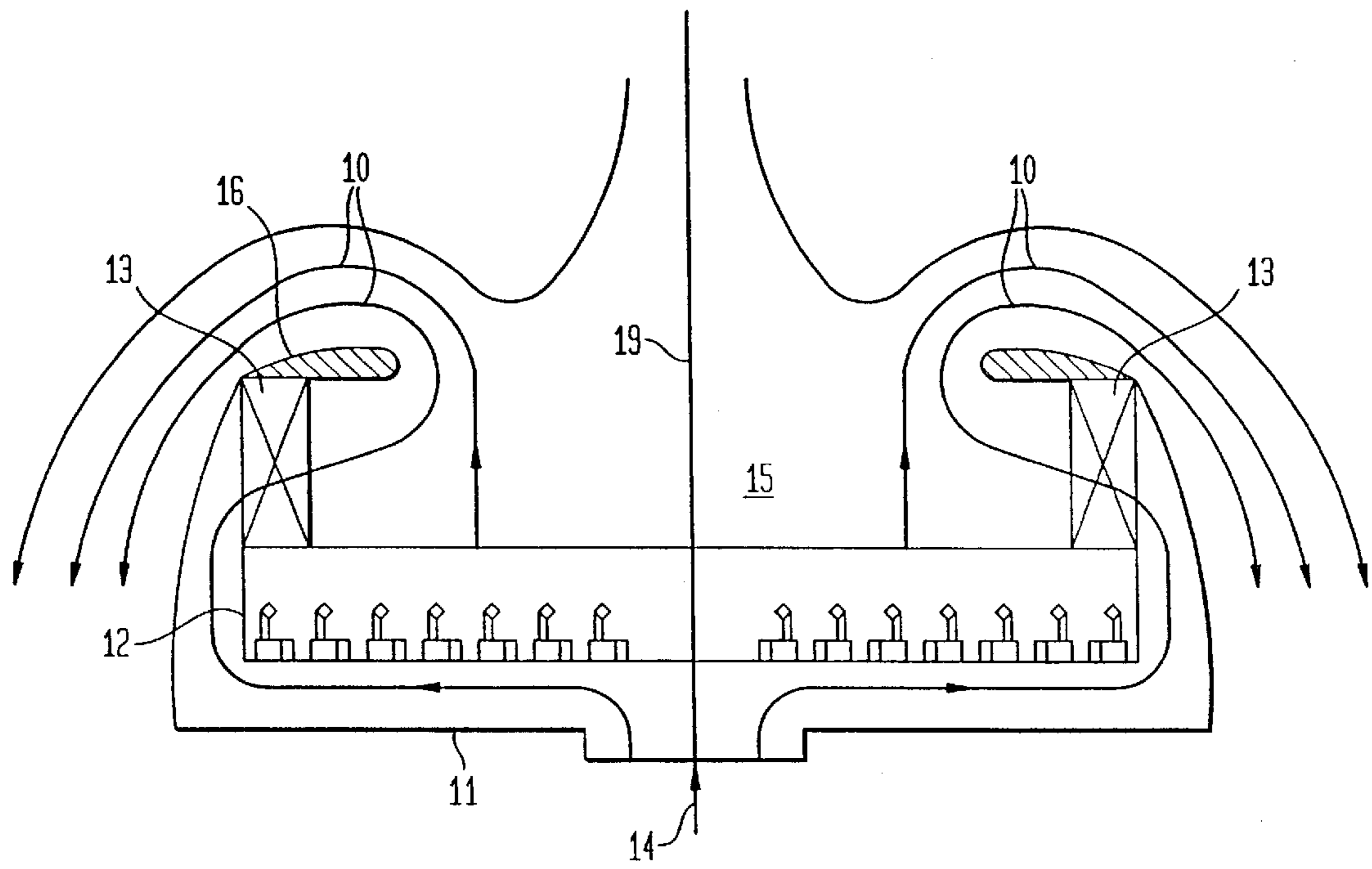
FIG. 1 (PRIOR ART)
