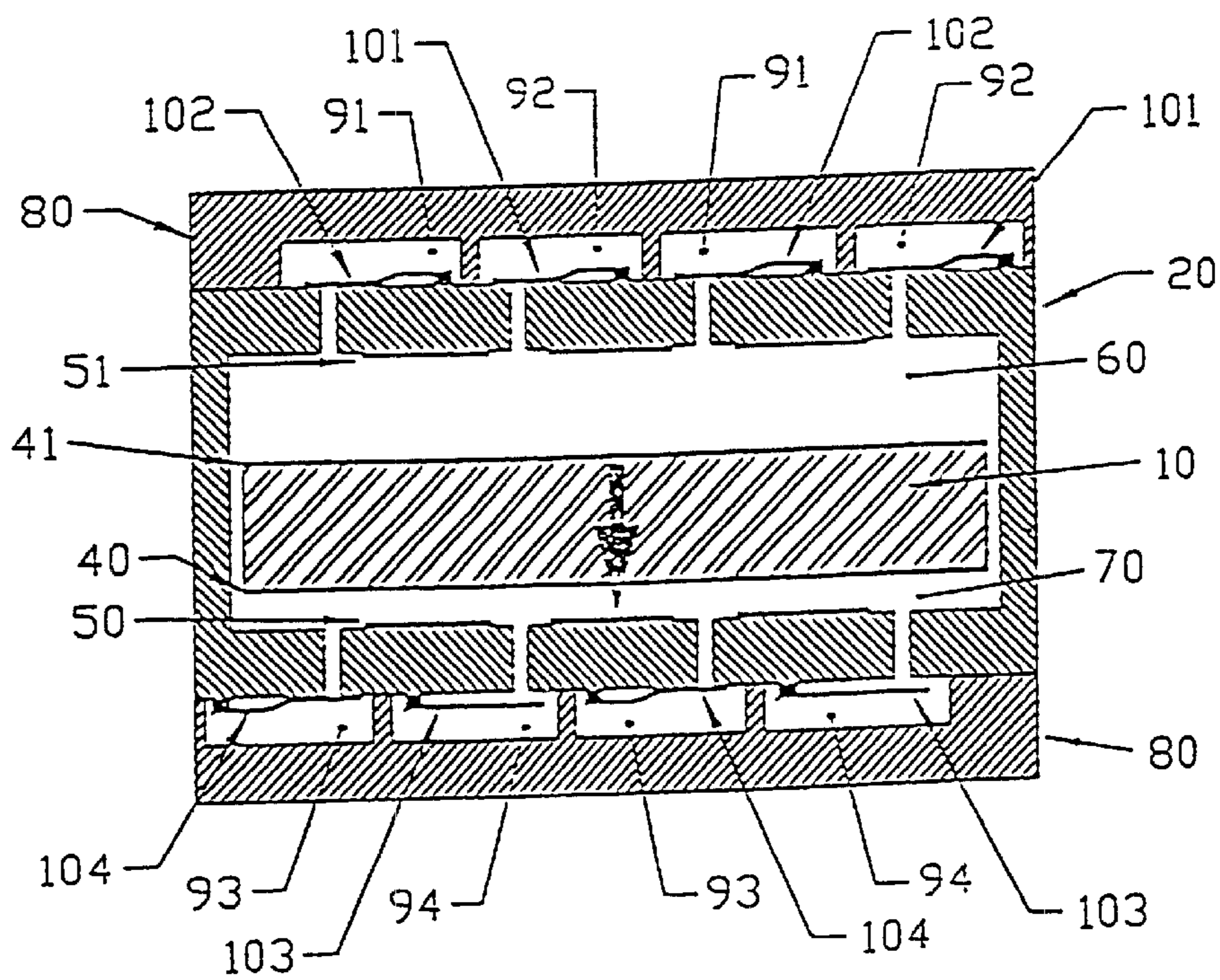
(expander, step 2) FIG. 5b
