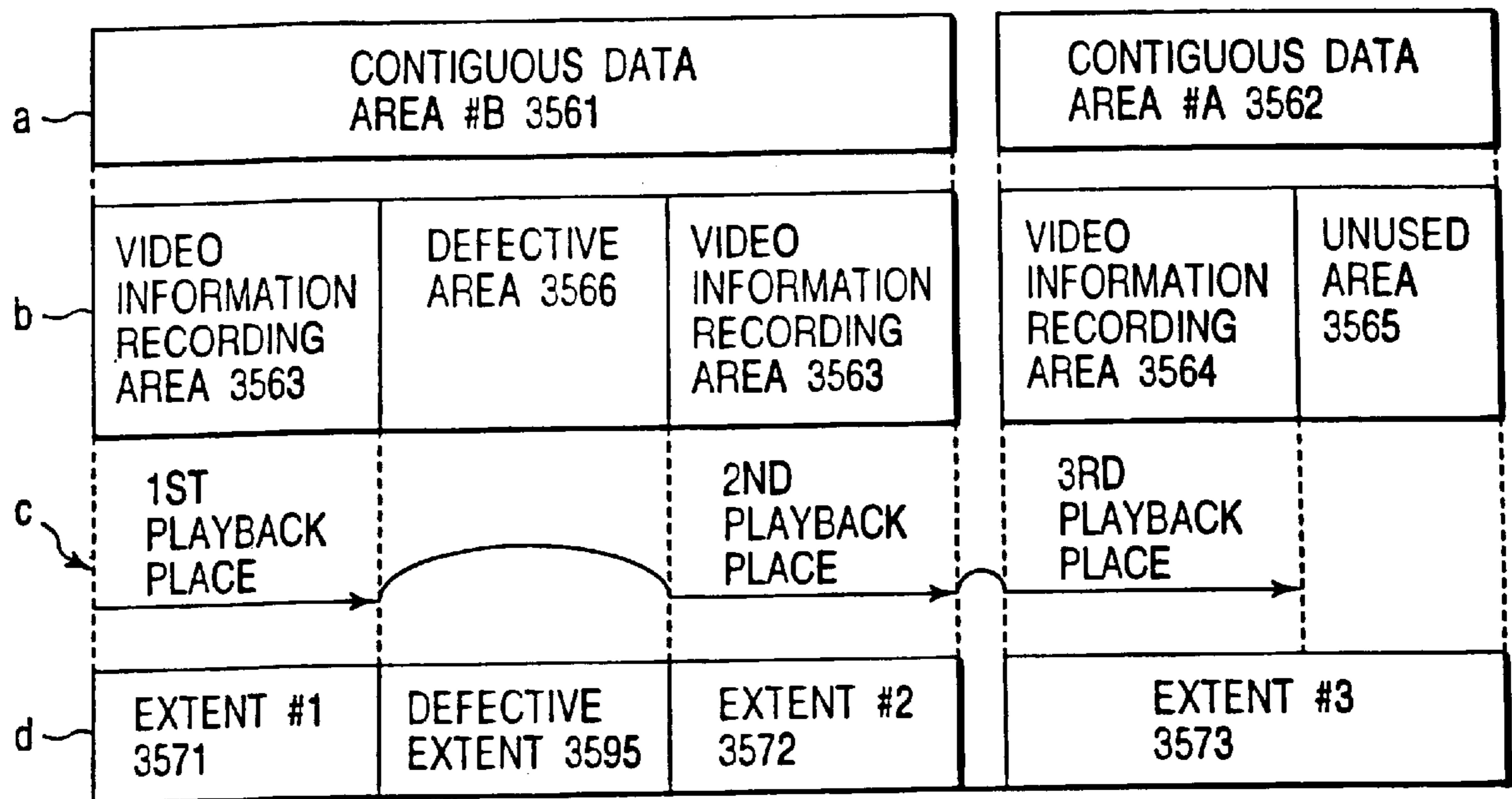
EXPLANATORY DIAGRAM OF ANOTHER EMBODIMENT RELATED TO A RECORDING METHOD AVOIDING DEFECTIVE AREA ACCORDING TO THE PRESENT INVENTION
