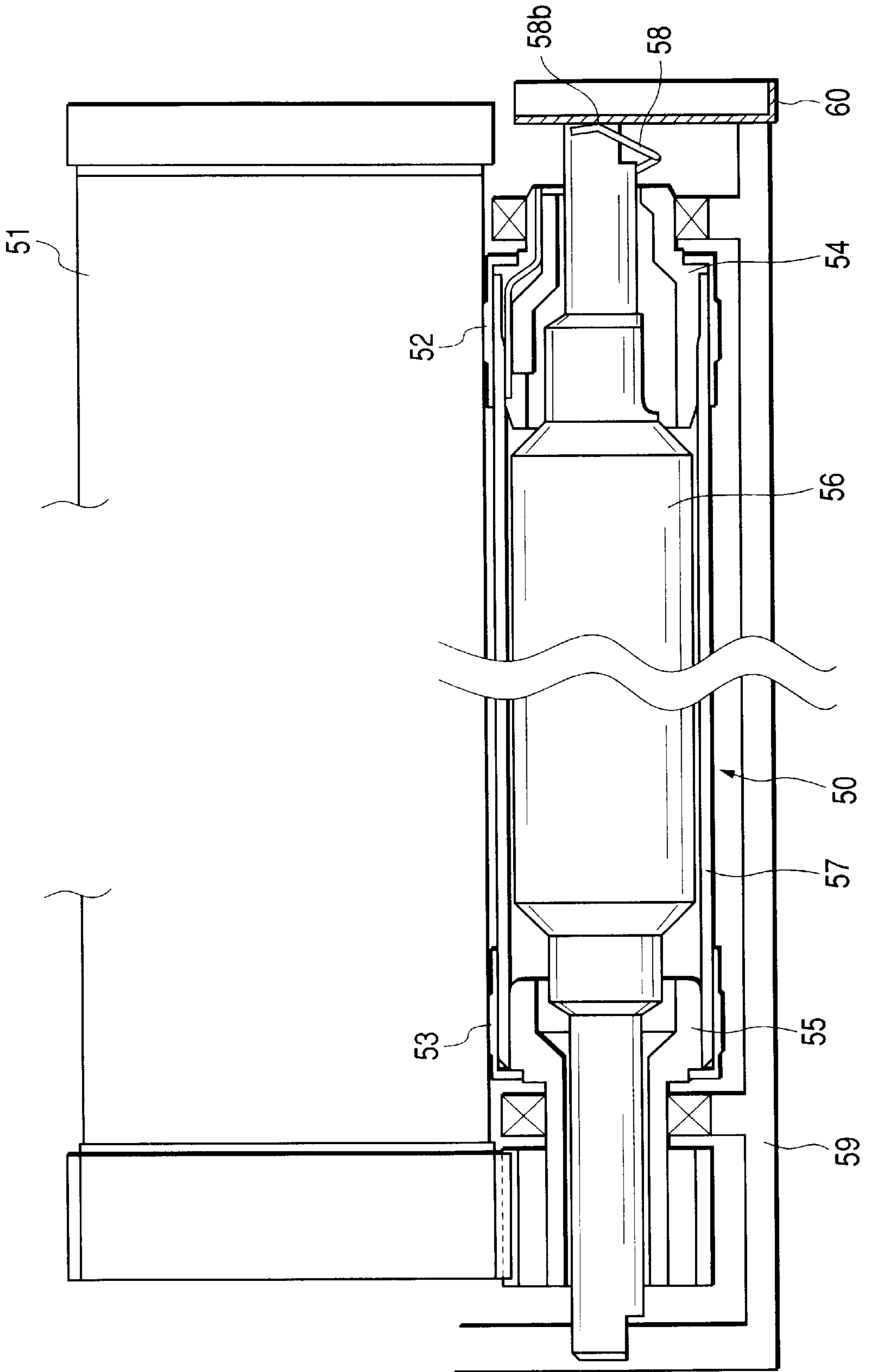
FIG. 2 PRIOR ART
