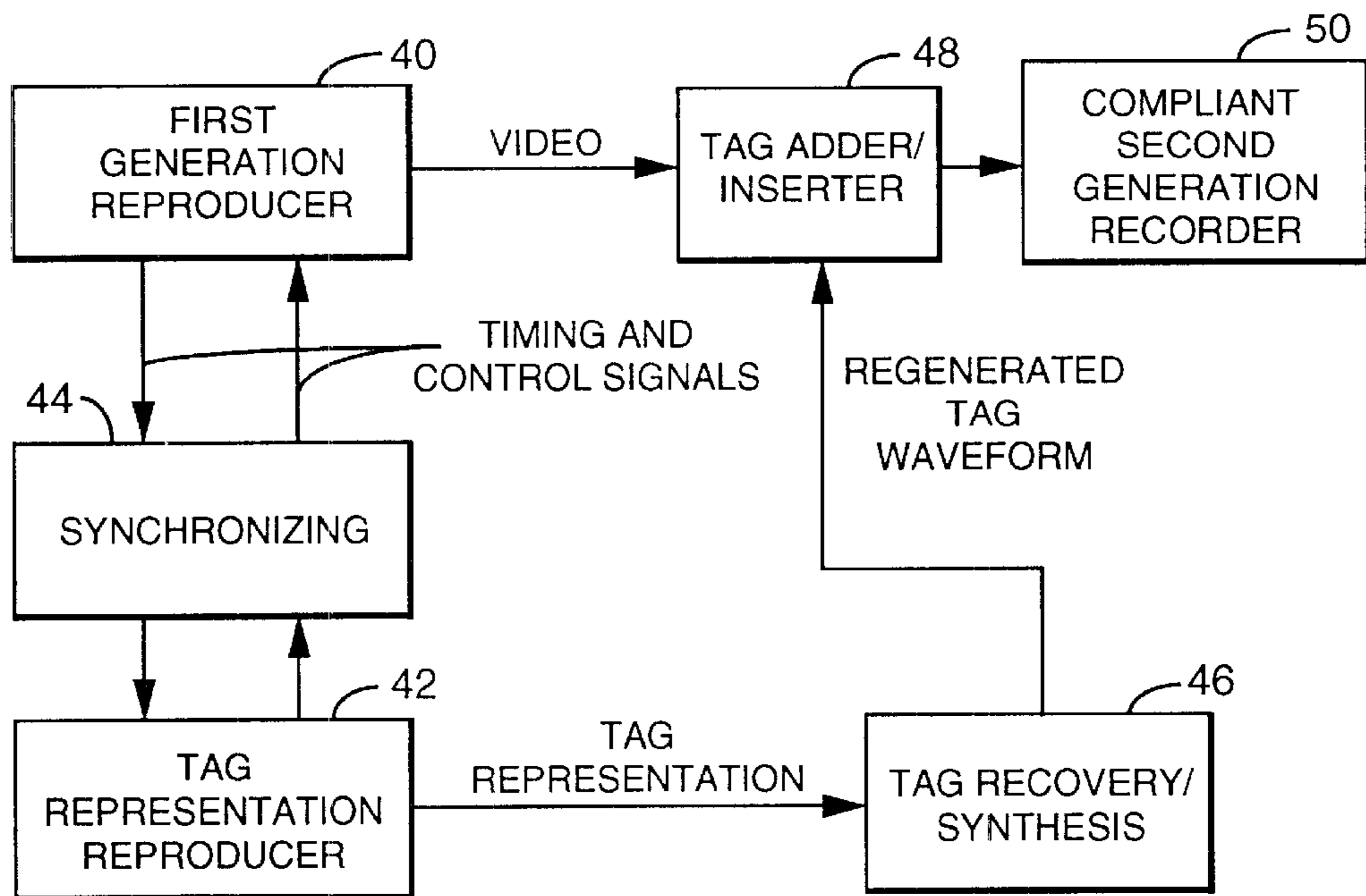
FIG. 4 (PLAYBACK)
