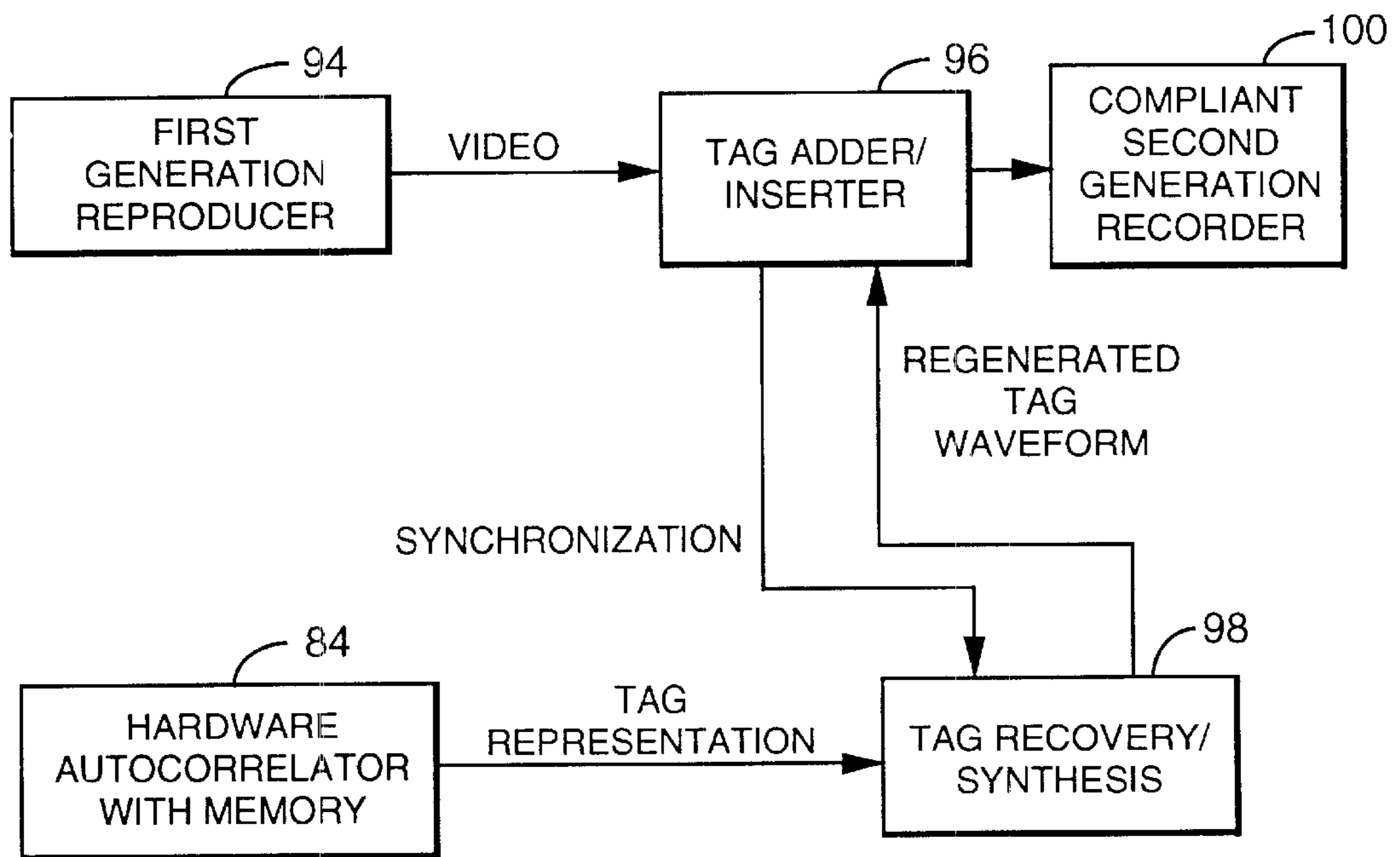
FIG. 10 (PLAYBACK)
