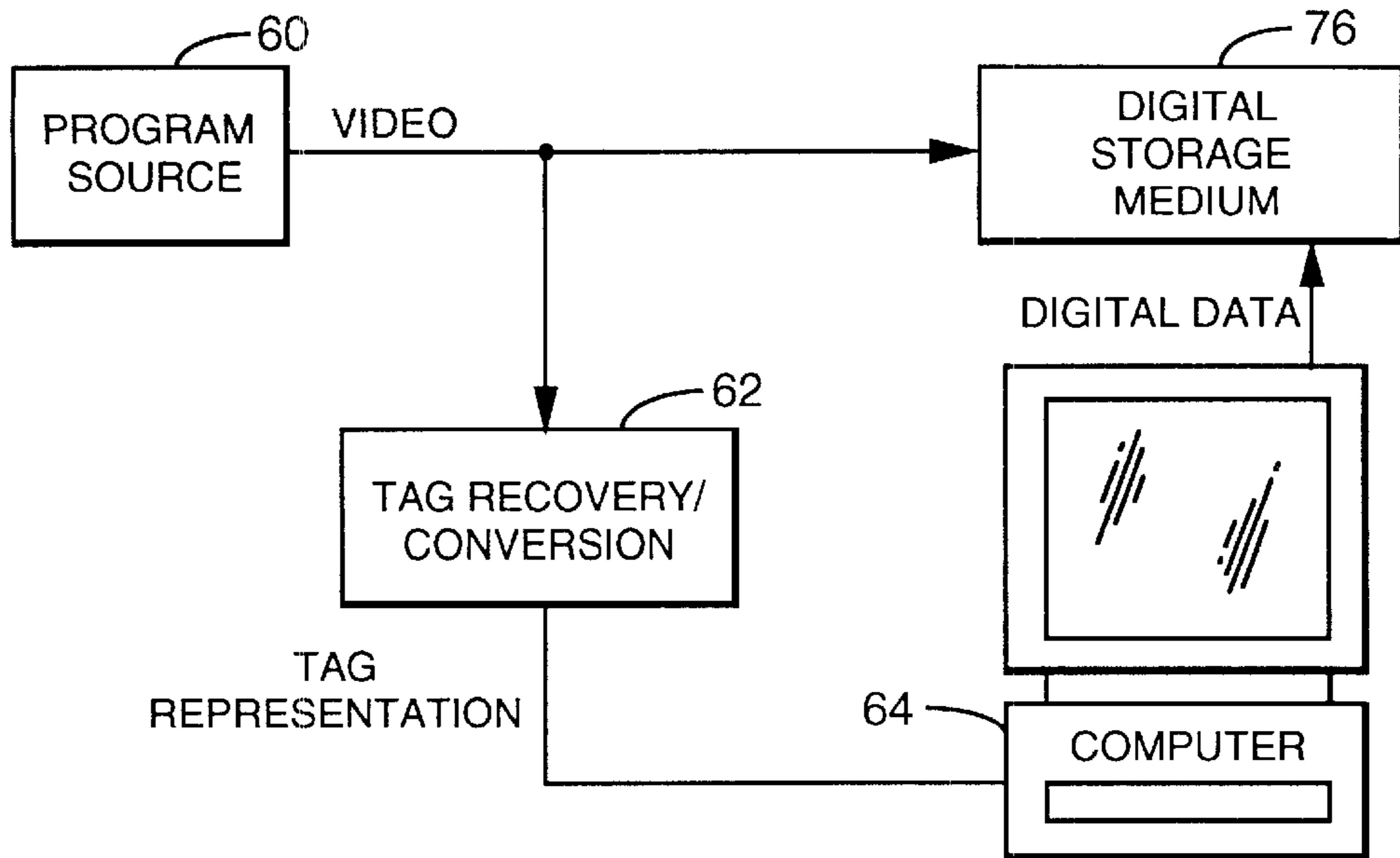
FIG. 7 (RECORDING)
