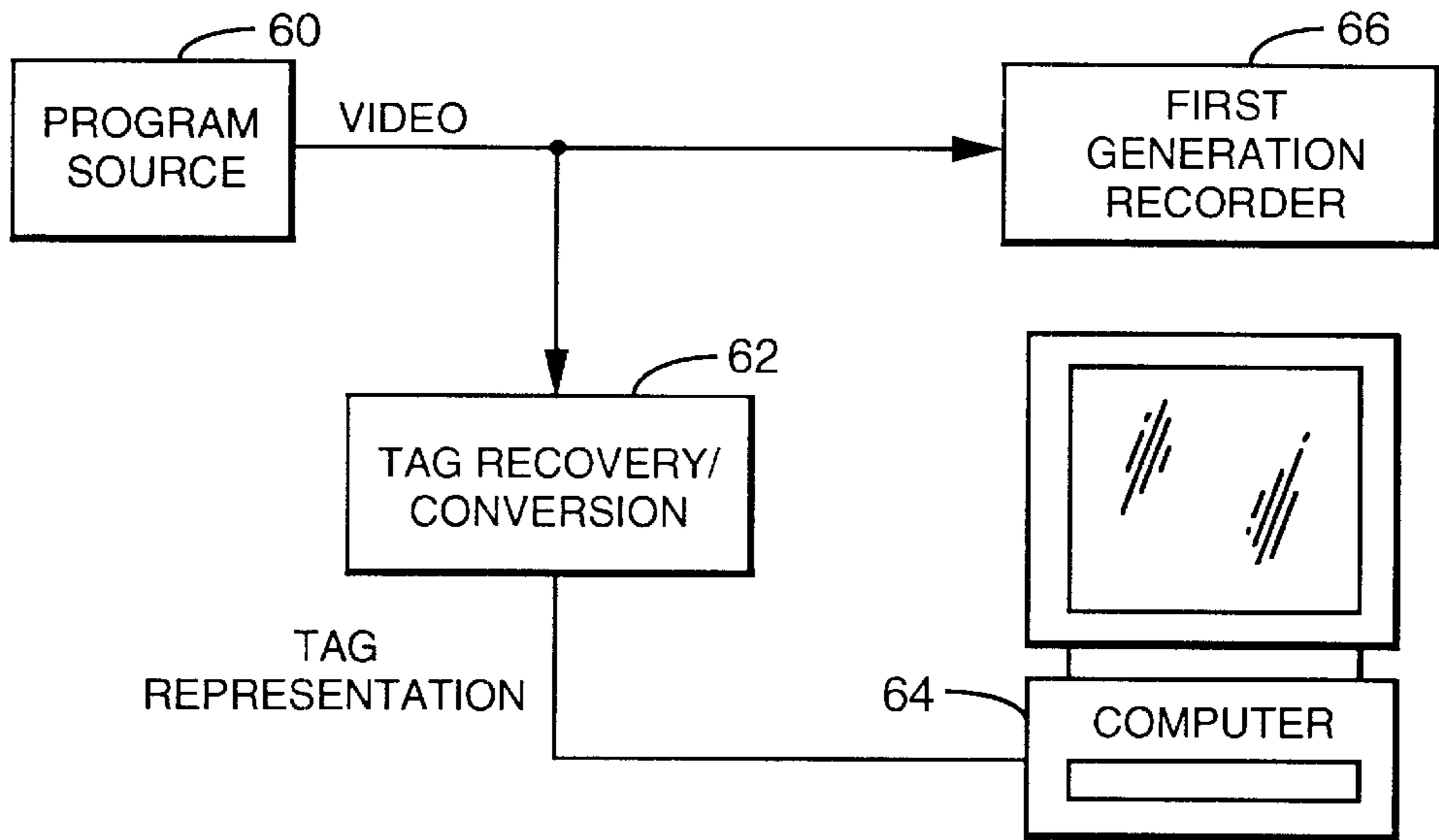
FIG. 5 (RECORDING)
