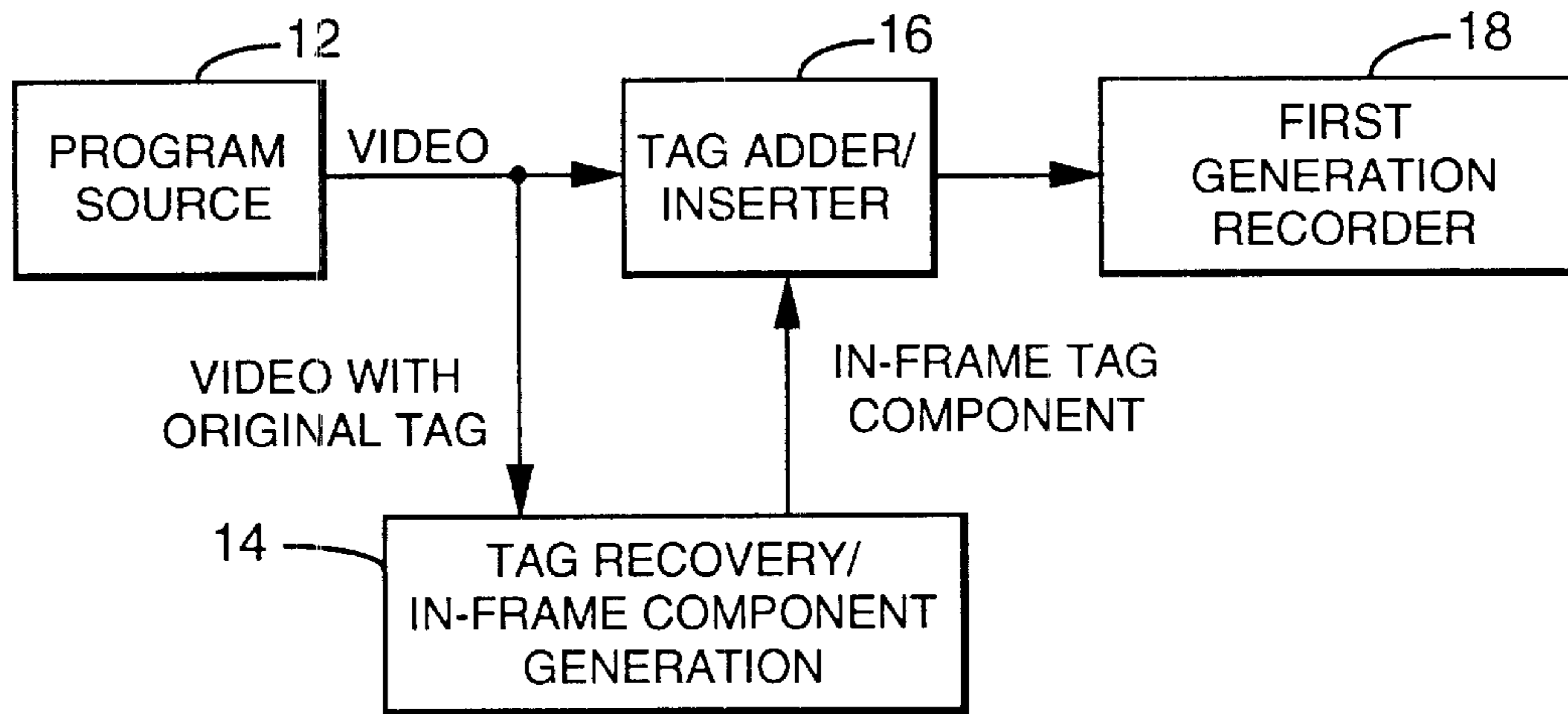
FIG. 1 (RECORDING)
