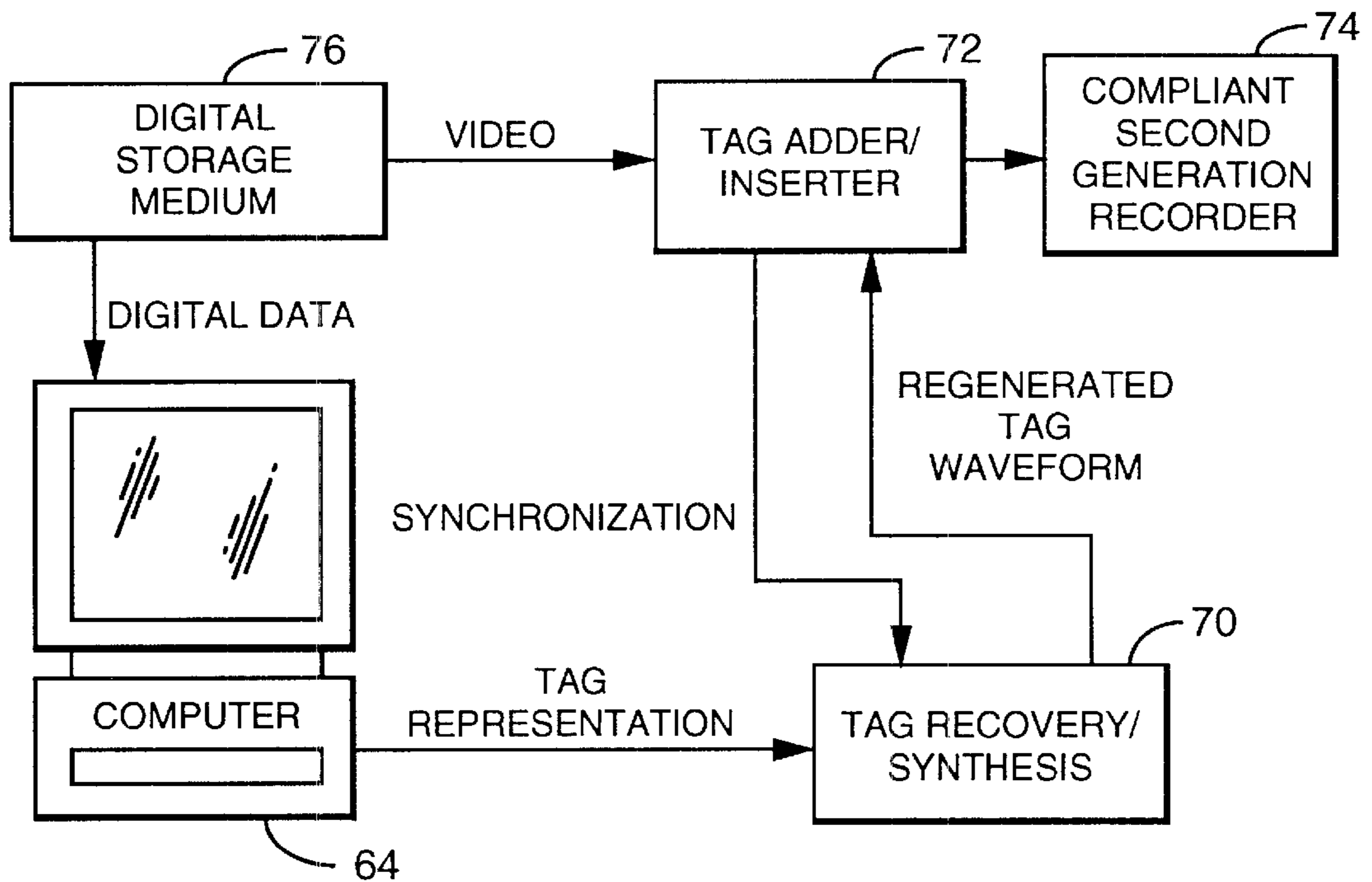
FIG. 8 (PLAYBACK)
