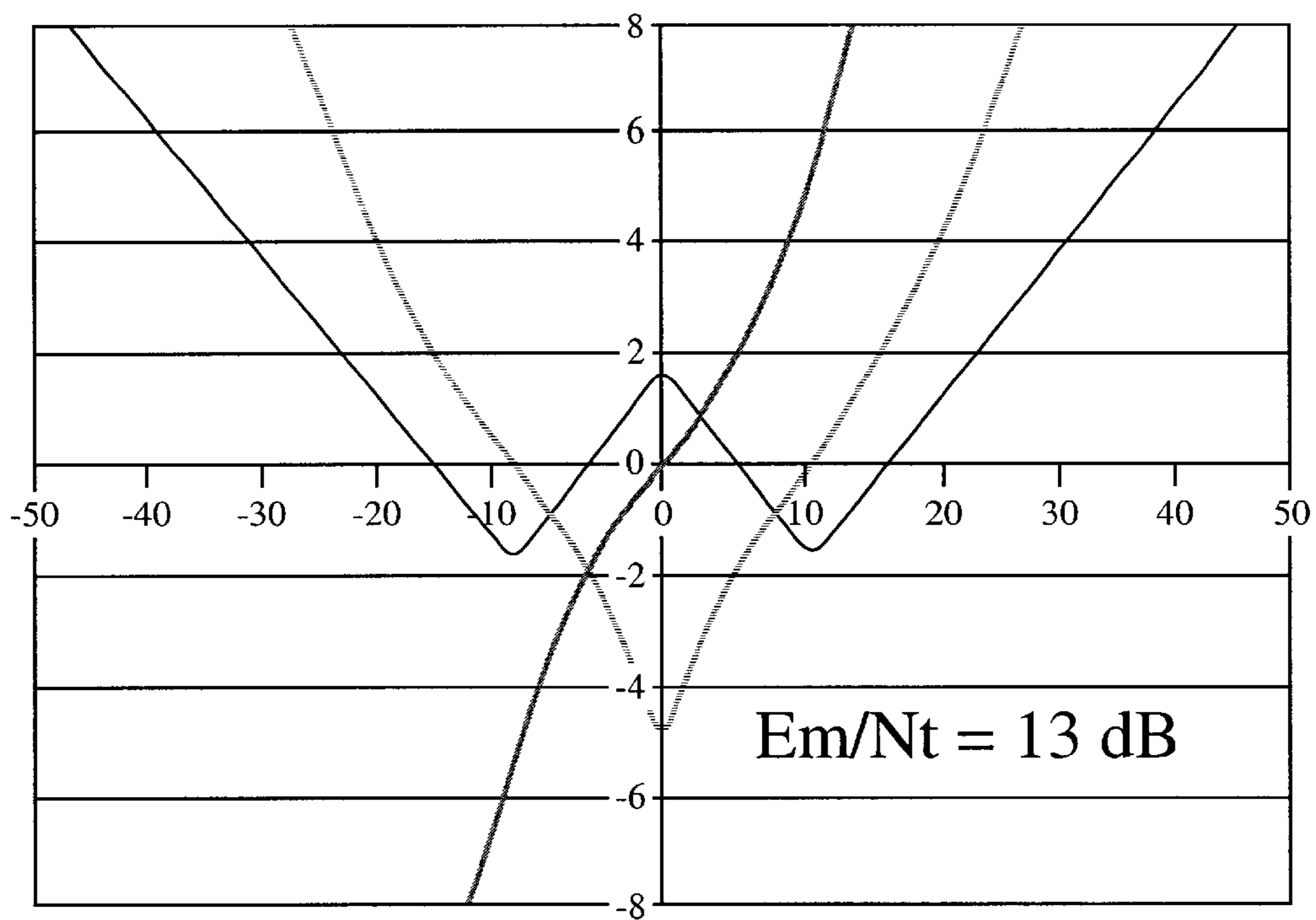
64 - QAM LLRs VS. MODULATION SYMBOL METRIC
