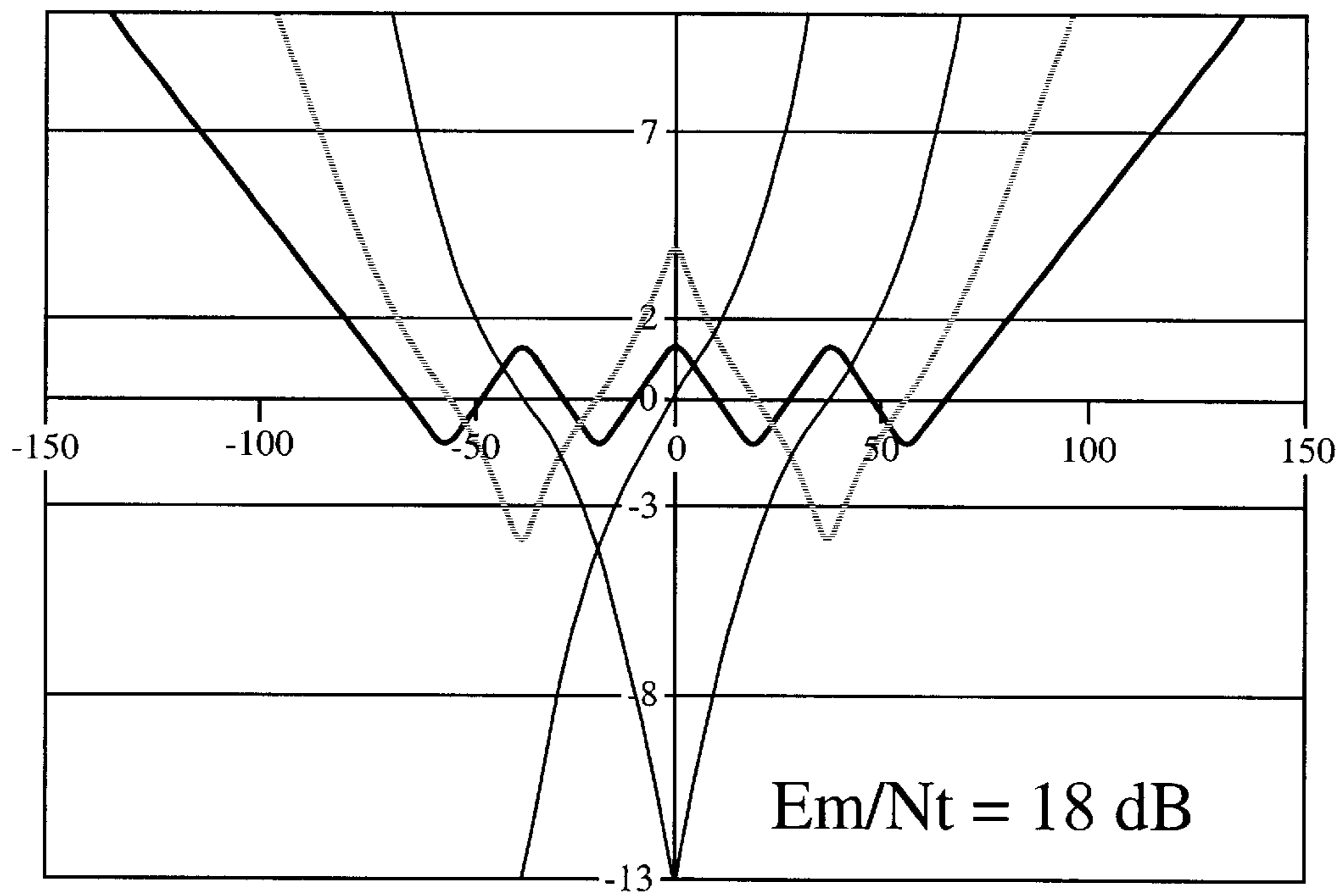
256 - QAM LLRs VS. MODULATION SYMBOL METRIC
