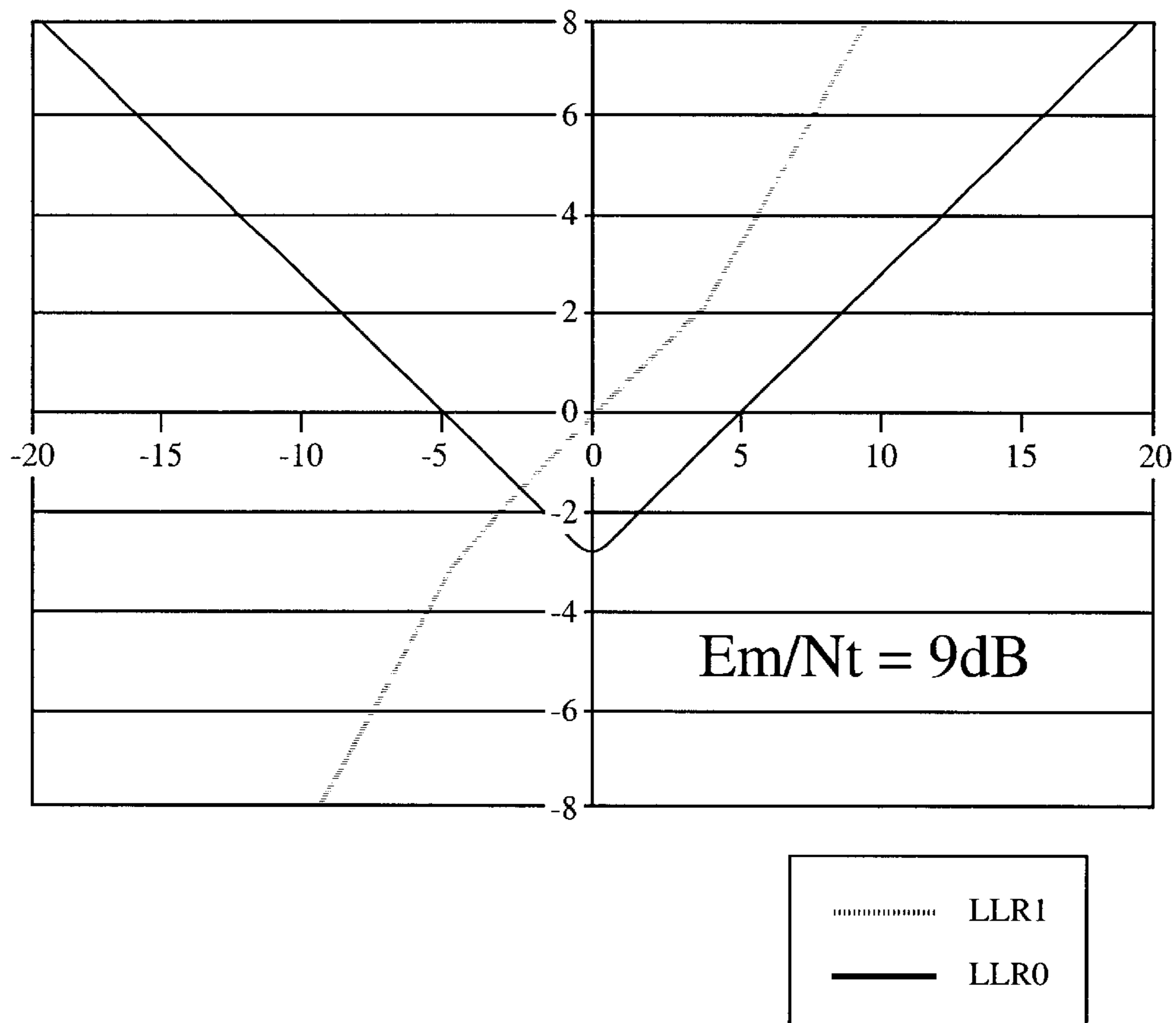
16 - QAM LLRs VS. MODULATION SYMBOL METRIC
