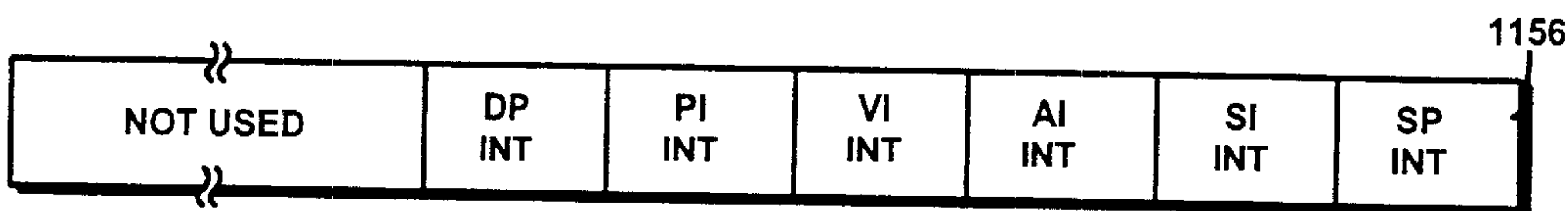
Fig. 39C INTERRUPT REGISTER (R)
