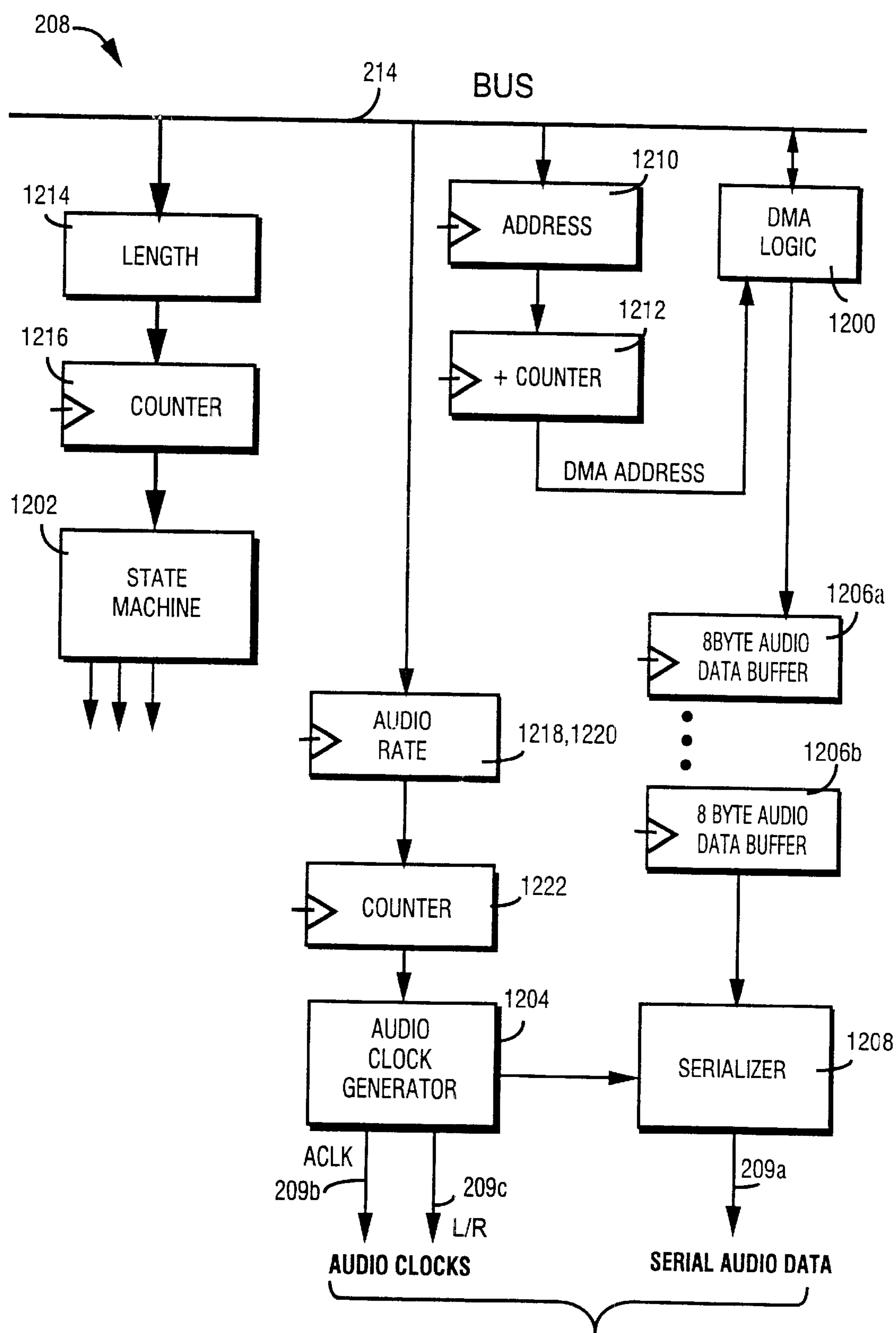
Fig. 40 EXAMPLE AUDIO INTERFACE ARCHITECTURE
