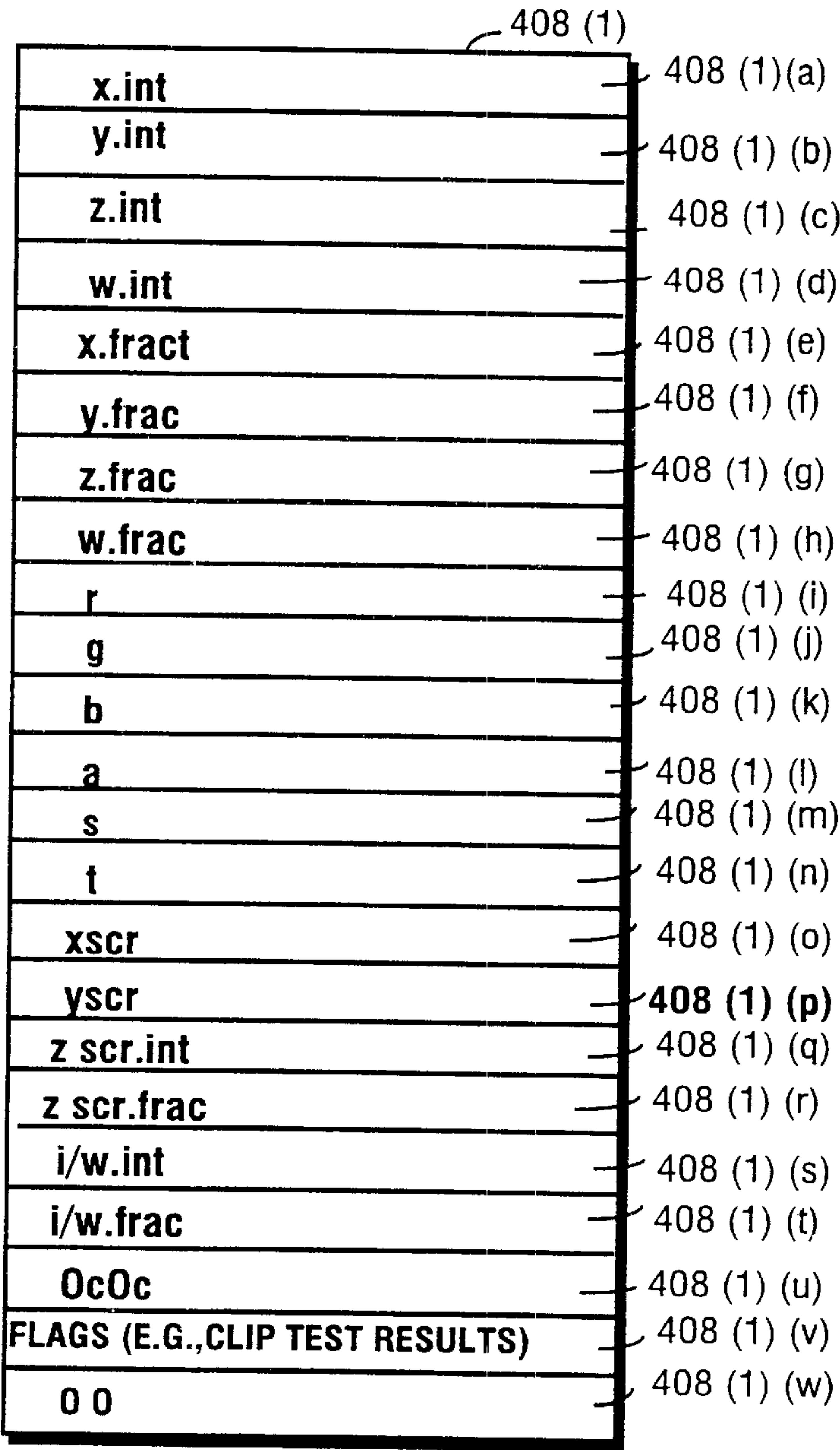
EXAMPLE VERTEX DATA STRUCTURE
