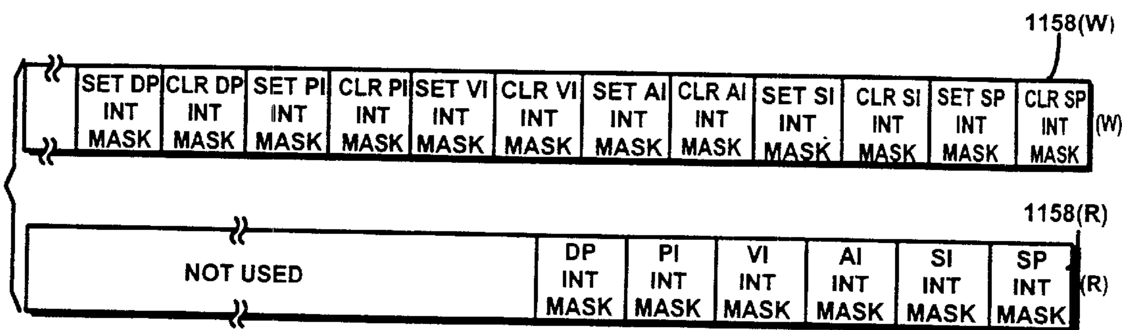
Fig. 39D INT MASK REGISTER
