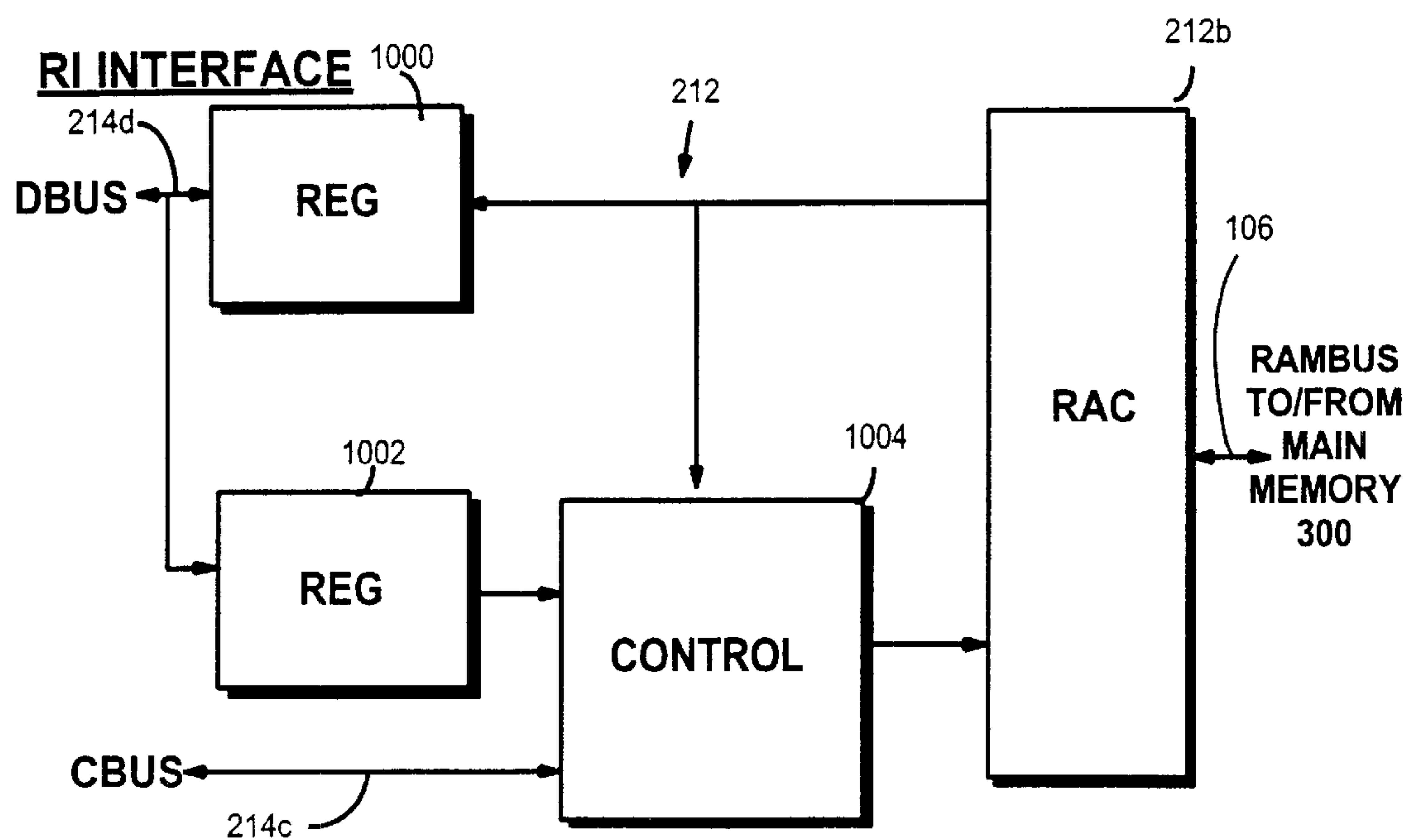
Fig. 36 EXAMPLE MEMORY INTERFACE
