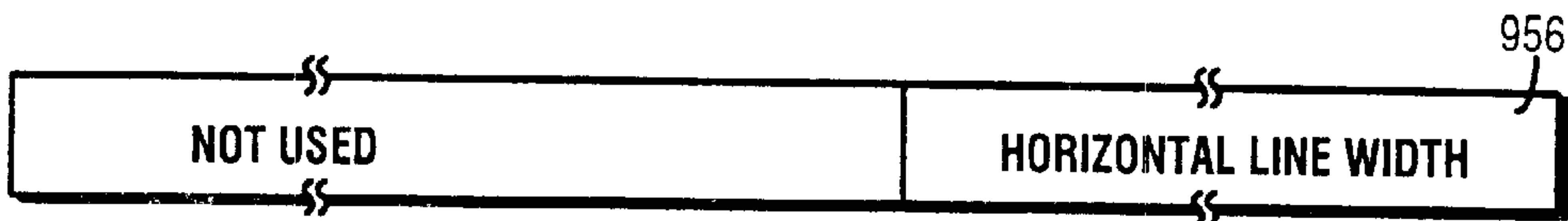
Fig. 35C VIDEO INTERFACE LINE WIDTH REGISTER (R/W)
