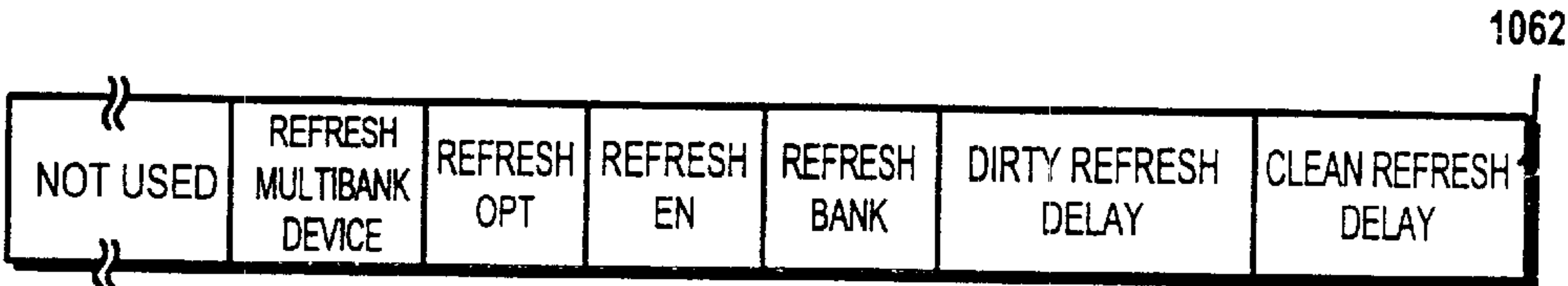
Fig. 37F REFRESH REGISTER (R/W)
