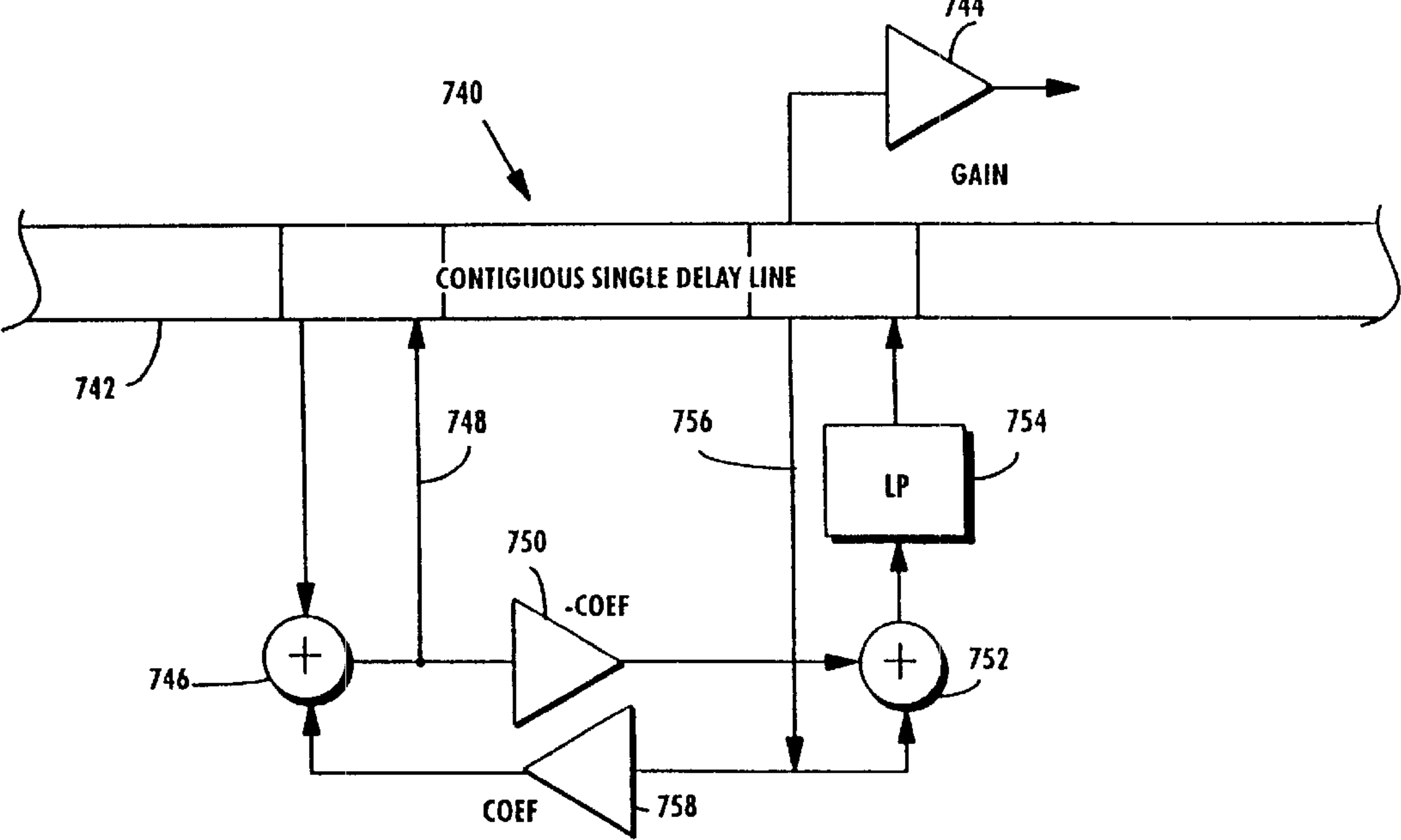
Fig. 17 EXAMPLE SP AUDIO PROCESSING
