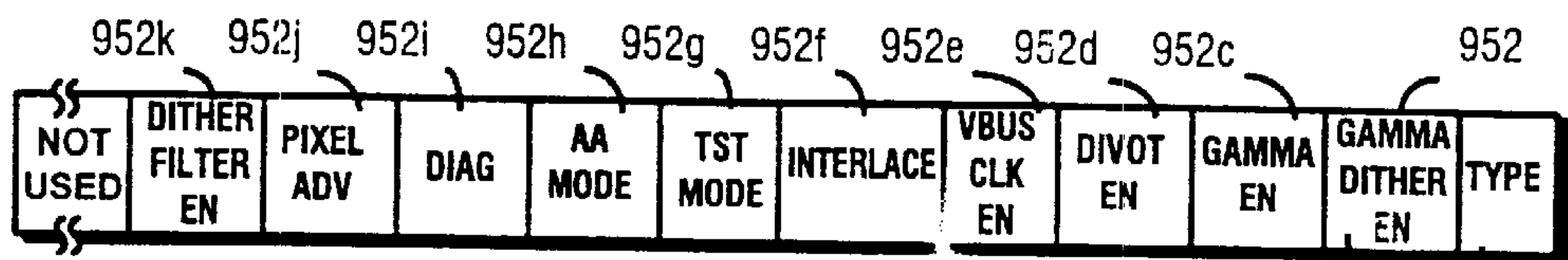
Fig. 35A VIDEO INTERFACE CONTROL REGISTER (R/W)
