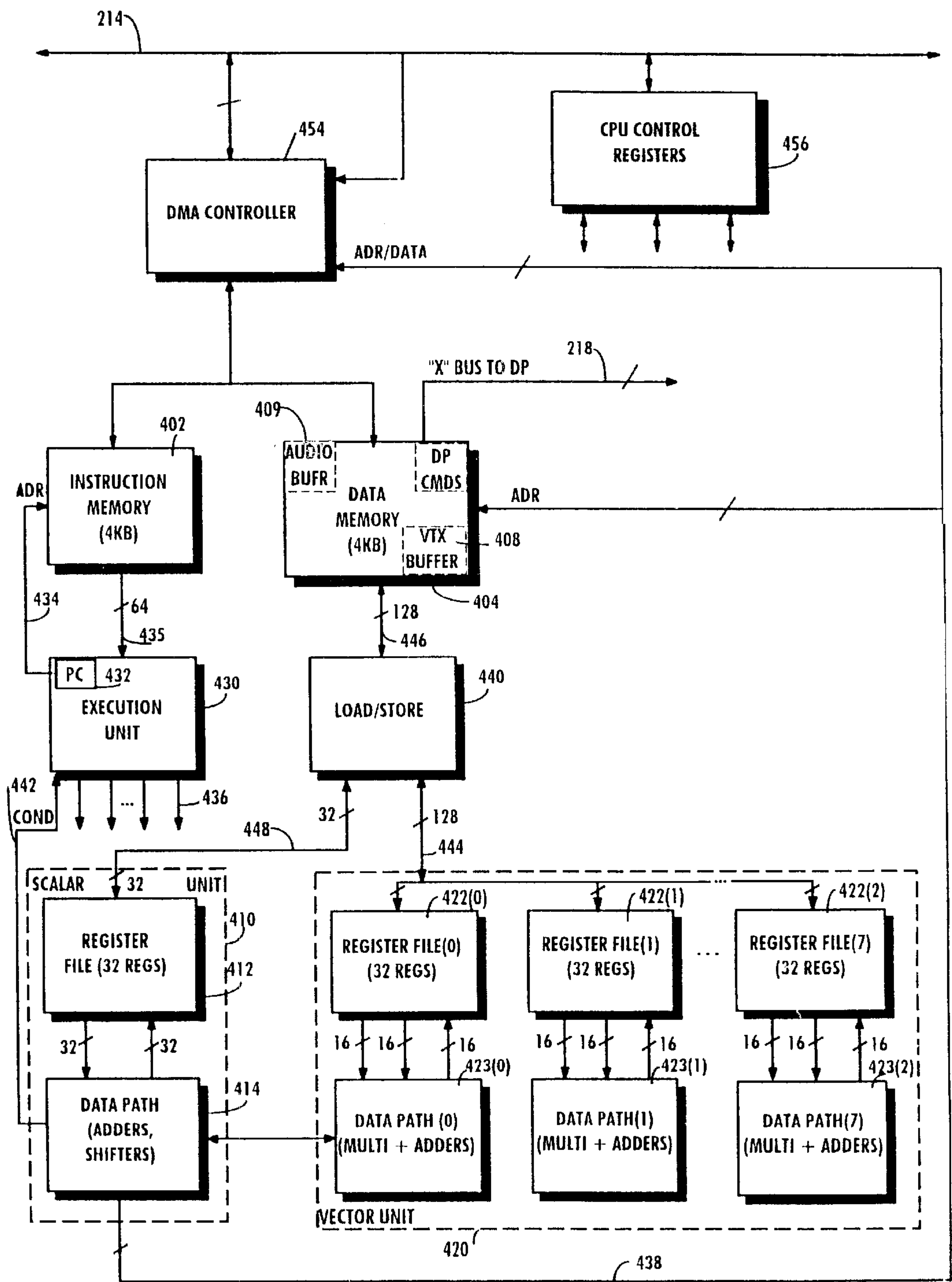
Fig. 7 SIGNAL PROCESSOR 400
