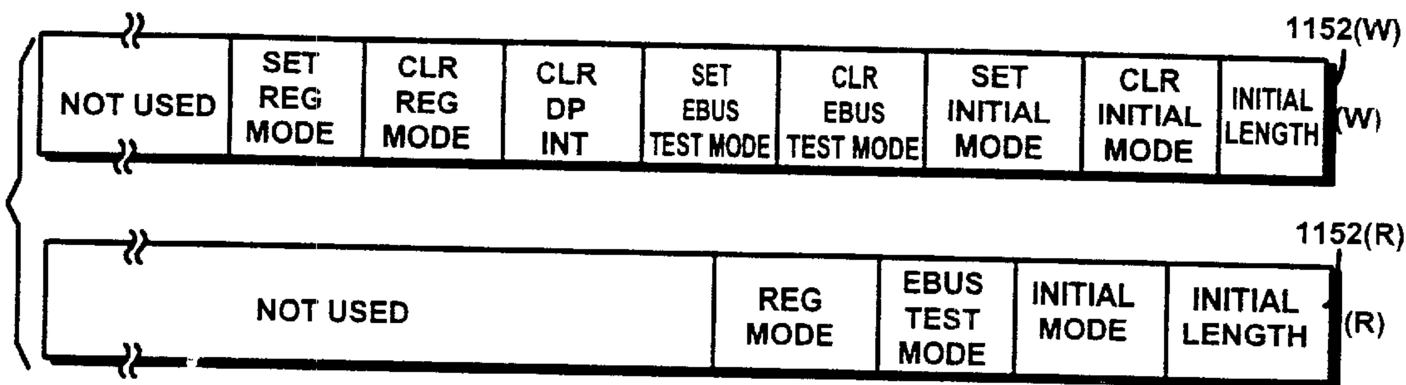
Fig. 39A CPU STATUS/CONTROL REGISTER (R/W)
