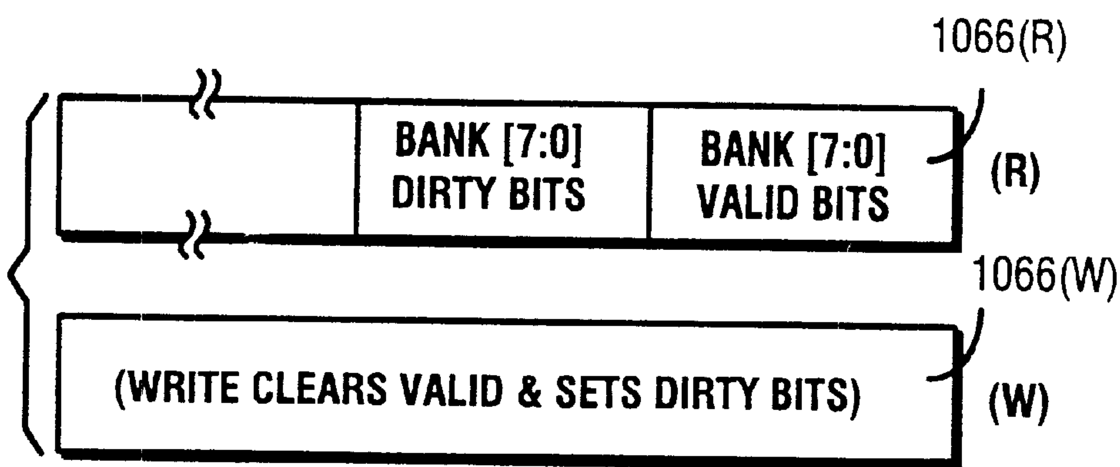
Fig. 37H BANK STATUS REG
