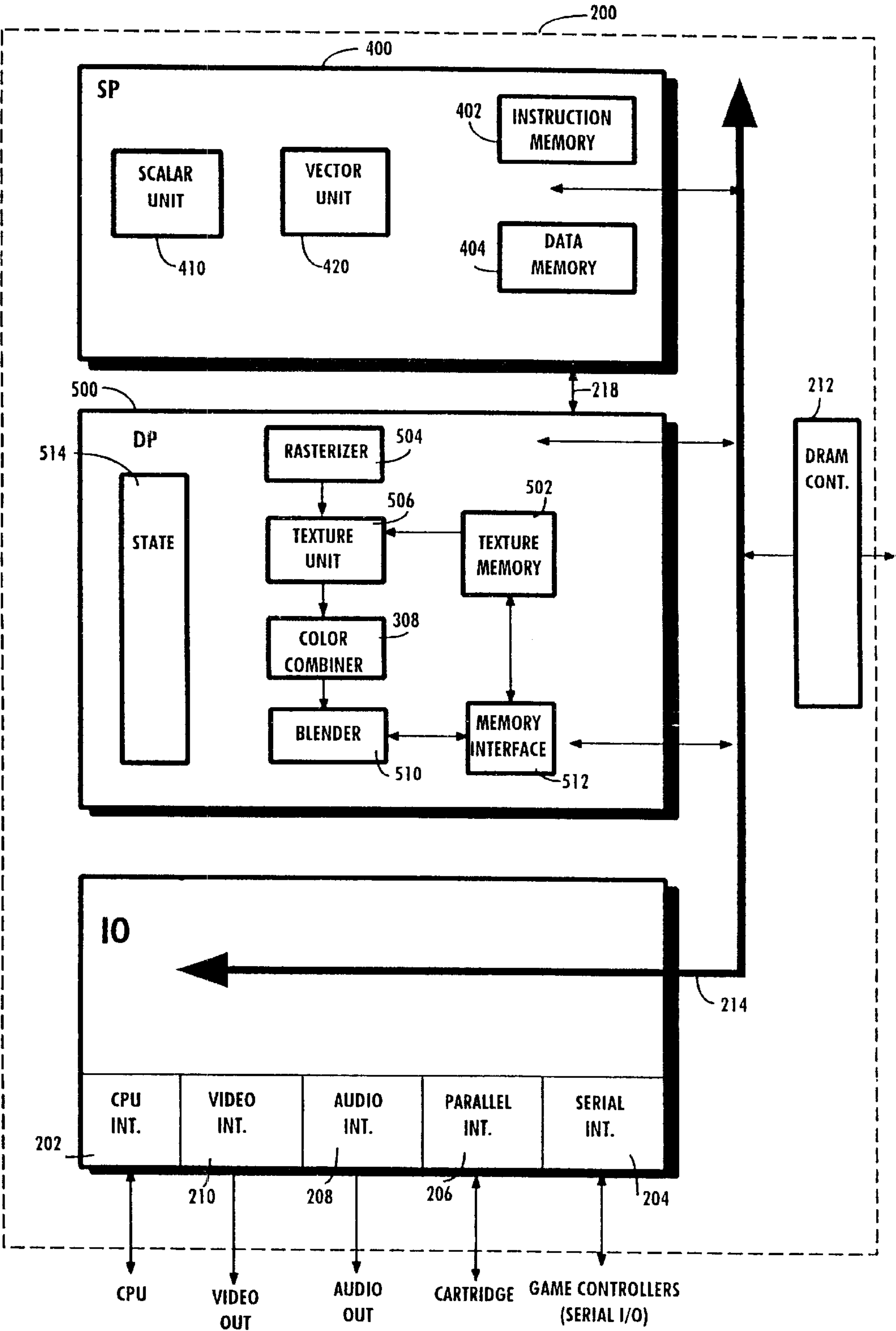
Fig. 6 COPROCESSOR
