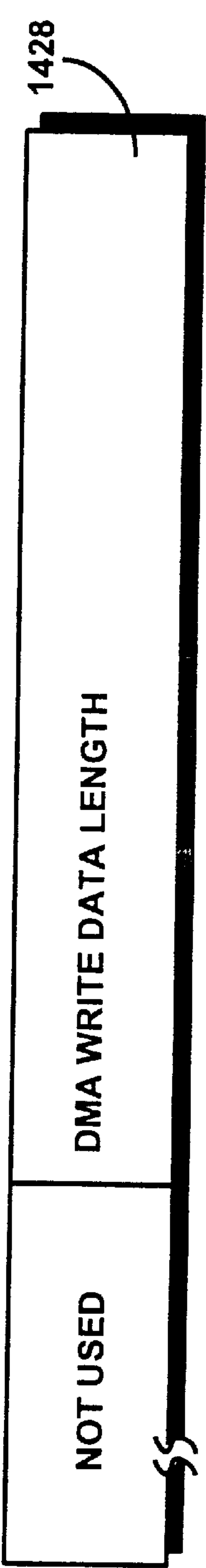
Fig. 45D PI WRITE LENGTH (R/W)
