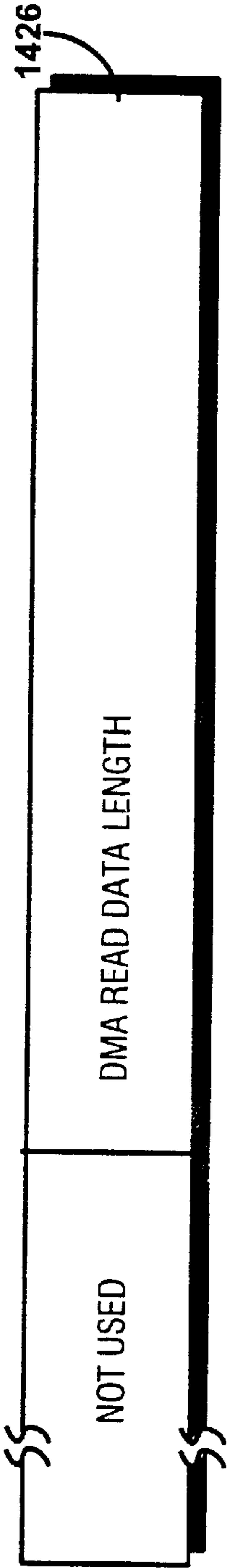
Fig. 45C PI DMA READ LENGTH (R/W)
