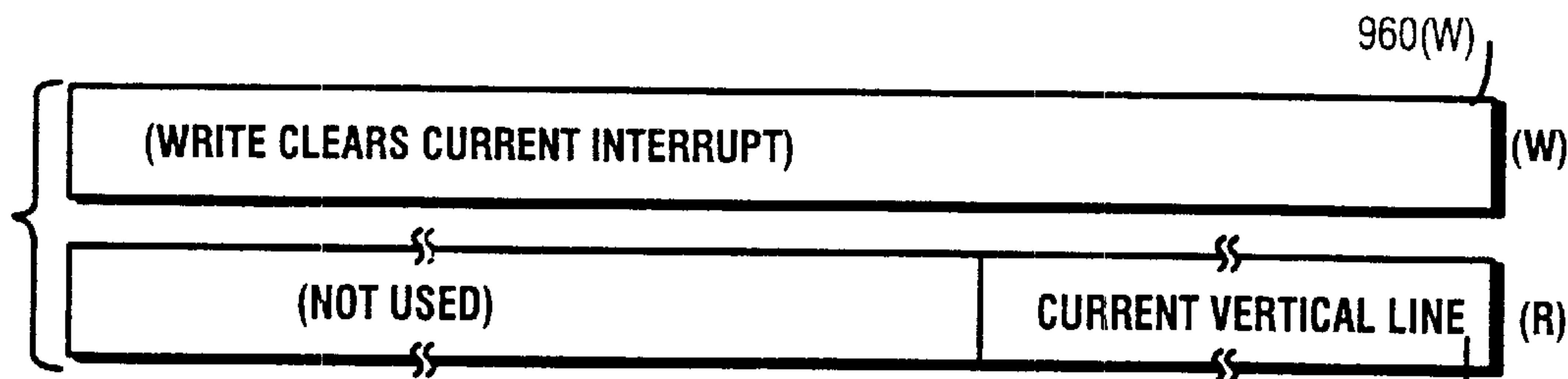
Fig. 35E VIDEO INTERFACE CURRENT LINE REGISTER
