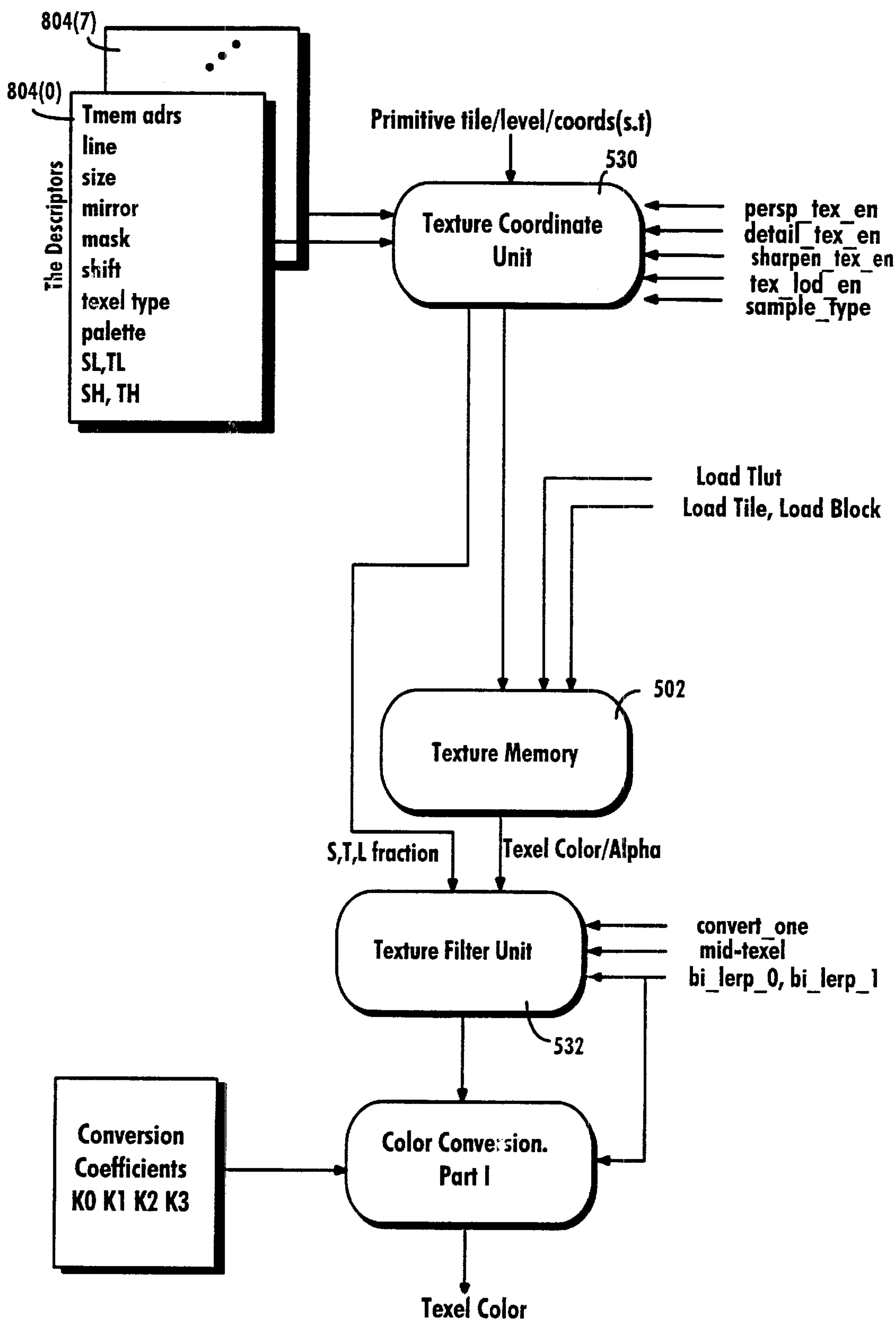
Fig. 23 TEXTURE UNIT EXAMPLE PROCESSES
