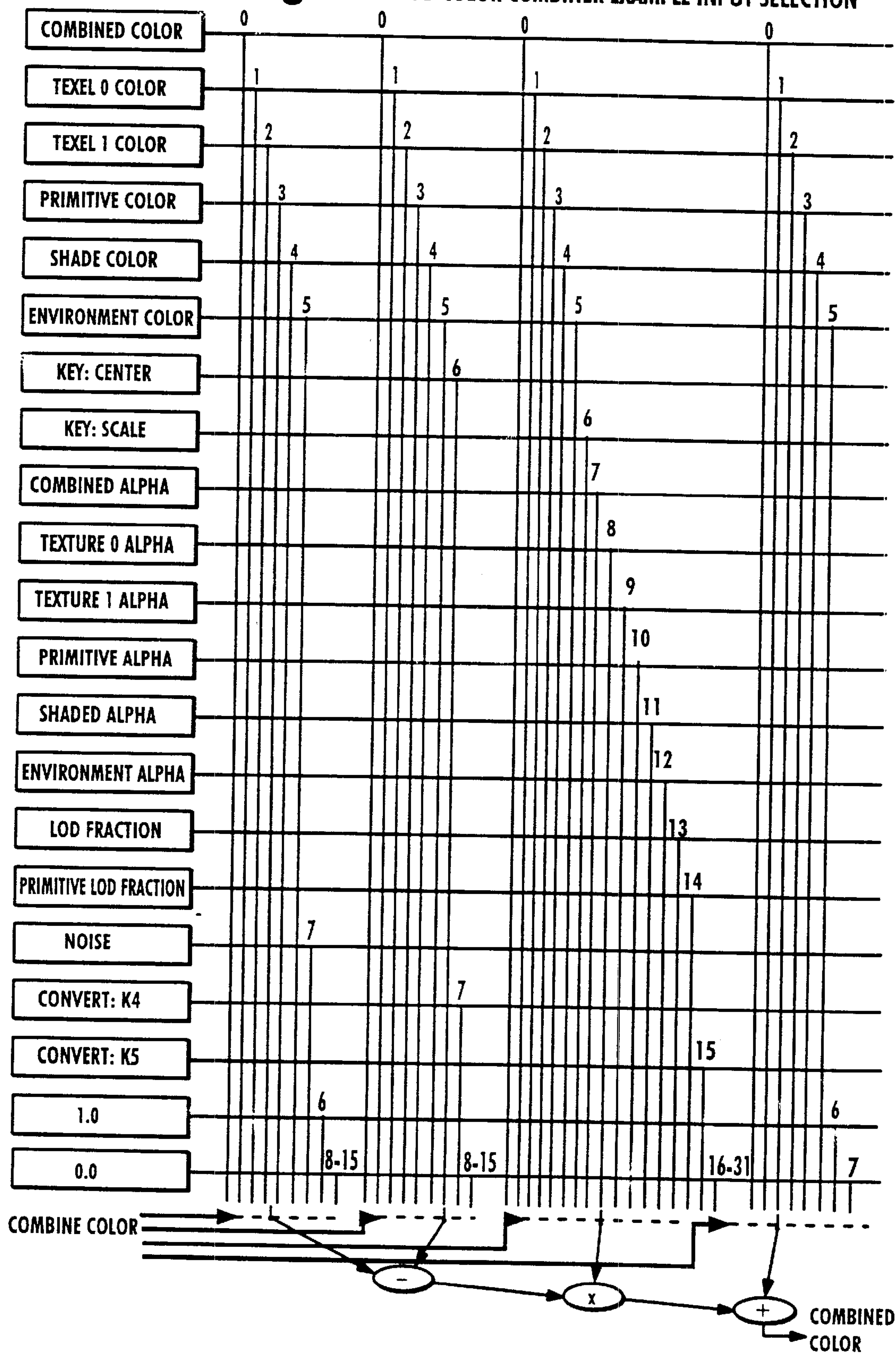
Fig. 27 RGB COLOR COMBINER EXAMPLE INPUT SELECTION
