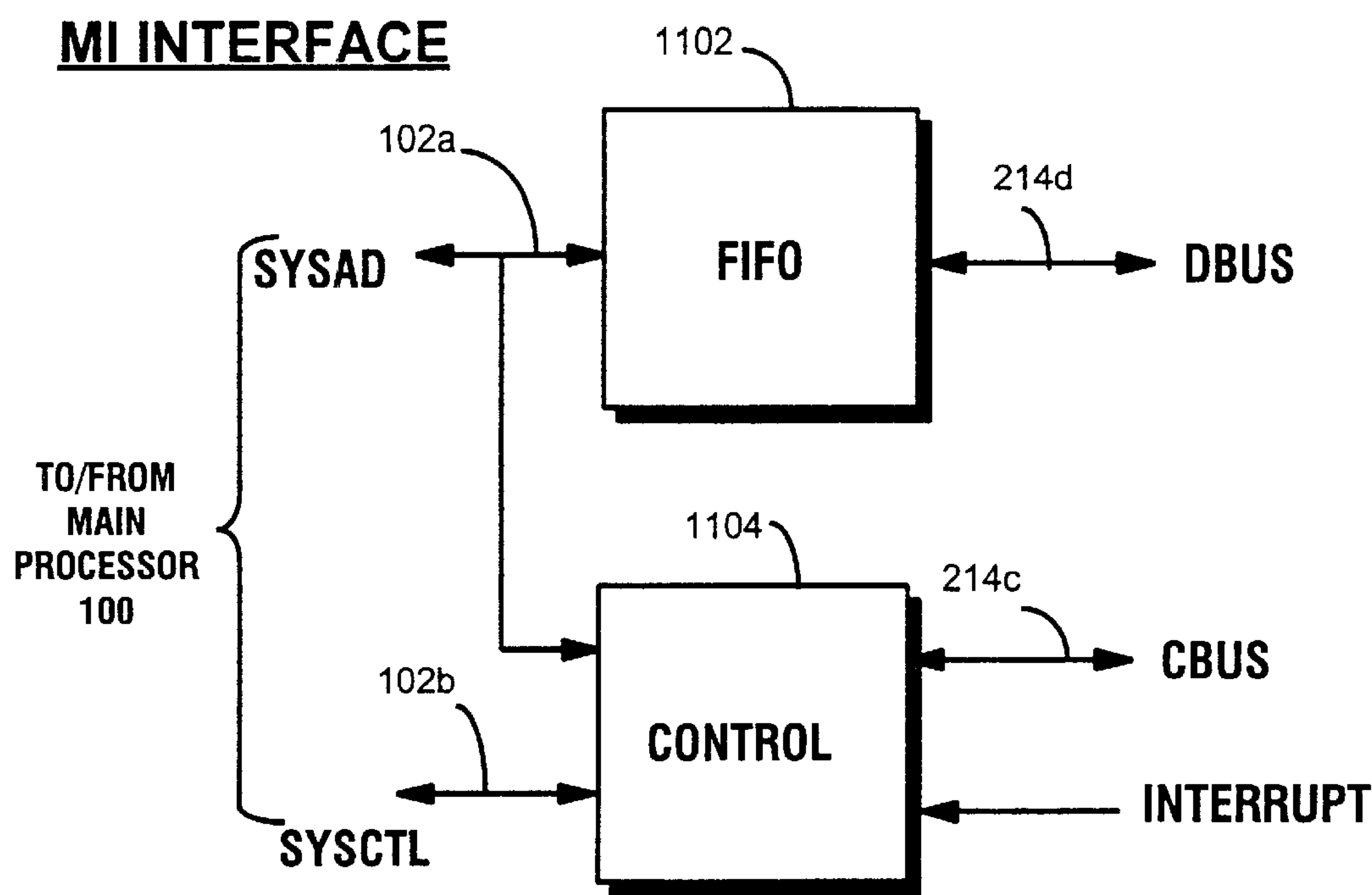
Fig. 38 EXAMPLE CPU INTERFACE
