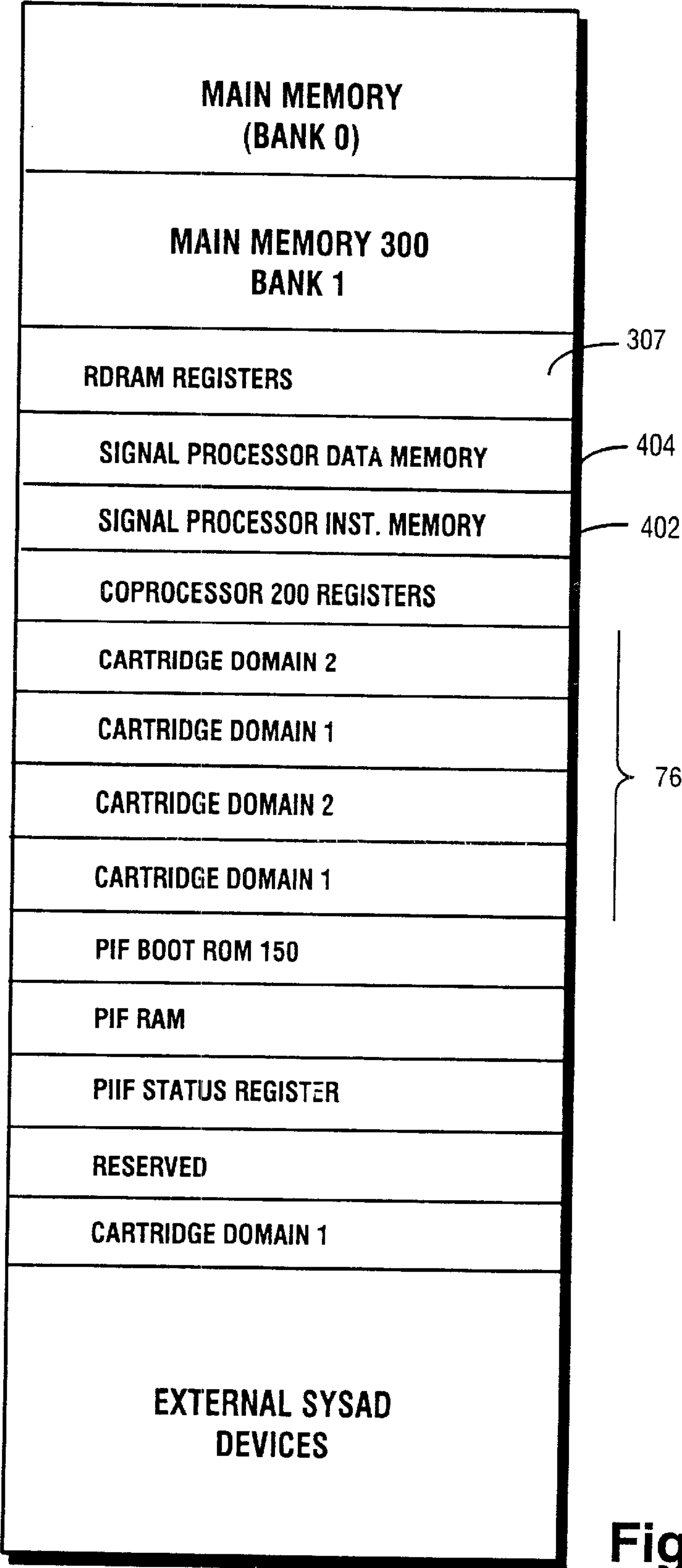
EXAMPLE CPU MEMORY MAP
