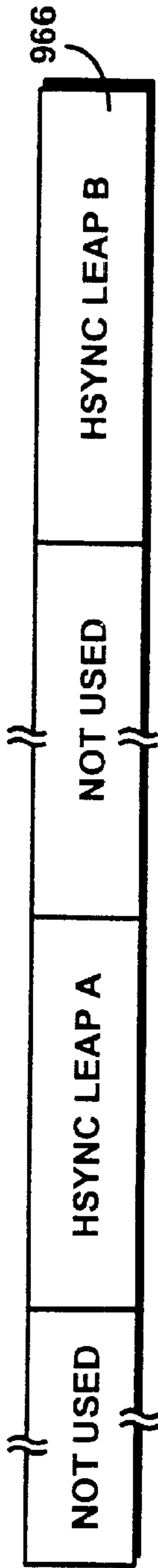
Fig. 35I VIDEO INTERFACE HSYNC LEAP REGISTER (R/W)
