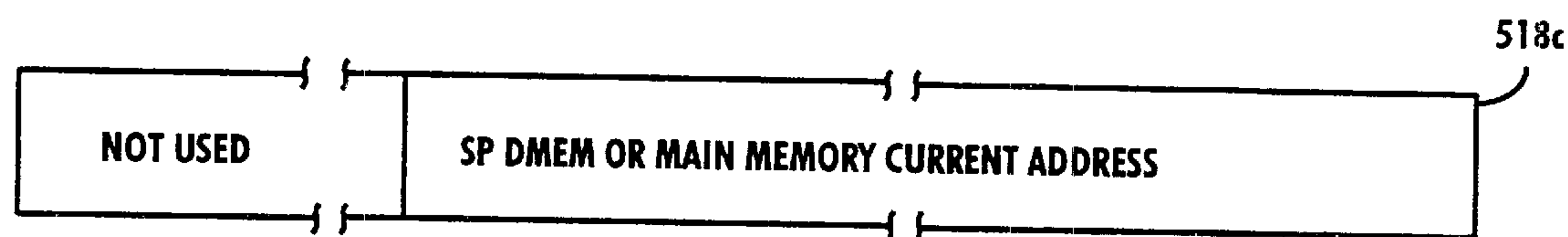
Fig. 21C DP CMD DMA CURRENT ADDRESS REGISTER (R/W)
