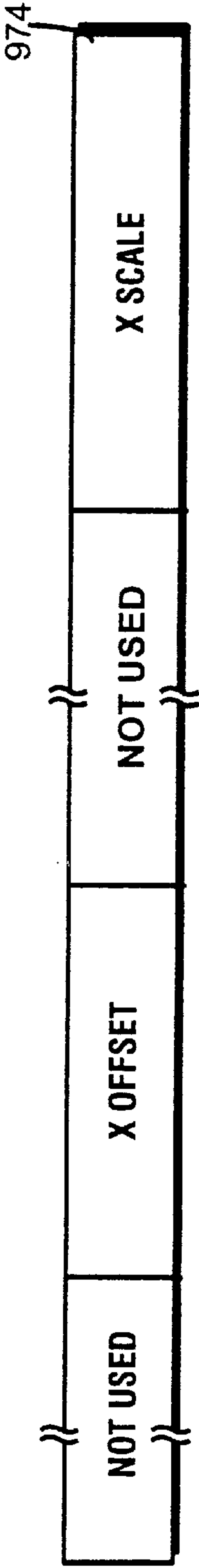
Fig. 35M VIDEO INTERFACE X SCALE REGISTER (R/W)
