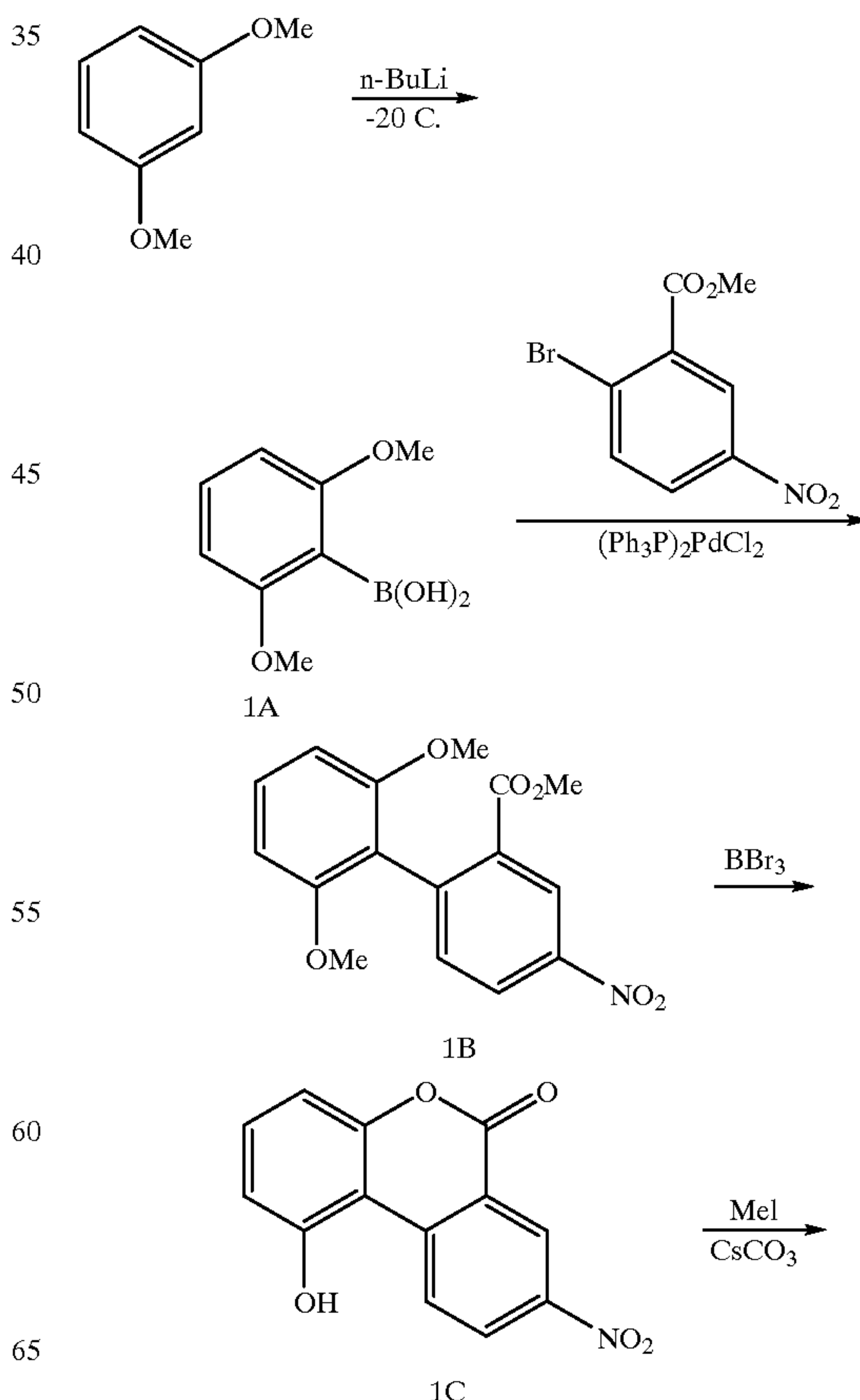
Scheme II
