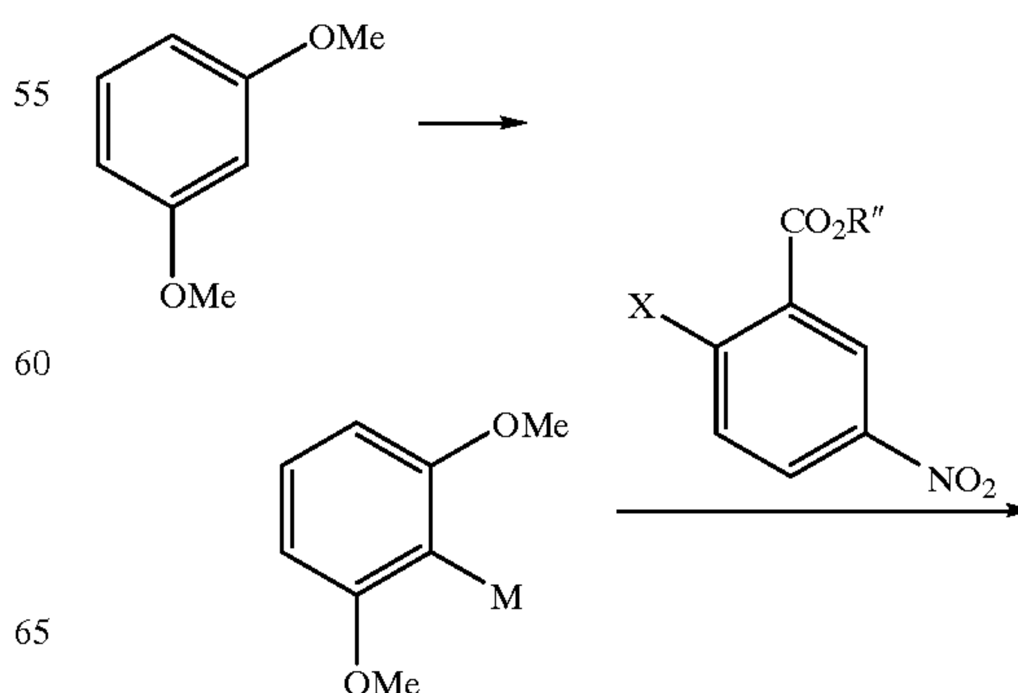
Scheme I
