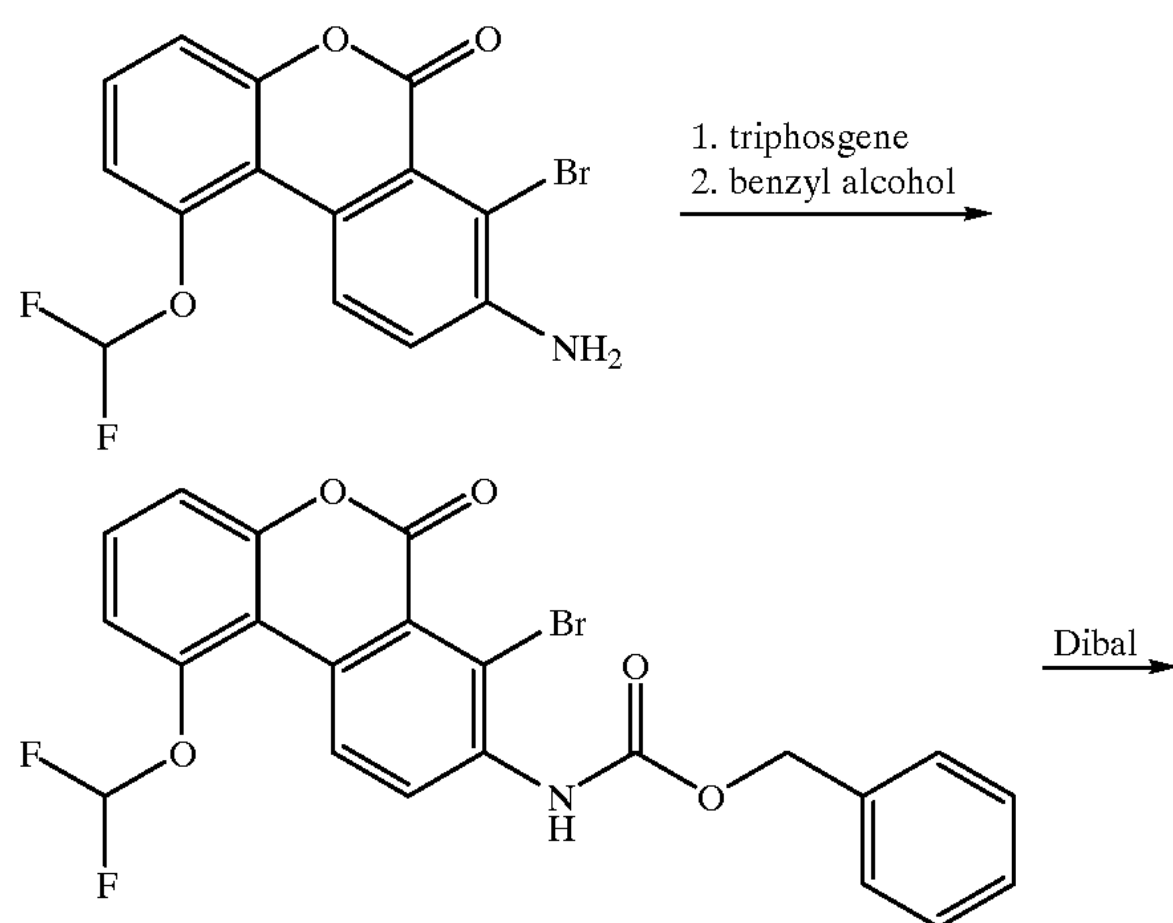
Scheme IV
