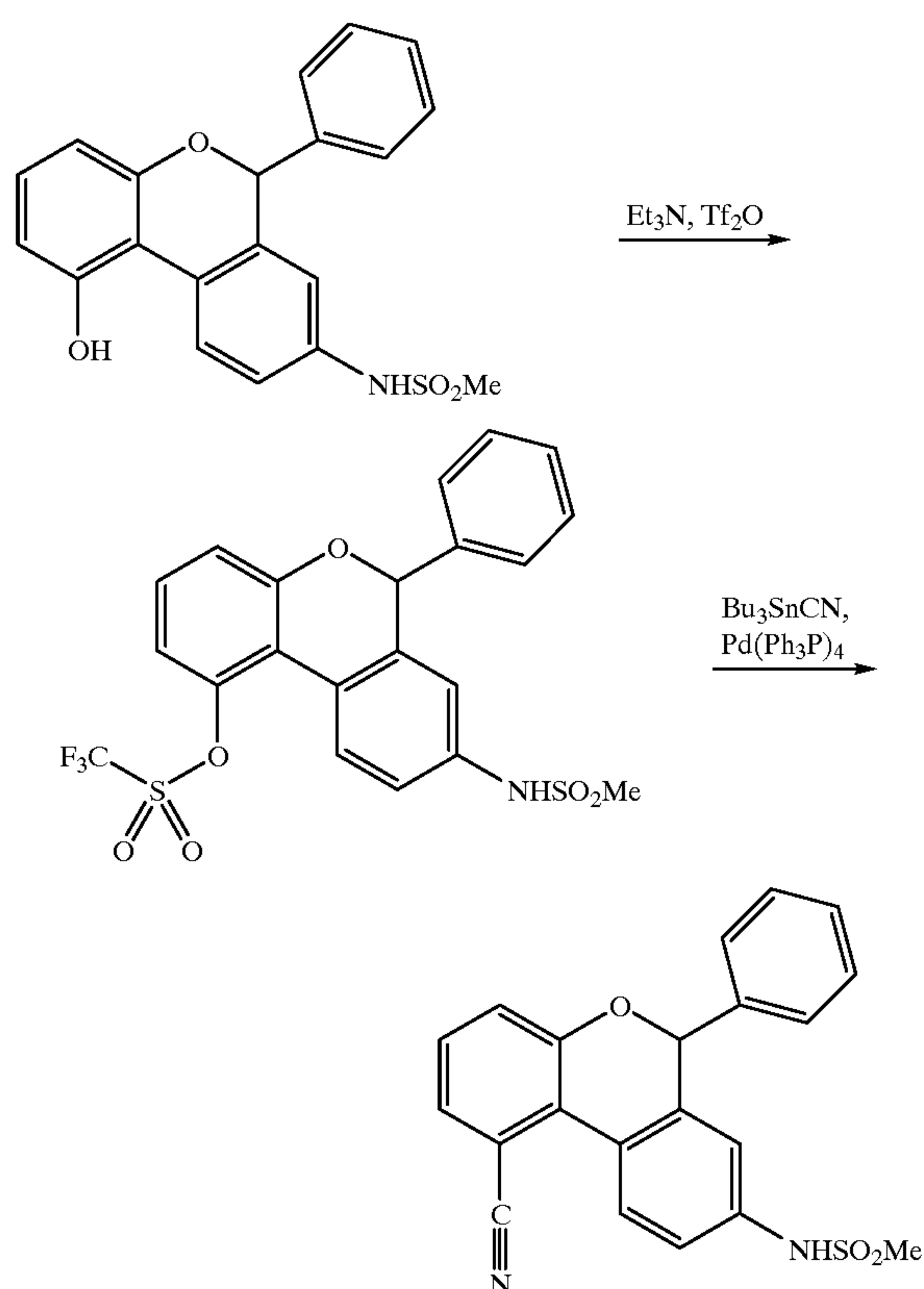
Scheme IX
