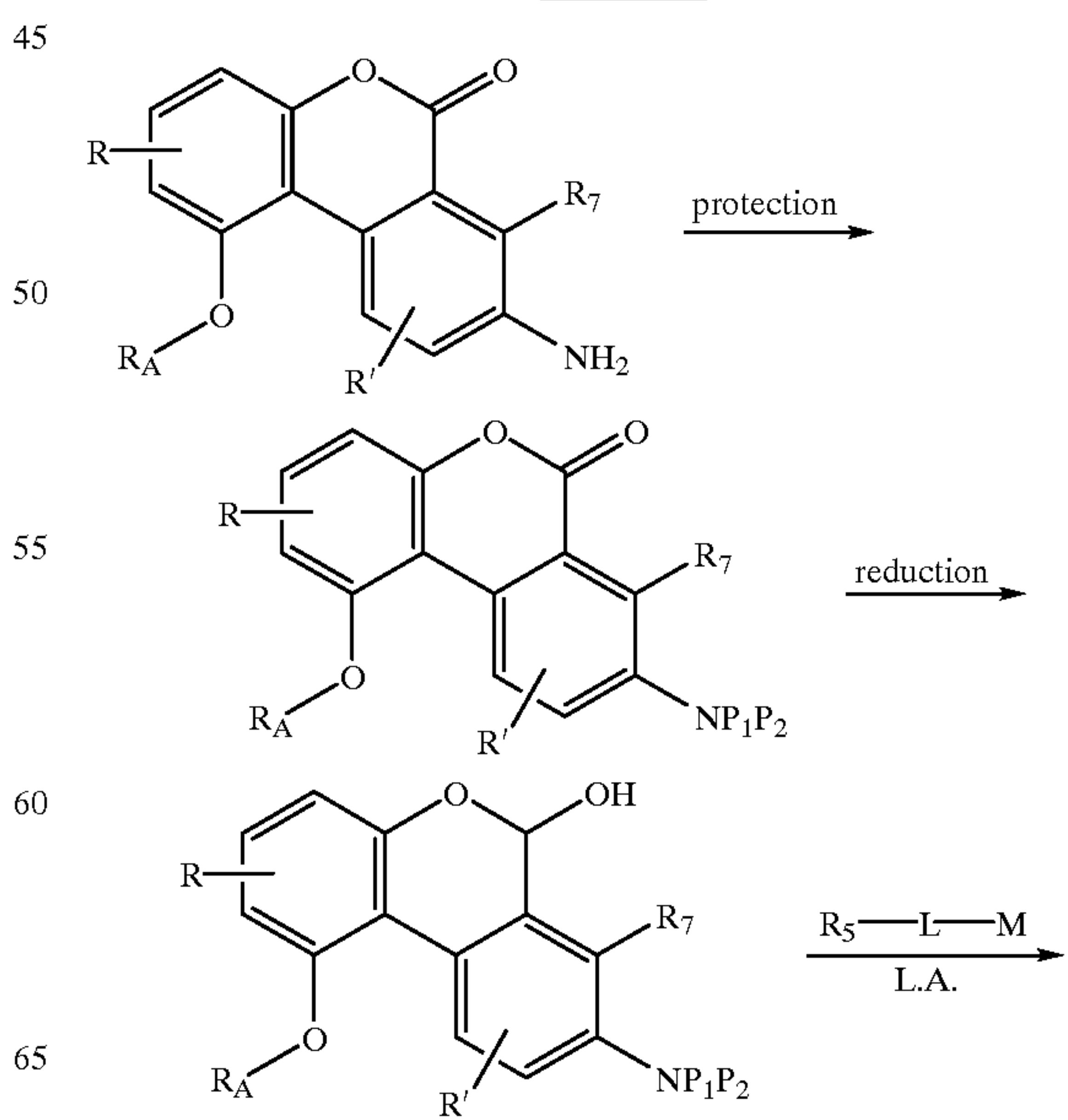
Scheme III
