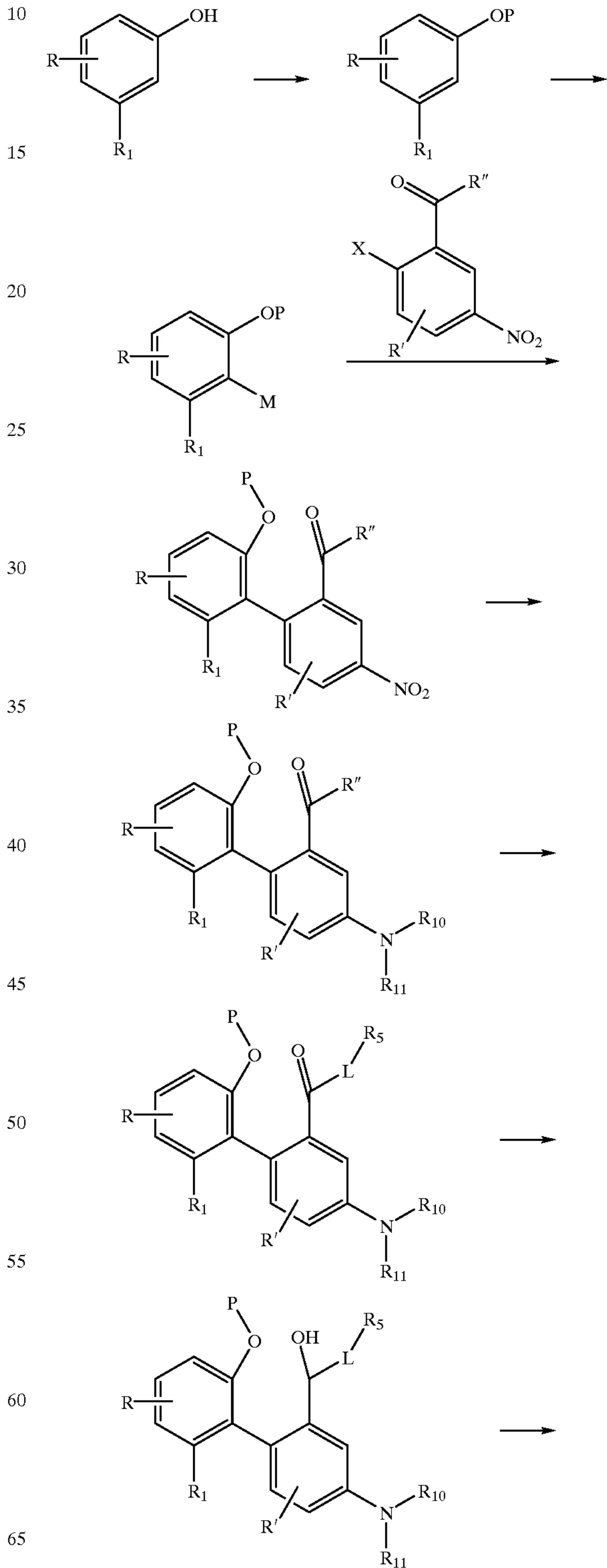
Scheme VII
