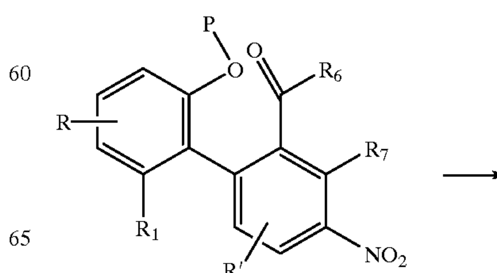
Scheme V
