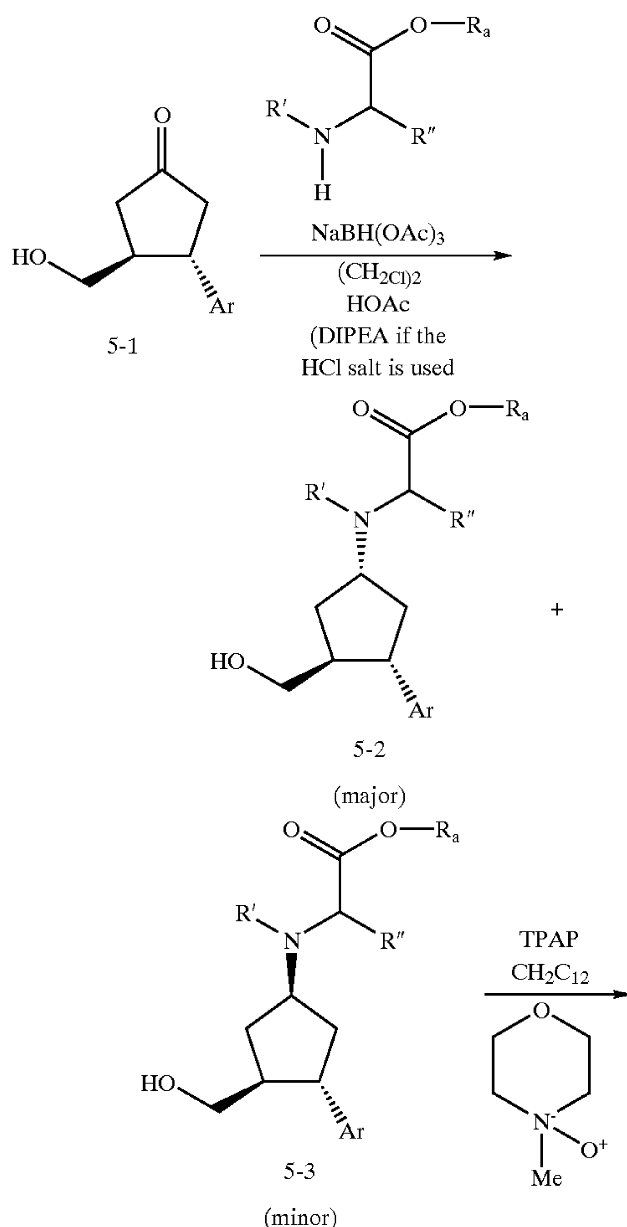
SCHEME 5
