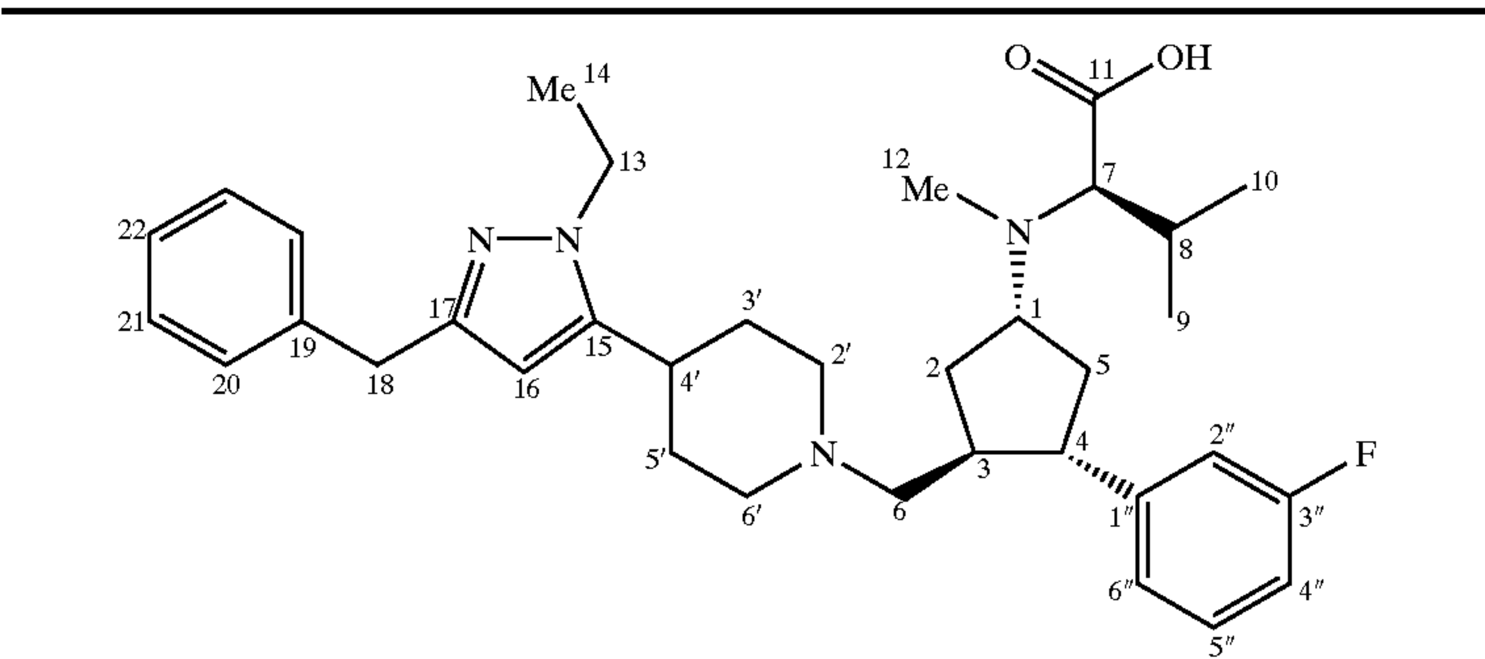
Carbon-13 and Proton Assignments
