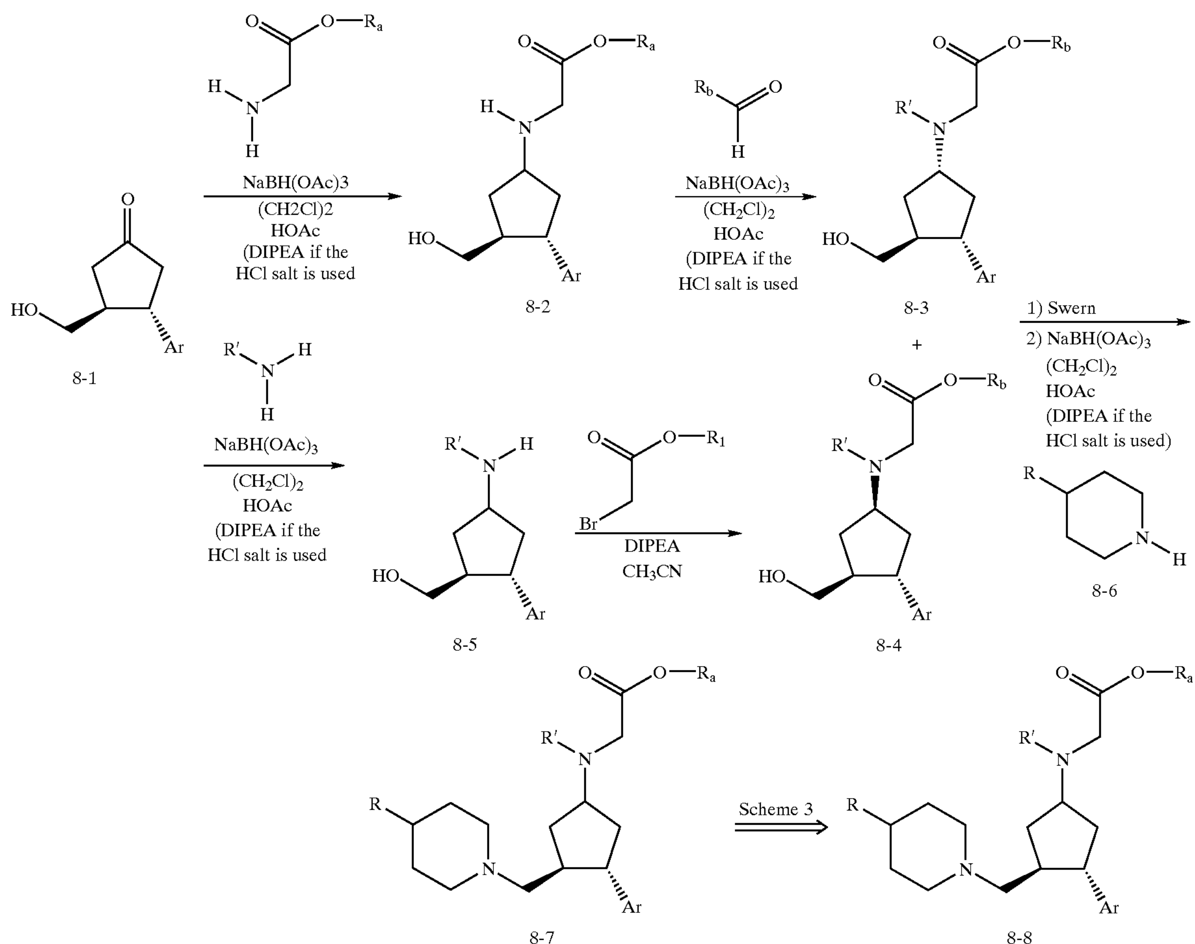
SCHEME 8
