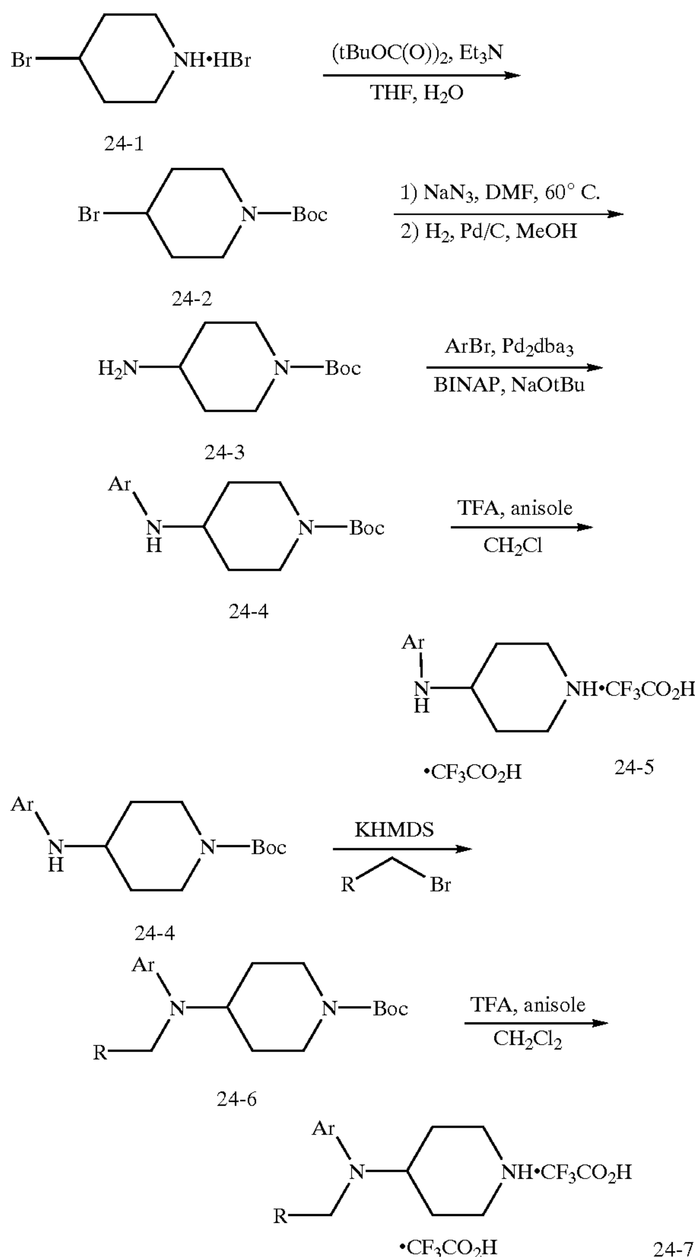
SCHEME 24
