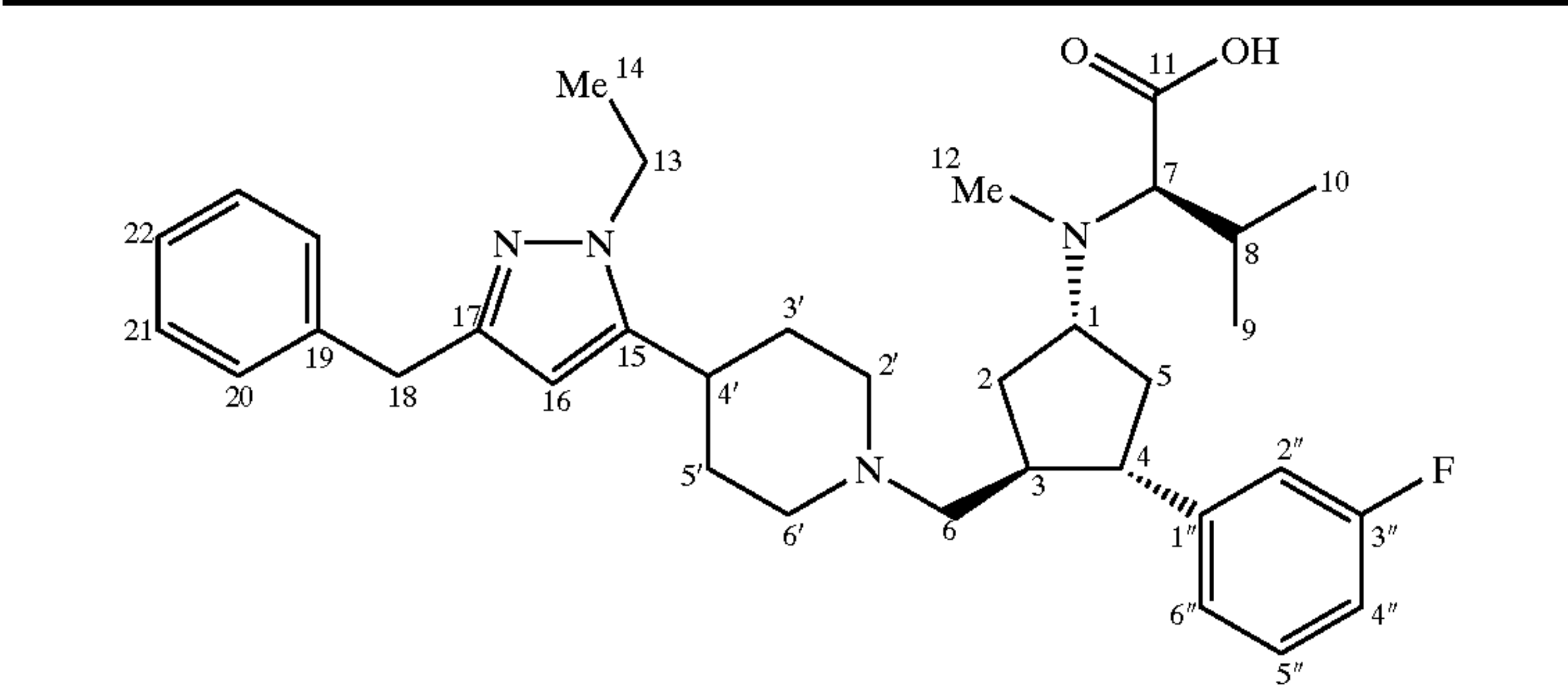
Carbon-13 and Proton Assignments
