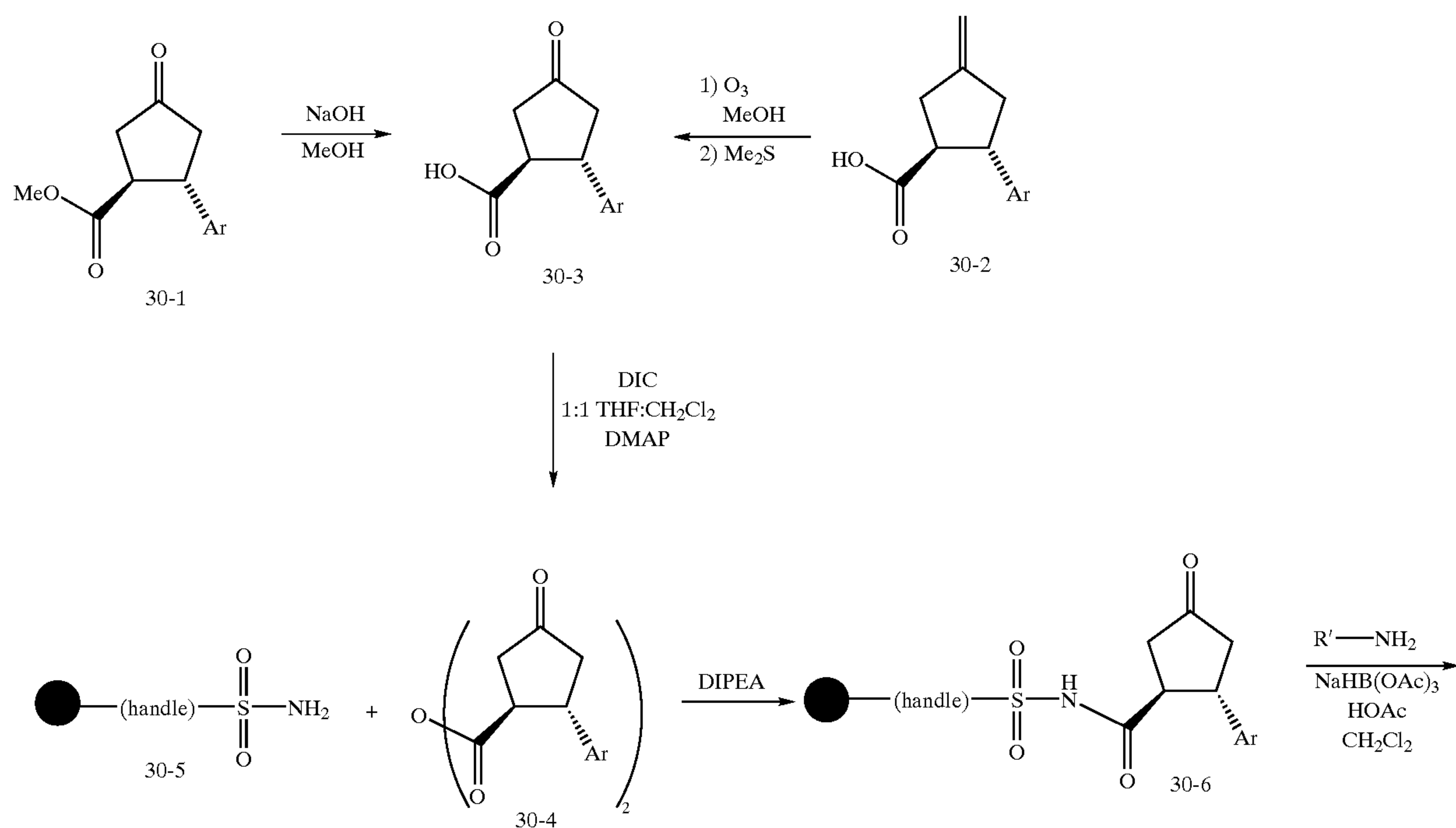
SCHEME 30
