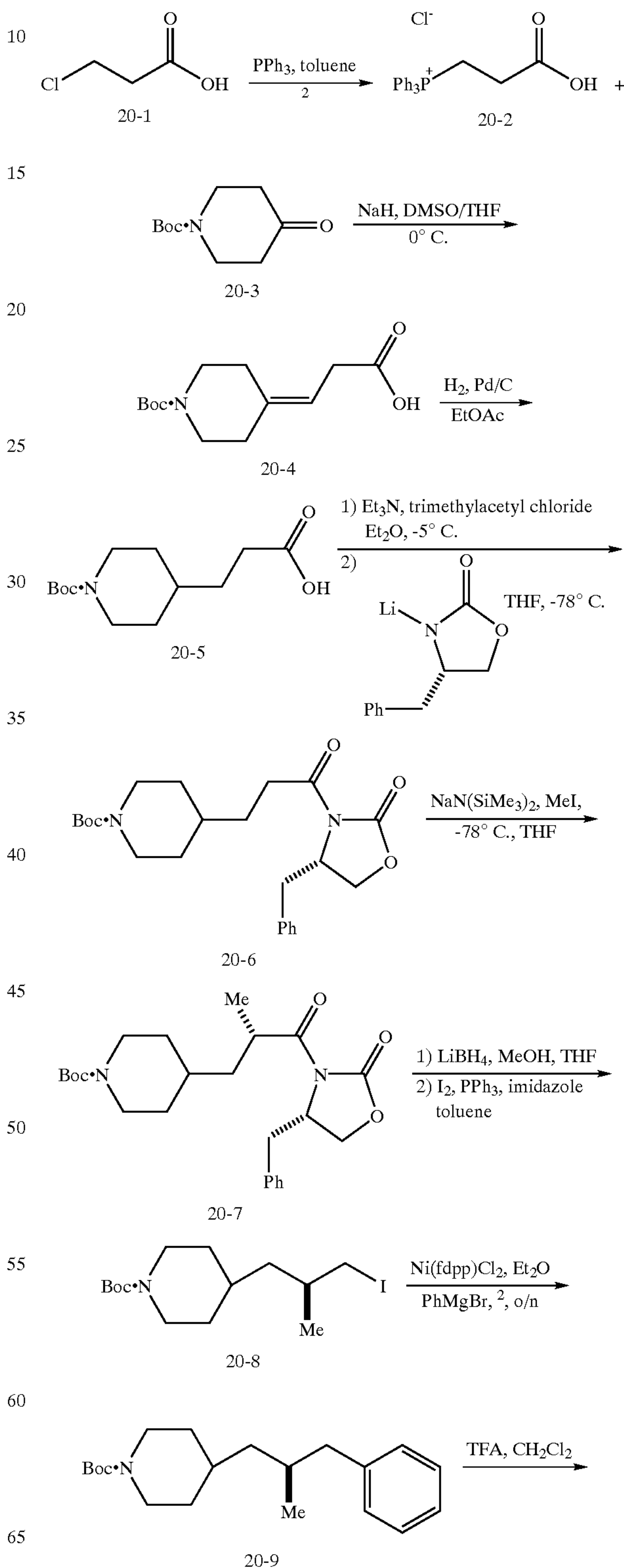
SCHEME 20
