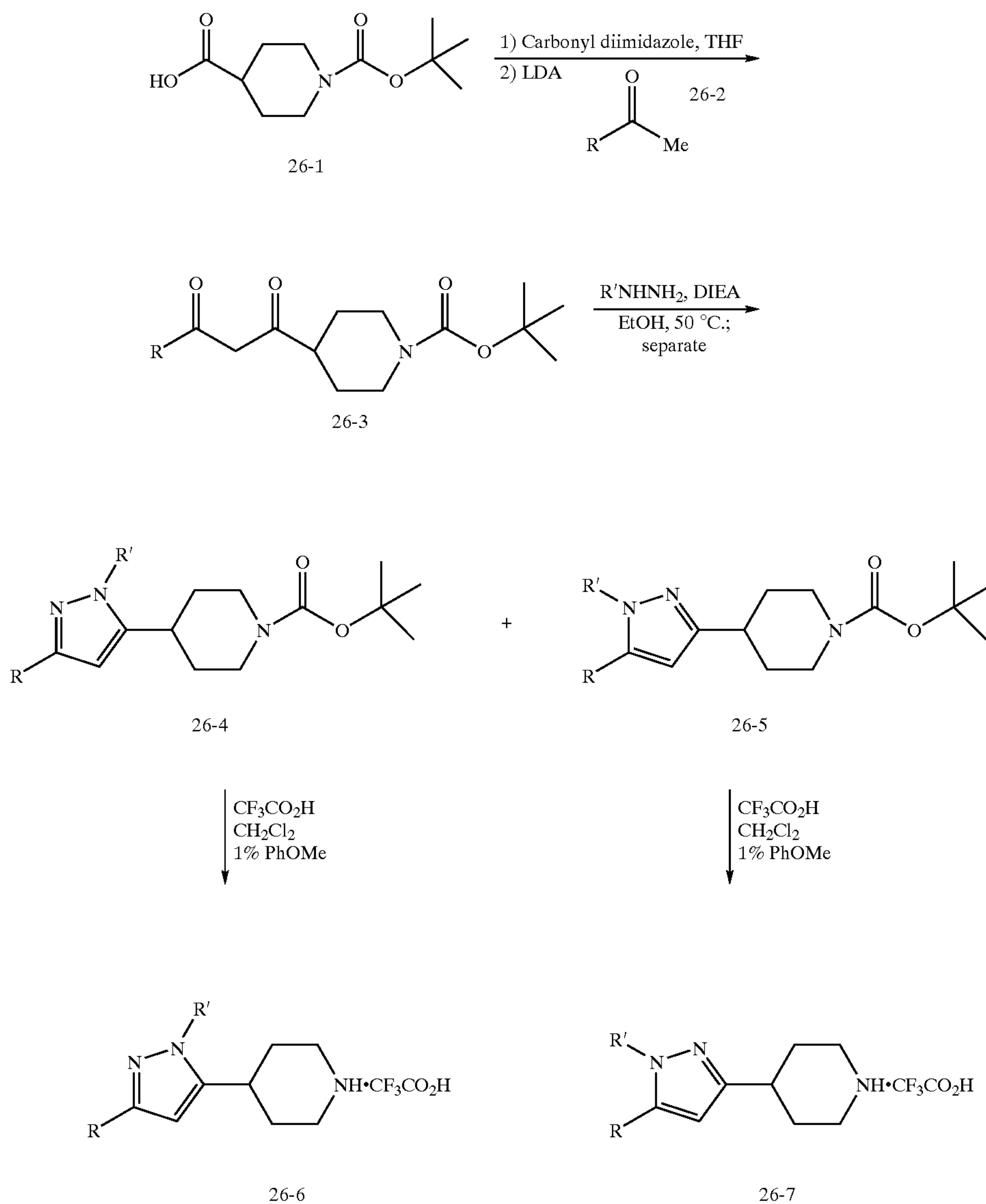
SCHEME 26
