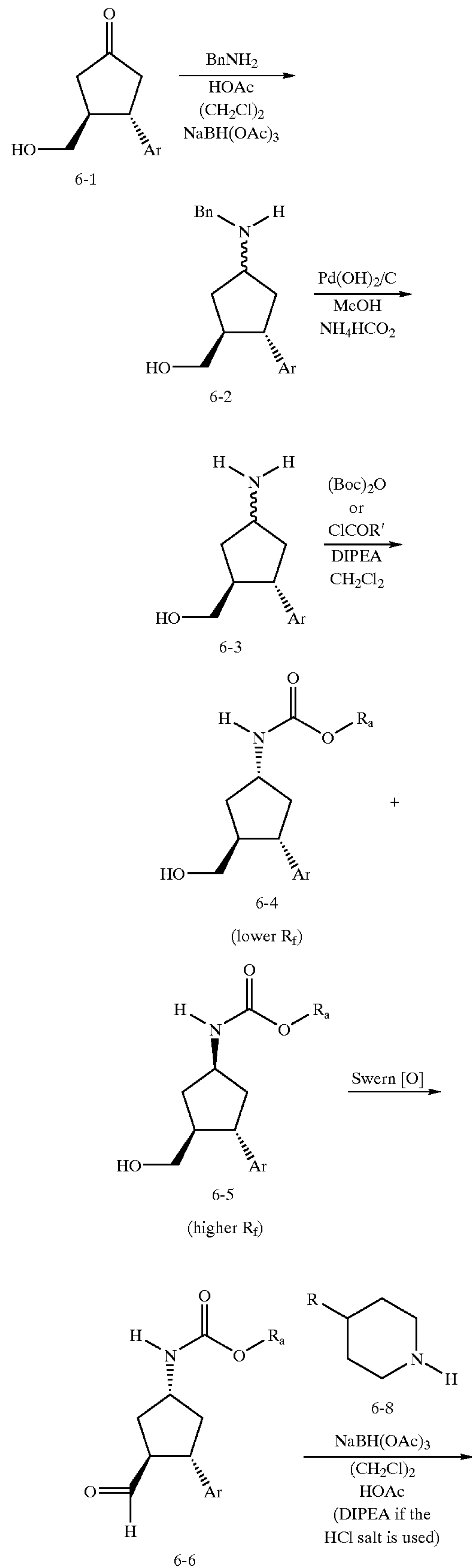
SCHEME 6
