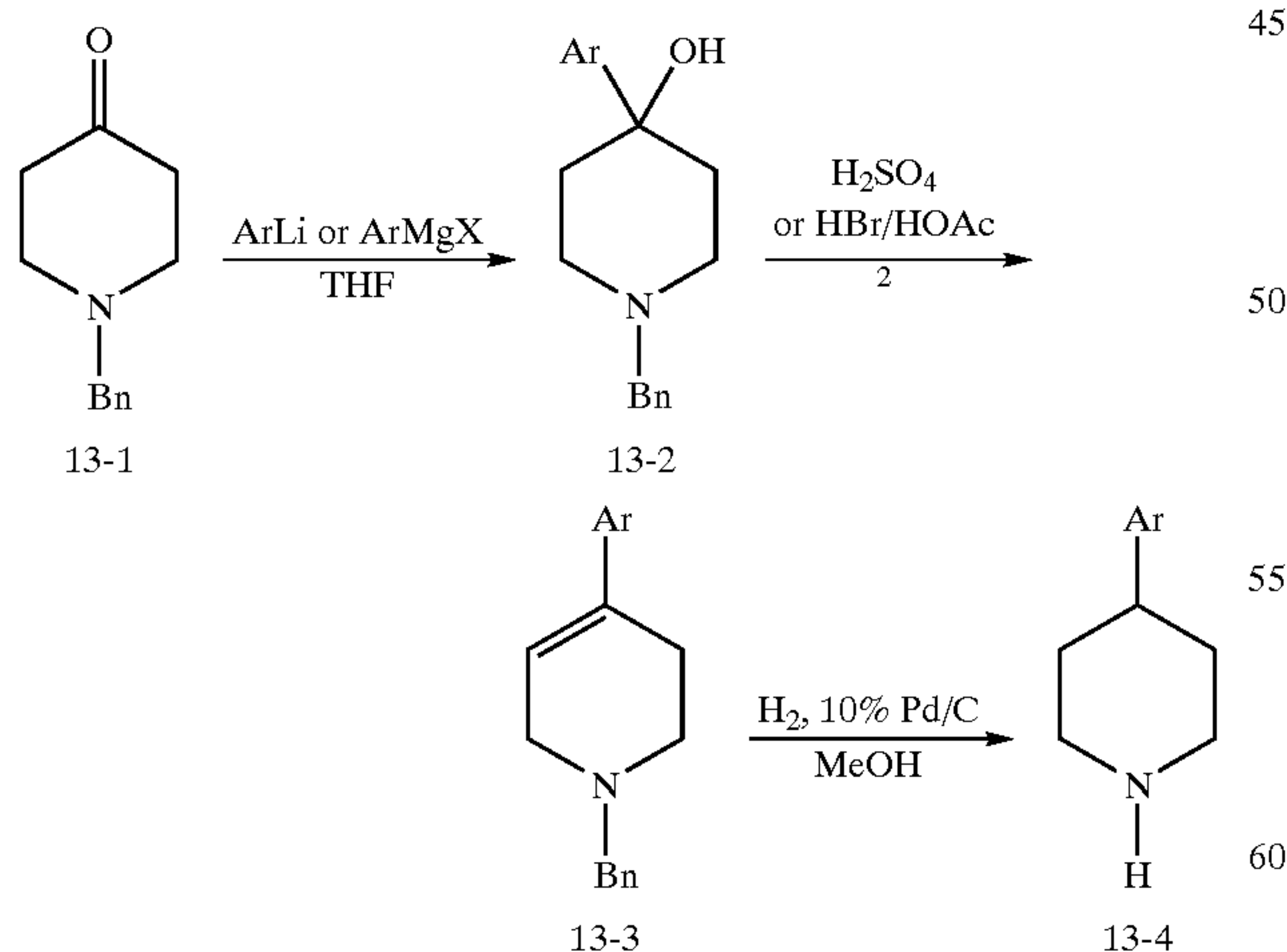
SCHEME 13
