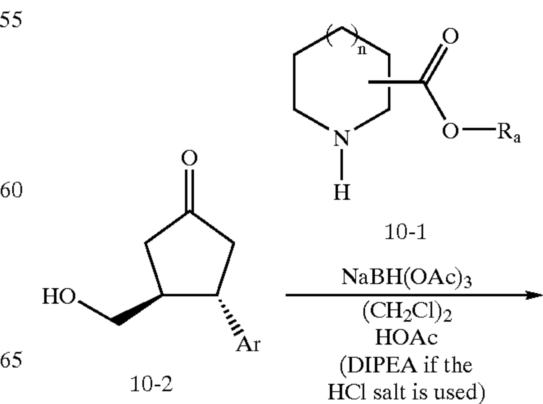
SCHEME 10
