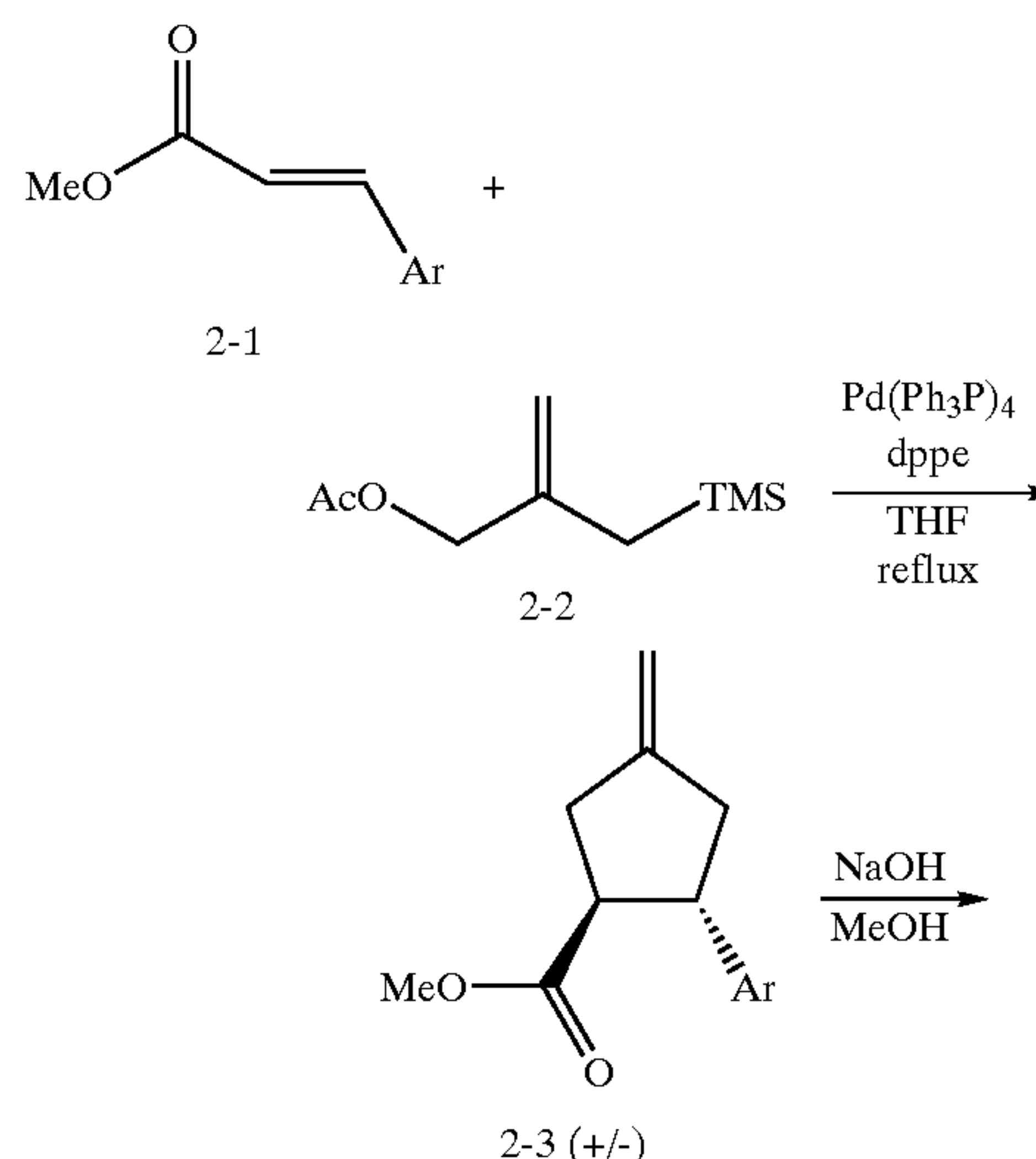
SCHEME 2
