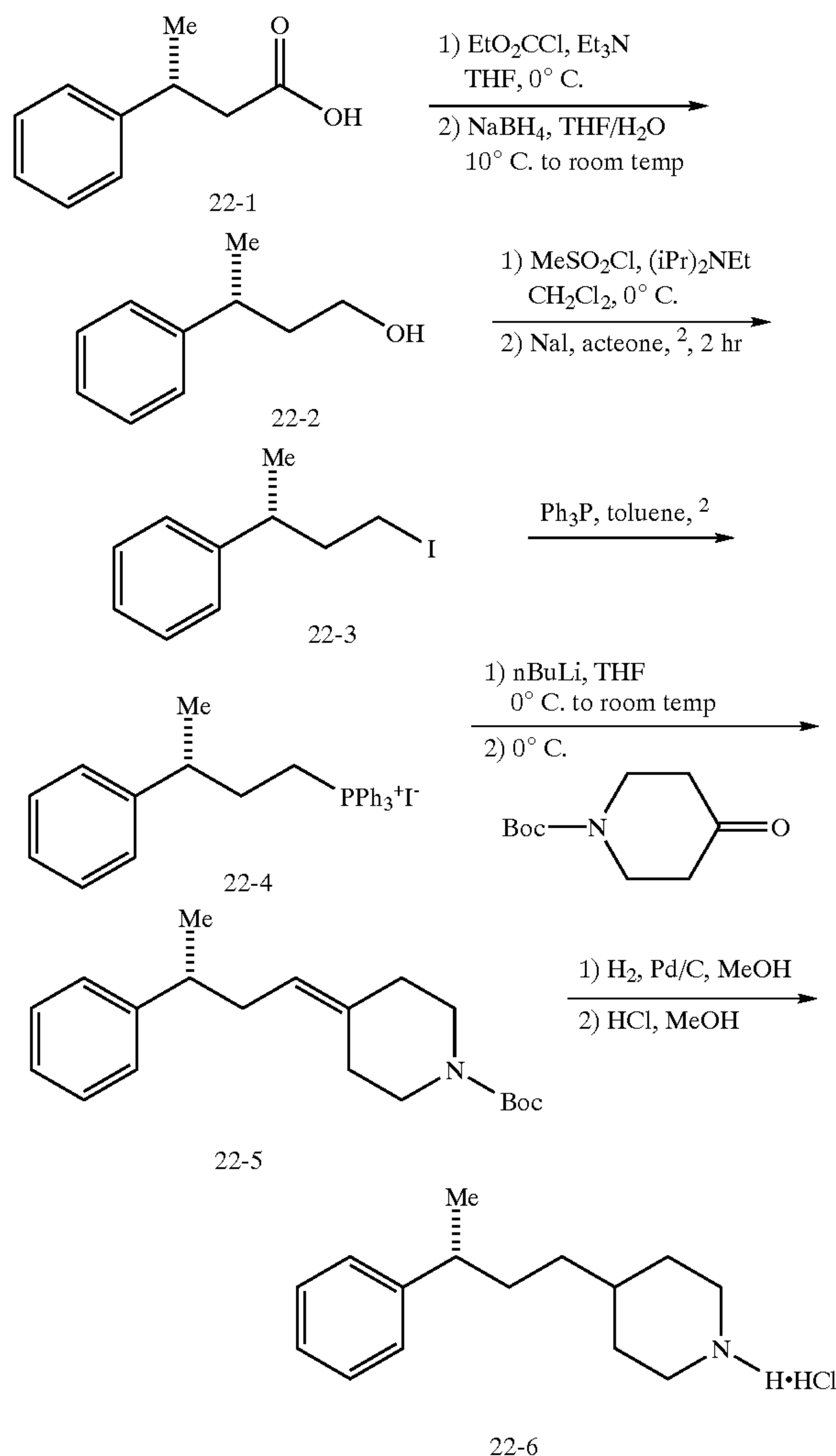
SCHEME 22
