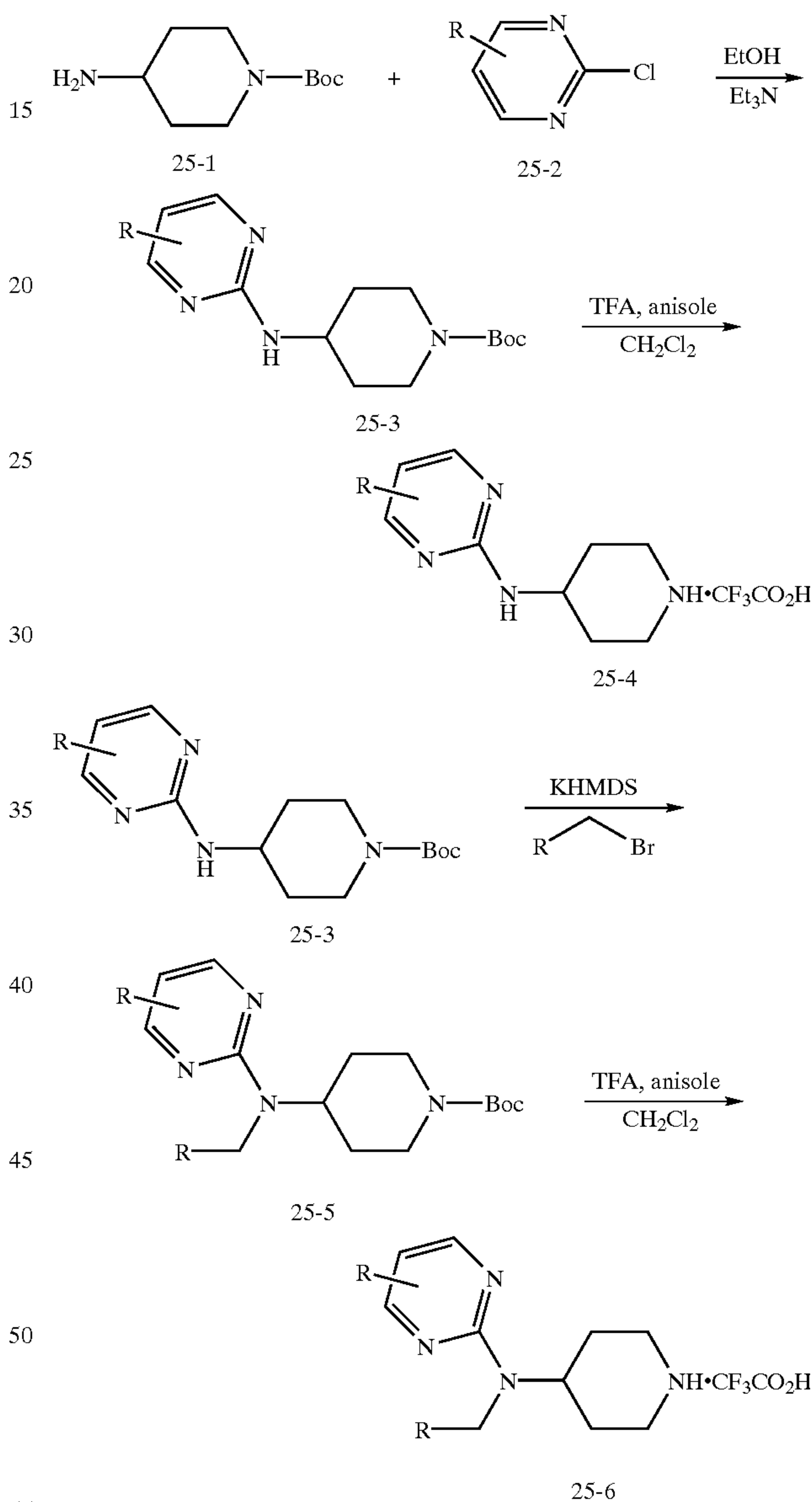
SCHEME 25
