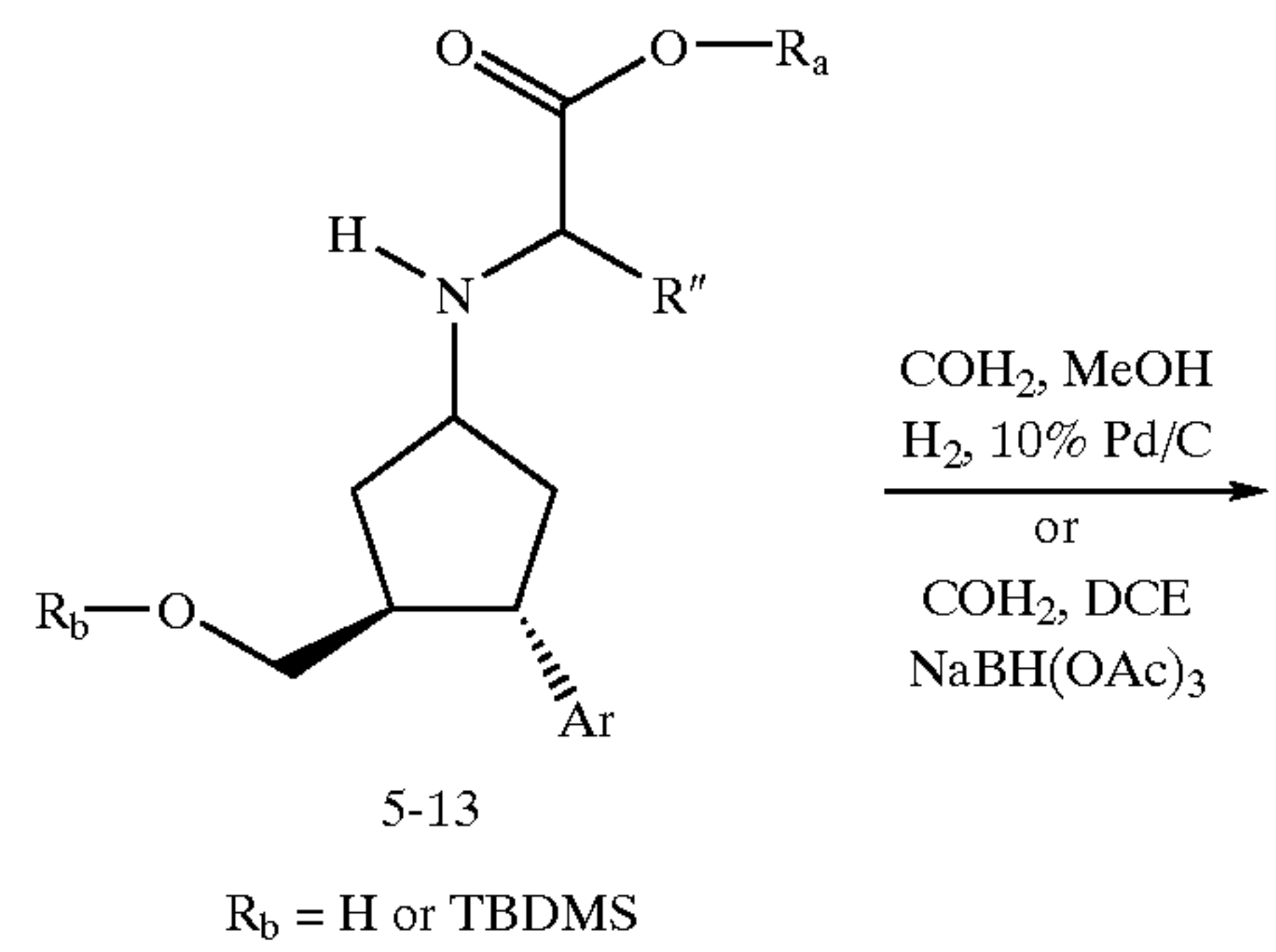
SCHEME 5B
