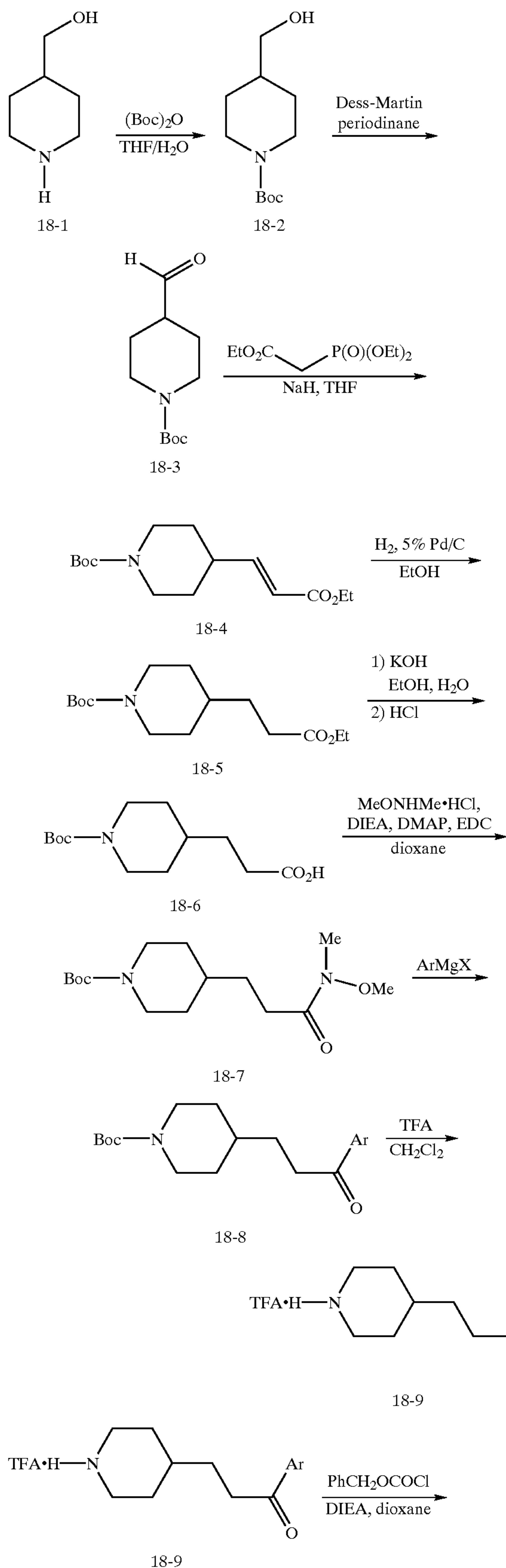
SCHEME 18
