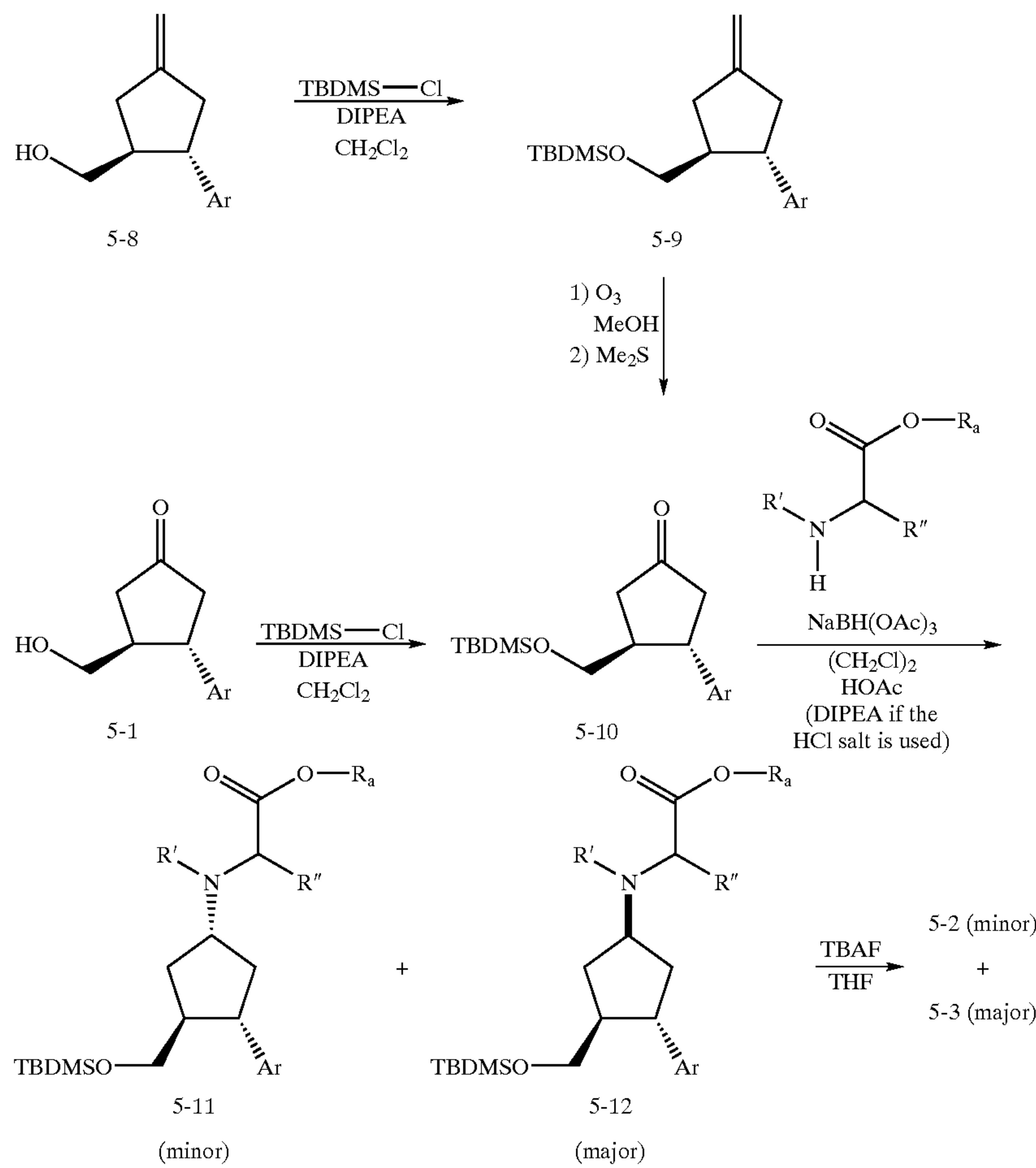
SCHEME 5A
