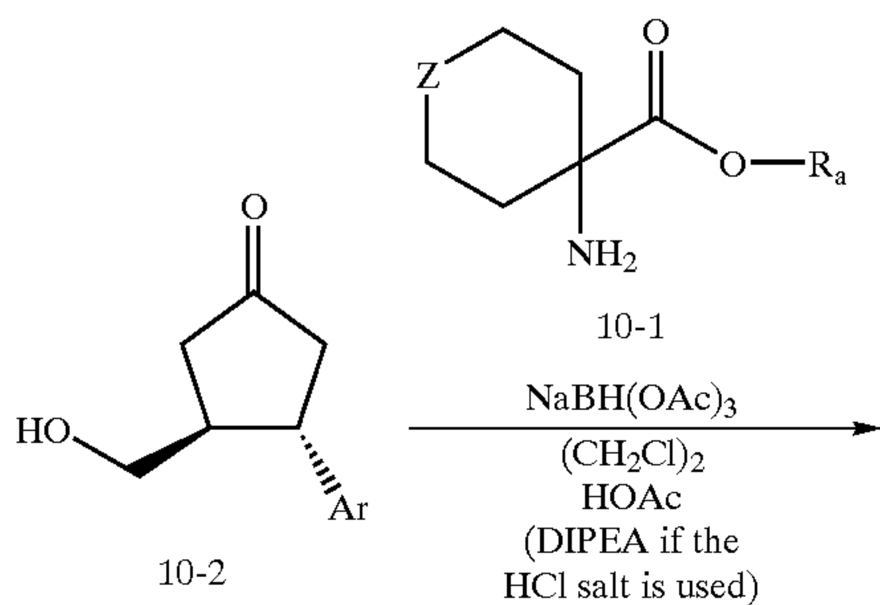
SCHEME 11
