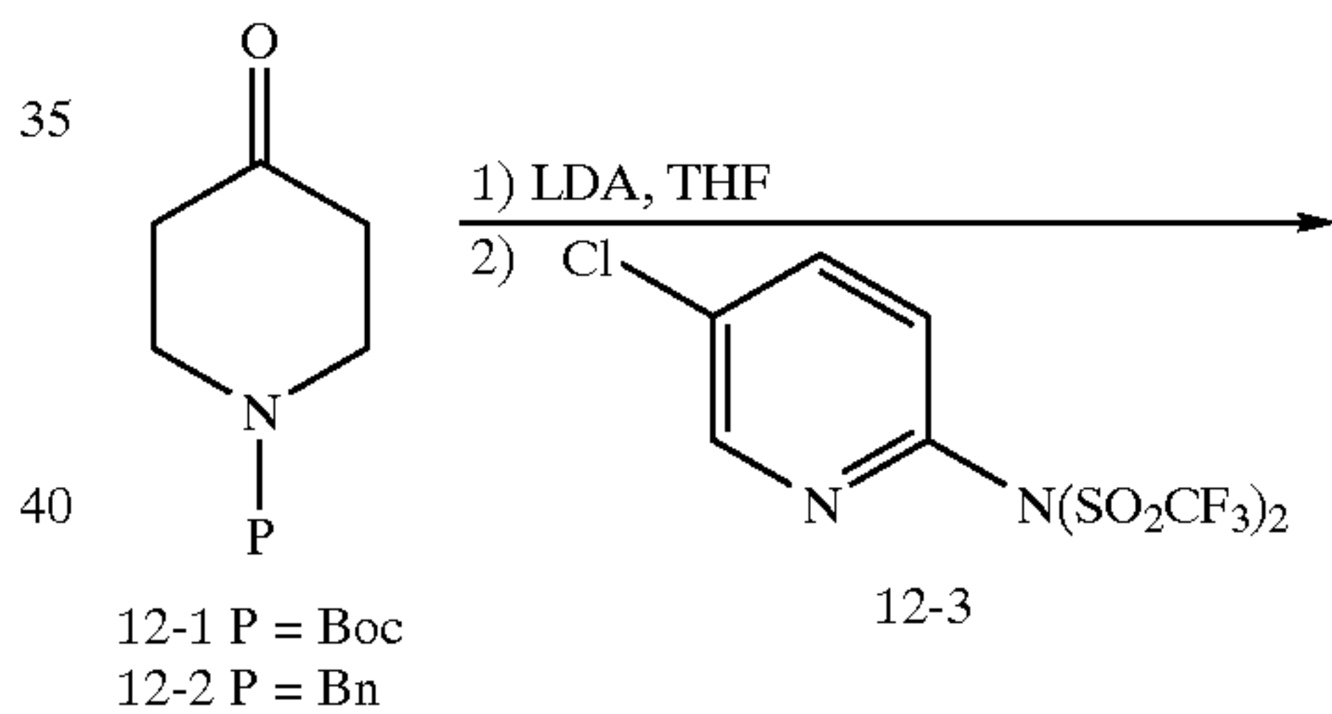
SCHEME 12
