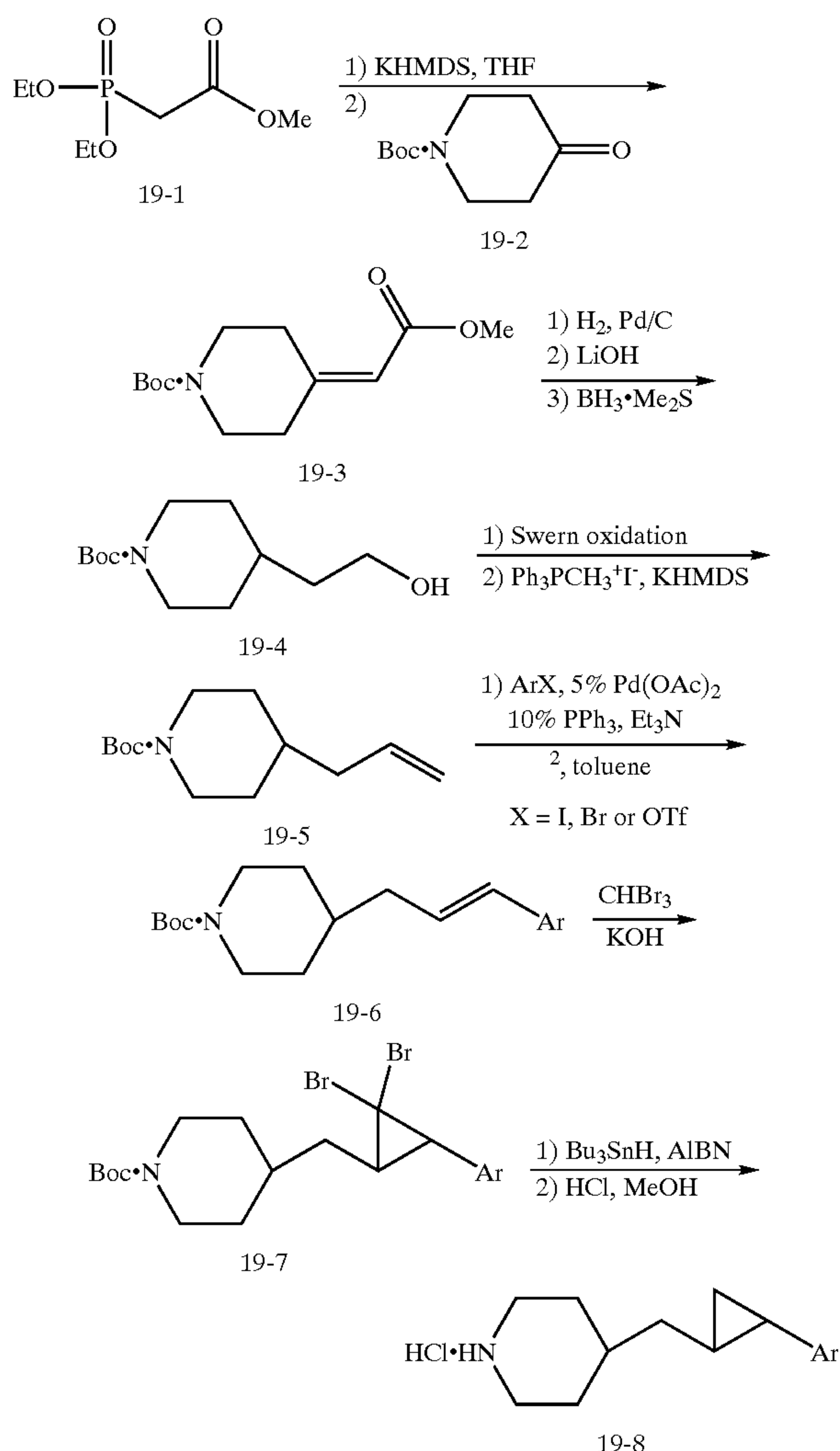
SCHEME 19
