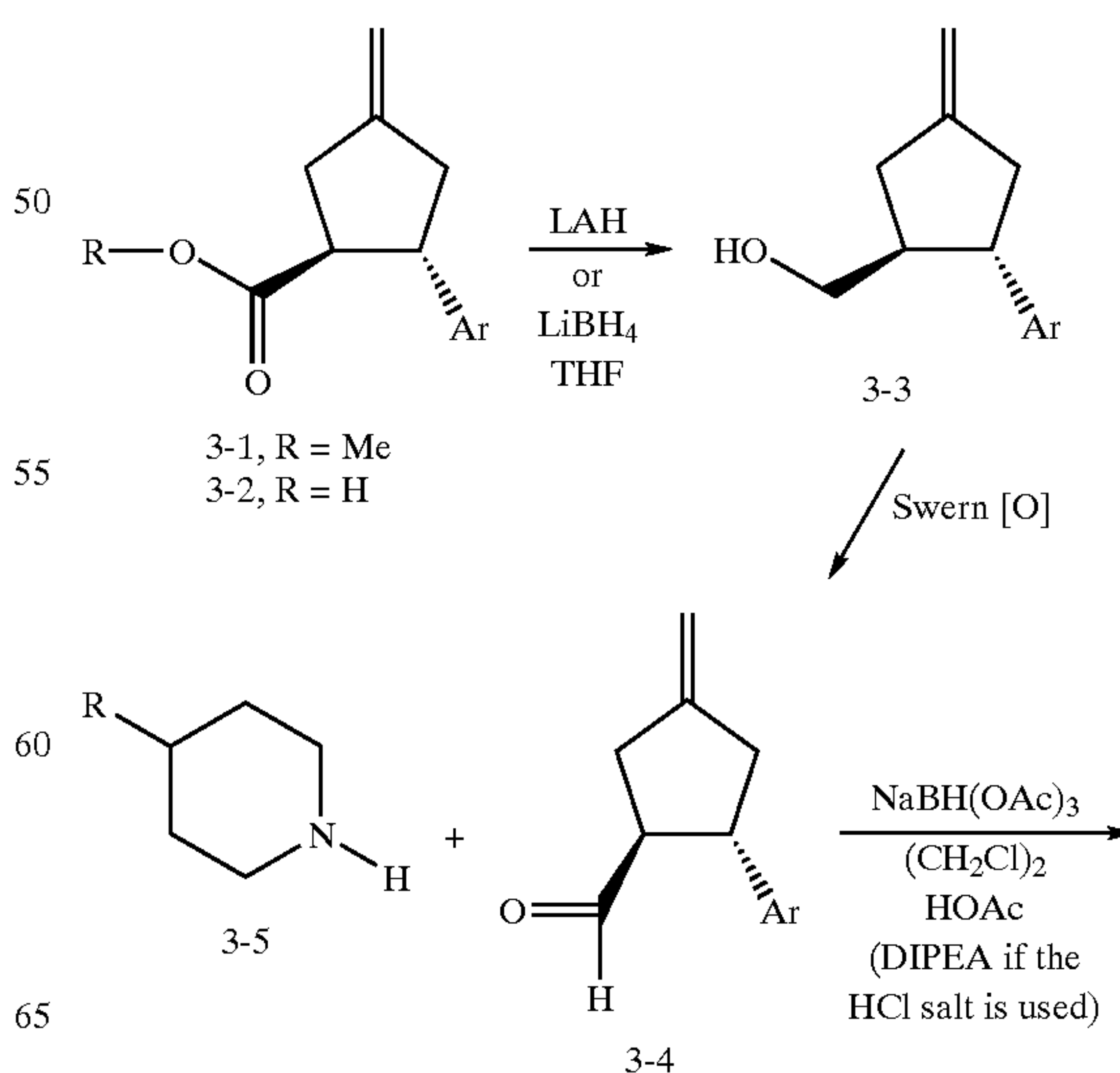
SCHEME 3
