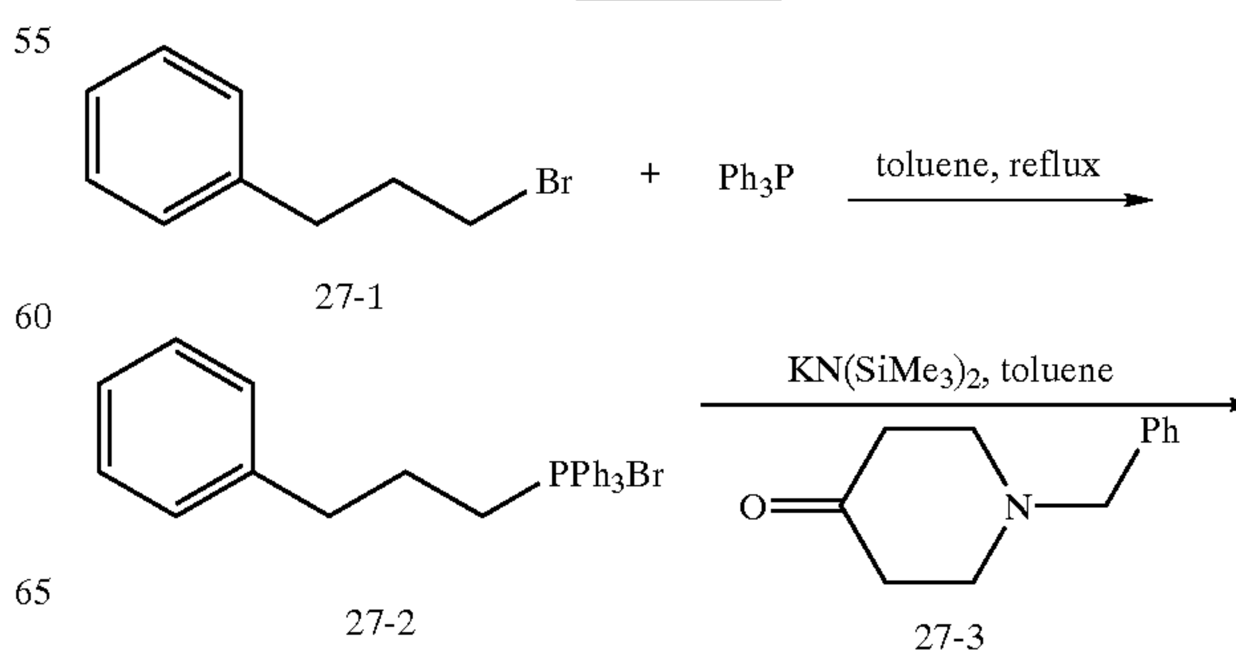
SCHEME 27
