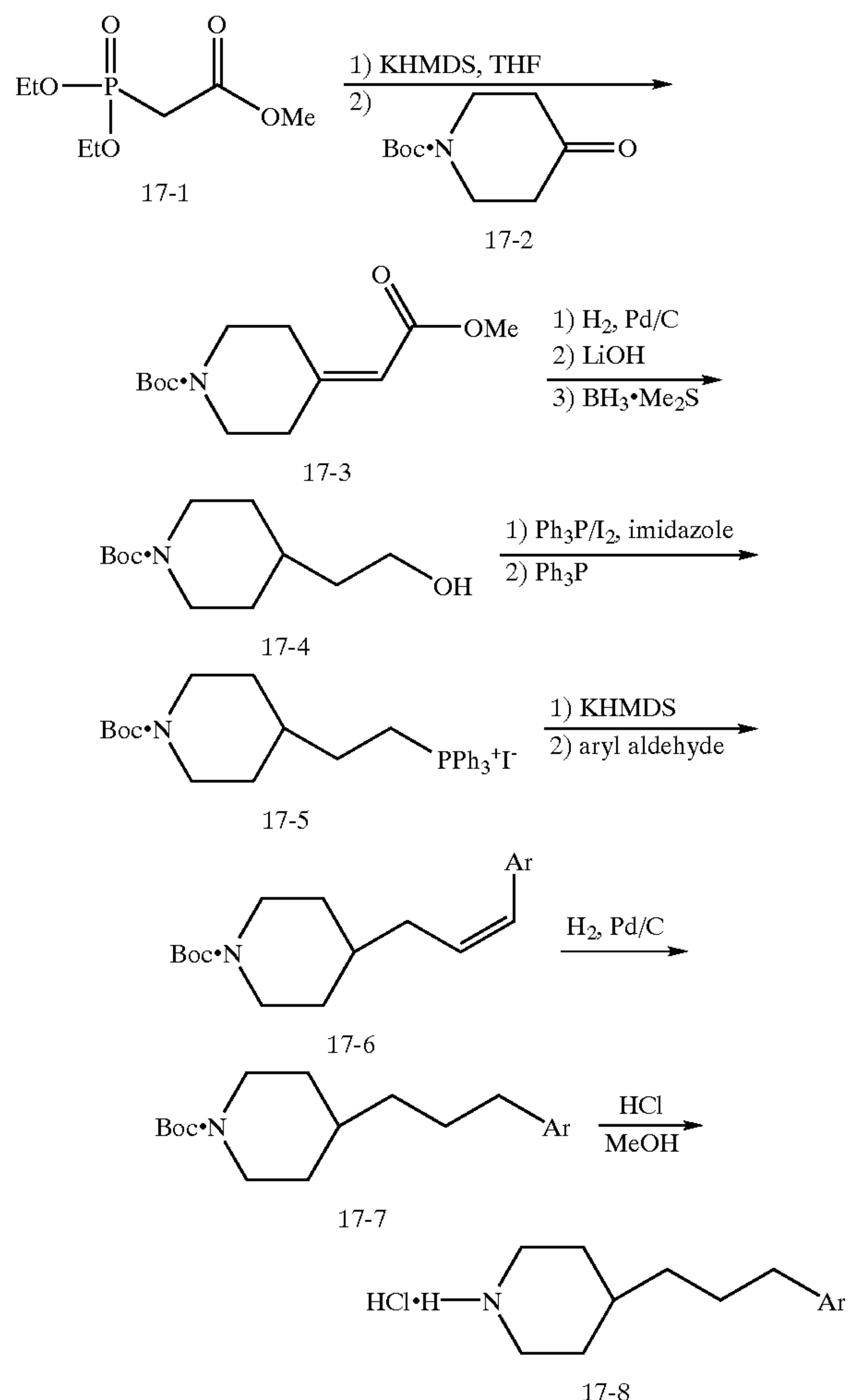
SCHEME 17
