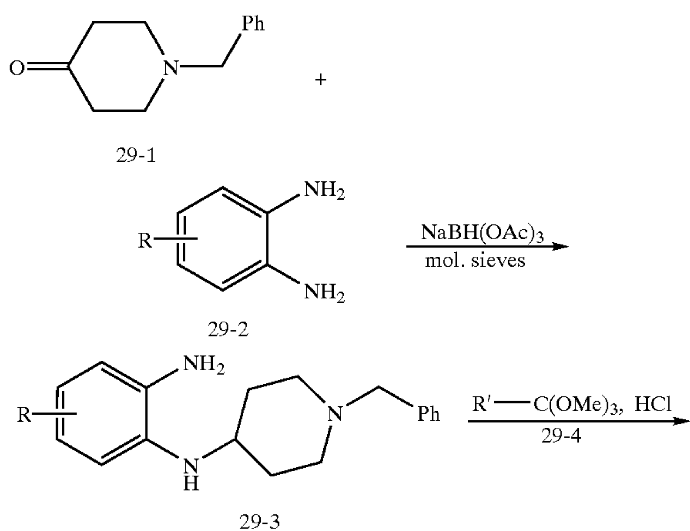
SCHEME 29
