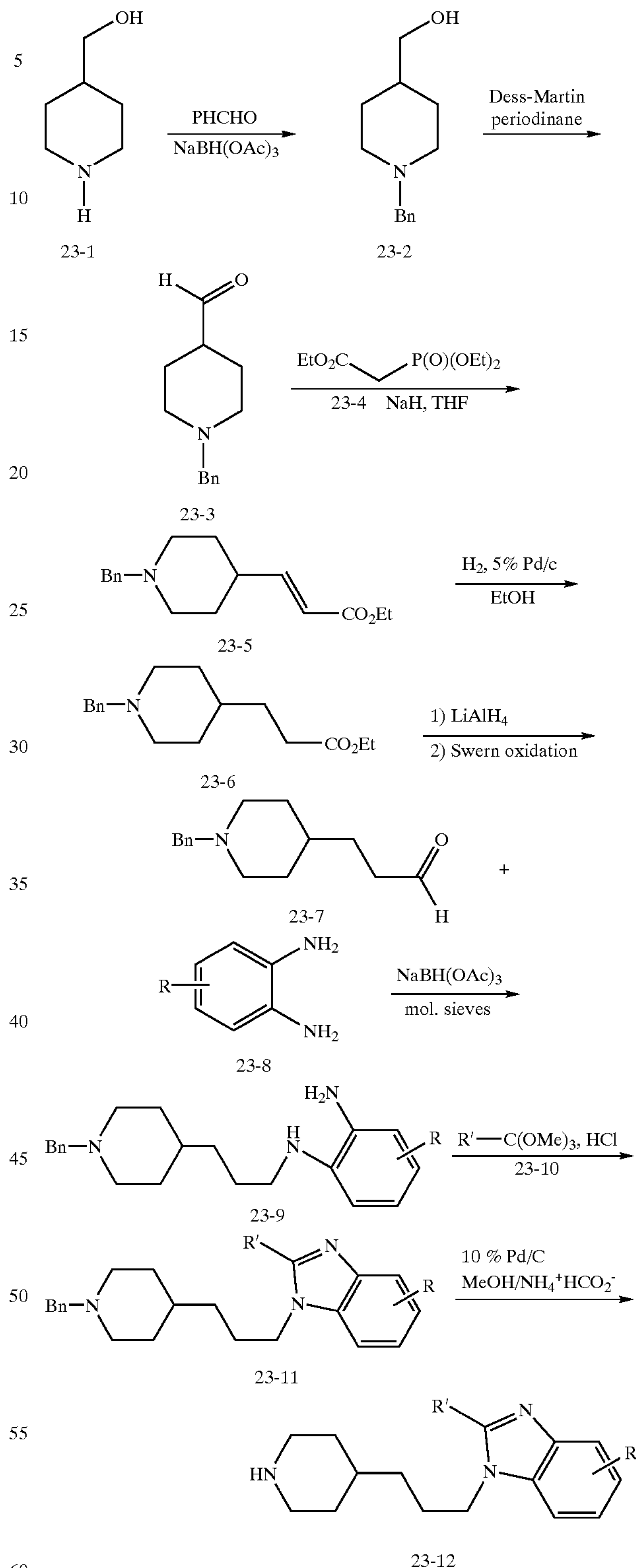
SCHEME 23
