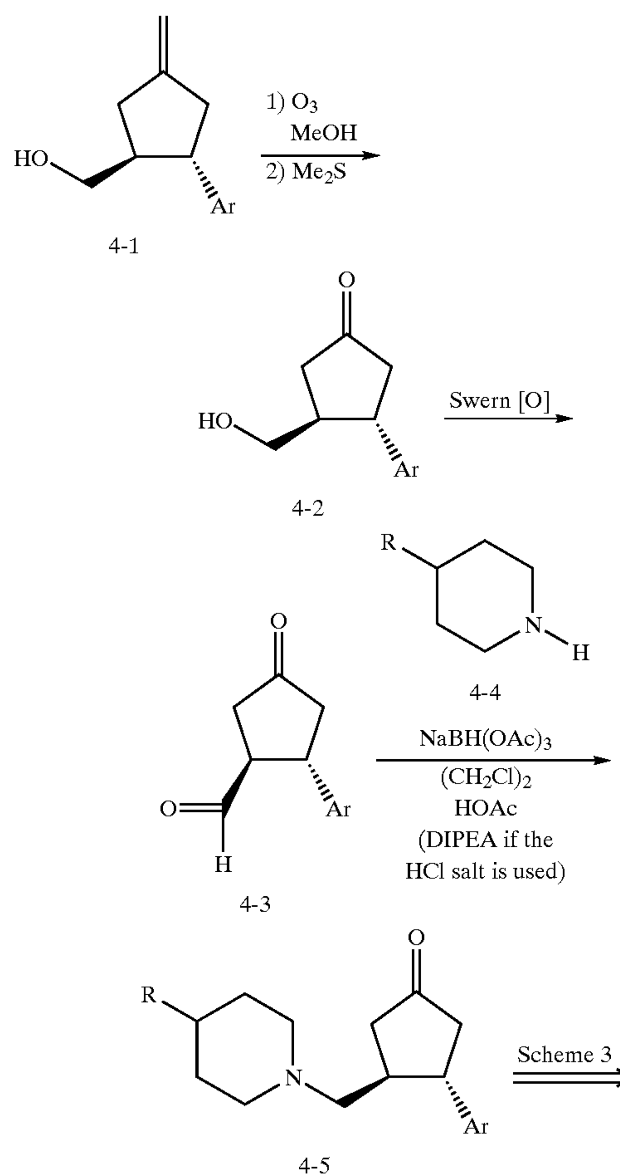
SCHEME 4
