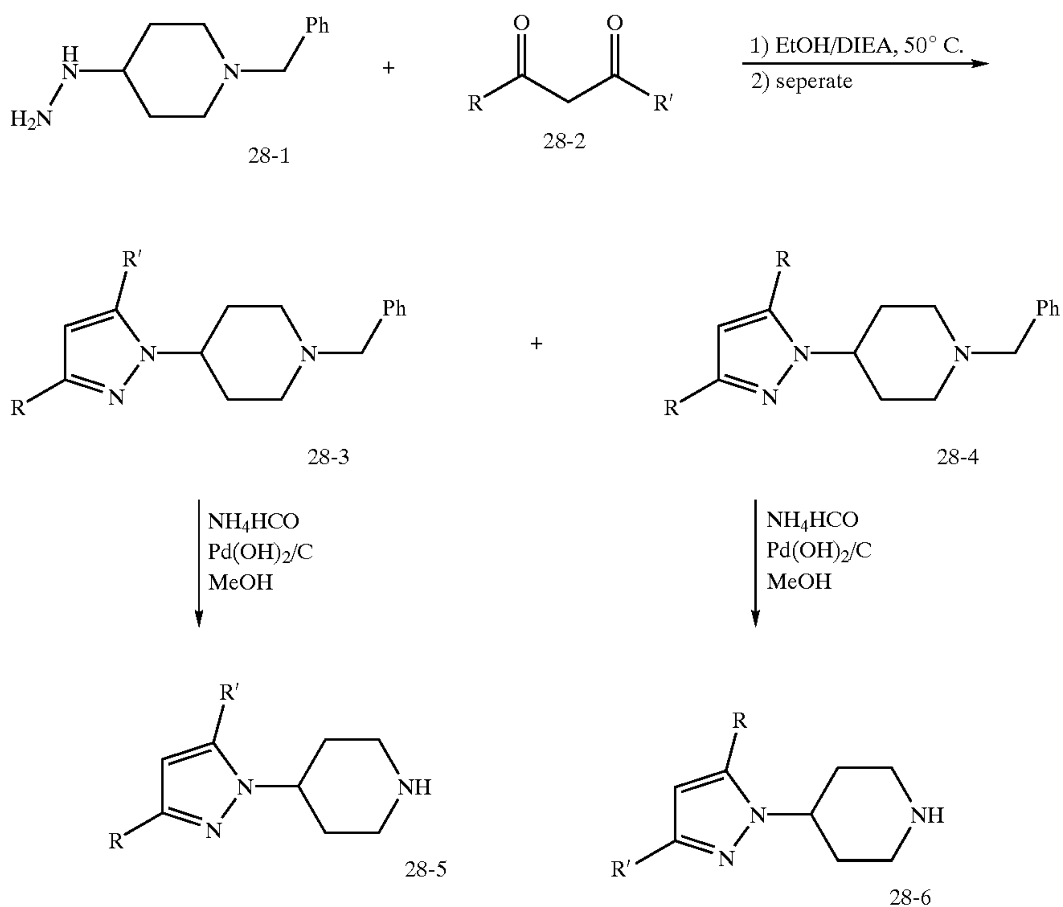
Scheme 28
