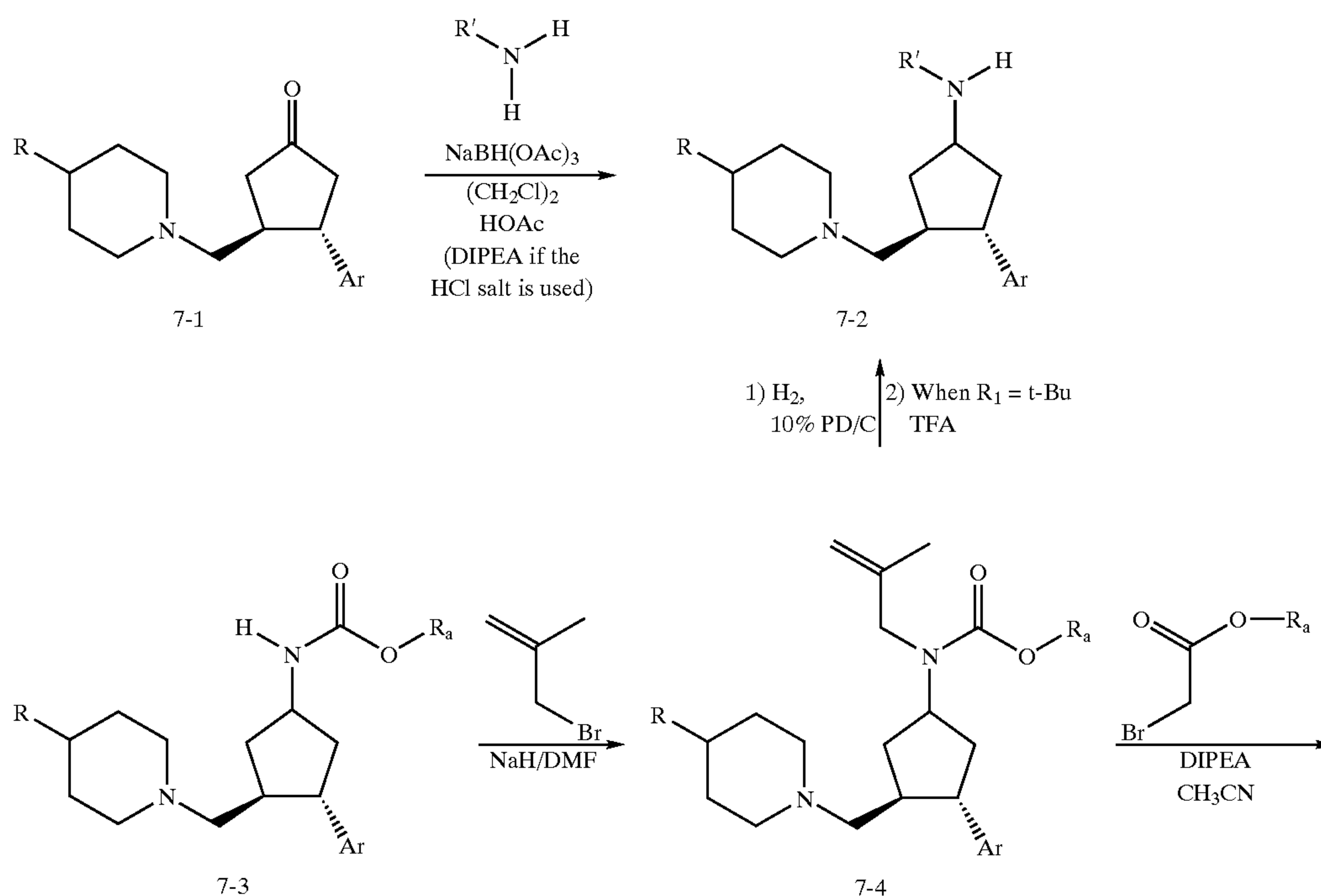
SCHEME 7
