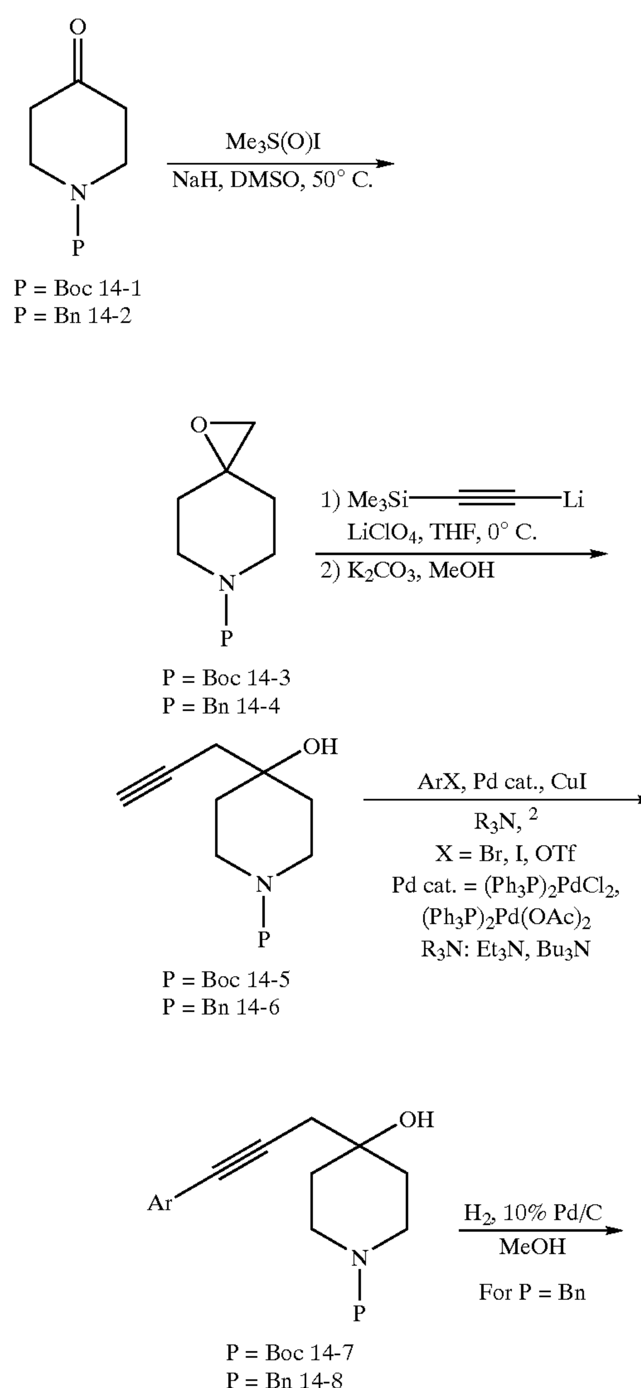
SCHEME 14
