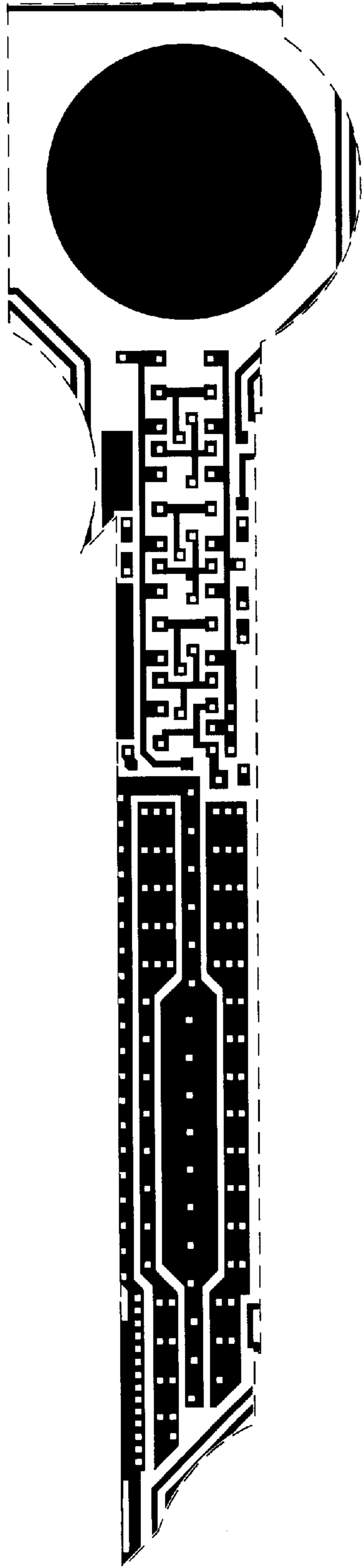
Metal 1 mask
