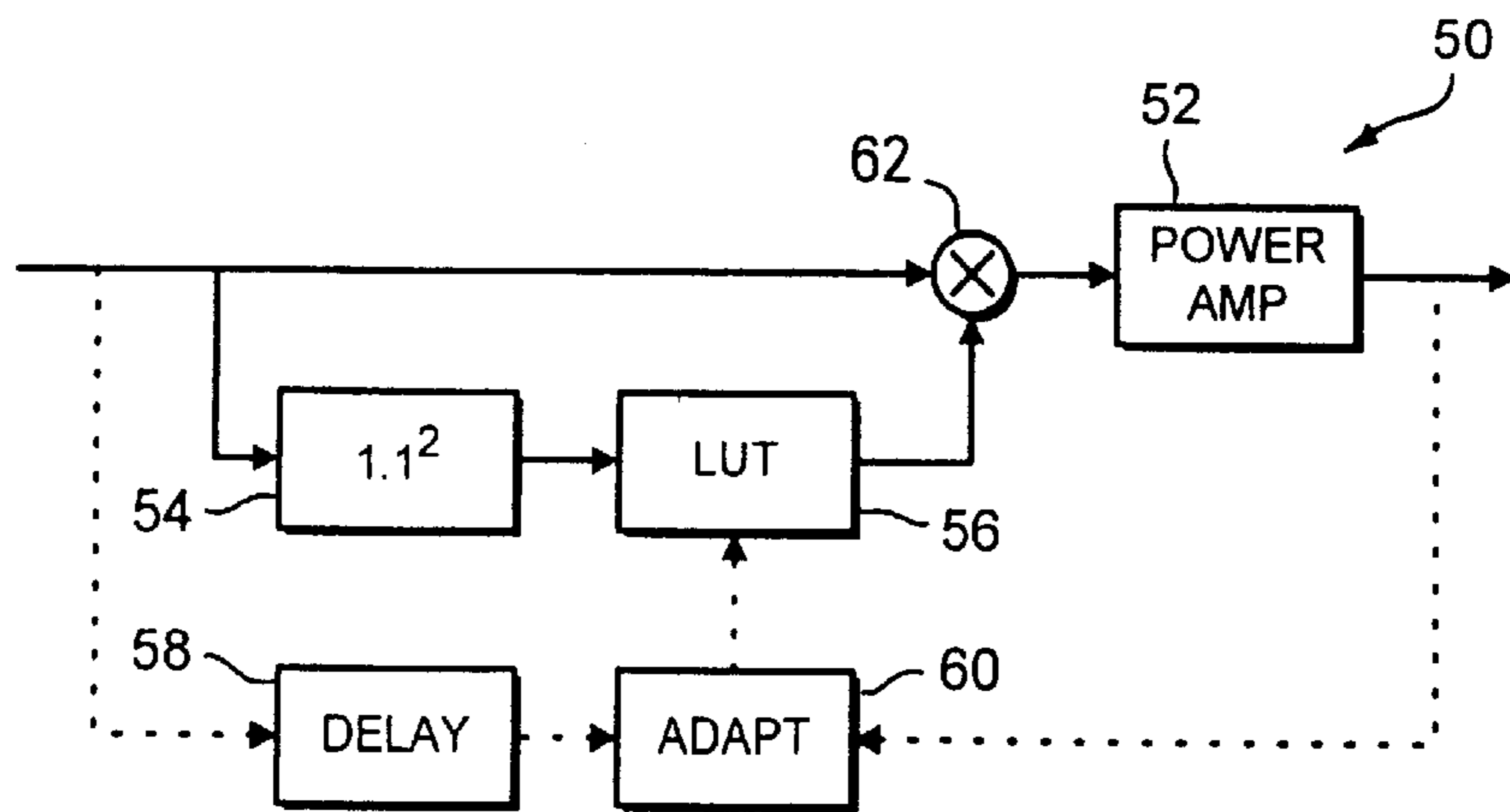
FIG. 1 PRIOR ART
