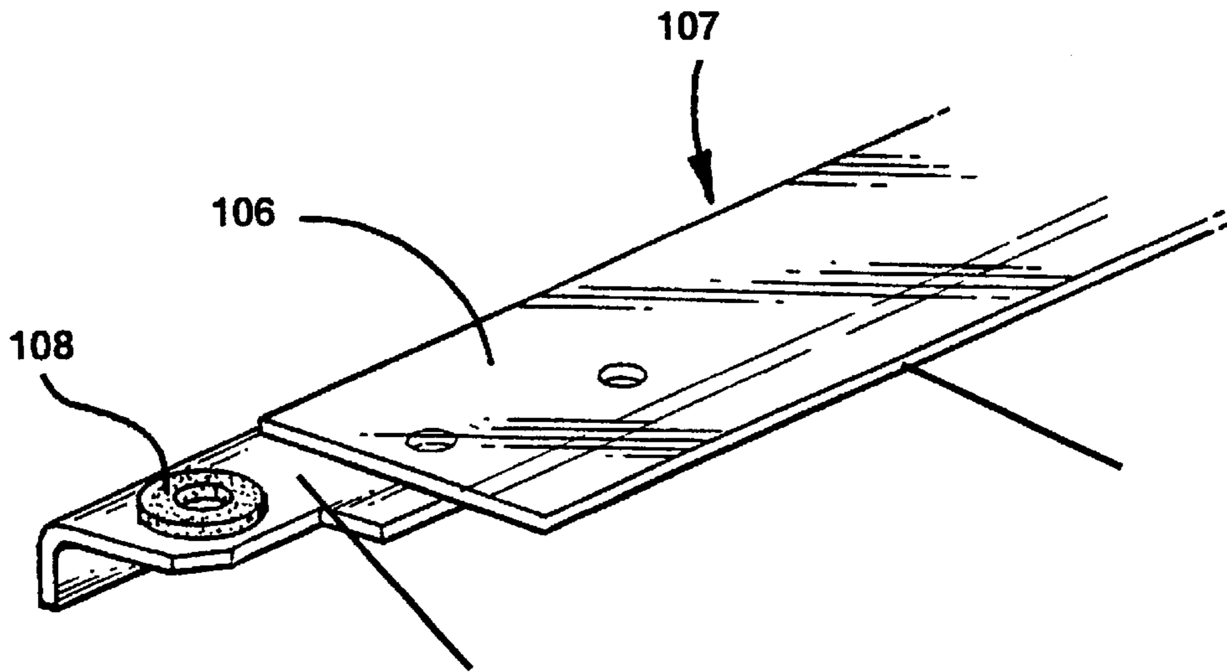
Figure 20 PRIOR ART
