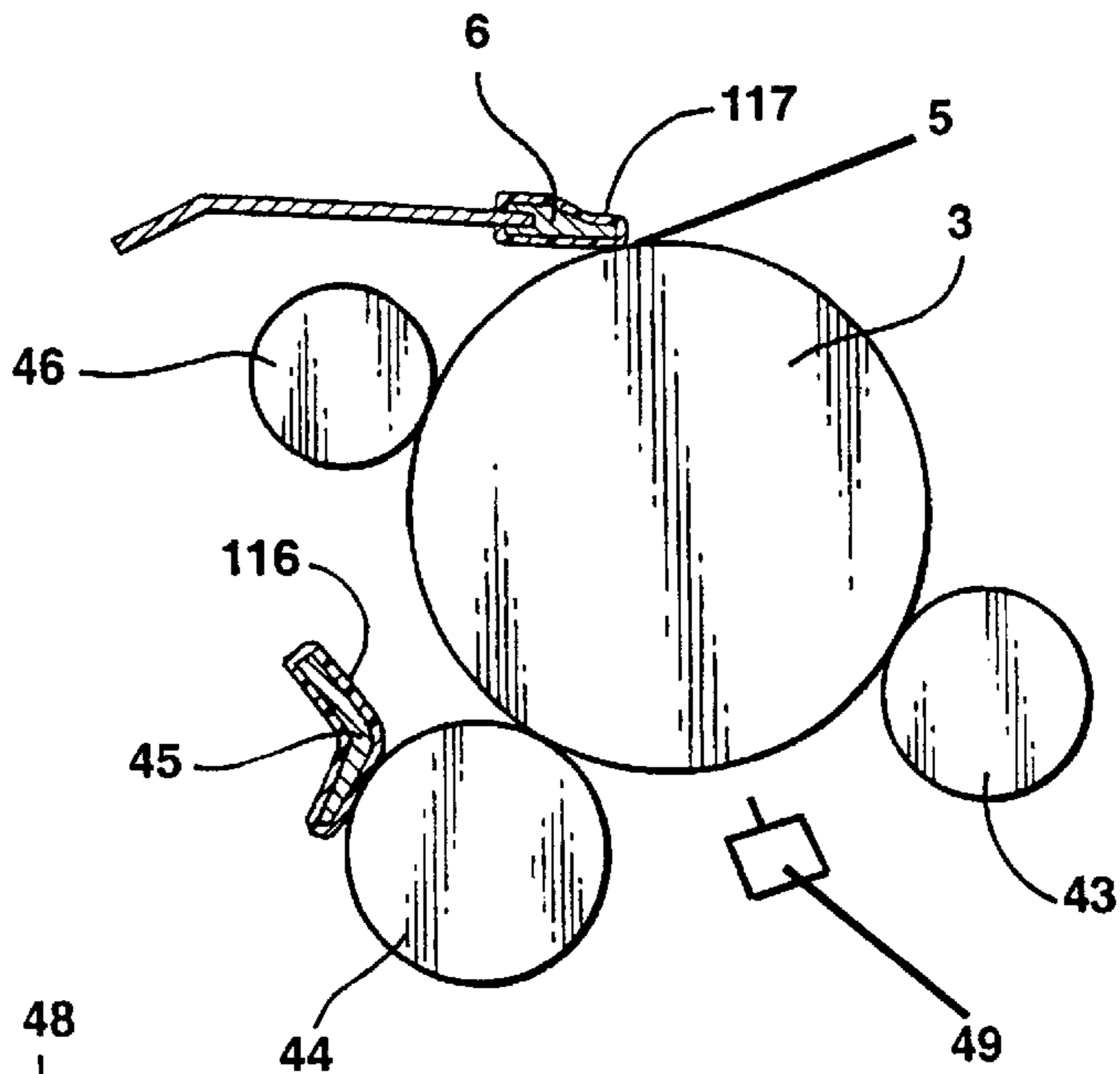
Figure 5 PRIOR ART
