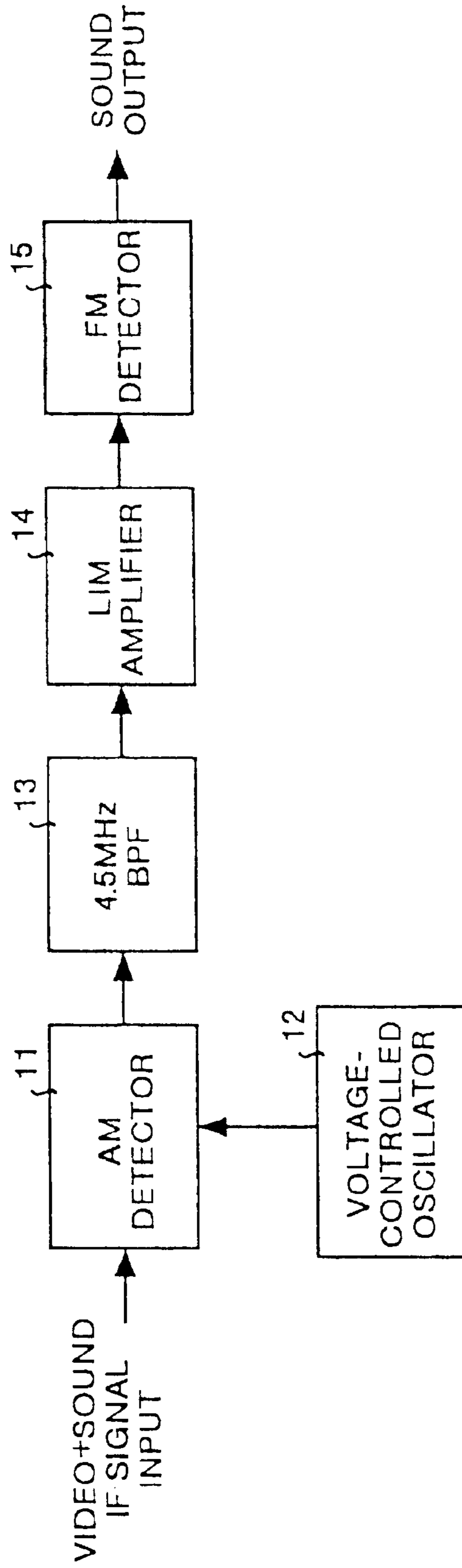
FIG. 6 PRIOR ART
