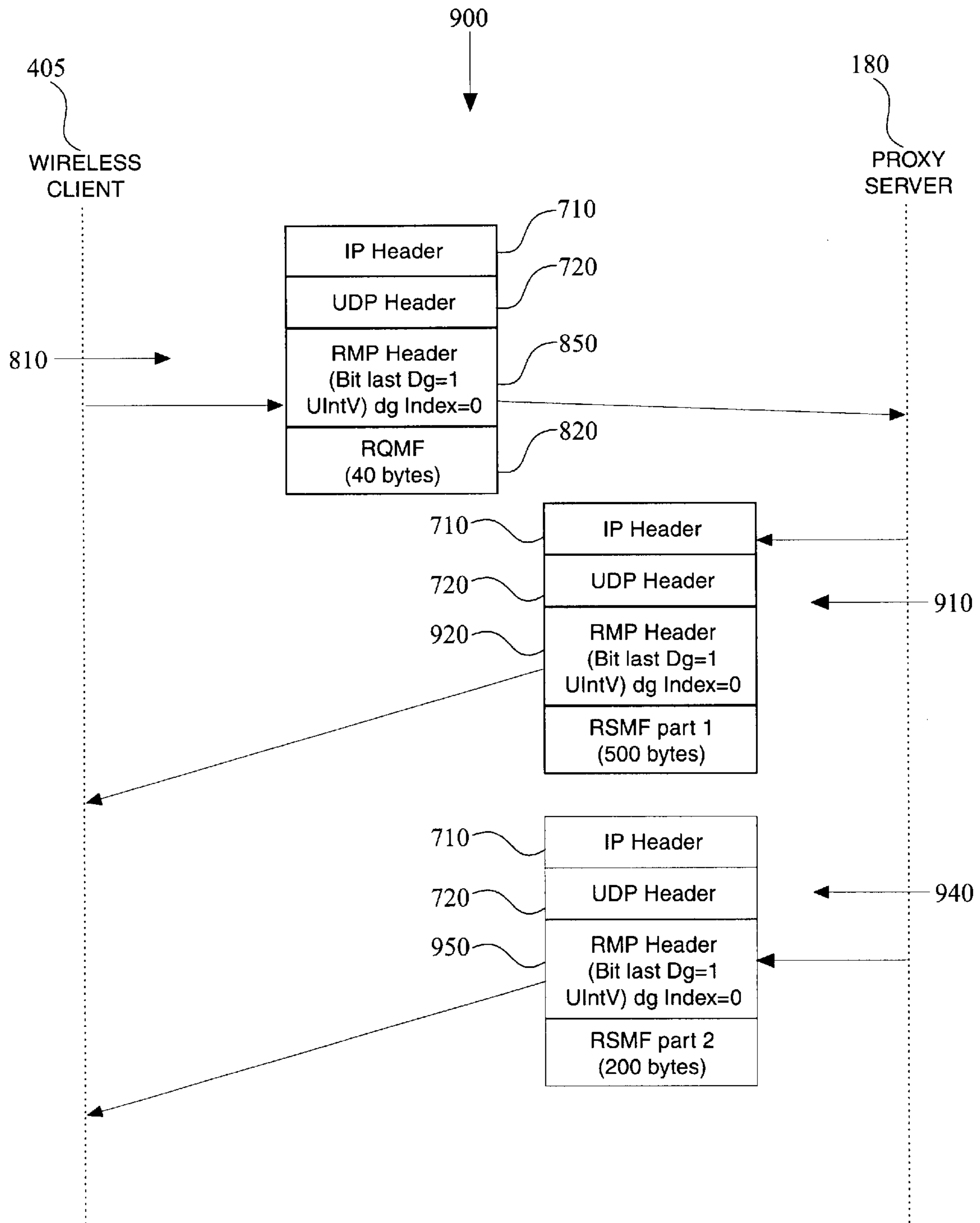
FIG. 9 – EXCHANGE OF MESSAGES COMPRISING A SINGLE REQUEST PACKET AND TWO RESPONSE PACKETS
