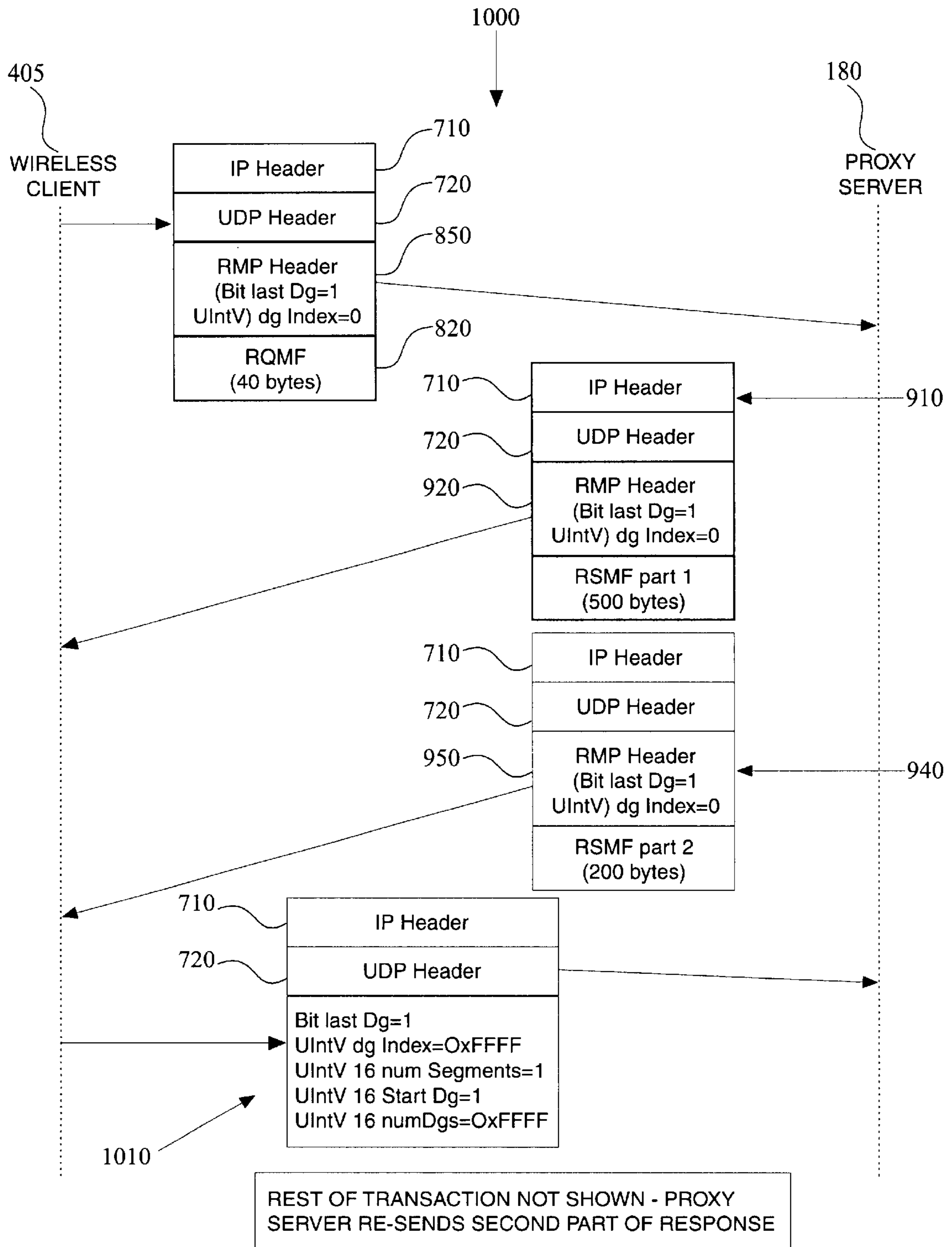
FIG. 10 – EXCHANGE OF MESSAGES INCLUDING A RE-TRANSMIT SEQUENCE
