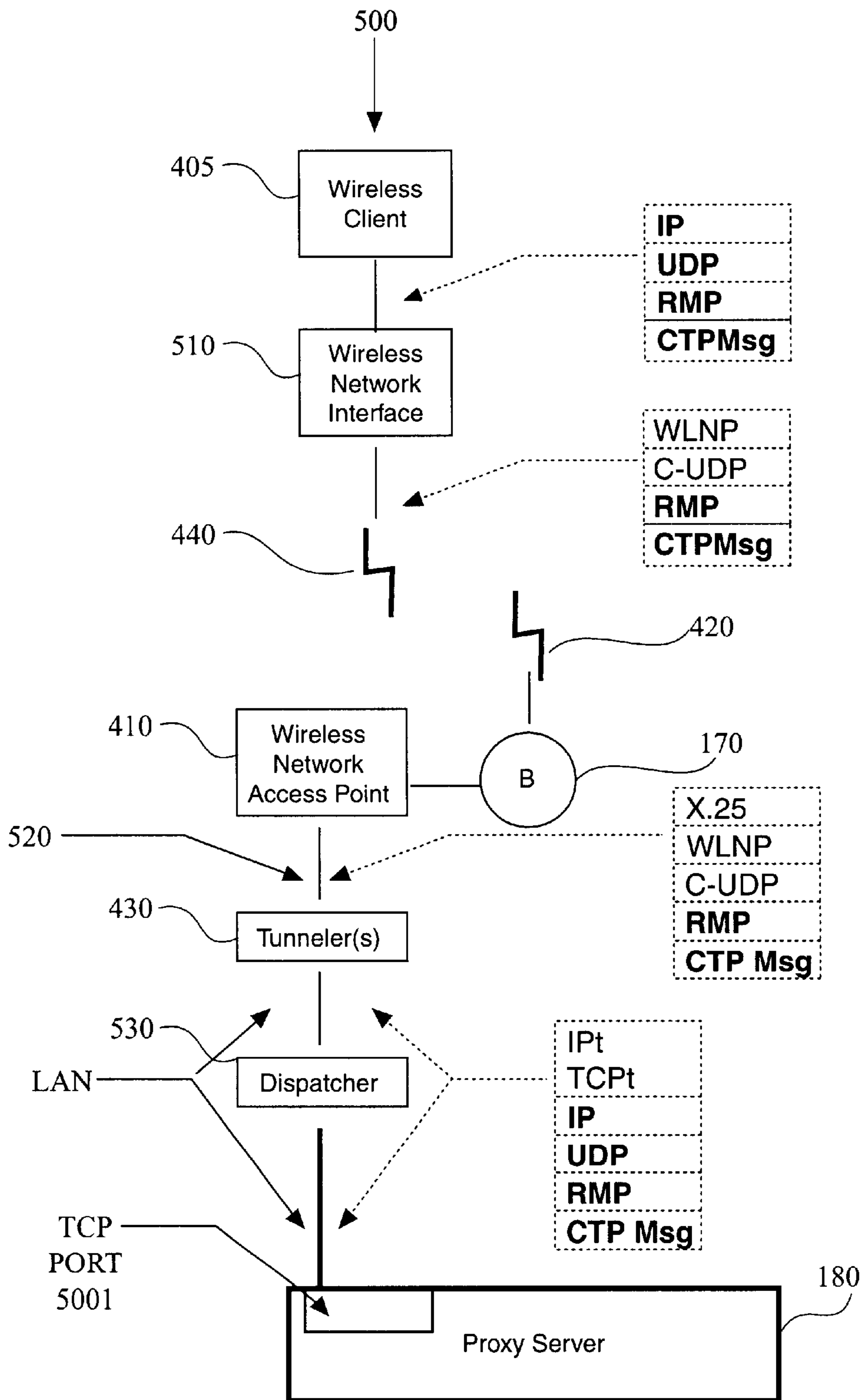
FIG. 5 – WIRELESS NETWORK TOPOLOGY INCLUDING A WIRELESS NETWORK INTERFACE, A LEASED LINE, AND A DISPATCHER
