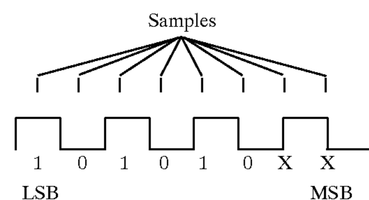
Late Sampling of Genlock Waveform
