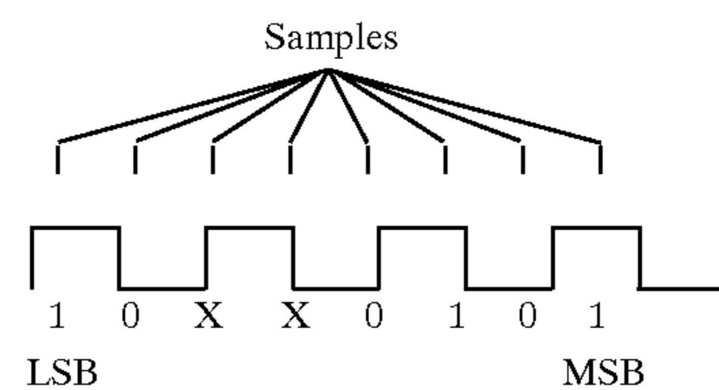
Early Sampling of Genlock Waveform
