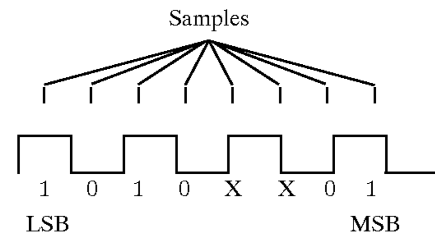
Nominal Sampling of Genlock Waveform
