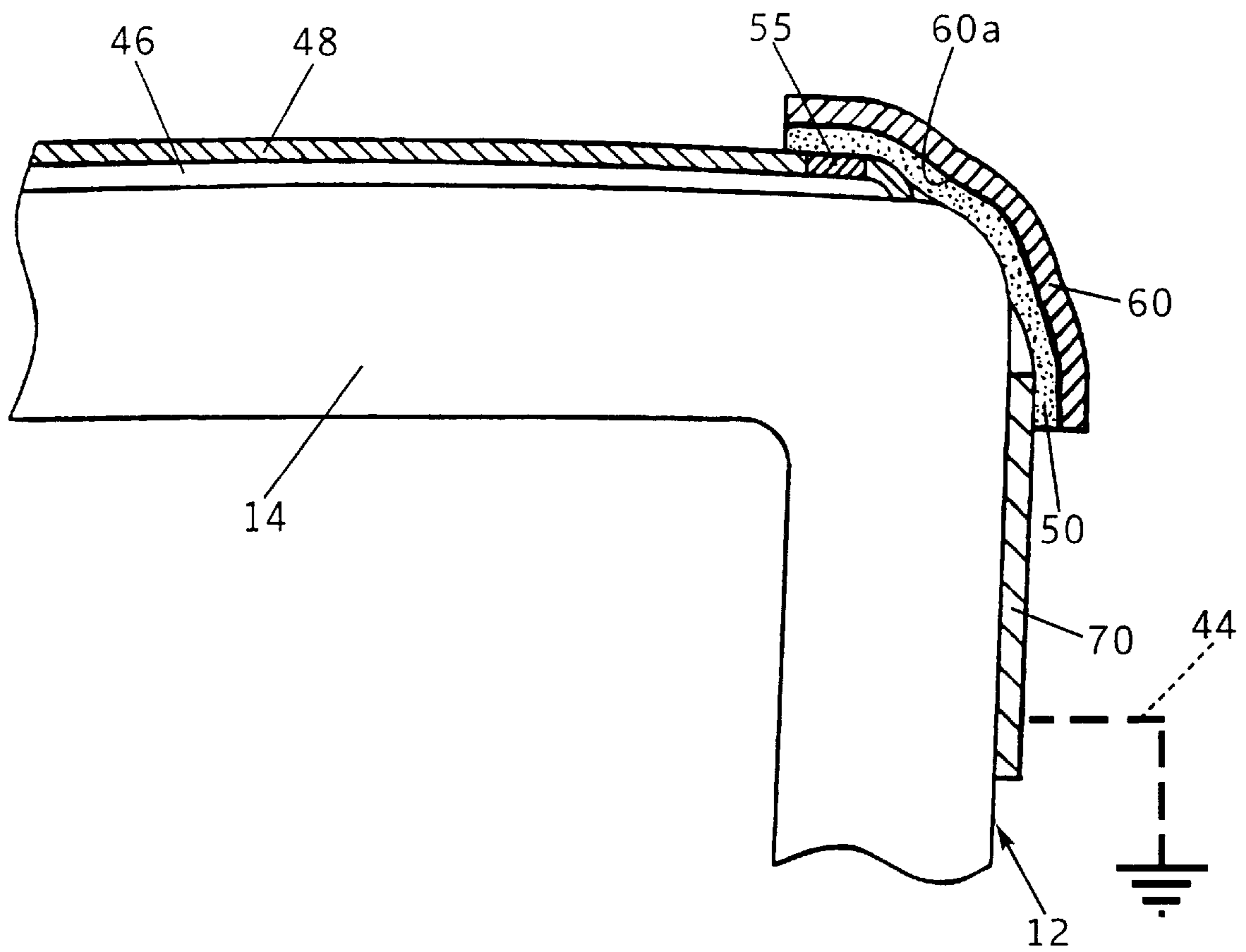
FIG. 4 (PRIOR ART)
