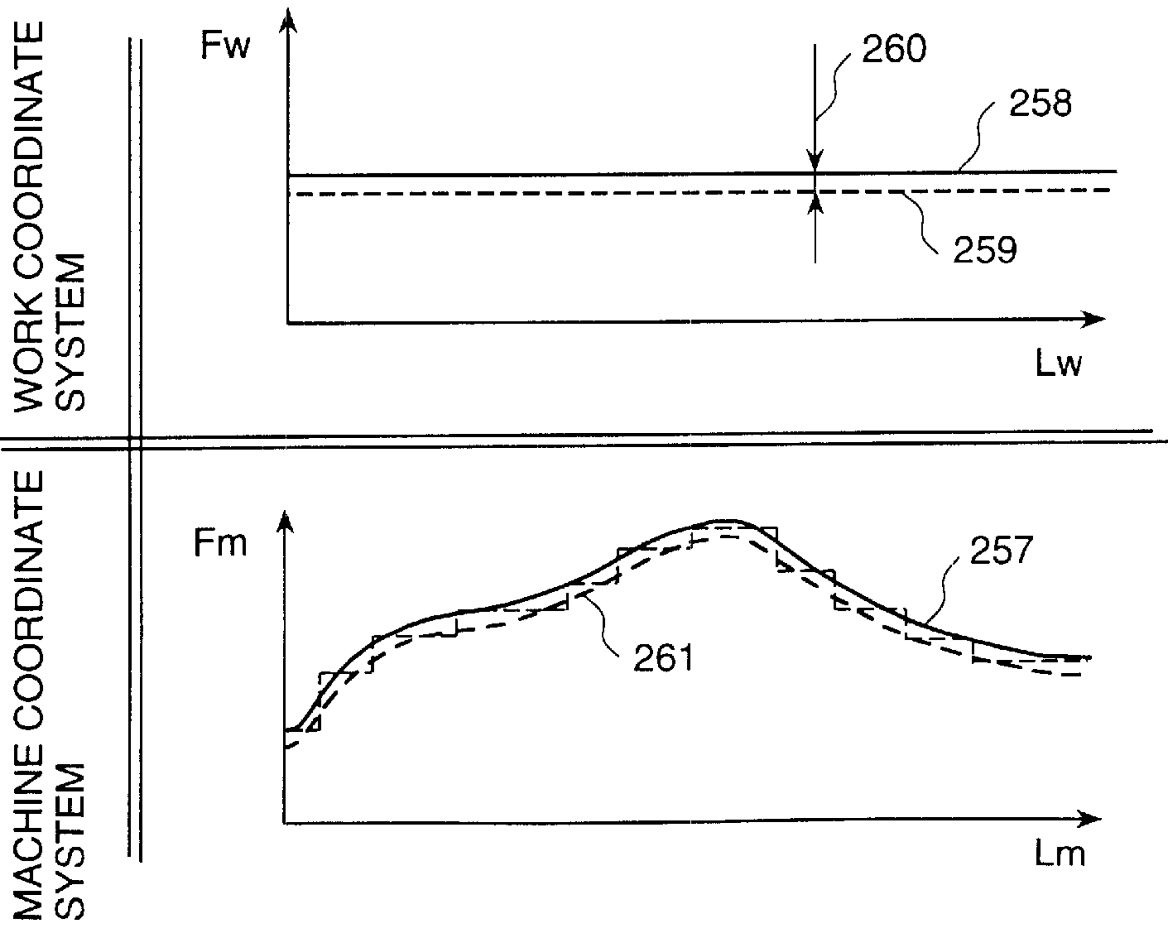
OPTIMIZATION OF MACHINE COORDINATE SYSTEM FEED RATE BY BLENDING COEFFICIENT
