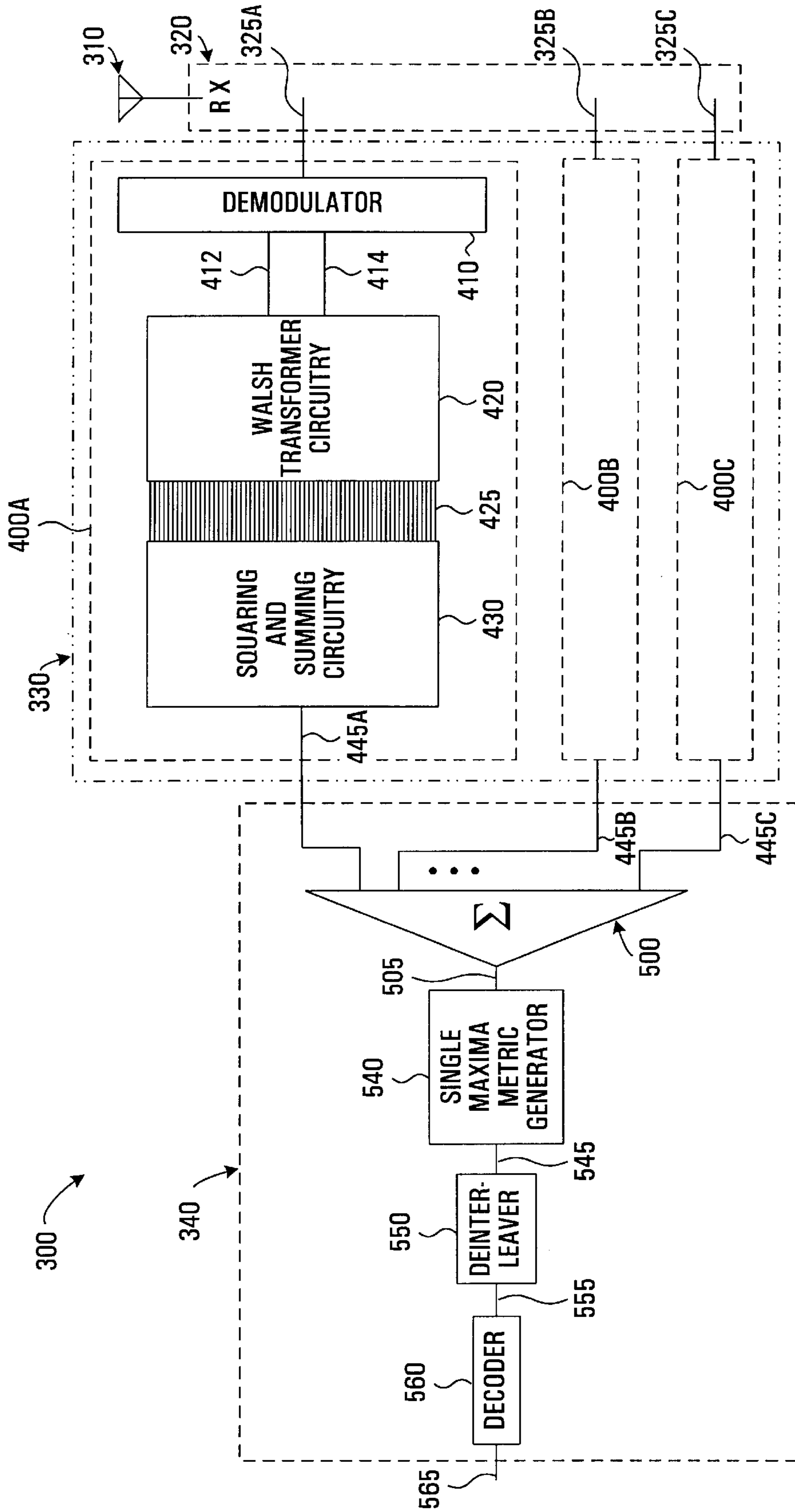
FIG. 2 PRIOR ART
