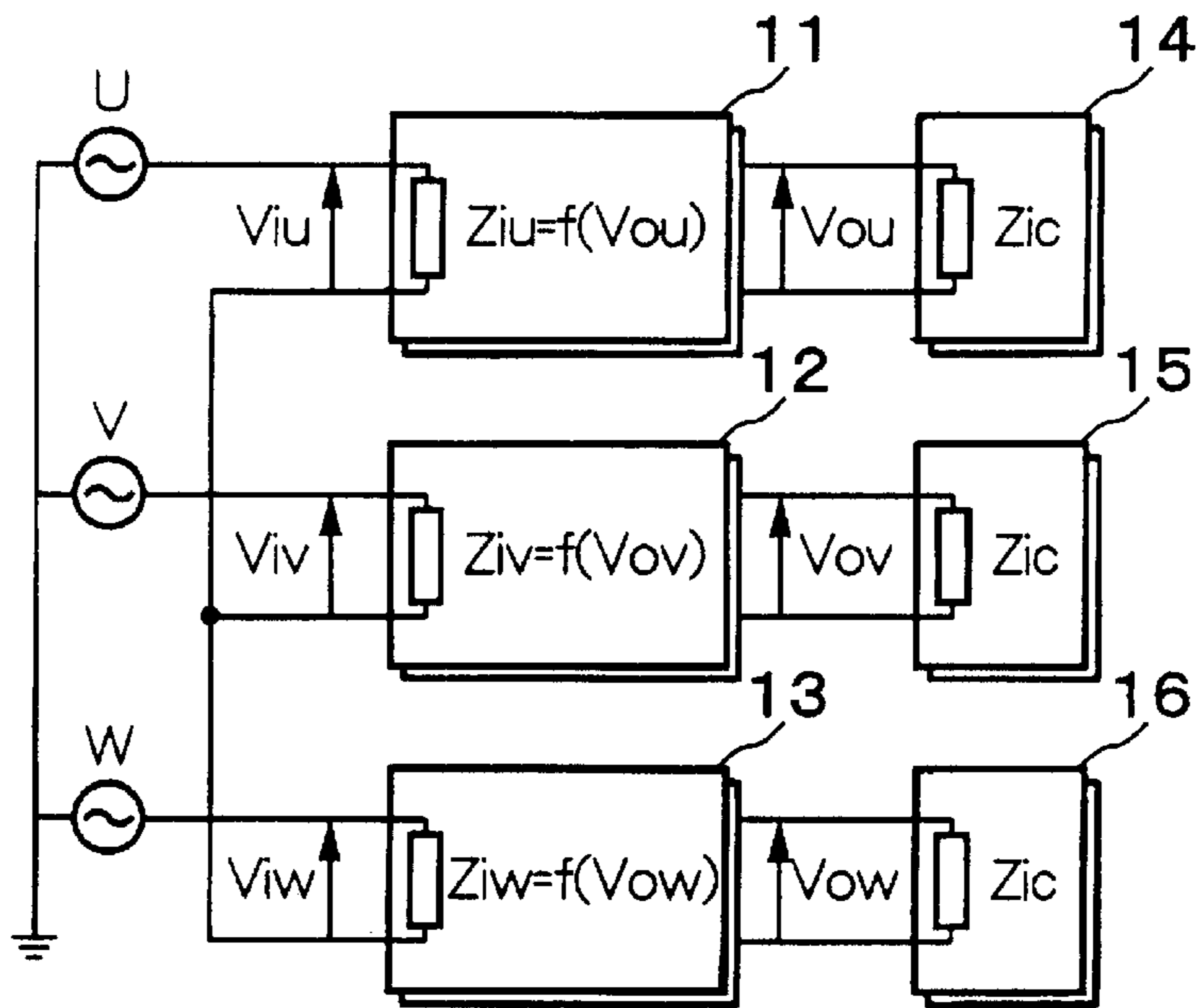
FIG. 6 PRIOR ART
