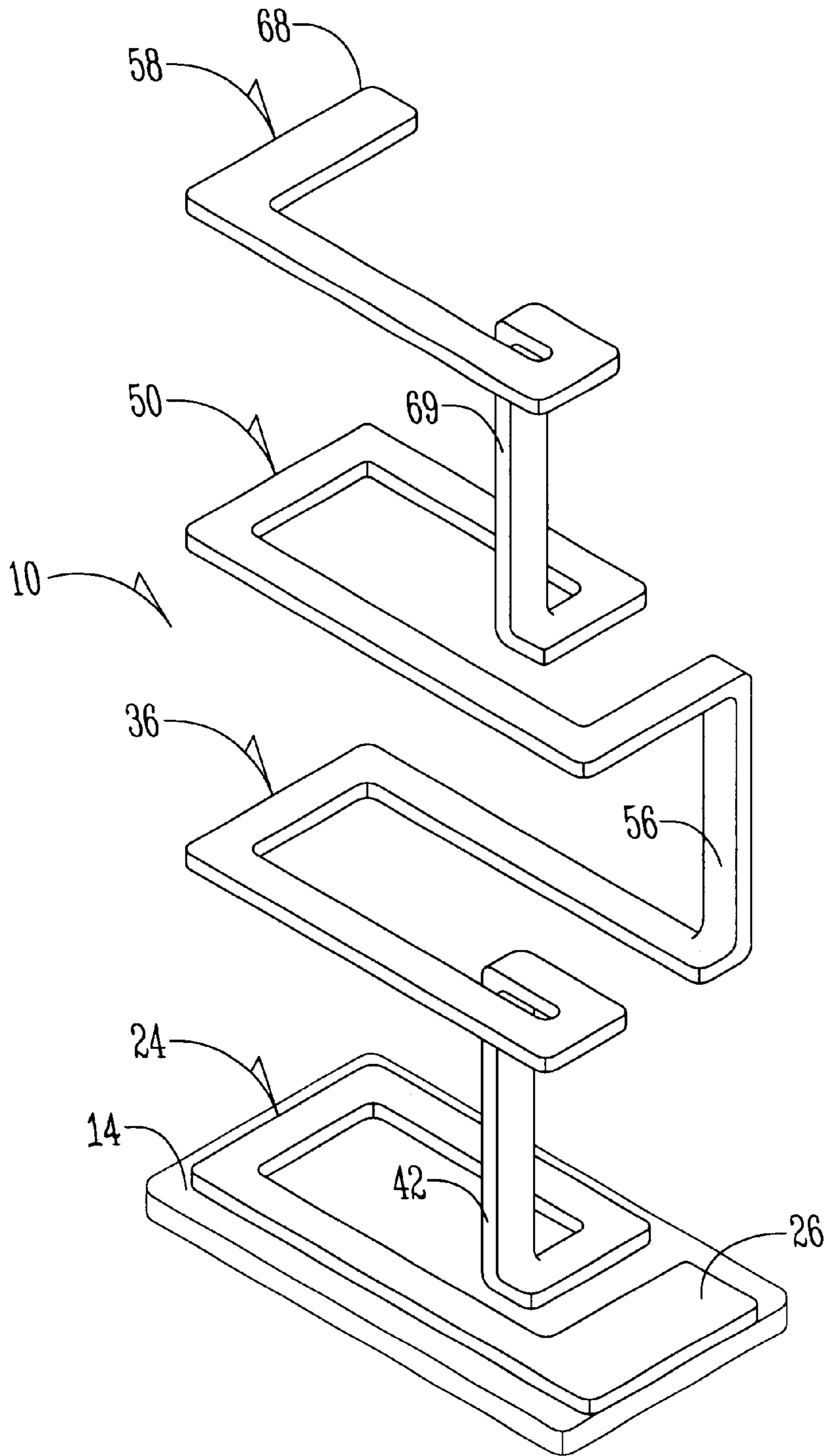
Fig. 2 (PRIOR ART)
