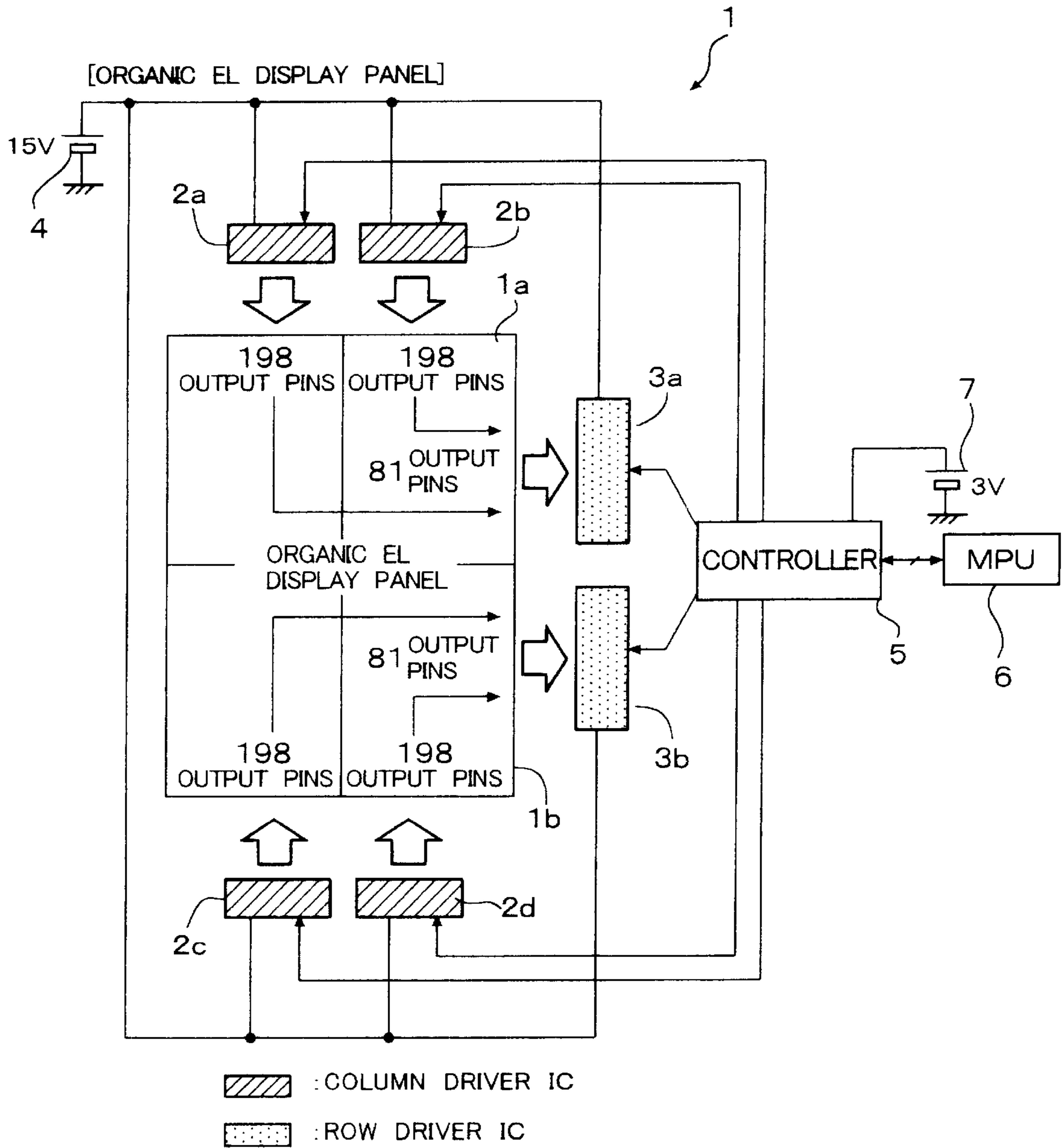
FIG. 7 PRIOR ART
