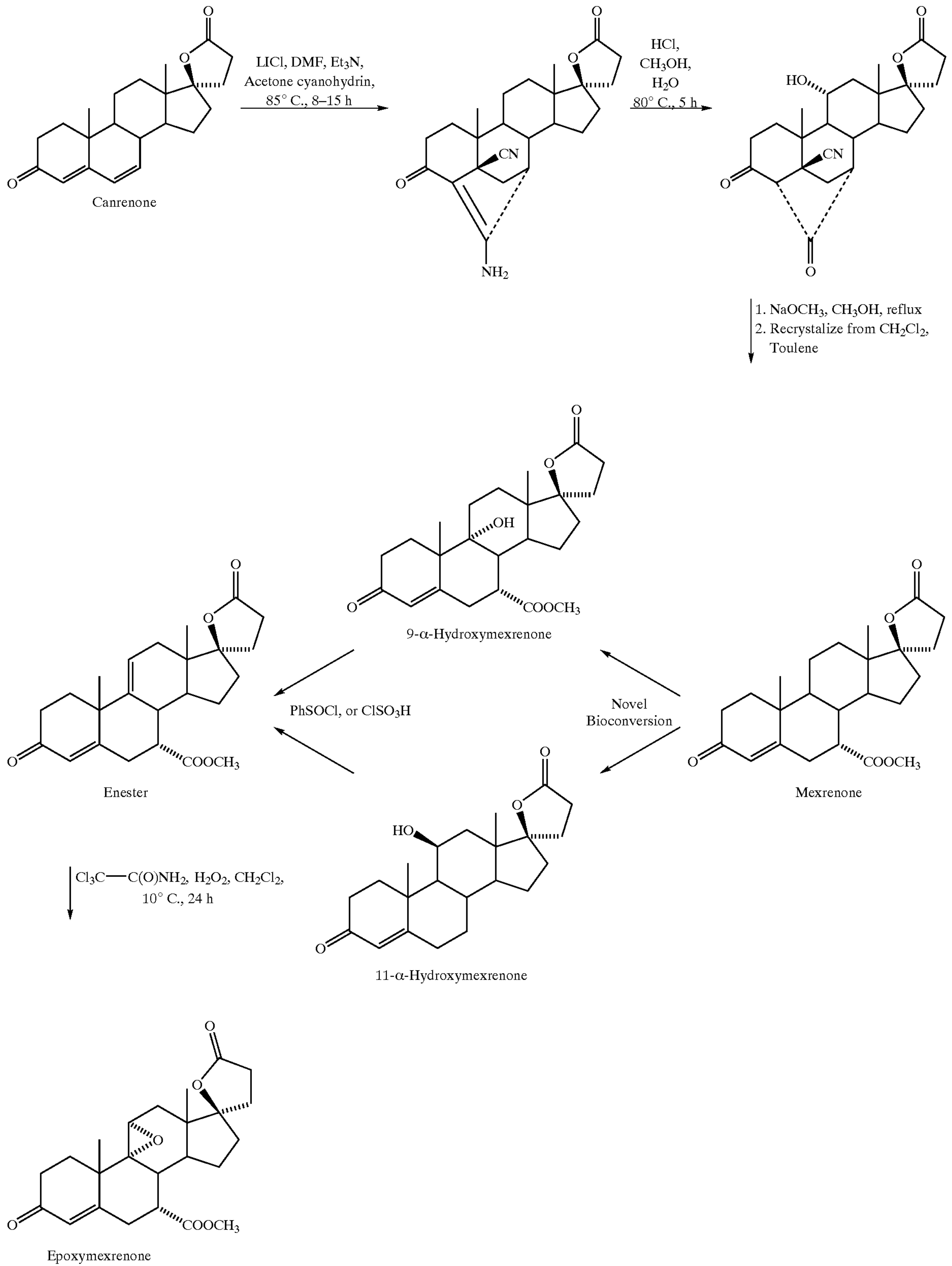
Scheme 3
