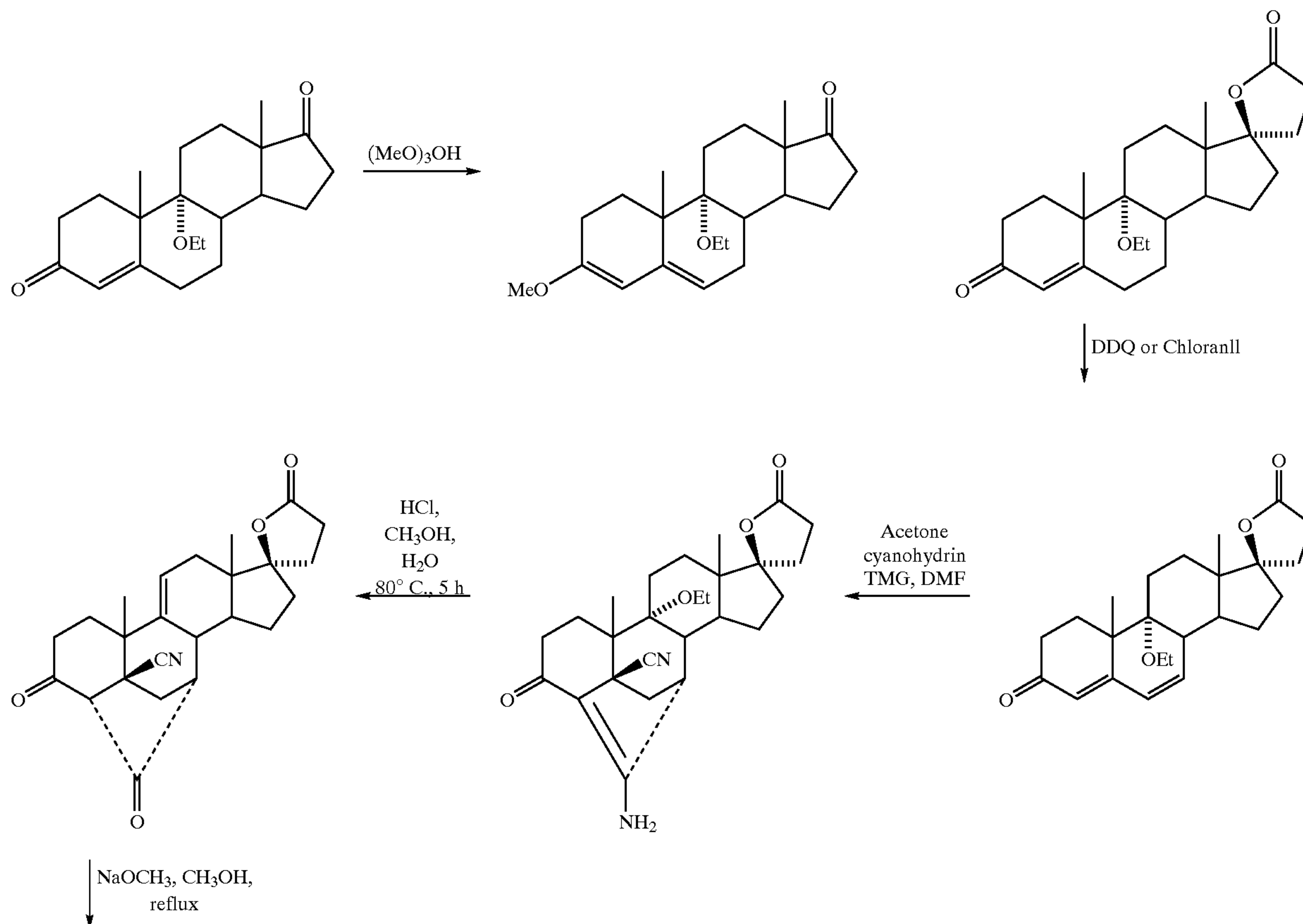
Scheme 6
