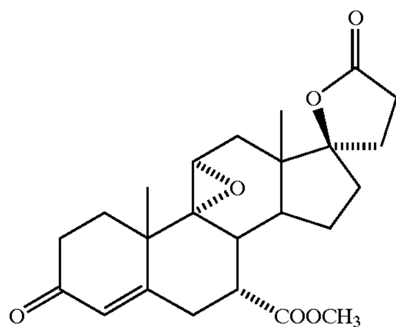
Epoximexrenone
