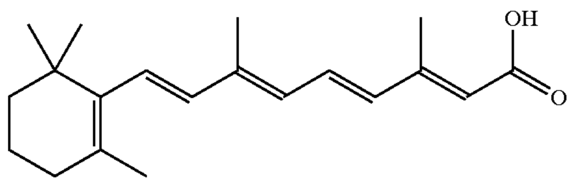
trans-retinoic acid [t-RA]
