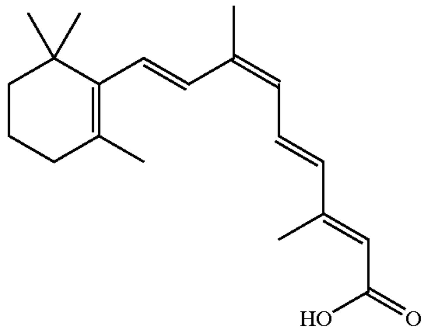
9-cis-retinoic acid [9-c-RA]
