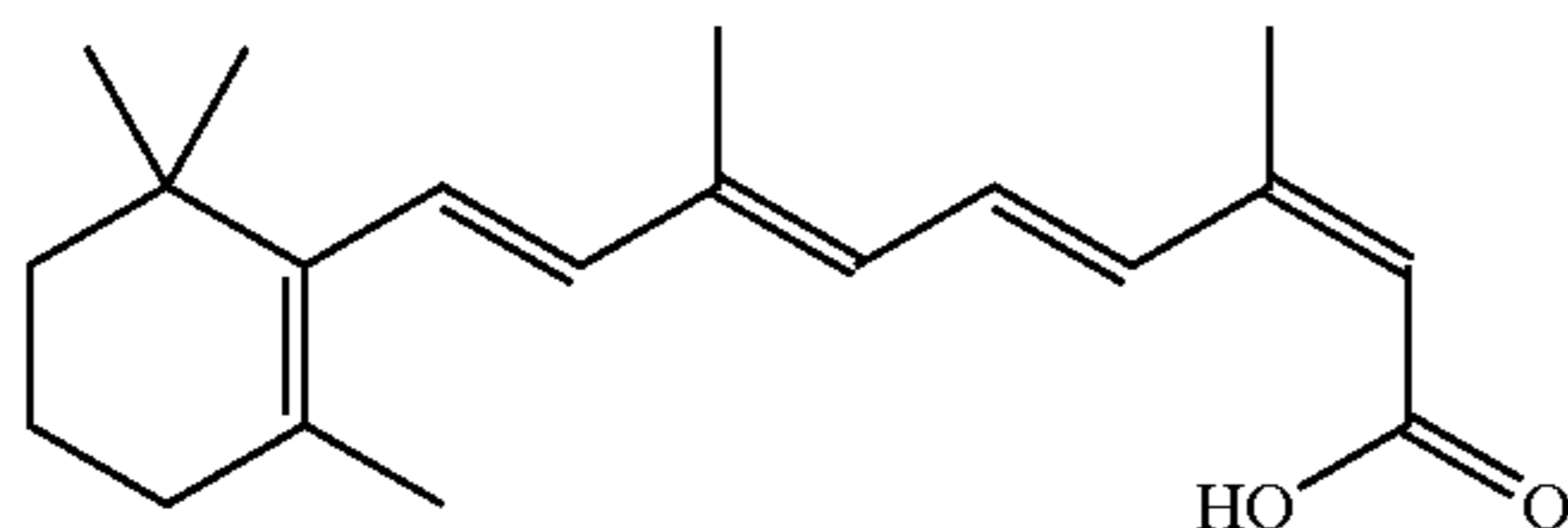
13-cis-retinoic acid [13-c-RA]
