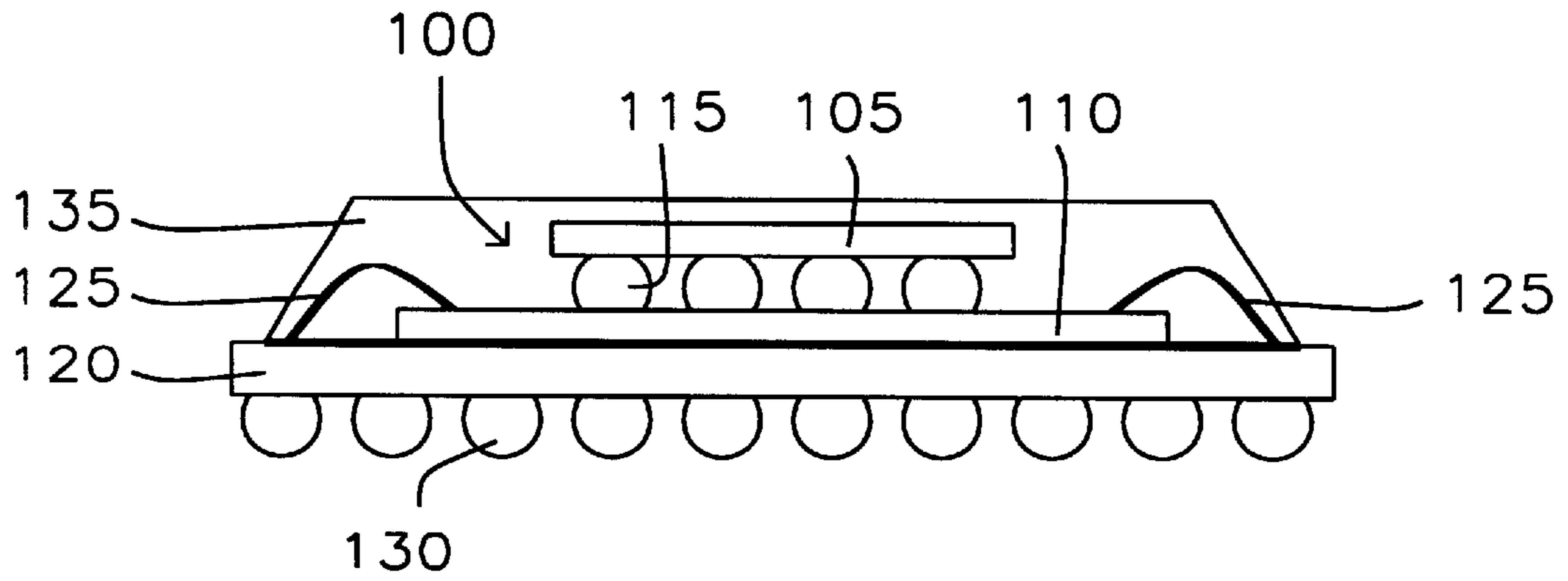
FIG. 1 - Prior Art
