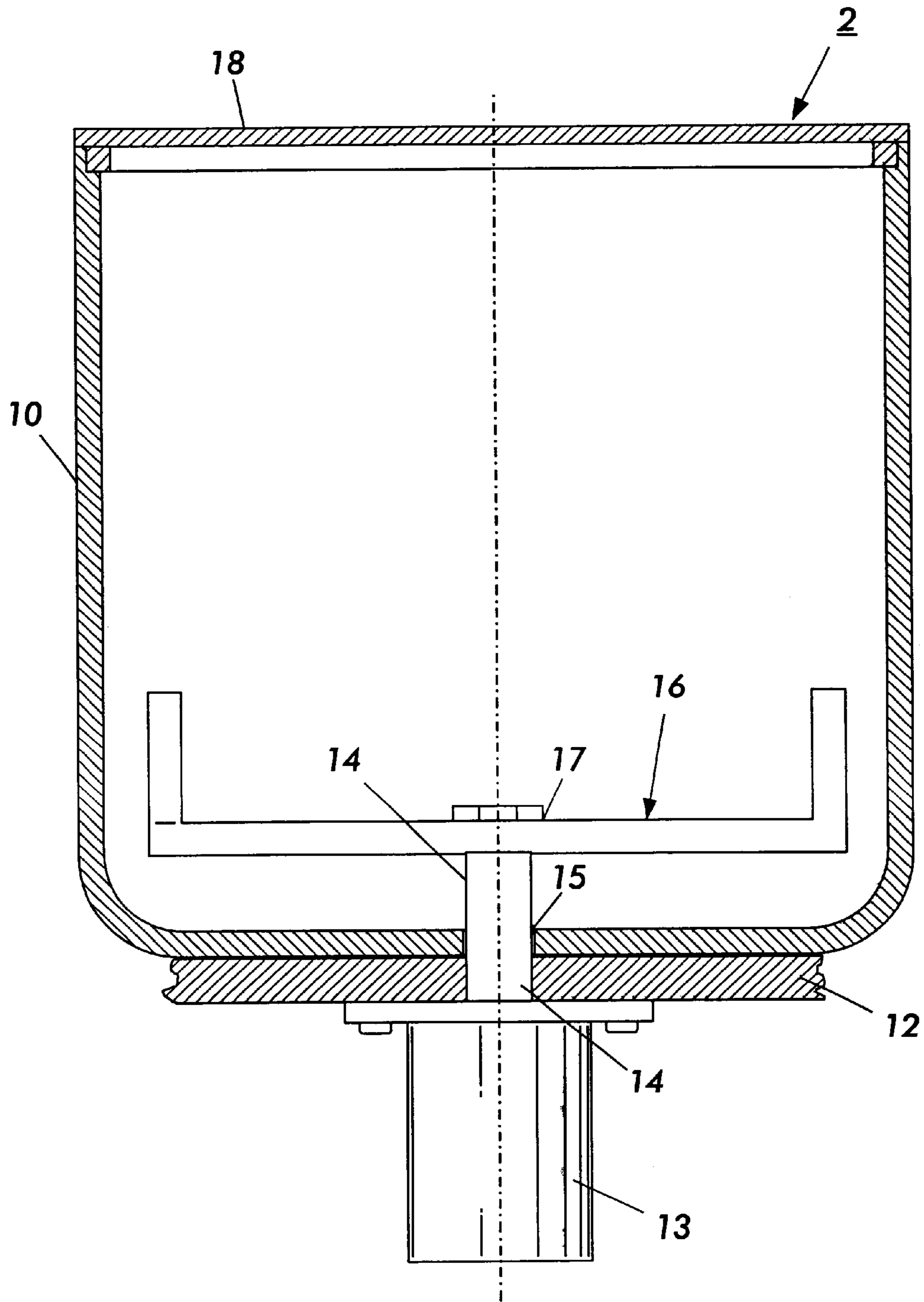
FIG. 1 PRIOR ART
