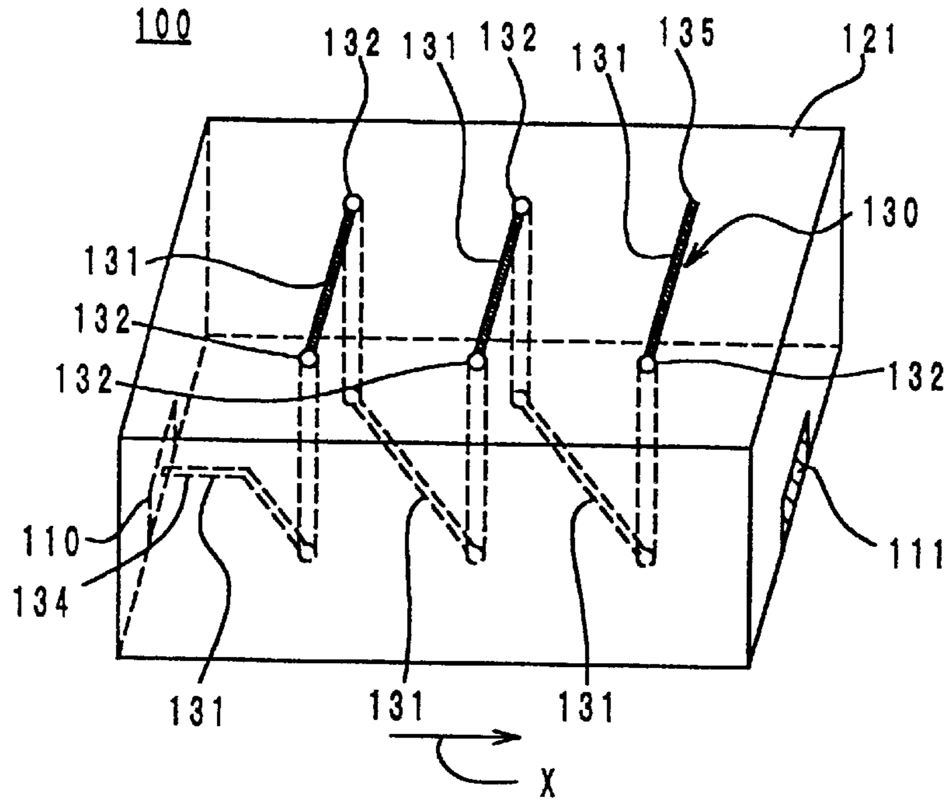
Fig. 10 PRIOR ART
