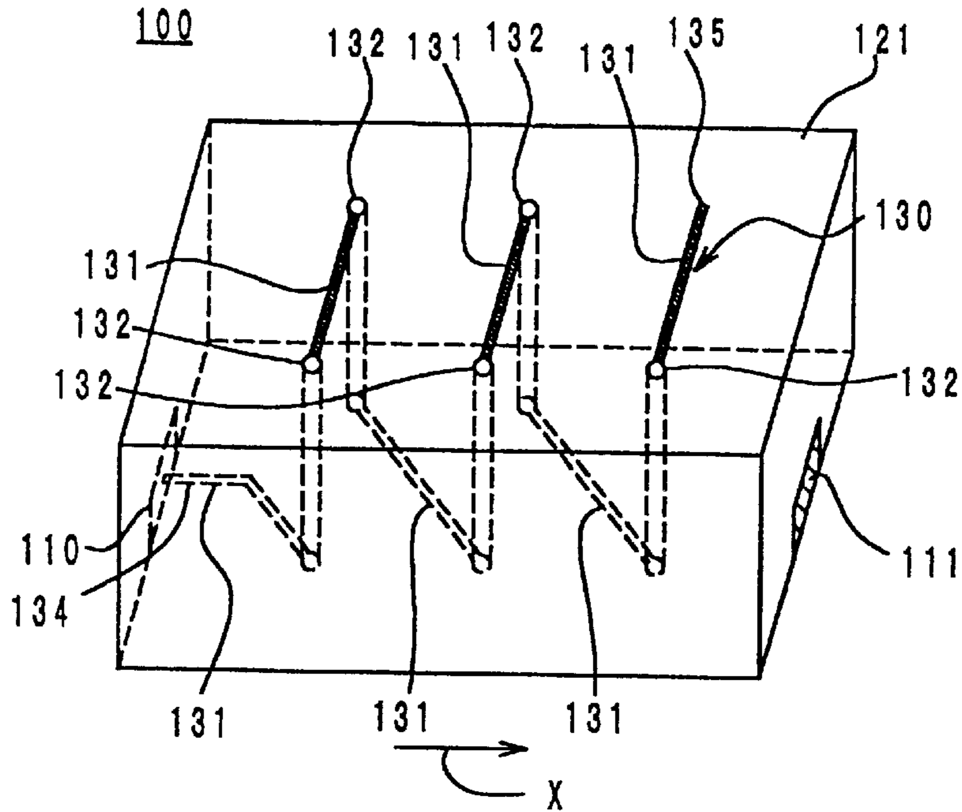
Fig. 10 PRIOR ART
