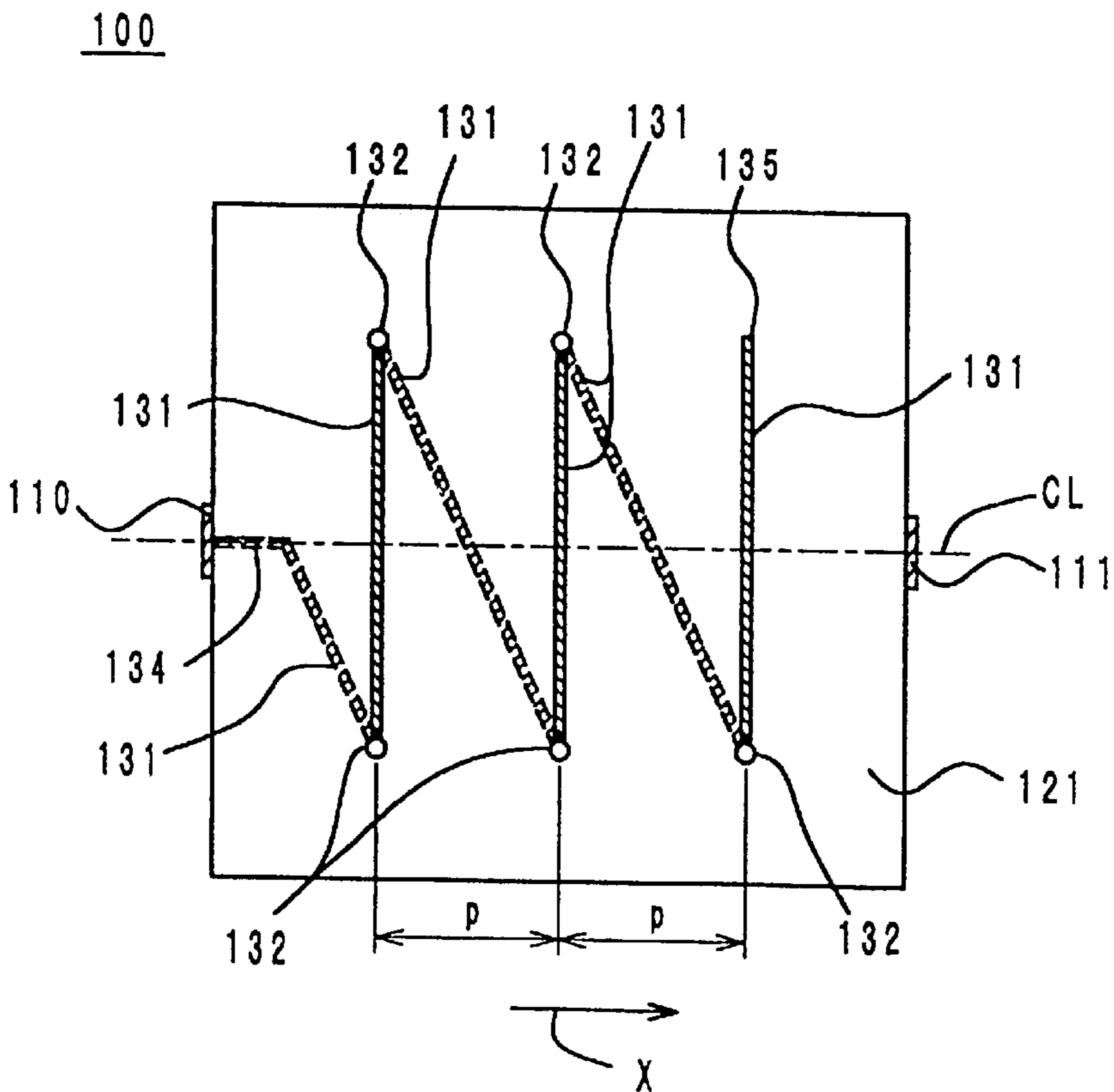
Fig. 10 PRIOR ART
