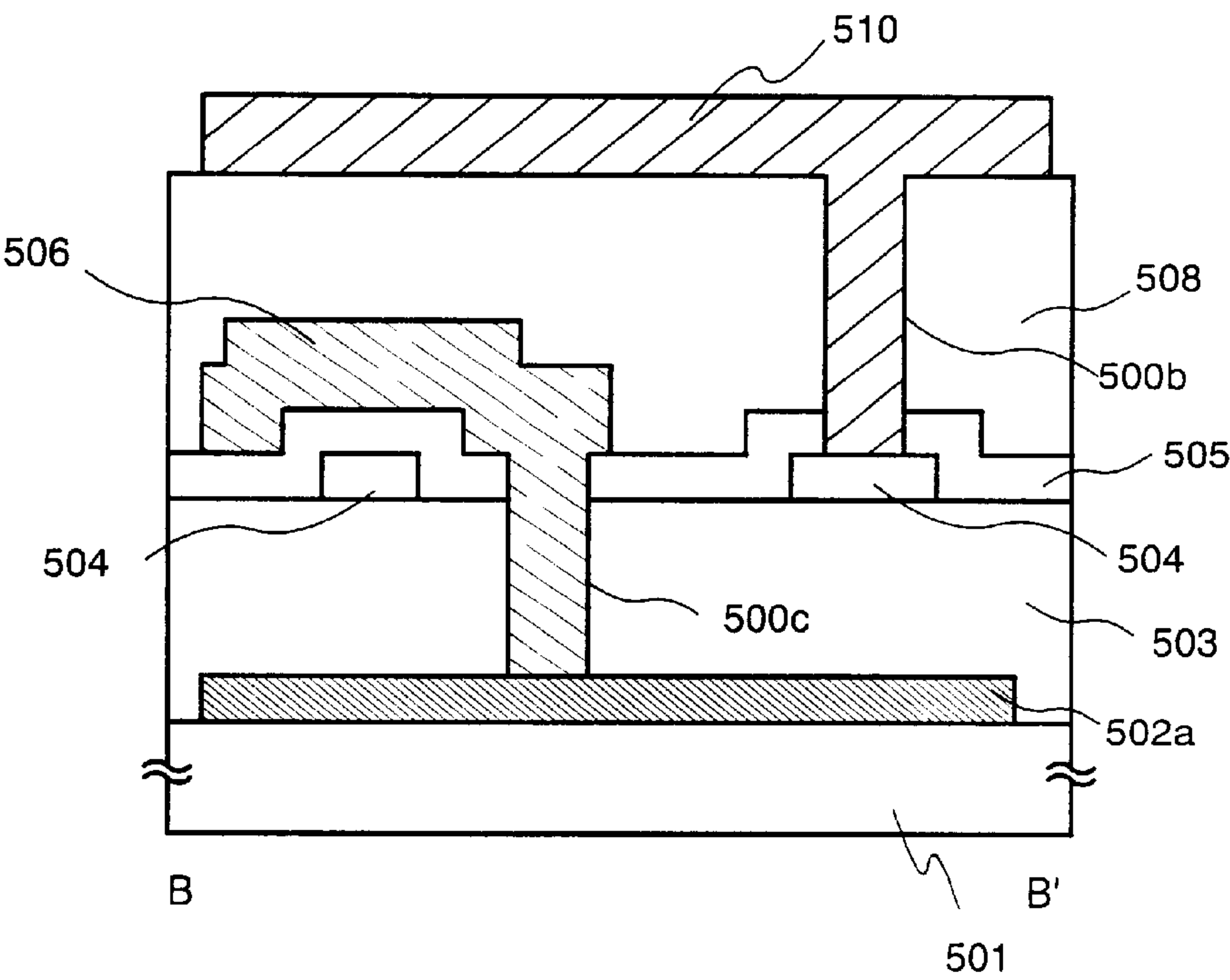
Fig. 15B B-B' Cross sectional view
