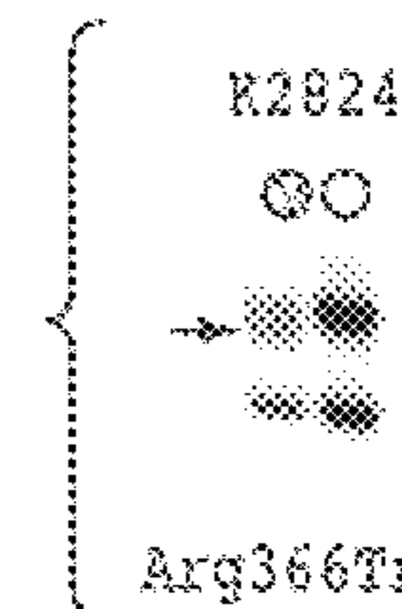
Arg366Trp FIG. 12O
