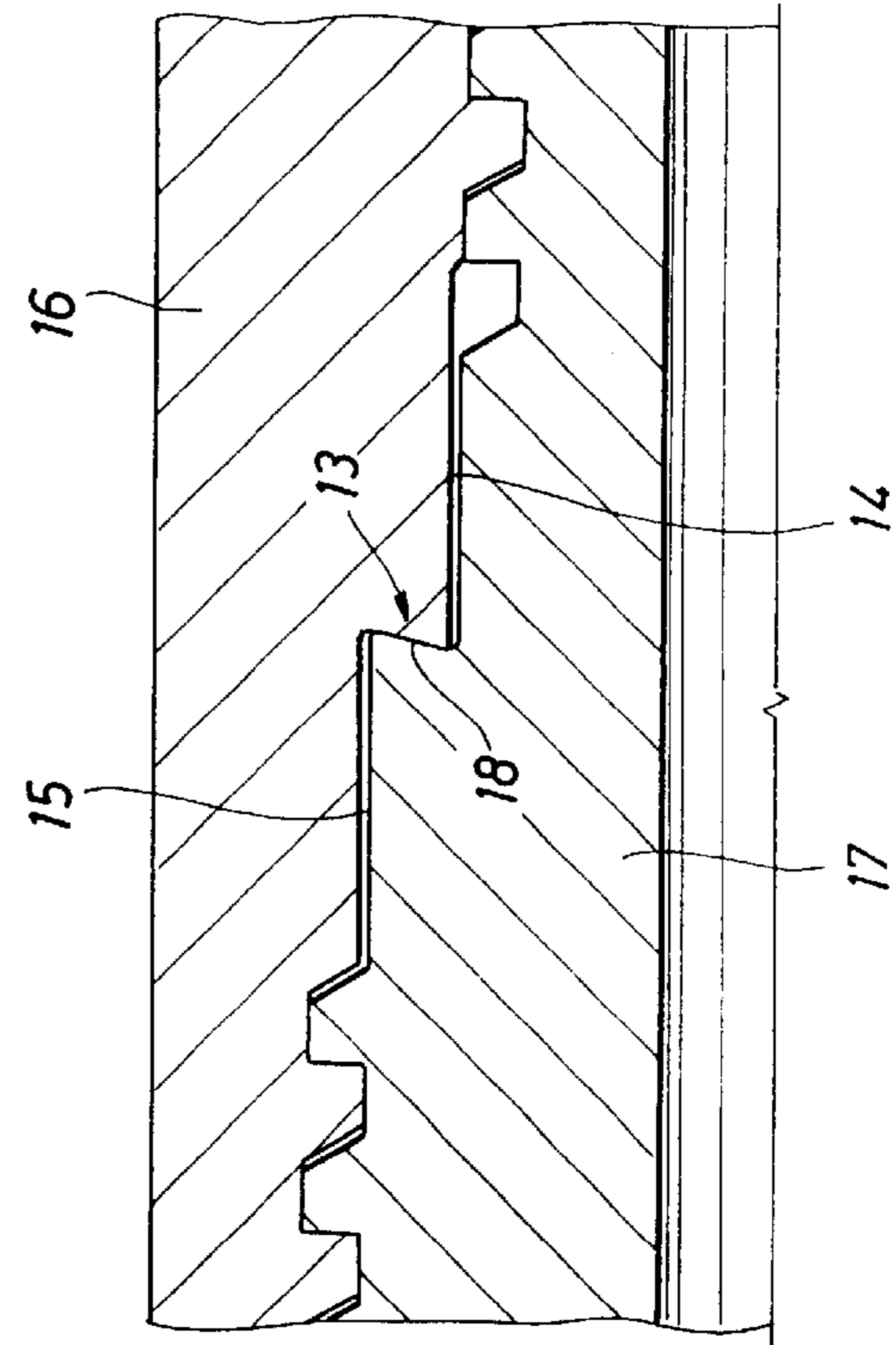
FIG. 2 (PRIOR ART)
