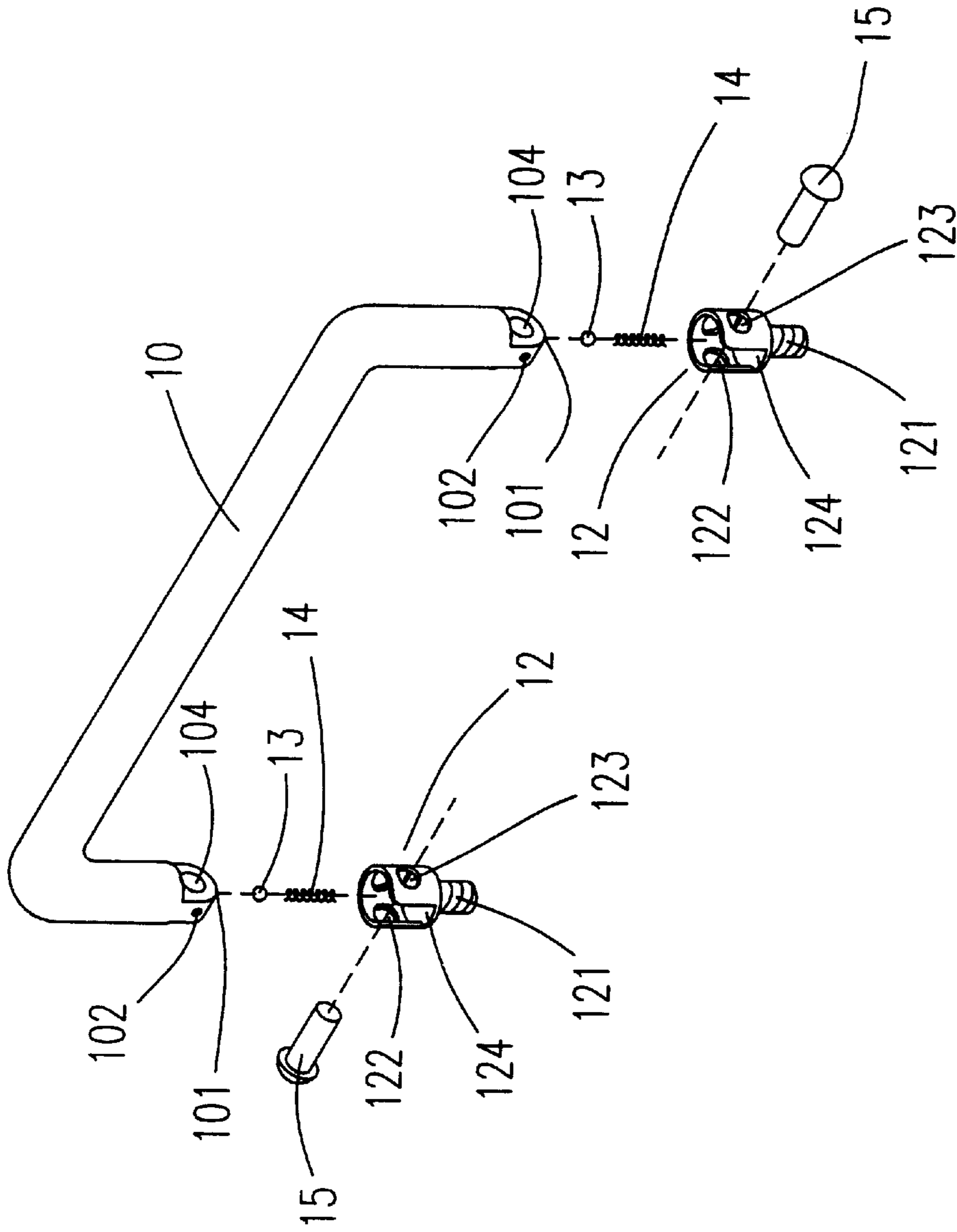
Fig. 1(a)(PRIOR ART)
