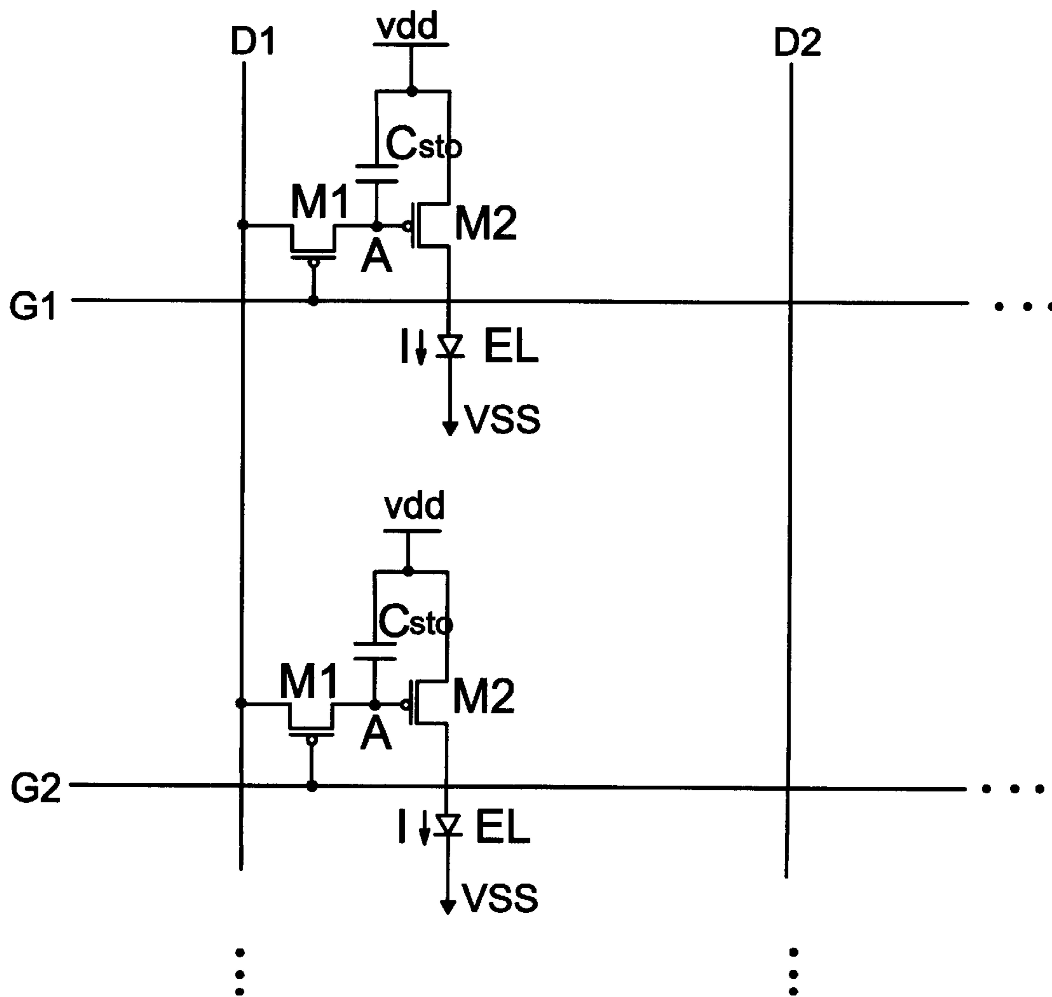
FIG. 1 RELATED ART
