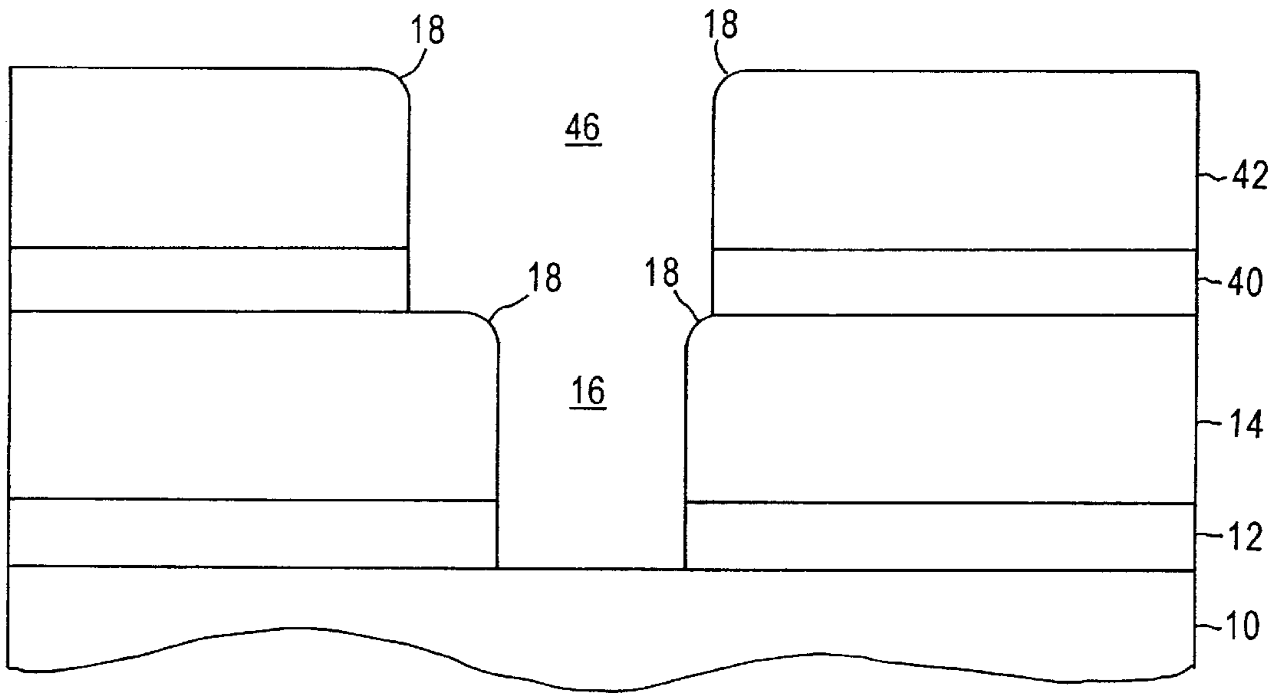
FIG. 2I (PRIOR ART)
