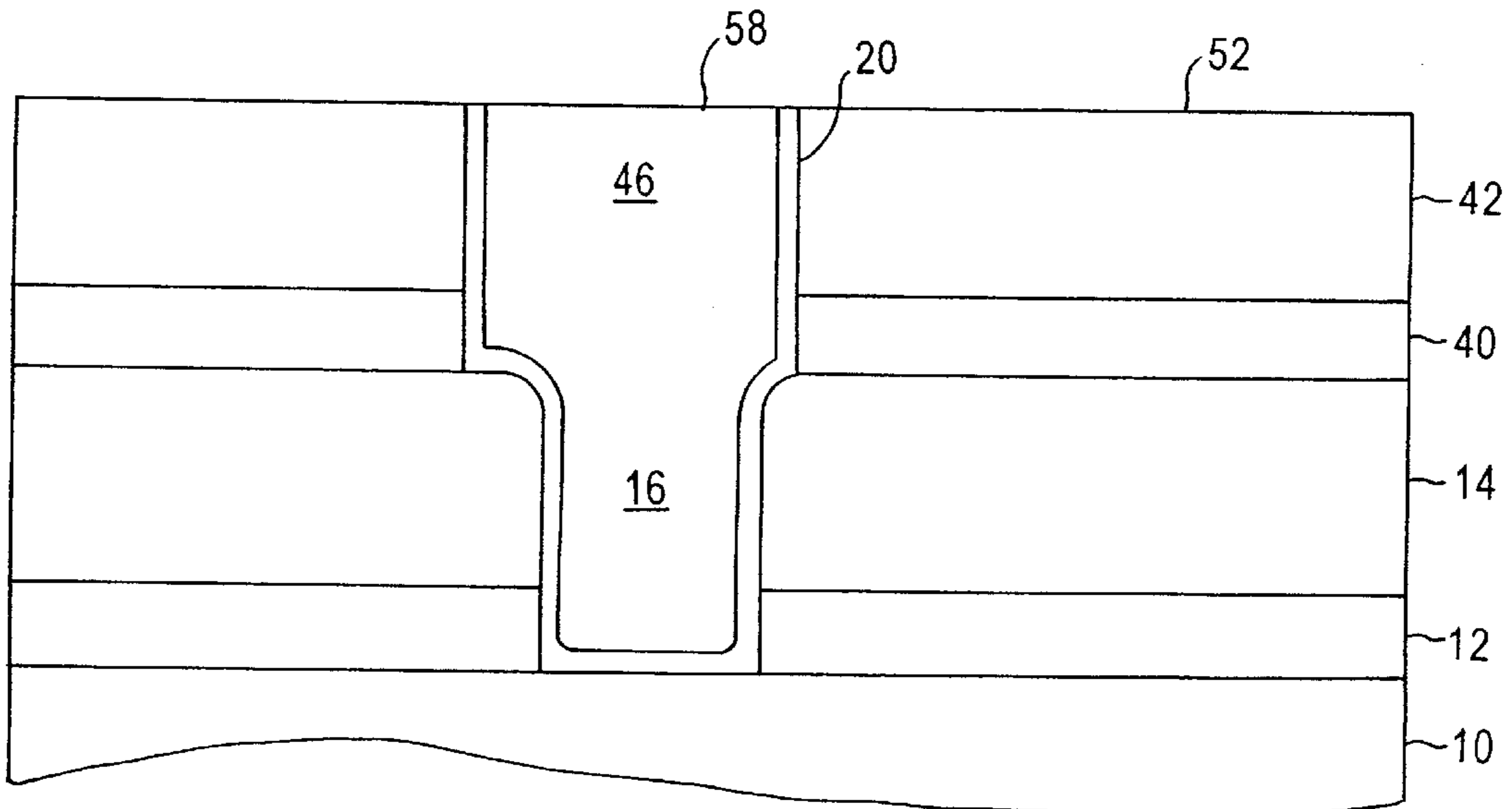
FIG. 2L (PRIOR ART)
