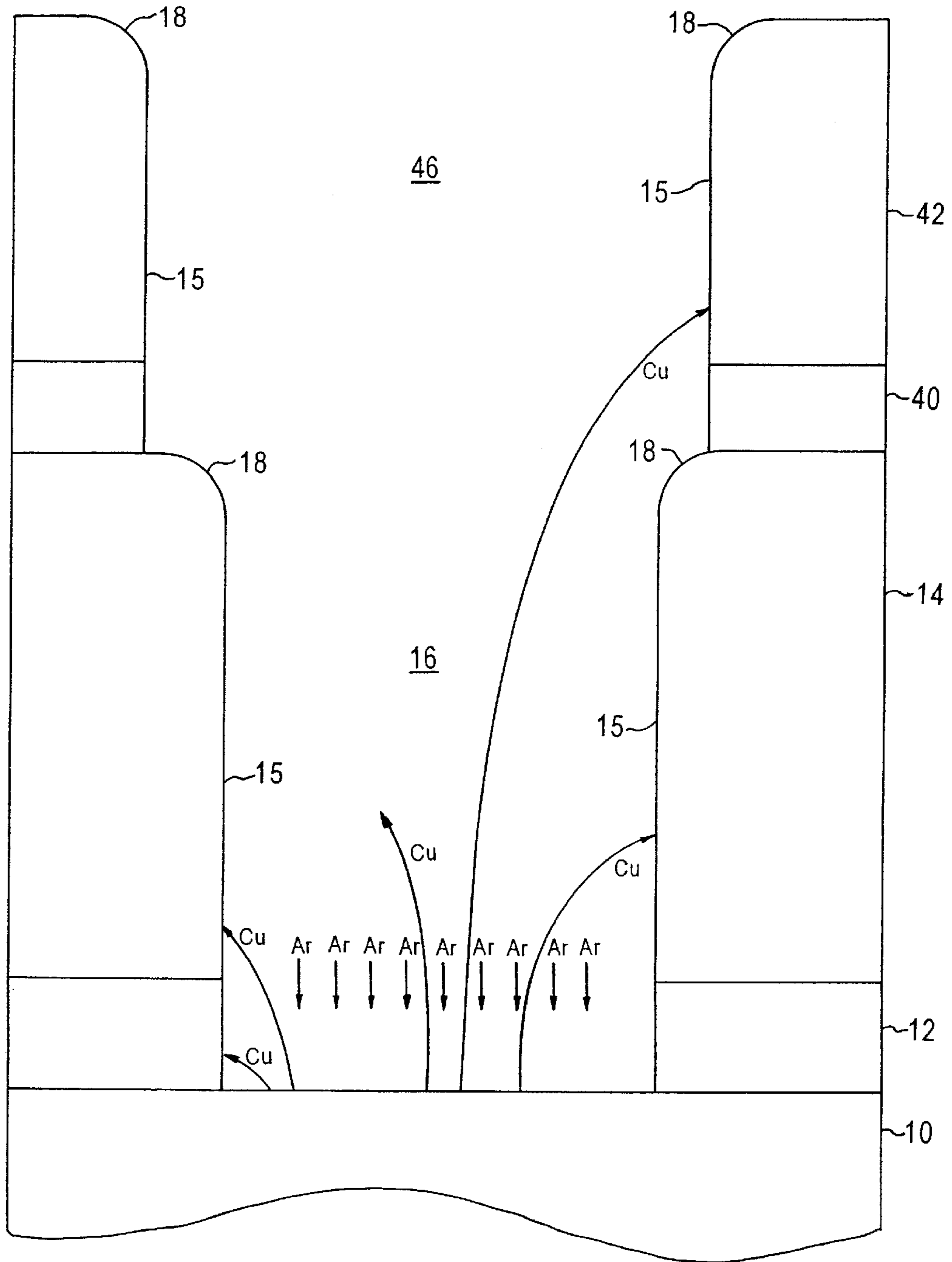
FIG. 3 (PRIOR ART)
