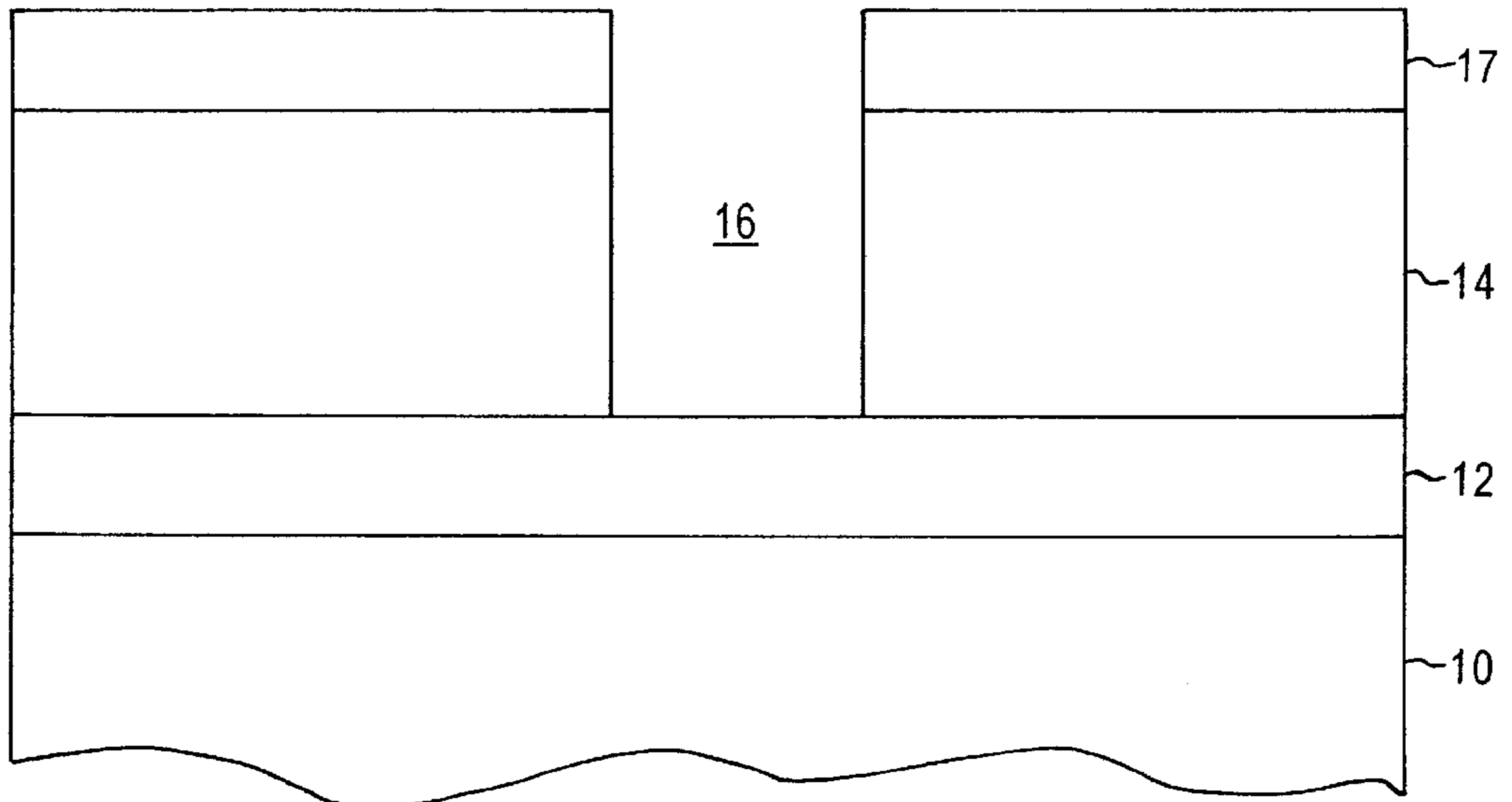
FIG. 1C (PRIOR ART)
