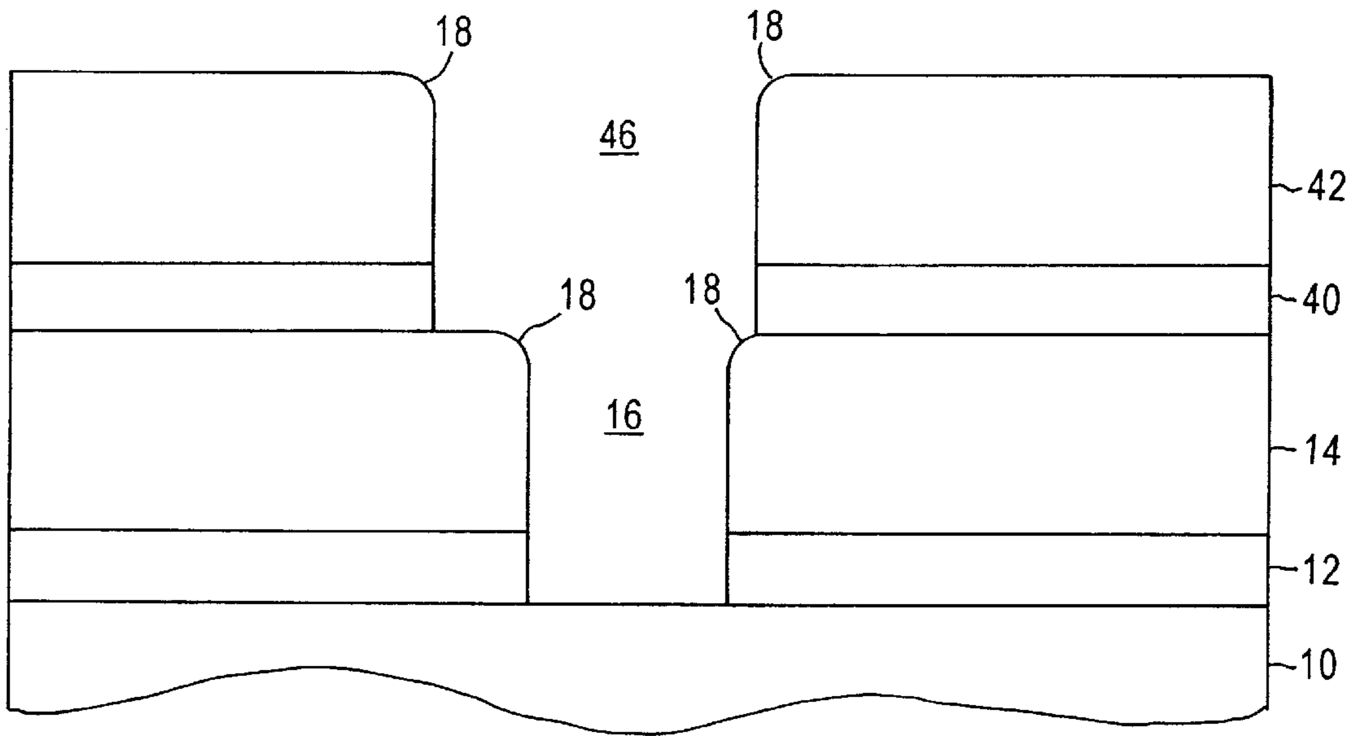
FIG. 2I (PRIOR ART)
