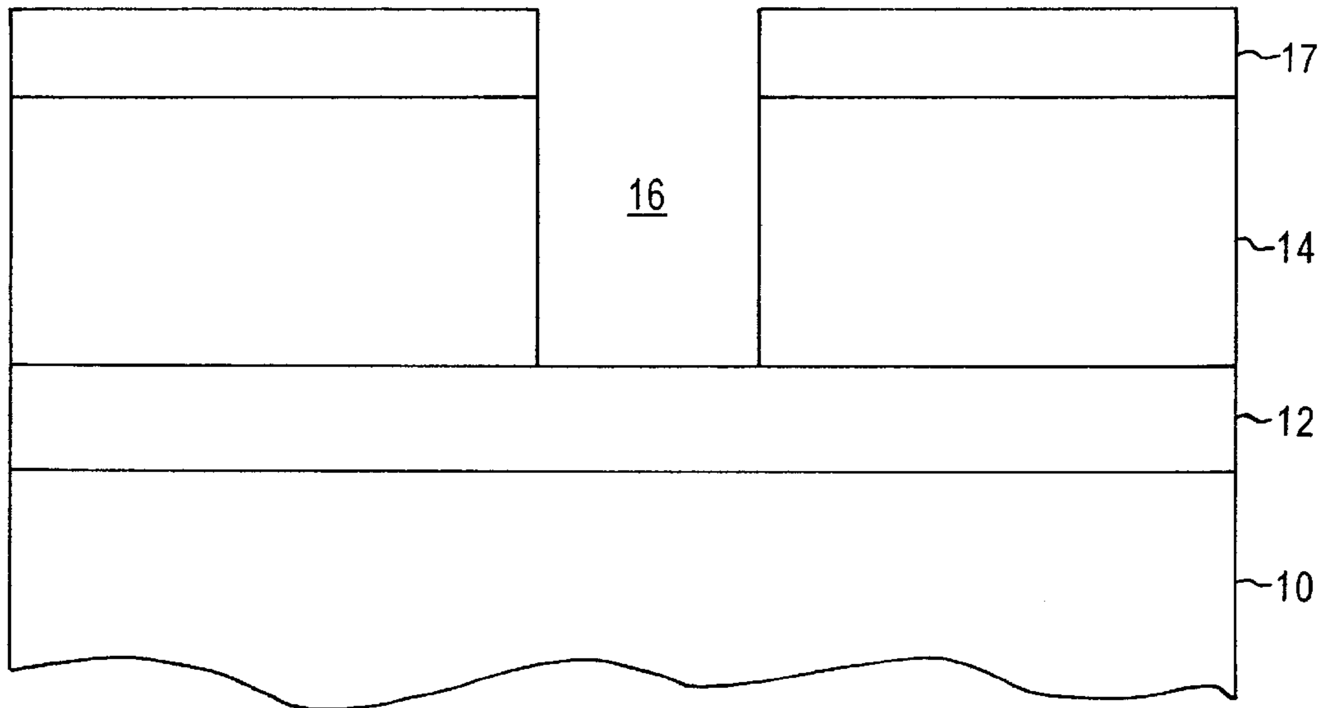
FIG. 1C (PRIOR ART)
